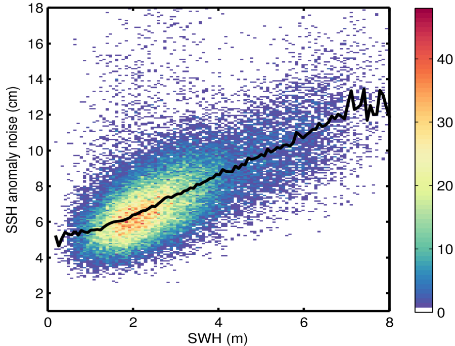
Figure 9. 2D histogram showing flag-valid SSH anomaly noise as a function of SWH for 31/10/2016. The black line denotes the median SSH anomaly noise as a function of SWH.
