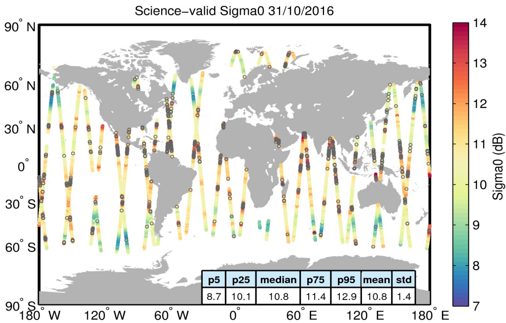
Figure 27. Geographical distribution of science-valid sigma0 data over oceans and lakes for 31/10/2016. The statistical values shown in the table refer to the sigma0 in dB and are calculated over all measurements shown in the figure. Gray circles denote records that have been rejected based on the editing criteria described in Table 4.
