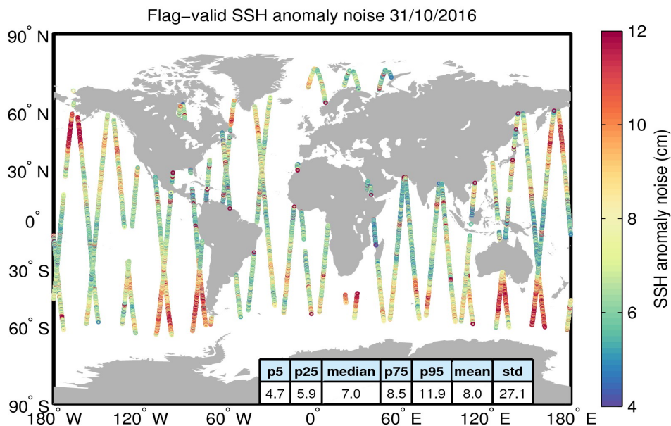
Figure 8. Geographical distribution of flag-valid 20-Hz SSH anomaly measurement noise over oceans and lakes for 31/10/2016. The statistical values shown in the table refer to the SSH anomaly noise and are calculated over all measurements shown in the figure.
