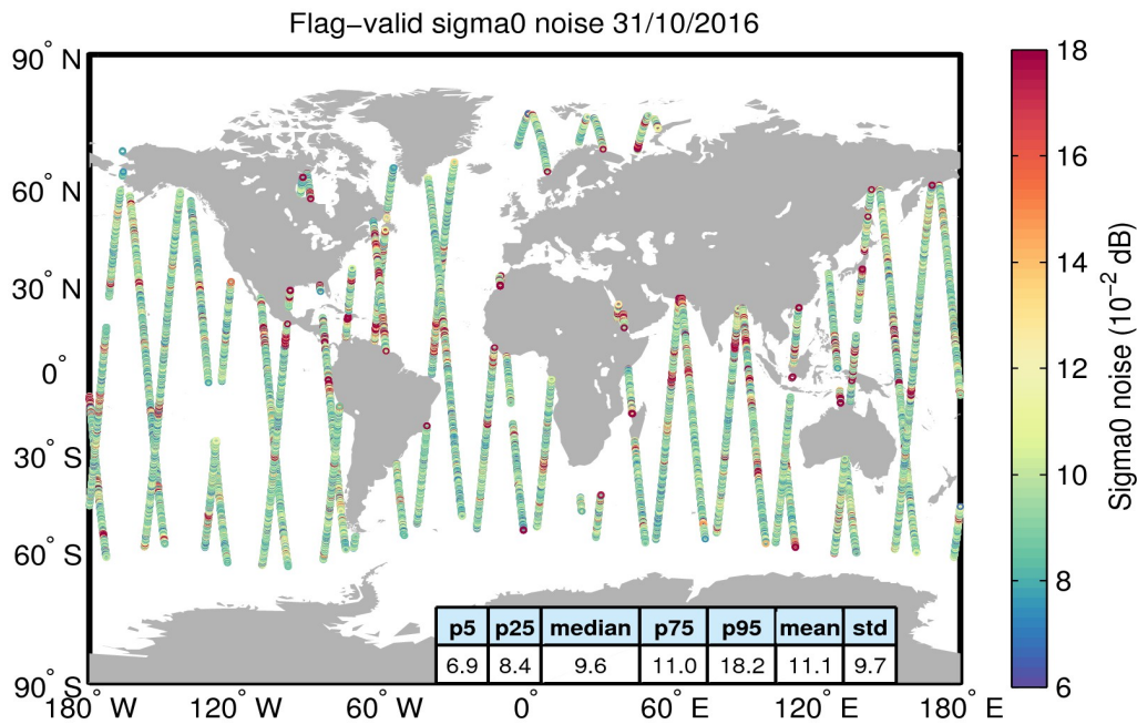
Figure 26. Geographical distribution of flag-valid 20-Hz sigma0 measurement noise over oceans and lakes for 31/10/2016. The statistical values shown in the table refer to the sigma0 noise and are calculated over all measurements shown in the figure.
