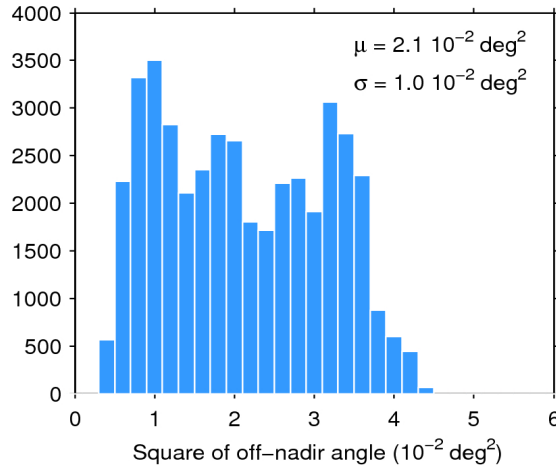
Figure 39. Histogram of flag-valid mispointing over oceans and lakes for 31/10/2016. The mean ( \mu ) and standard deviation ( \sigma ) are also shown. Note that values larger than 6 \cdot 10^{-2} \text{ deg}^2 are excluded from the histogram for the sake of readability but not from the computation of \mu and \sigma .
