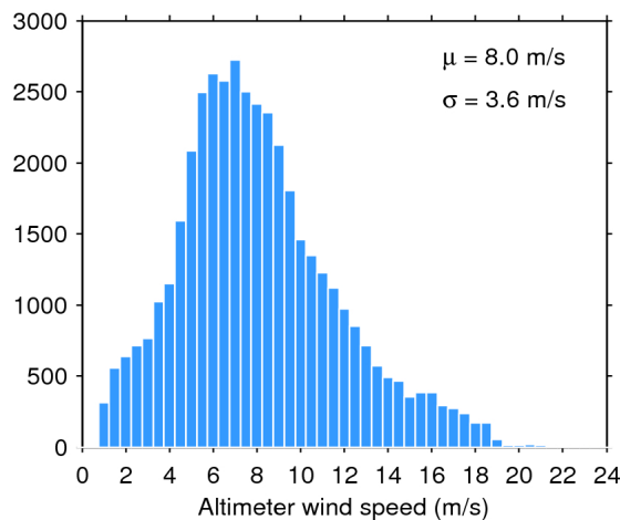
Figure 35. Histogram of science-valid wind over oceans and lakes for 31/10/2016. The mean ( \mu ) and standard deviation ( \sigma ) are also shown. Note that values larger than 24 m/s are excluded from the histogram for the sake of readability but not from the computation of \mu and \sigma .
