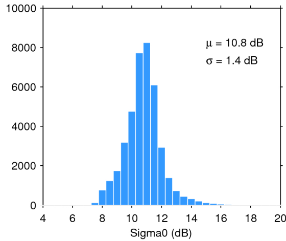
Figure 28. Histogram of science-valid sigma0 over oceans and lakes for 31/10/2016. The mean ( \mu ) and standard deviation ( \sigma ) are also shown. Note that values outside [4 20] dB are excluded from the histogram for the sake of readability but not from the computation of \mu and \sigma .
