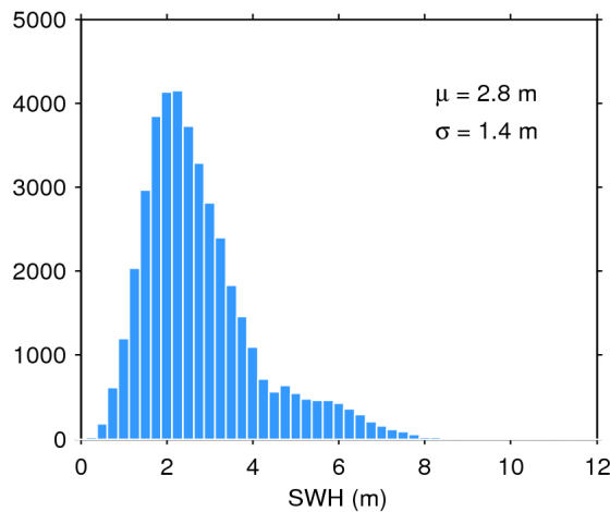
Figure 20. Histogram of science-valid SWH over oceans and lakes for 31/10/2016. The mean ( \mu ) and standard deviation ( \sigma ) are also shown. Note that values larger than 12 m are excluded from the histogram for the sake of readability but not from the computation of \mu and \sigma .
