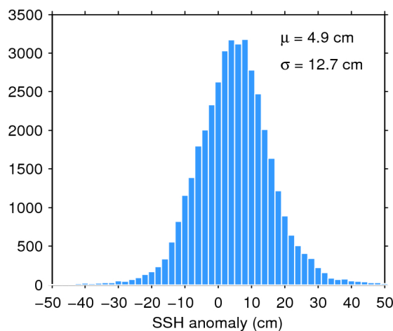
Figure 11. Histogram of science-valid SSH anomaly over oceans and lakes for 31/10/2016. The mean ( \mu ) and standard deviation ( \sigma ) are also shown. Note that values outside [-50 50] cm are excluded from the histogram for the sake of readability but not from the computation of \mu and \sigma .
