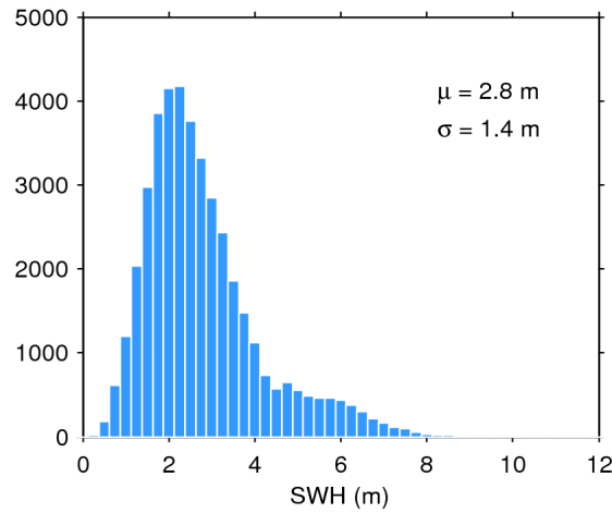
Figure 17. Histogram of flag-valid SWH over oceans and lakes for 31/10/2016. The mean ( \mu ) and standard deviation ( \sigma ) are also shown. Note that values larger than 12 m are excluded from the histogram for the sake of readability but not from the computation of \mu and \sigma .
