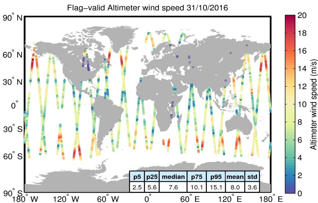
Figure 31. Geographical distribution of flag-valid wind data over oceans and lakes for 31/10/2016. The statistical values shown in the table refer to the wind in m/s and are calculated over all measurements shown in the figure.
