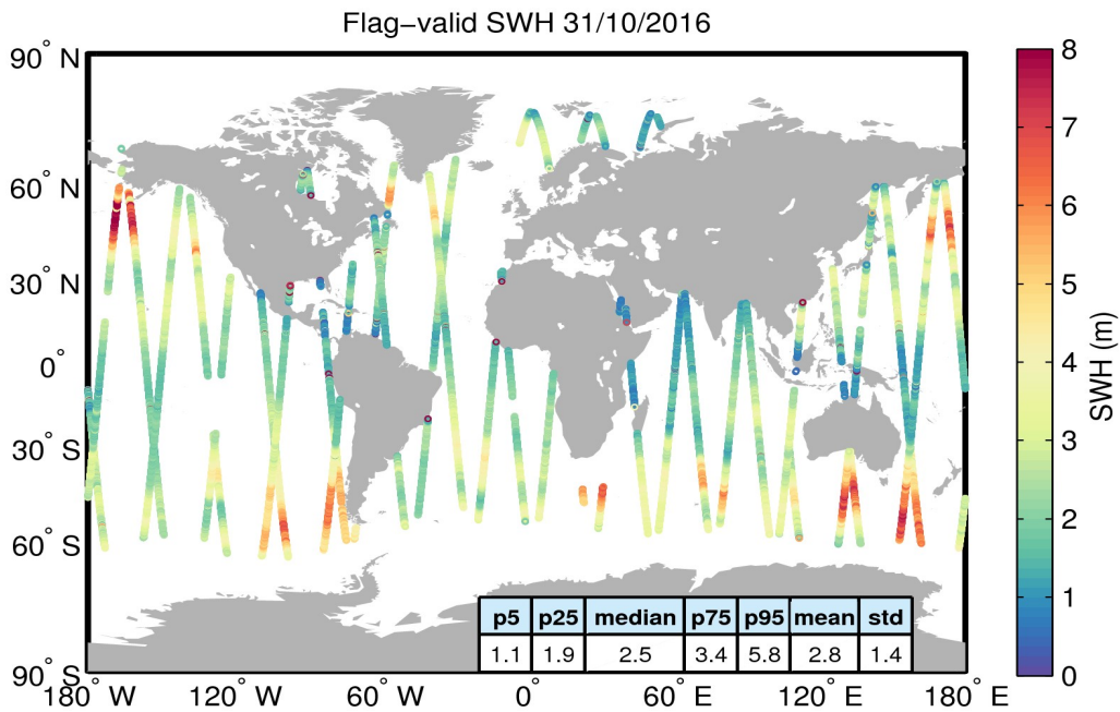
Figure 15. Geographical distribution of flag-valid SWH data over oceans and lakes for 31/10/2016. The statistical values shown in the table refer to the SWH in m and are calculated over all measurements shown in the figure.
