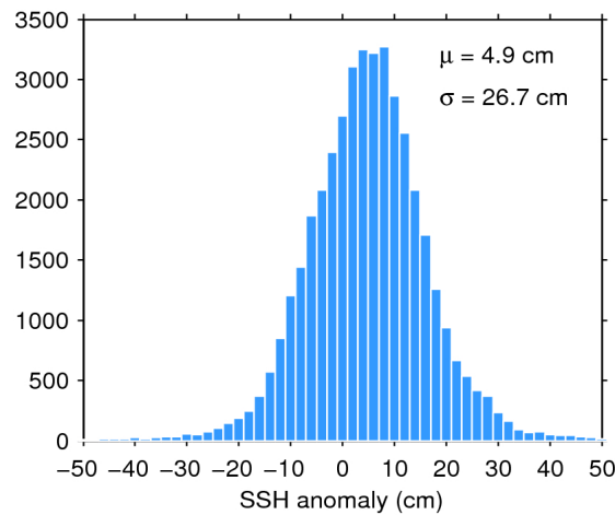
Figure 7. Histogram of flag-valid SSH anomaly over oceans and lakes for 31/10/2016. The mean ( \mu ) and standard deviation ( \sigma ) are also shown. Note that values outside [-50\ 50] cm are excluded from the histogram for the sake of readability but not from the computation of \mu and \sigma .
