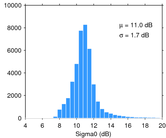
Figure 25. Histogram of flag-valid sigma0 over oceans and lakes for 31/10/2016. The mean ( \mu ) and standard deviation ( \sigma ) are also shown. Note that values outside [4 20] dB are excluded from the histogram for the sake of readability but not from the computation of \mu and \sigma .
