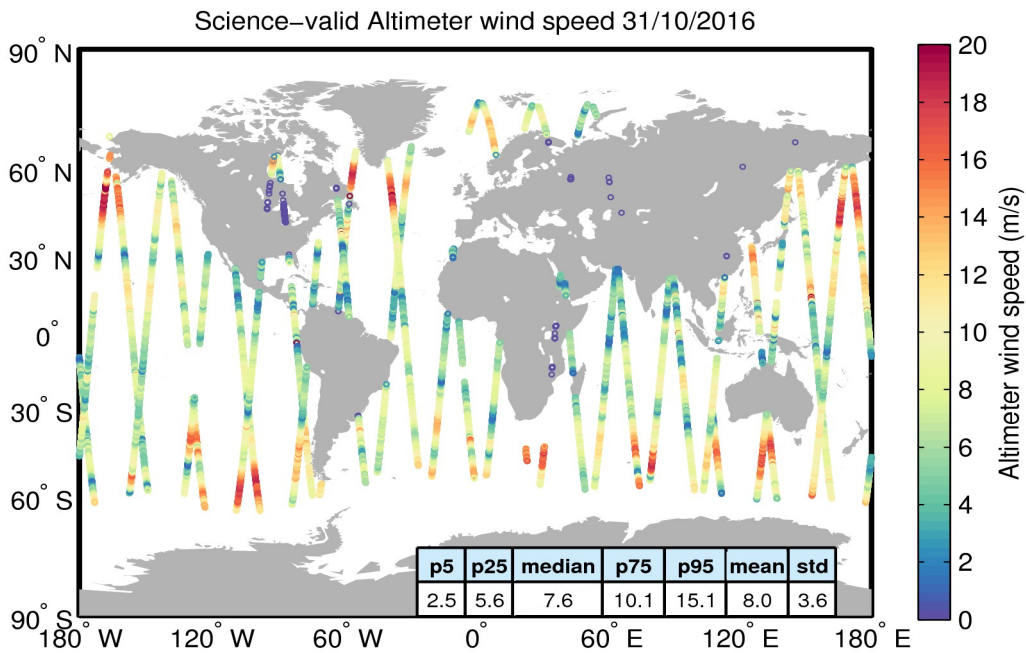
Figure 34. Geographical distribution of science-valid wind data over oceans and lakes for 31/10/2016. The statistical values shown in the table refer to the wind in m/s and are calculated over all measurements shown in the figure. Gray circles denote records that have been rejected based on the editing criteria described in Table 5.
