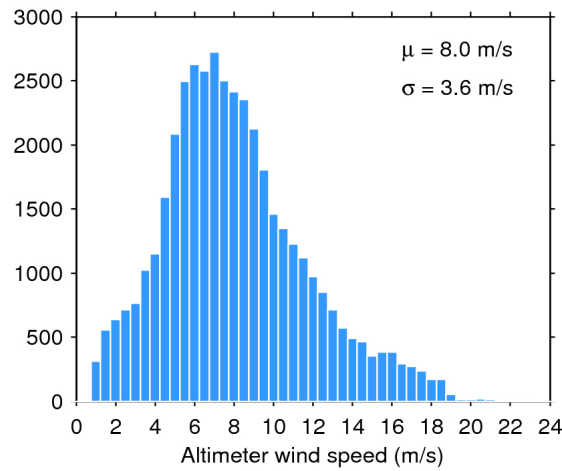
Figure 33. Histogram of flag-valid wind over oceans and lakes for 31/10/2016. The mean ( \mu ) and standard deviation ( \sigma ) are also shown. Note that values larger than 24 m/s are excluded from the histogram for the sake of readability but not from the computation of \mu and \sigma .
