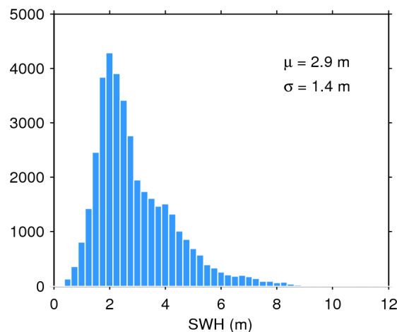
Figure 20. Histogram of science-valid SWH over oceans and lakes for 30/10/2016. The mean ( \mu ) and standard deviation ( \sigma ) are also shown. Note that values larger than 12 m are excluded from the histogram for the sake of readability but not from the computation of \mu and \sigma .
