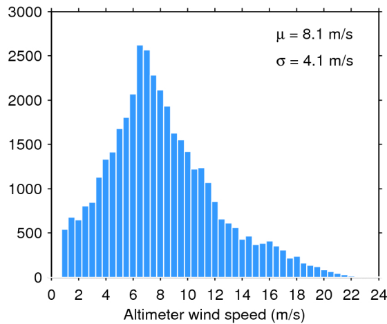
Figure 33. Histogram of flag-valid wind over oceans and lakes for 30/10/2016. The mean ( \mu ) and standard deviation ( \sigma ) are also shown. Note that values larger than 24 m/s are excluded from the histogram for the sake of readability but not from the computation of \mu and \sigma .
