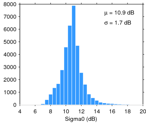
Figure 28. Histogram of science-valid sigma0 over oceans and lakes for 30/10/2016. The mean ( \mu ) and standard deviation ( \sigma ) are also shown. Note that values outside [4 20] dB are excluded from the histogram for the sake of readability but not from the computation of \mu and \sigma .
