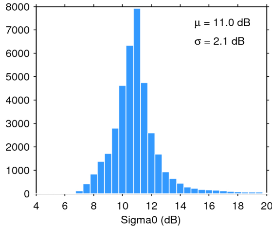
Figure 25. Histogram of flag-valid sigma0 over oceans and lakes for 30/10/2016. The mean ( \mu ) and standard deviation ( \sigma ) are also shown. Note that values outside [4 20] dB are excluded from the histogram for the sake of readability but not from the computation of \mu and \sigma .
