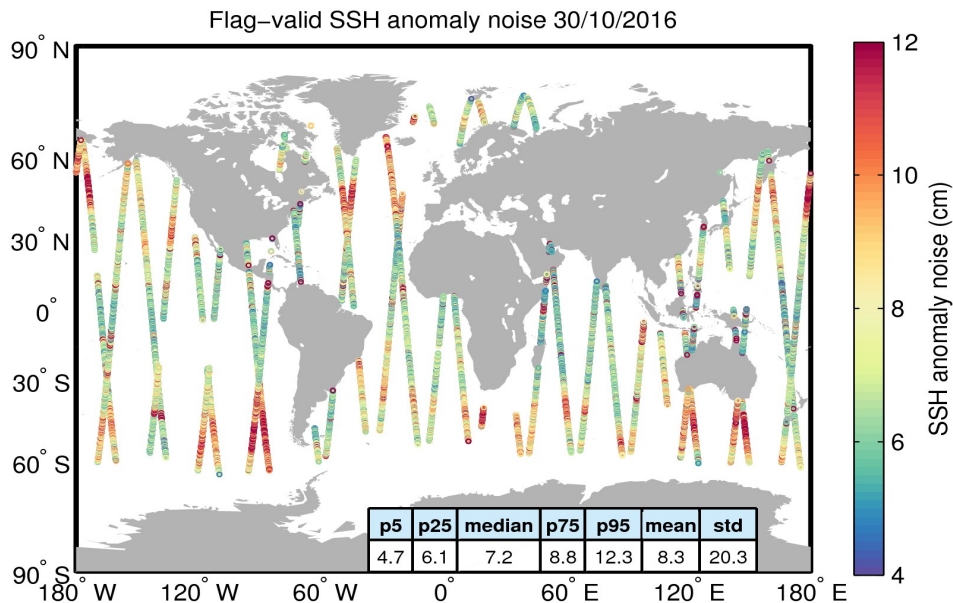
Figure 8. Geographical distribution of flag-valid 20-Hz SSH anomaly measurement noise over oceans and lakes for 30/10/2016. The statistical values shown in the table refer to the SSH anomaly noise and are calculated over all measurements shown in the figure.
