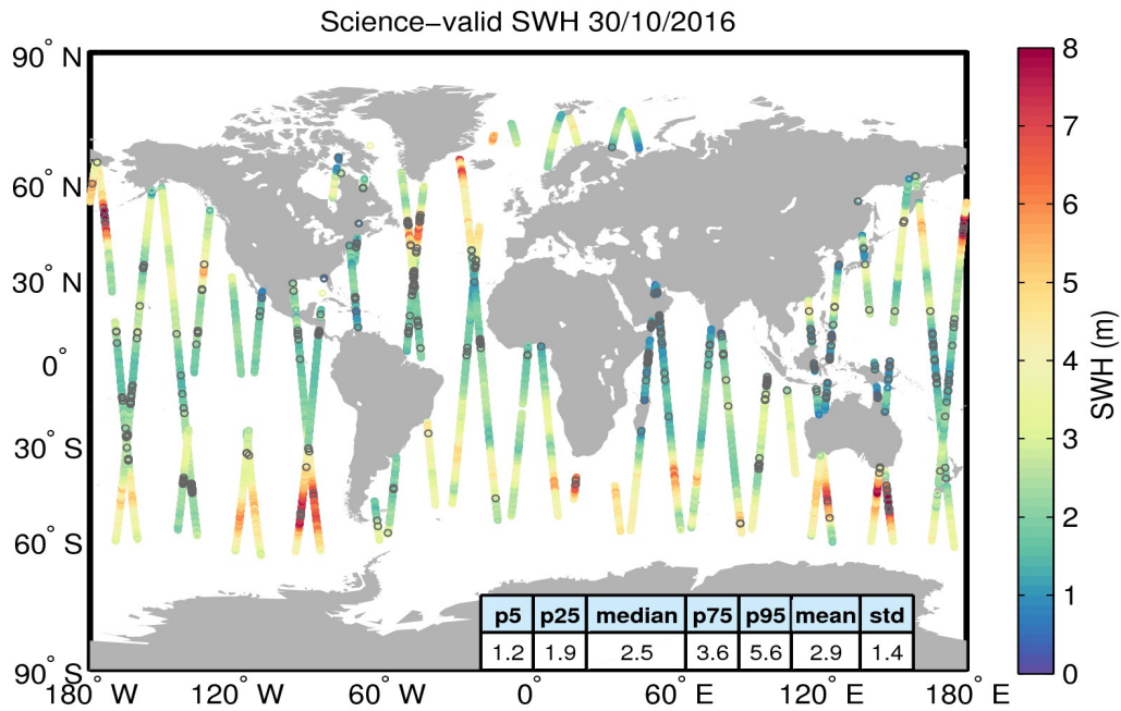
Figure 19. Geographical distribution of science-valid SWH data over oceans and lakes for 30/10/2016. The statistical values shown in the table refer to the SWH in m and are calculated over all measurements shown in the figure. Gray circles denote records that have been rejected based on the editing criteria described in Table 3.
