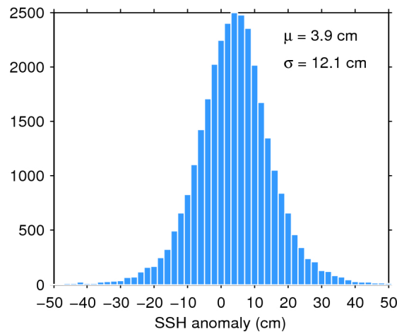
Figure 11. Histogram of science-valid SSH anomaly over oceans and lakes for 30/10/2016. The mean ( \mu ) and standard deviation ( \sigma ) are also shown. Note that values outside [-50 50] cm are excluded from the histogram for the sake of readability but not from the computation of \mu and \sigma .
