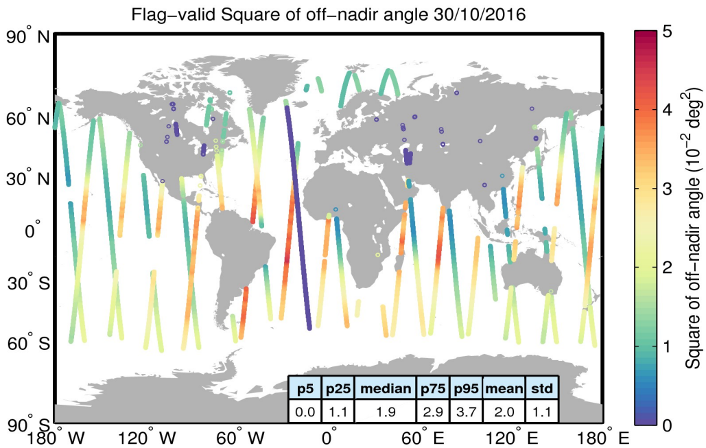
Figure 37. Geographical distribution of flag-valid mispointing data over oceans and lakes for 30/10/2016. The statistical values shown in the table refer to the mispointing in 10^{-2} deg 2 and are calculated over all measurements shown in the figure.
