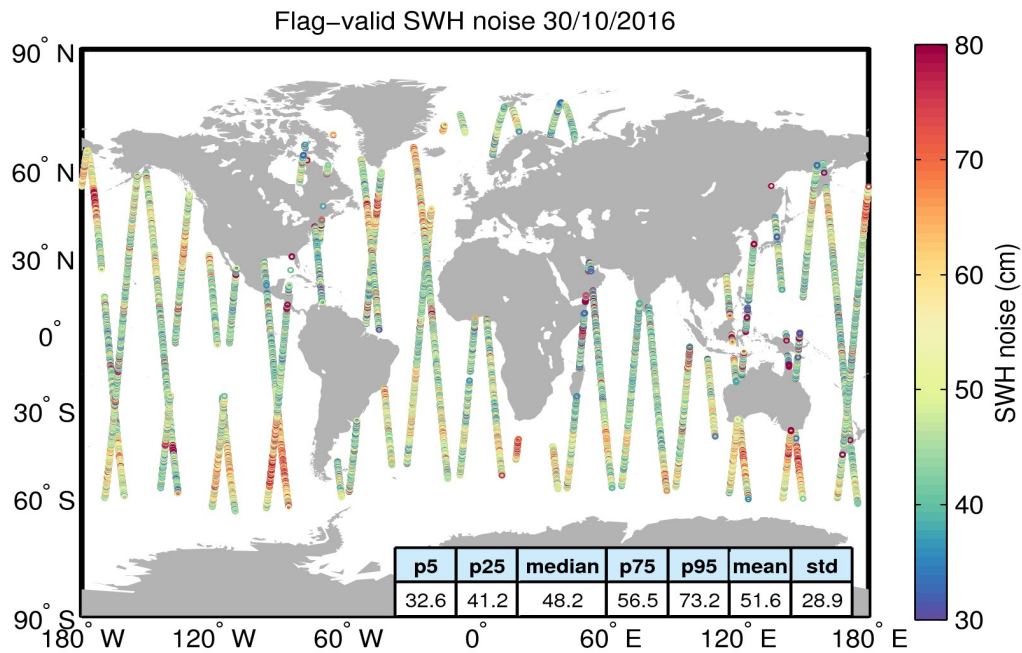
Figure 18. Geographical distribution of flag-valid 20-Hz SWH measurement noise over oceans and lakes for 30/10/2016. The statistical values shown in the table refer to the SWH noise and are calculated over all measurements shown in the figure.
