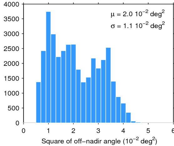
Figure 39. Histogram of flag-valid mispointing over oceans and lakes for 30/10/2016. The mean ( \mu ) and standard deviation ( \sigma ) are also shown. Note that values larger than 6 \cdot 10^{-2} \text{ deg}^2 are excluded from the histogram for the sake of readability but not from the computation of \mu and \sigma .
