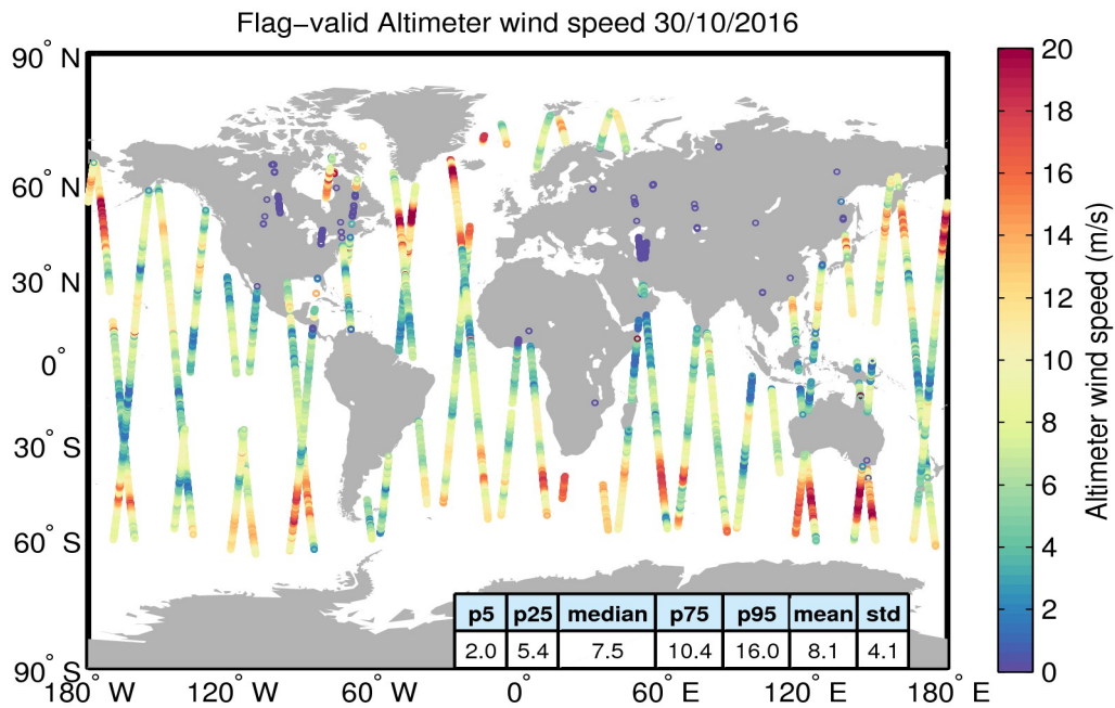
Figure 31. Geographical distribution of flag-valid wind data over oceans and lakes for 30/10/2016. The statistical values shown in the table refer to the wind in m/s and are calculated over all measurements shown in the figure.
