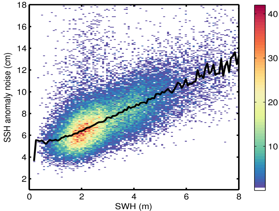
Figure 9. 2D histogram showing flag-valid SSH anomaly noise as a function of SWH for 30/10/2016. The black line denotes the median SSH anomaly noise as a function of SWH.
