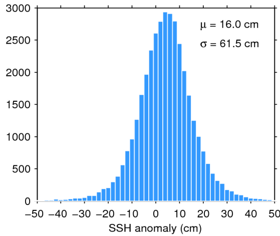
Figure 7. Histogram of flag-valid SSH anomaly over oceans and lakes for 30/10/2016. The mean ( \mu ) and standard deviation ( \sigma ) are also shown. Note that values outside [-50 50] cm are excluded from the histogram for the sake of readability but not from the computation of \mu and \sigma .
