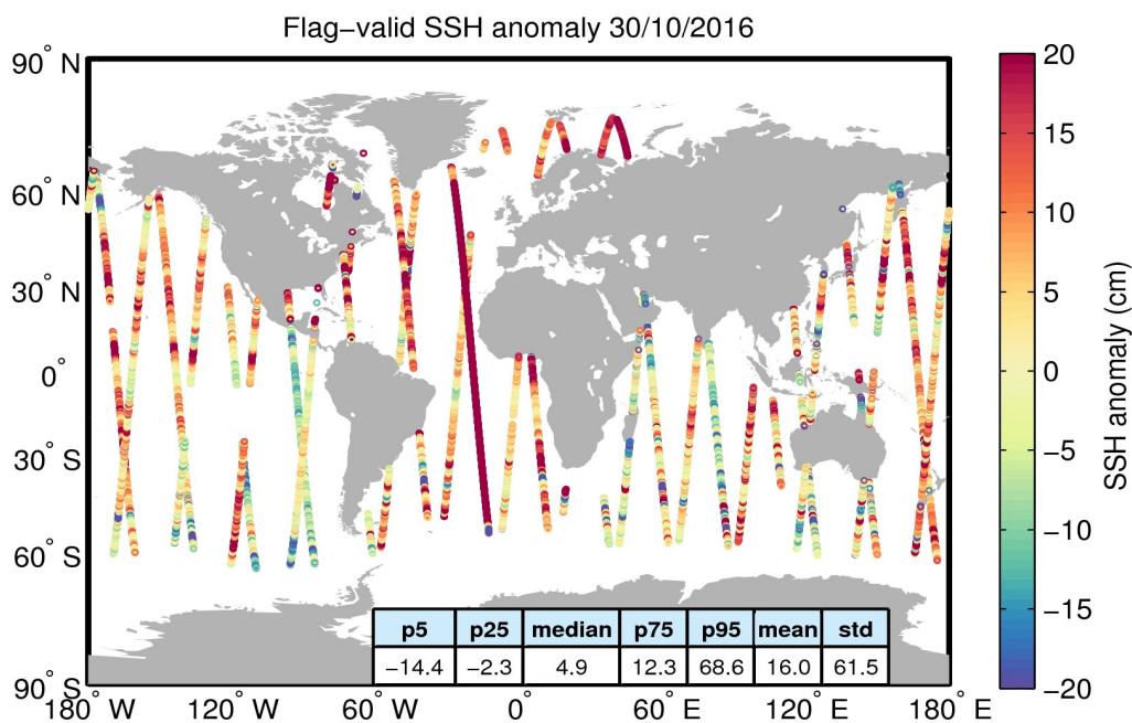
Figure 5. Geographical distribution of flag-valid 1-Hz SSH anomaly data over oceans and lakes for 30/10/2016. The statistical values shown in the table refer to the SSH anomaly in cm and are calculated over all measurements shown in the figure.
