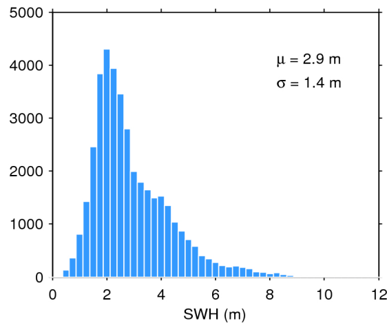
Figure 17. Histogram of flag-valid SWH over oceans and lakes for 30/10/2016. The mean ( \mu ) and standard deviation ( \sigma ) are also shown. Note that values larger than 12 m are excluded from the histogram for the sake of readability but not from the computation of \mu and \sigma .
