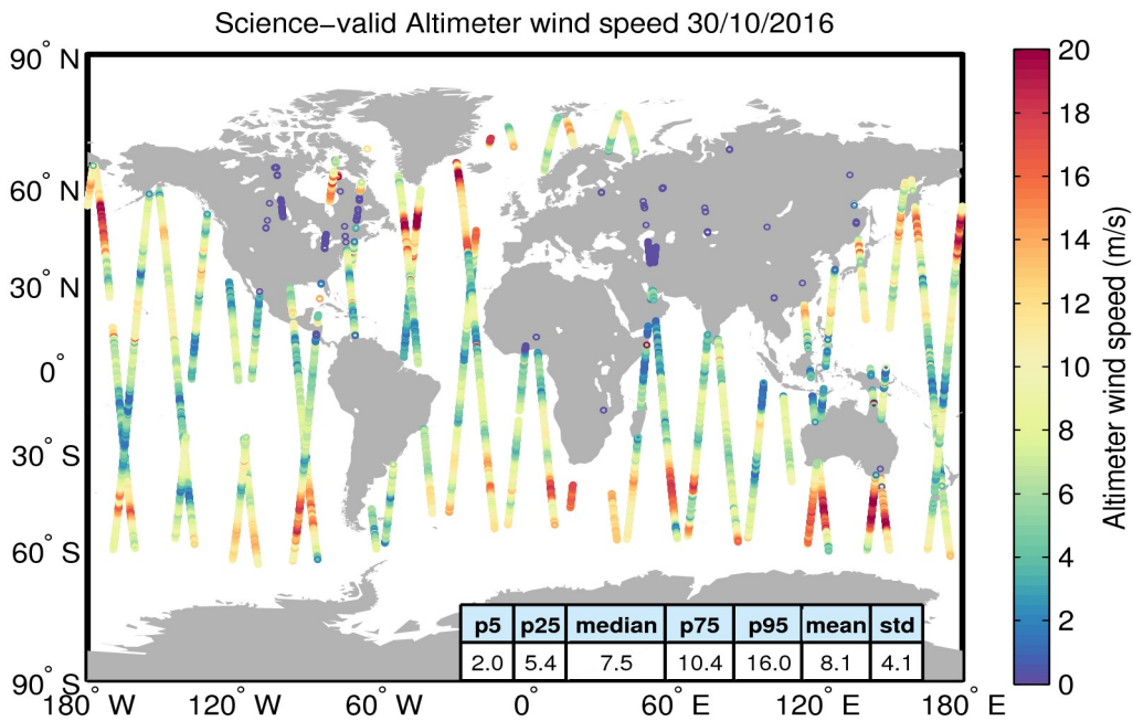
Figure 34. Geographical distribution of science-valid wind data over oceans and lakes for 30/10/2016. The statistical values shown in the table refer to the wind in m/s and are calculated over all measurements shown in the figure. Gray circles denote records that have been rejected based on the editing criteria described in Table 5.
