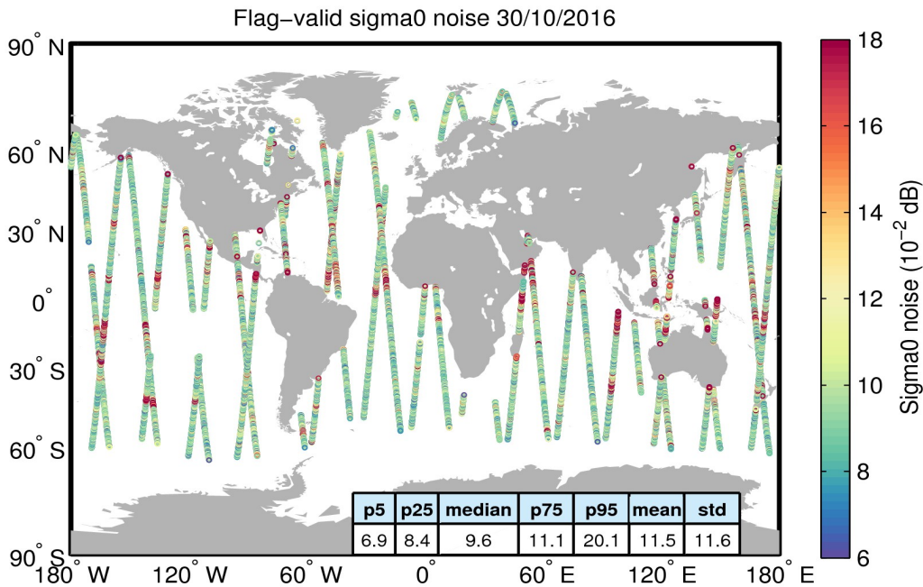
Figure 26. Geographical distribution of flag-valid 20-Hz sigma0 measurement noise over oceans and lakes for 30/10/2016. The statistical values shown in the table refer to the sigma0 noise and are calculated over all measurements shown in the figure.
