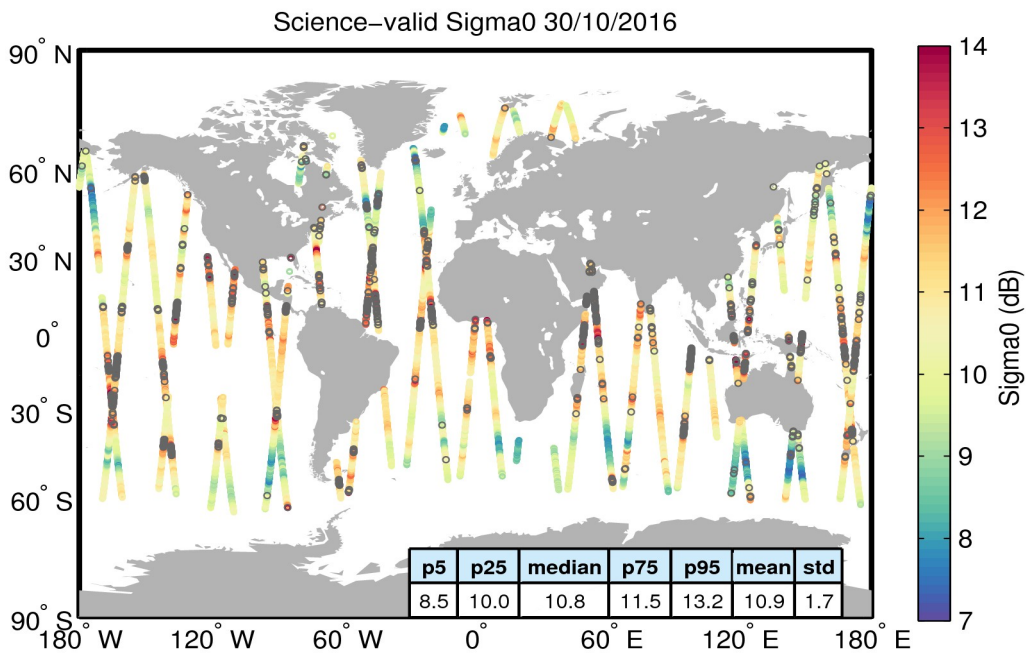
Figure 27. Geographical distribution of science-valid sigma0 data over oceans and lakes for 30/10/2016. The statistical values shown in the table refer to the sigma0 in dB and are calculated over all measurements shown in the figure. Gray circles denote records that have been rejected based on the editing criteria described in Table 4.
