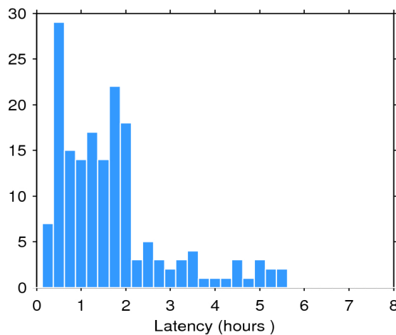
Figure 2. Histogram of the data latency for 30/10/2016. The y-axis denotes the number of files that are made available with a delay of x-hours with respect to the mean time of the records stored in the file.
