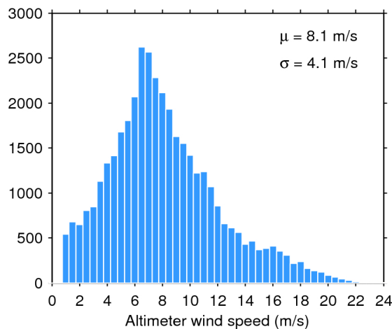
Figure 35. Histogram of science-valid wind over oceans and lakes for 30/10/2016. The mean ( \mu ) and standard deviation ( \sigma ) are also shown. Note that values larger than 24 m/s are excluded from the histogram for the sake of readability but not from the computation of \mu and \sigma .
