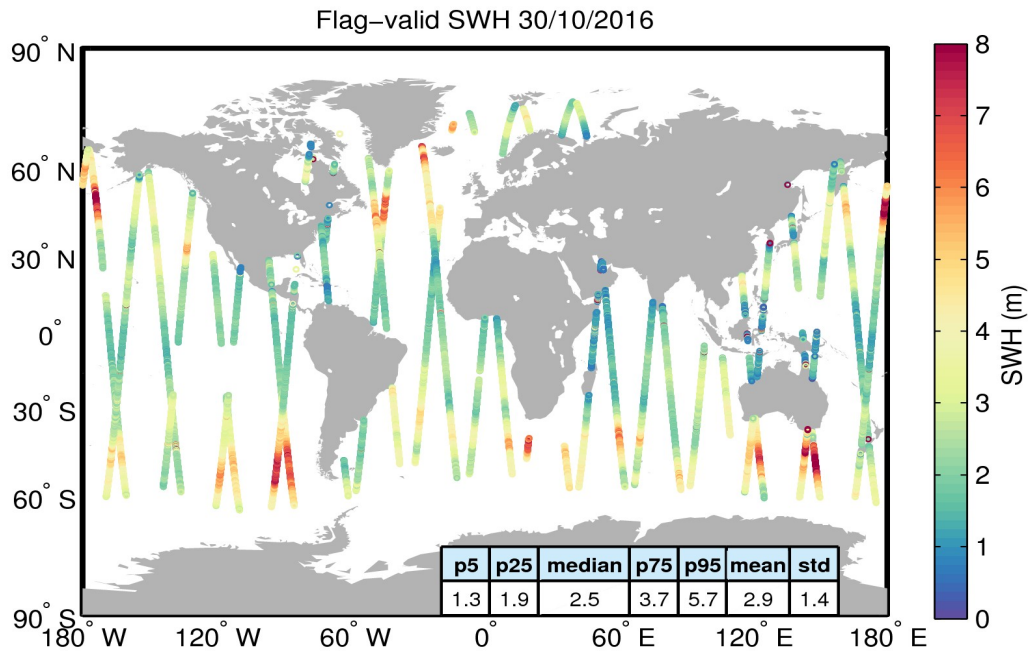
Figure 15. Geographical distribution of flag-valid SWH data over oceans and lakes for 30/10/2016. The statistical values shown in the table refer to the SWH in m and are calculated over all measurements shown in the figure.
