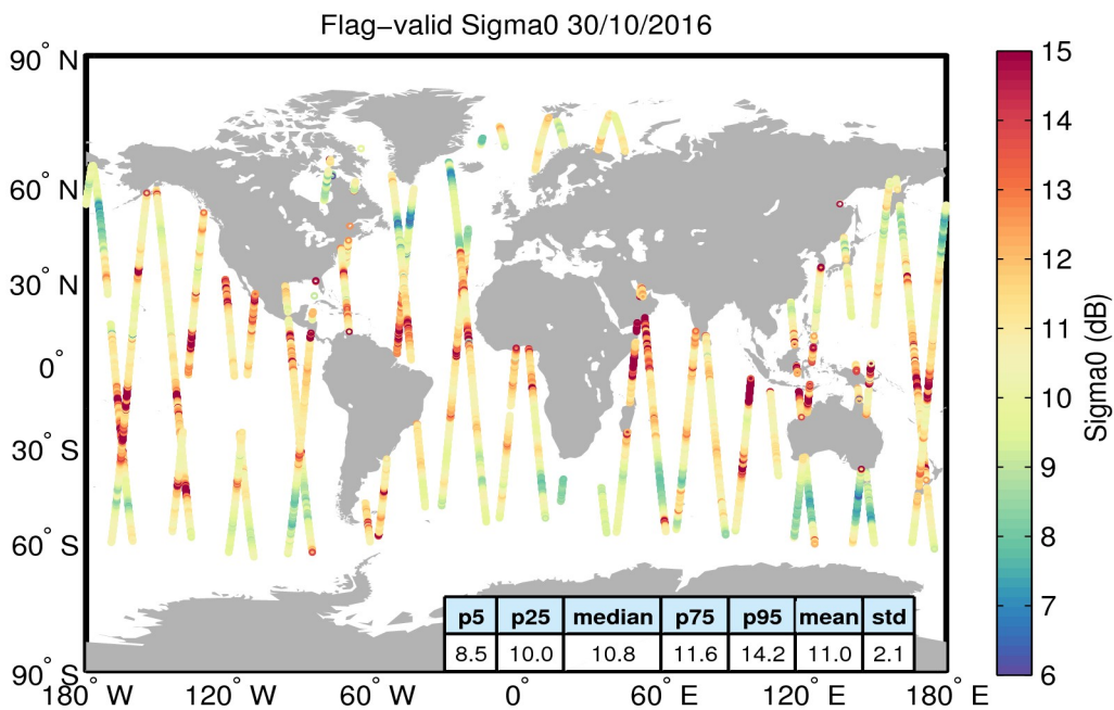
Figure 23. Geographical distribution of flag-valid sigma0 data over oceans and lakes for 30/10/2016. The statistical values shown in the table refer to the sigma0 in dB and are calculated over all measurements shown in the figure.
