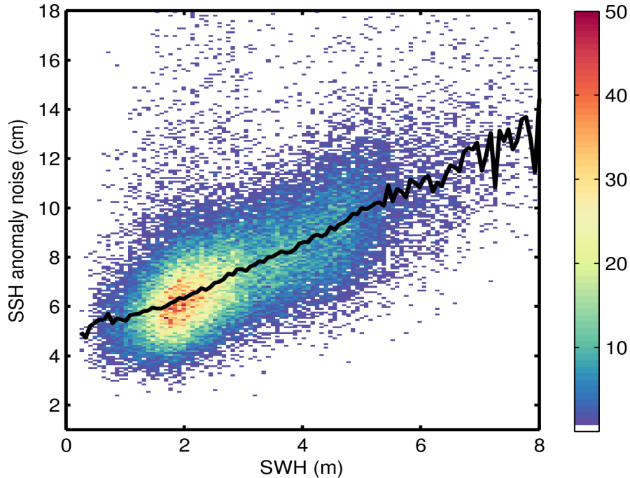
Figure 9. 2D histogram showing flag-valid SSH anomaly noise as a function of SWH for 29/10/2016. The black line denotes the median SSH anomaly noise as a function of SWH.
