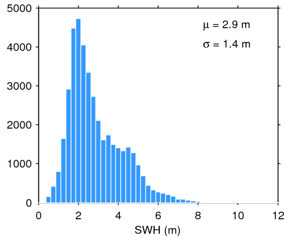
Figure 17. Histogram of flag-valid SWH over oceans and lakes for 29/10/2016. The mean ( \mu ) and standard deviation ( \sigma ) are also shown. Note that values larger than 12 m are excluded from the histogram for the sake of readability but not from the computation of \mu and \sigma .
