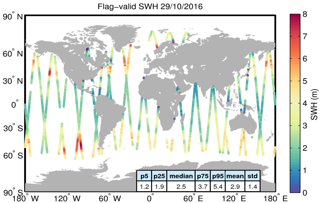
Figure 15. Geographical distribution of flag-valid SWH data over oceans and lakes for 29/10/2016. The statistical values shown in the table refer to the SWH in m and are calculated over all measurements shown in the figure.
