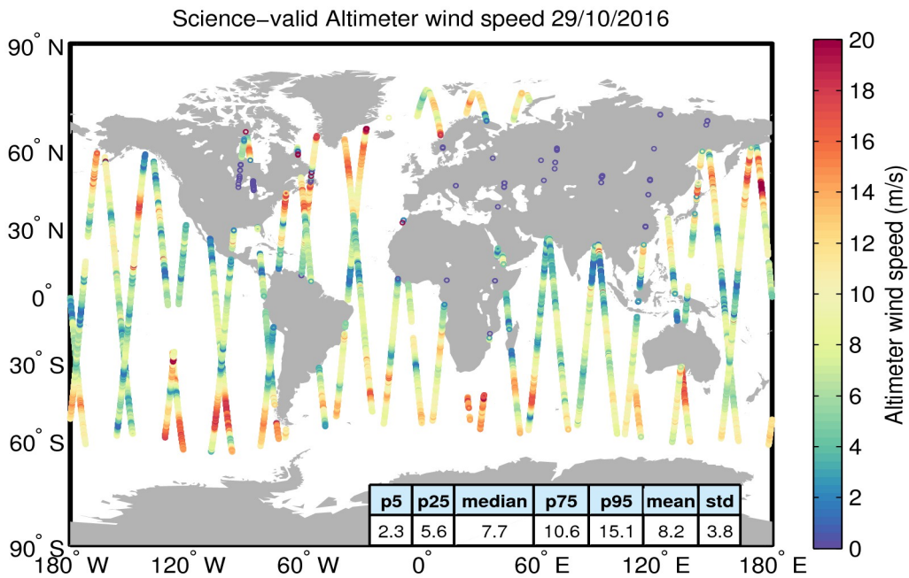
Figure 34. Geographical distribution of science-valid wind data over oceans and lakes for 29/10/2016. The statistical values shown in the table refer to the wind in m/s and are calculated over all measurements shown in the figure. Gray circles denote records that have been rejected based on the editing criteria described in Table 5.
