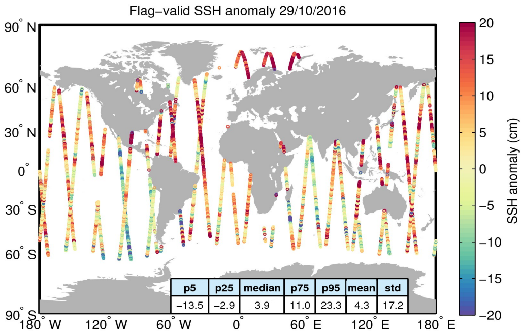
Figure 5. Geographical distribution of flag-valid 1-Hz SSH anomaly data over oceans and lakes for 29/10/2016. The statistical values shown in the table refer to the SSH anomaly in cm and are calculated over all measurements shown in the figure.
