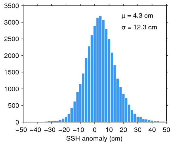
Figure 11. Histogram of science-valid SSH anomaly over oceans and lakes for 29/10/2016. The mean ( \mu ) and standard deviation ( \sigma ) are also shown. Note that values outside [-50 50] cm are excluded from the histogram for the sake of readability but not from the computation of \mu and \sigma .
