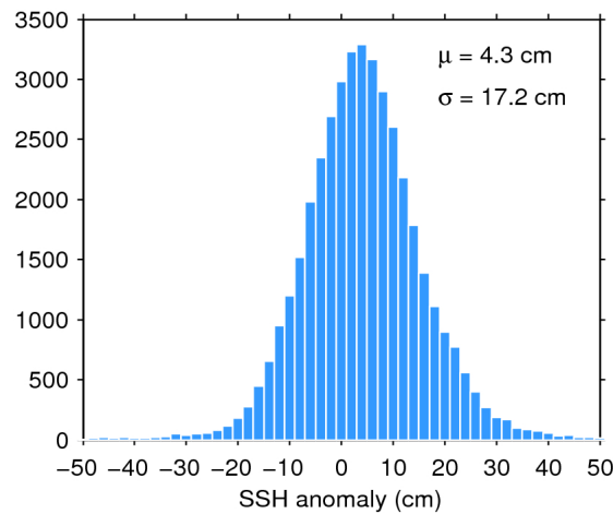
Figure 7. Histogram of flag-valid SSH anomaly over oceans and lakes for 29/10/2016. The mean ( \mu ) and standard deviation ( \sigma ) are also shown. Note that values outside [-50\ 50] cm are excluded from the histogram for the sake of readability but not from the computation of \mu and \sigma .
