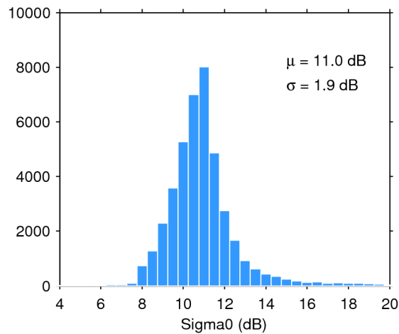
Figure 25. Histogram of flag-valid sigma0 over oceans and lakes for 29/10/2016. The mean ( \mu ) and standard deviation ( \sigma ) are also shown. Note that values outside [4 20] dB are excluded from the histogram for the sake of readability but not from the computation of \mu and \sigma .
