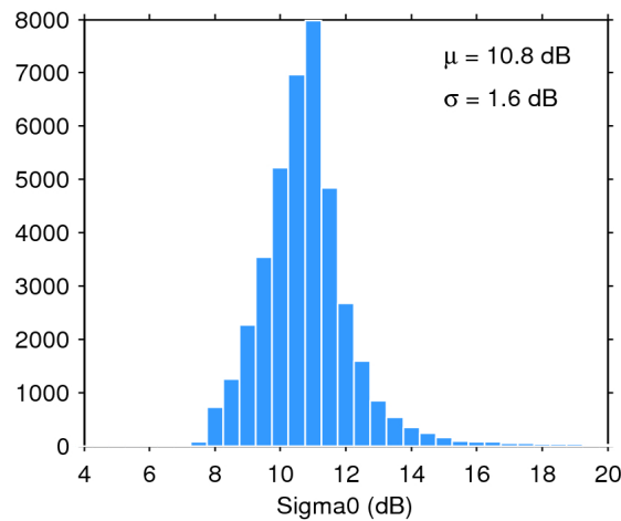
Figure 28. Histogram of science-valid sigma0 over oceans and lakes for 29/10/2016. The mean ( \mu ) and standard deviation ( \sigma ) are also shown. Note that values outside [4 20] dB are excluded from the histogram for the sake of readability but not from the computation of \mu and \sigma .
