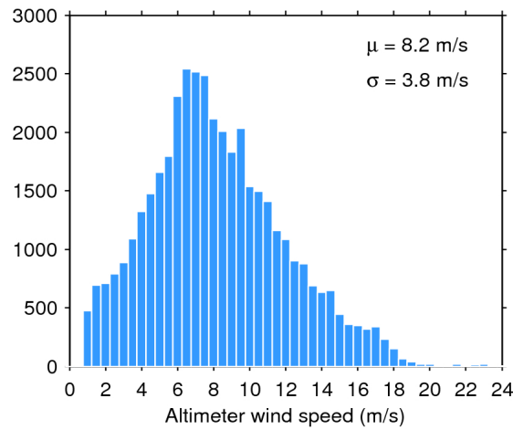
Figure 33. Histogram of flag-valid wind over oceans and lakes for 29/10/2016. The mean ( \mu ) and standard deviation ( \sigma ) are also shown. Note that values larger than 24 m/s are excluded from the histogram for the sake of readability but not from the computation of \mu and \sigma .
