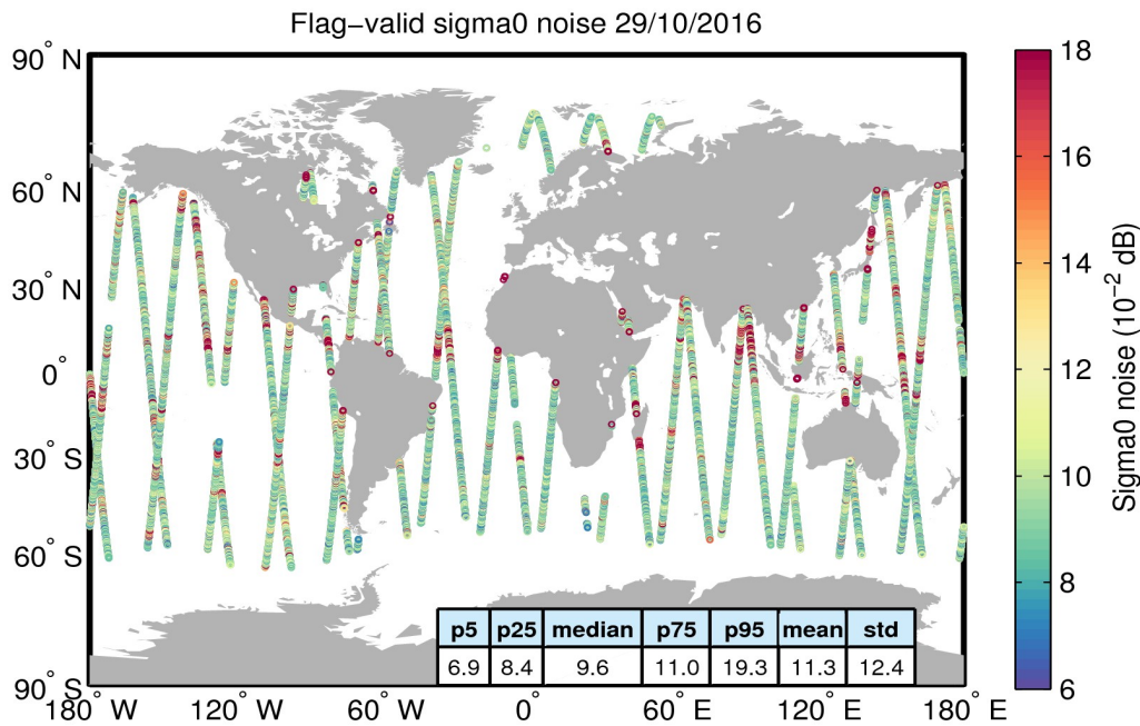
Figure 26. Geographical distribution of flag-valid 20-Hz sigma0 measurement noise over oceans and lakes for 29/10/2016. The statistical values shown in the table refer to the sigma0 noise and are calculated over all measurements shown in the figure.
