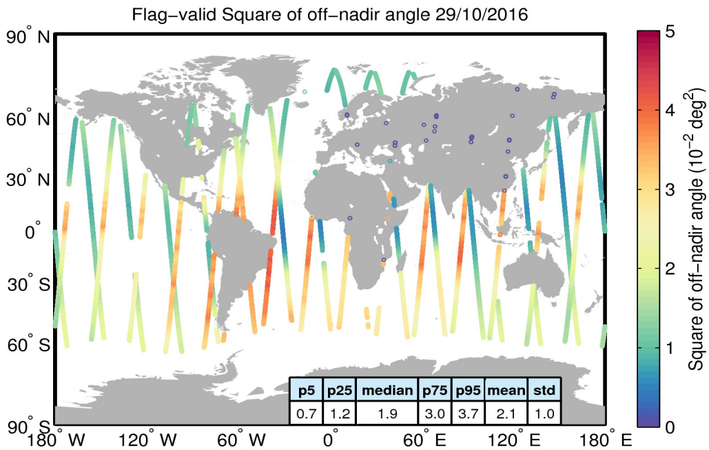
Figure 37. Geographical distribution of flag-valid mispointing data over oceans and lakes for 29/10/2016. The statistical values shown in the table refer to the mispointing in 10^{-2} deg 2 and are calculated over all measurements shown in the figure.
