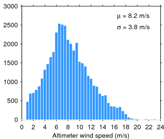
Figure 35. Histogram of science-valid wind over oceans and lakes for 29/10/2016. The mean ( \mu ) and standard deviation ( \sigma ) are also shown. Note that values larger than 24 m/s are excluded from the histogram for the sake of readability but not from the computation of \mu and \sigma .
