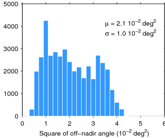
Figure 39. Histogram of flag-valid mispointing over oceans and lakes for 29/10/2016. The mean ( \mu ) and standard deviation ( \sigma ) are also shown. Note that values larger than 6 \cdot 10^{-2} \text{ deg}^2 are excluded from the histogram for the sake of readability but not from the computation of \mu and \sigma .
