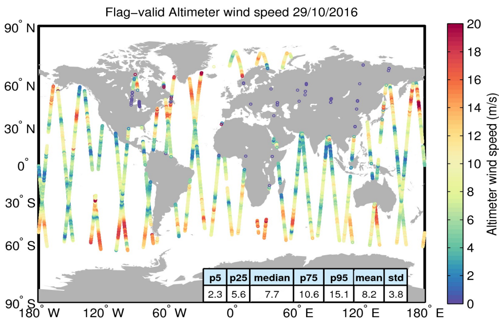
Figure 31. Geographical distribution of flag-valid wind data over oceans and lakes for 29/10/2016. The statistical values shown in the table refer to the wind in m/s and are calculated over all measurements shown in the figure.
