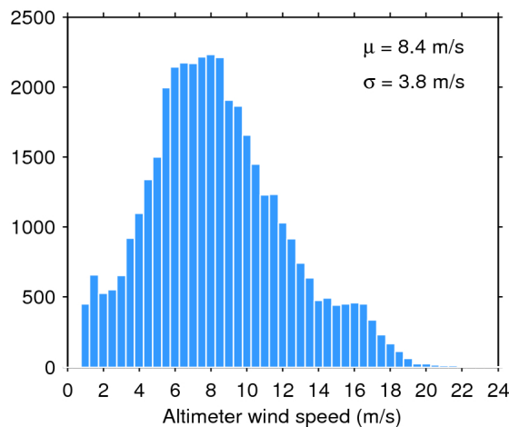
Figure 35. Histogram of science-valid wind over oceans and lakes for 28/10/2016. The mean ( \mu ) and standard deviation ( \sigma ) are also shown. Note that values larger than 24 m/s are excluded from the histogram for the sake of readability but not from the computation of \mu and \sigma .
