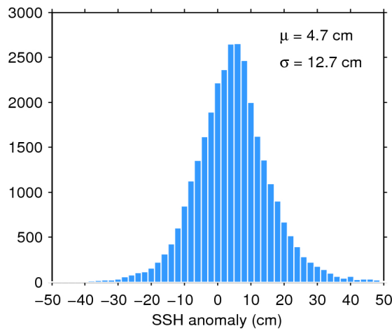
Figure 11. Histogram of science-valid SSH anomaly over oceans and lakes for 28/10/2016. The mean ( \mu ) and standard deviation ( \sigma ) are also shown. Note that values outside [-50 50] cm are excluded from the histogram for the sake of readability but not from the computation of \mu and \sigma .
