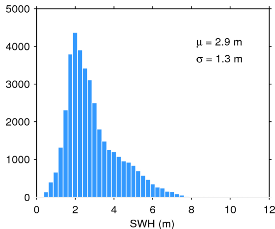
Figure 20. Histogram of science-valid SWH over oceans and lakes for 28/10/2016. The mean ( \mu ) and standard deviation ( \sigma ) are also shown. Note that values larger than 12 m are excluded from the histogram for the sake of readability but not from the computation of \mu and \sigma .
