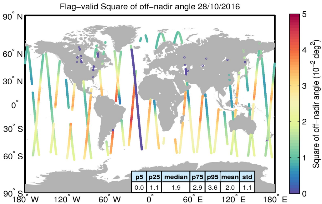
Figure 37. Geographical distribution of flag-valid mispointing data over oceans and lakes for 28/10/2016. The statistical values shown in the table refer to the mispointing in 10^{-2} deg 2 and are calculated over all measurements shown in the figure.
