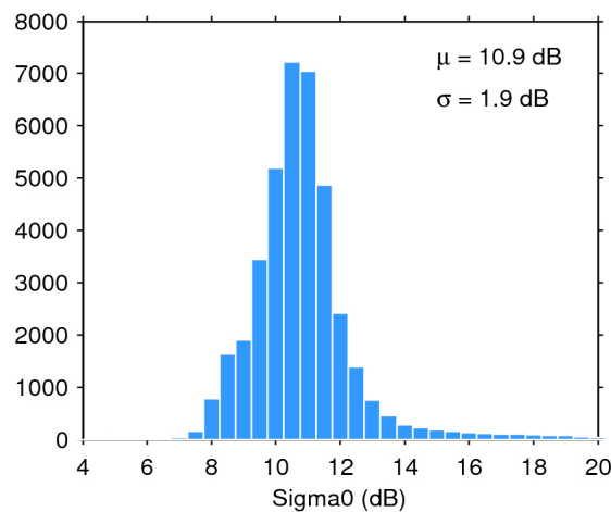
Figure 25. Histogram of flag-valid sigma0 over oceans and lakes for 28/10/2016. The mean ( \mu ) and standard deviation ( \sigma ) are also shown. Note that values outside [4 20] dB are excluded from the histogram for the sake of readability but not from the computation of \mu and \sigma .
