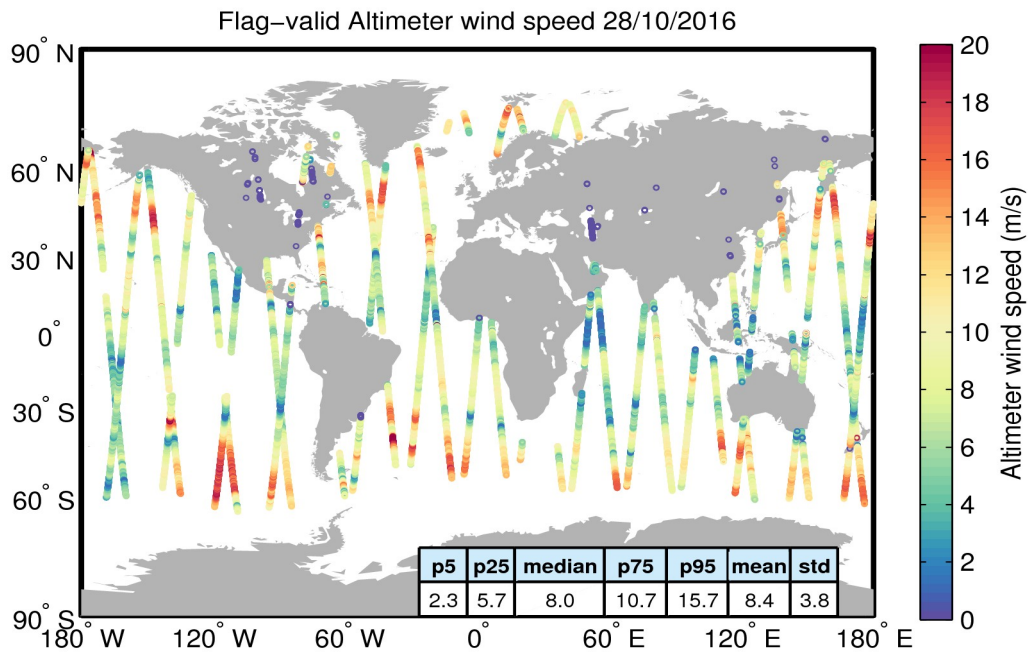
Figure 31. Geographical distribution of flag-valid wind data over oceans and lakes for 28/10/2016. The statistical values shown in the table refer to the wind in m/s and are calculated over all measurements shown in the figure.
