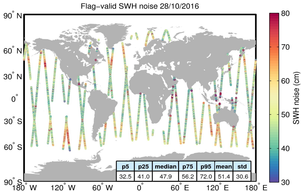
Figure 18. Geographical distribution of flag-valid 20-Hz SWH measurement noise over oceans and lakes for 28/10/2016. The statistical values shown in the table refer to the SWH noise and are calculated over all measurements shown in the figure.
