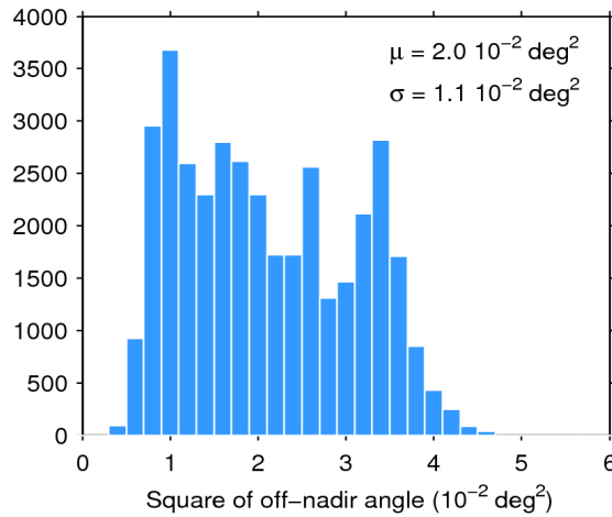
Figure 39. Histogram of flag-valid mispointing over oceans and lakes for 28/10/2016. The mean ( \mu ) and standard deviation ( \sigma ) are also shown. Note that values larger than 6 \cdot 10^{-2} \text{ deg}^2 are excluded from the histogram for the sake of readability but not from the computation of \mu and \sigma .
