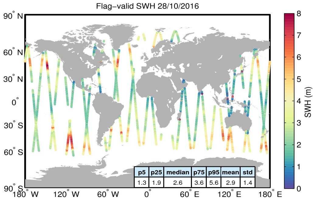
Figure 15. Geographical distribution of flag-valid SWH data over oceans and lakes for 28/10/2016. The statistical values shown in the table refer to the SWH in m and are calculated over all measurements shown in the figure.
