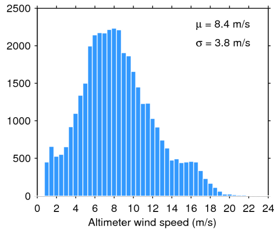
Figure 33. Histogram of flag-valid wind over oceans and lakes for 28/10/2016. The mean ( \mu ) and standard deviation ( \sigma ) are also shown. Note that values larger than 24 m/s are excluded from the histogram for the sake of readability but not from the computation of \mu and \sigma .
