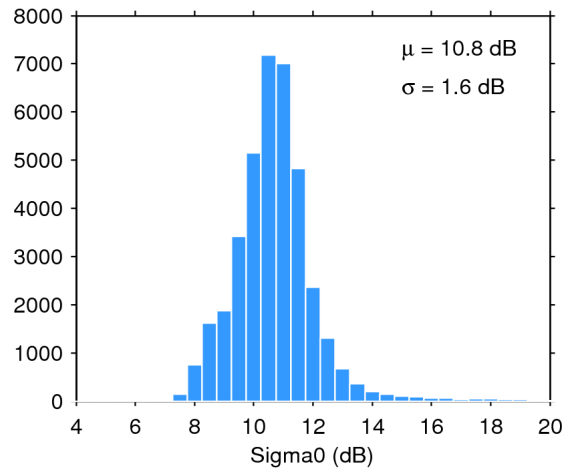
Figure 28. Histogram of science-valid sigma0 over oceans and lakes for 28/10/2016. The mean ( \mu ) and standard deviation ( \sigma ) are also shown. Note that values outside [4 20] dB are excluded from the histogram for the sake of readability but not from the computation of \mu and \sigma .
