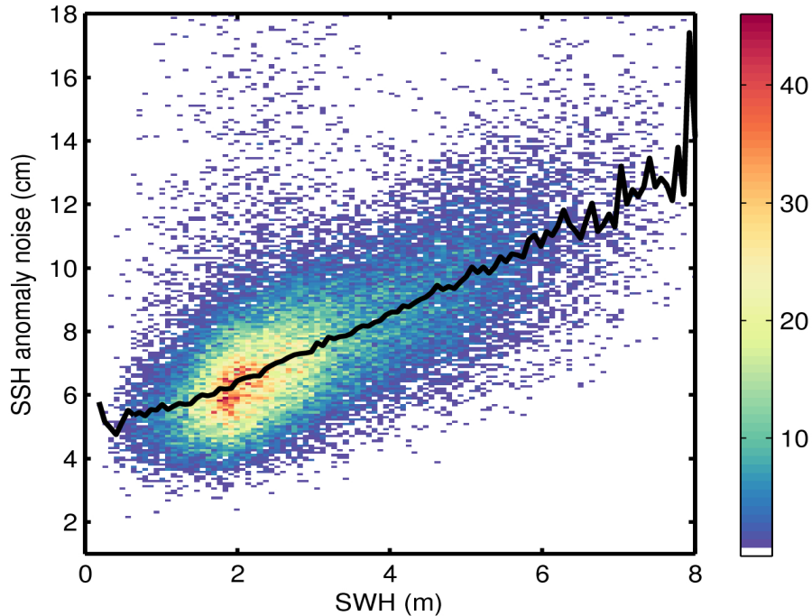
Figure 9. 2D histogram showing flag-valid SSH anomaly noise as a function of SWH for 28/10/2016. The black line denotes the median SSH anomaly noise as a function of SWH.
