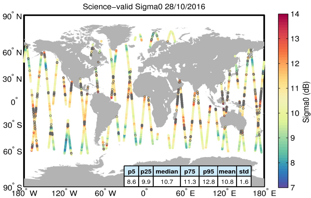
Figure 27. Geographical distribution of science-valid sigma0 data over oceans and lakes for 28/10/2016. The statistical values shown in the table refer to the sigma0 in dB and are calculated over all measurements shown in the figure. Gray circles denote records that have been rejected based on the editing criteria described in Table 4.
