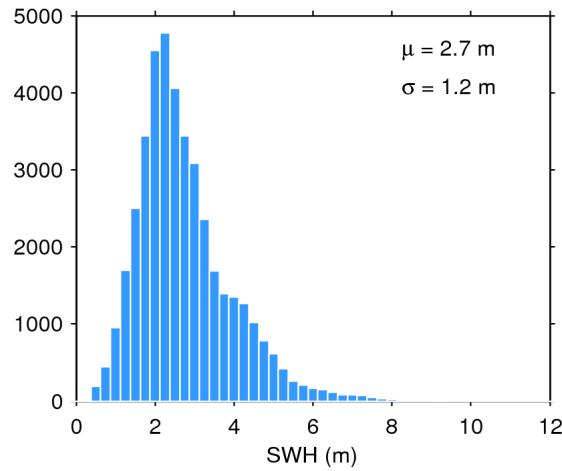
Figure 17. Histogram of flag-valid SWH over oceans and lakes for 27/10/2016. The mean ( \mu ) and standard deviation ( \sigma ) are also shown. Note that values larger than 12 m are excluded from the histogram for the sake of readability but not from the computation of \mu and \sigma .
