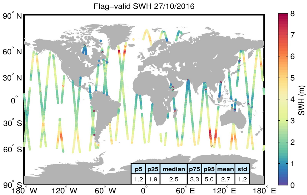
Figure 15. Geographical distribution of flag-valid SWH data over oceans and lakes for 27/10/2016. The statistical values shown in the table refer to the SWH in m and are calculated over all measurements shown in the figure.
