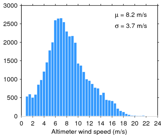
Figure 35. Histogram of science-valid wind over oceans and lakes for 27/10/2016. The mean ( \mu ) and standard deviation ( \sigma ) are also shown. Note that values larger than 24 m/s are excluded from the histogram for the sake of readability but not from the computation of \mu and \sigma .
