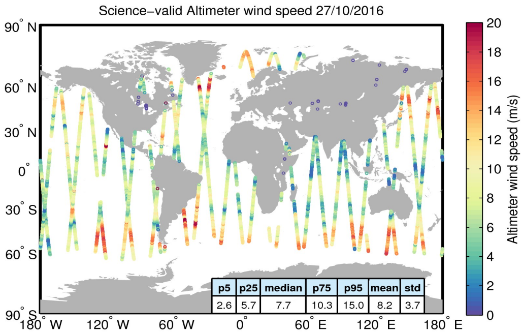
Figure 34. Geographical distribution of science-valid wind data over oceans and lakes for 27/10/2016. The statistical values shown in the table refer to the wind in m/s and are calculated over all measurements shown in the figure. Gray circles denote records that have been rejected based on the editing criteria described in Table 5.
