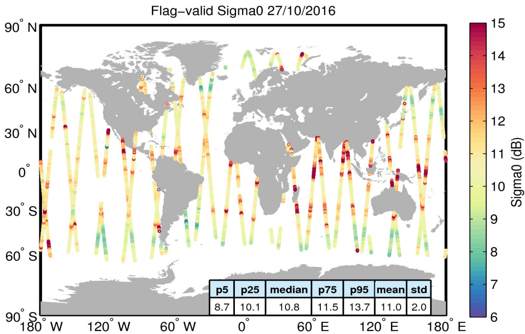
Figure 23. Geographical distribution of flag-valid sigma0 data over oceans and lakes for 27/10/2016. The statistical values shown in the table refer to the sigma0 in dB and are calculated over all measurements shown in the figure.
