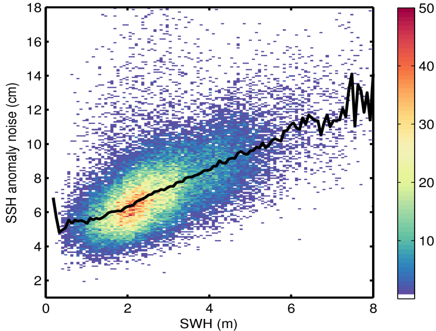
Figure 9. 2D histogram showing flag-valid SSH anomaly noise as a function of SWH for 27/10/2016. The black line denotes the median SSH anomaly noise as a function of SWH.
