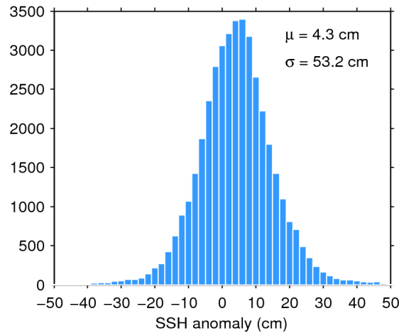
Figure 7. Histogram of flag-valid SSH anomaly over oceans and lakes for 27/10/2016. The mean ( \mu ) and standard deviation ( \sigma ) are also shown. Note that values outside [-50\ 50] cm are excluded from the histogram for the sake of readability but not from the computation of \mu and \sigma .
