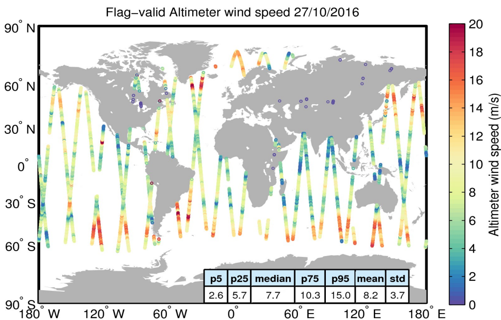
Figure 31. Geographical distribution of flag-valid wind data over oceans and lakes for 27/10/2016. The statistical values shown in the table refer to the wind in m/s and are calculated over all measurements shown in the figure.
