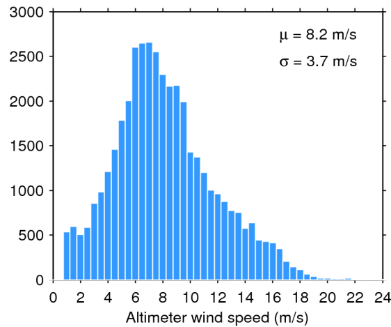
Figure 33. Histogram of flag-valid wind over oceans and lakes for 27/10/2016. The mean ( \mu ) and standard deviation ( \sigma ) are also shown. Note that values larger than 24 m/s are excluded from the histogram for the sake of readability but not from the computation of \mu and \sigma .
