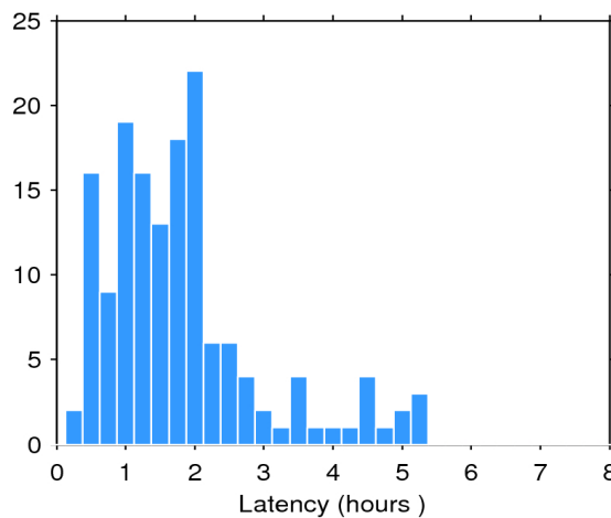
Figure 2. Histogram of the data latency for 27/10/2016. The y-axis denotes the number of files that are made available with a delay of x-hours with respect to the mean time of the records stored in the file.
