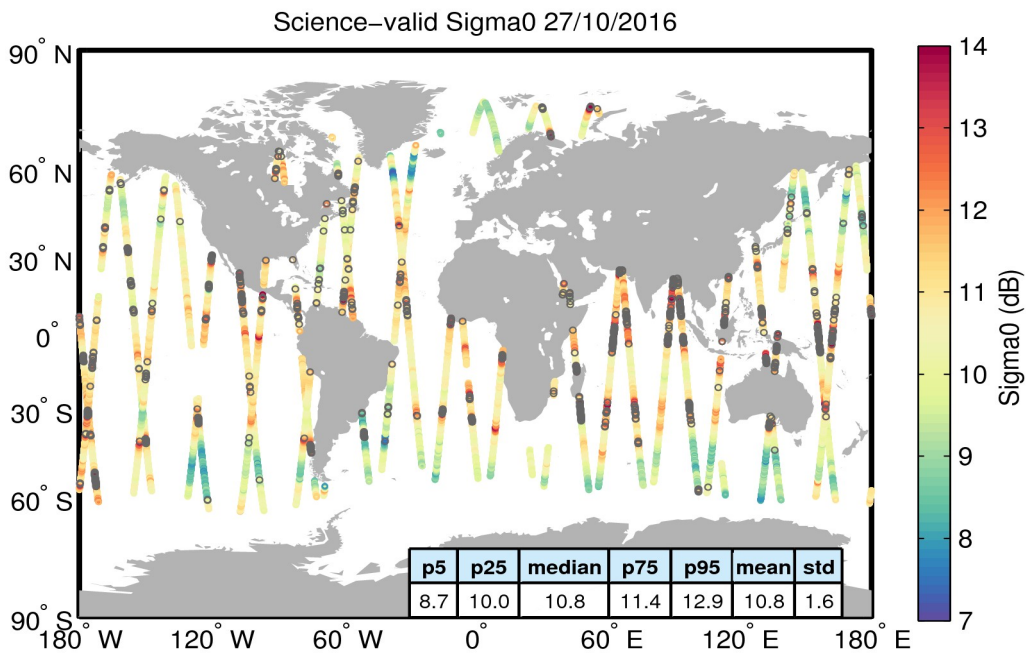
Figure 27. Geographical distribution of science-valid sigma0 data over oceans and lakes for 27/10/2016. The statistical values shown in the table refer to the sigma0 in dB and are calculated over all measurements shown in the figure. Gray circles denote records that have been rejected based on the editing criteria described in Table 4.
