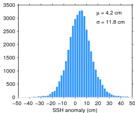
Figure 11. Histogram of science-valid SSH anomaly over oceans and lakes for 27/10/2016. The mean ( \mu ) and standard deviation ( \sigma ) are also shown. Note that values outside [-50 50] cm are excluded from the histogram for the sake of readability but not from the computation of \mu and \sigma .
