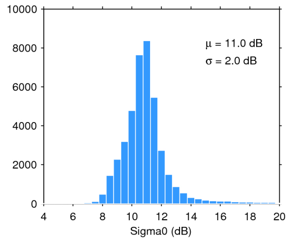
Figure 25. Histogram of flag-valid sigma0 over oceans and lakes for 27/10/2016. The mean ( \mu ) and standard deviation ( \sigma ) are also shown. Note that values outside [4 20] dB are excluded from the histogram for the sake of readability but not from the computation of \mu and \sigma .
