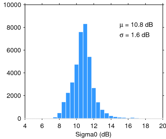
Figure 28. Histogram of science-valid sigma0 over oceans and lakes for 27/10/2016. The mean ( \mu ) and standard deviation ( \sigma ) are also shown. Note that values outside [4 20] dB are excluded from the histogram for the sake of readability but not from the computation of \mu and \sigma .
