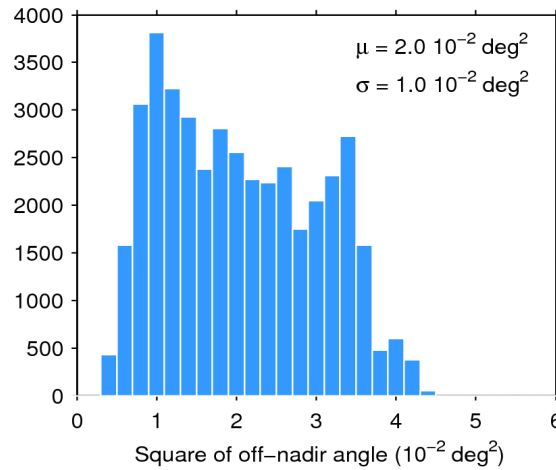
Figure 39. Histogram of flag-valid mispointing over oceans and lakes for 27/10/2016. The mean ( \mu ) and standard deviation ( \sigma ) are also shown. Note that values larger than 6 \cdot 10^{-2} \text{ deg}^2 are excluded from the histogram for the sake of readability but not from the computation of \mu and \sigma .
