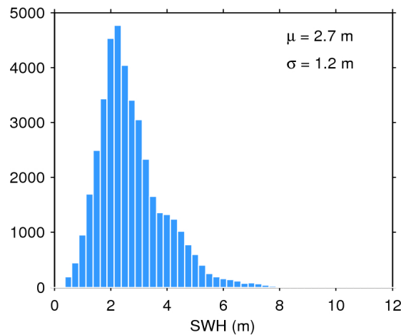
Figure 20. Histogram of science-valid SWH over oceans and lakes for 27/10/2016. The mean ( \mu ) and standard deviation ( \sigma ) are also shown. Note that values larger than 12 m are excluded from the histogram for the sake of readability but not from the computation of \mu and \sigma .
