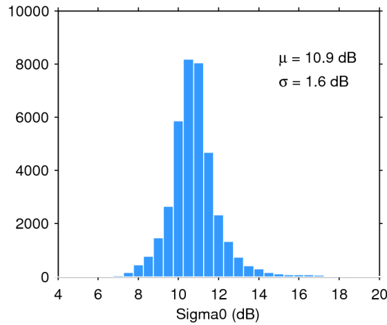
Figure 28. Histogram of science-valid sigma0 over oceans and lakes for 26/10/2016. The mean ( \mu ) and standard deviation ( \sigma ) are also shown. Note that values outside [4 20] dB are excluded from the histogram for the sake of readability but not from the computation of \mu and \sigma .
