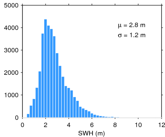
Figure 17. Histogram of flag-valid SWH over oceans and lakes for 26/10/2016. The mean ( \mu ) and standard deviation ( \sigma ) are also shown. Note that values larger than 12 m are excluded from the histogram for the sake of readability but not from the computation of \mu and \sigma .
