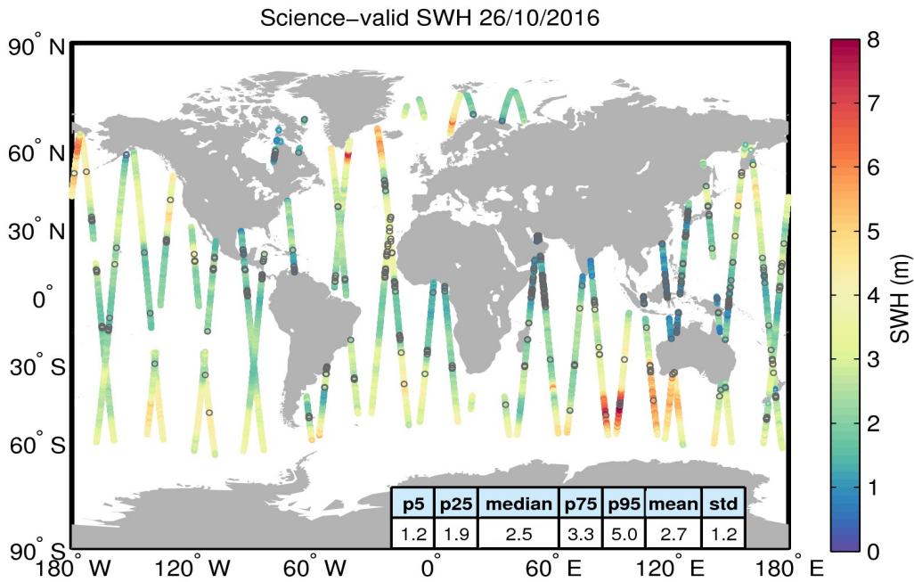
Figure 19. Geographical distribution of science-valid SWH data over oceans and lakes for 26/10/2016. The statistical values shown in the table refer to the SWH in m and are calculated over all measurements shown in the figure. Gray circles denote records that have been rejected based on the editing criteria described in Table 3.
