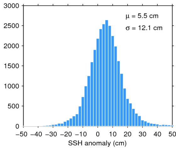
Figure 11. Histogram of science-valid SSH anomaly over oceans and lakes for 26/10/2016. The mean ( \mu ) and standard deviation ( \sigma ) are also shown. Note that values outside [-50 50] cm are excluded from the histogram for the sake of readability but not from the computation of \mu and \sigma .
