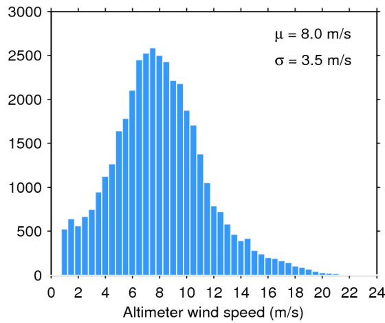
Figure 33. Histogram of flag-valid wind over oceans and lakes for 26/10/2016. The mean ( \mu ) and standard deviation ( \sigma ) are also shown. Note that values larger than 24 m/s are excluded from the histogram for the sake of readability but not from the computation of \mu and \sigma .
