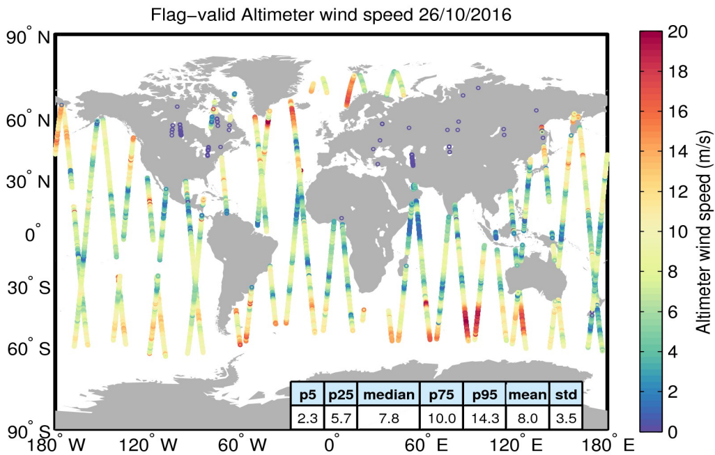
Figure 31. Geographical distribution of flag-valid wind data over oceans and lakes for 26/10/2016. The statistical values shown in the table refer to the wind in m/s and are calculated over all measurements shown in the figure.
