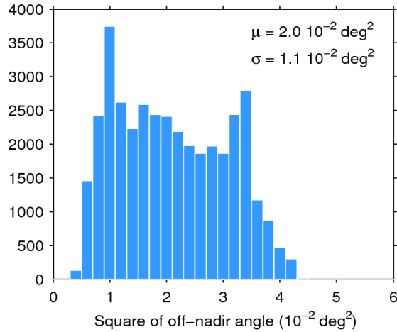
Figure 39. Histogram of flag-valid mispointing over oceans and lakes for 26/10/2016. The mean ( \mu ) and standard deviation ( \sigma ) are also shown. Note that values larger than 6 \cdot 10^{-2} \text{ deg}^2 are excluded from the histogram for the sake of readability but not from the computation of \mu and \sigma .
