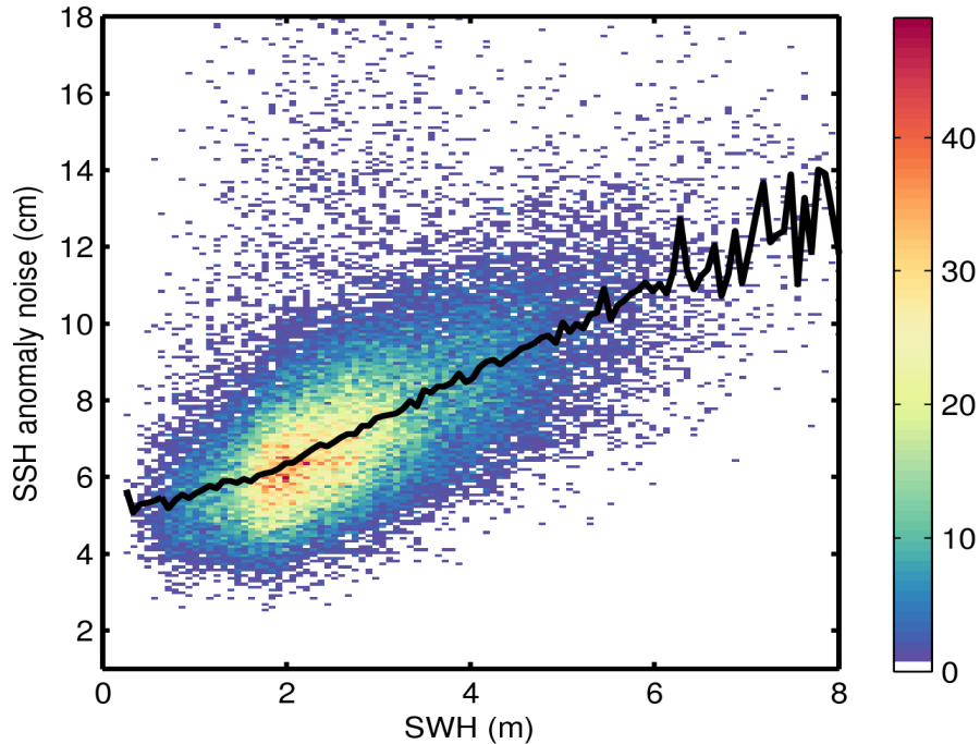
Figure 9. 2D histogram showing flag-valid SSH anomaly noise as a function of SWH for 26/10/2016. The black line denotes the median SSH anomaly noise as a function of SWH.
