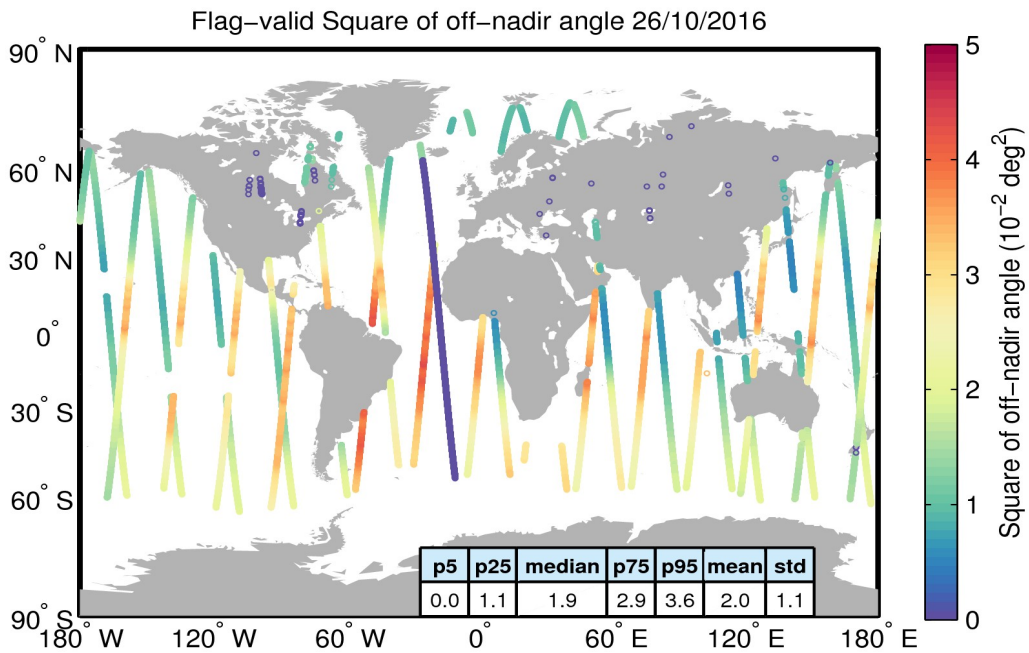
Figure 37. Geographical distribution of flag-valid mispointing data over oceans and lakes for 26/10/2016. The statistical values shown in the table refer to the mispointing in 10^{-2} deg 2 and are calculated over all measurements shown in the figure.
