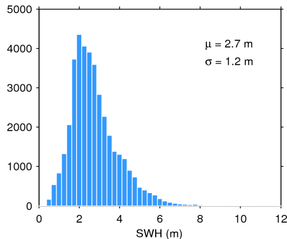
Figure 20. Histogram of science-valid SWH over oceans and lakes for 26/10/2016. The mean ( \mu ) and standard deviation ( \sigma ) are also shown. Note that values larger than 12 m are excluded from the histogram for the sake of readability but not from the computation of \mu and \sigma .
