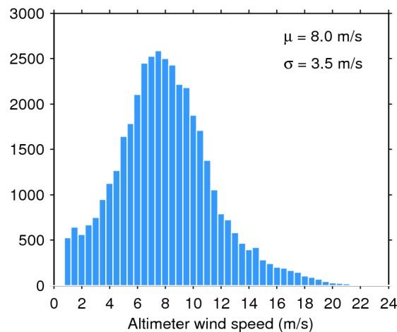
Figure 35. Histogram of science-valid wind over oceans and lakes for 26/10/2016. The mean ( \mu ) and standard deviation ( \sigma ) are also shown. Note that values larger than 24 m/s are excluded from the histogram for the sake of readability but not from the computation of \mu and \sigma .
