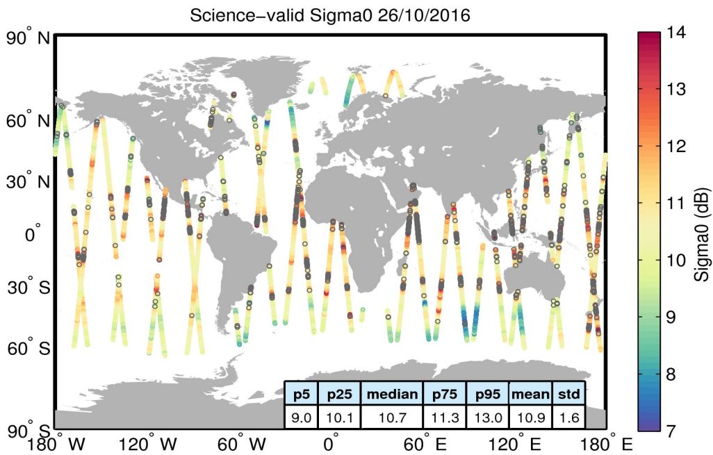
Figure 27. Geographical distribution of science-valid sigma0 data over oceans and lakes for 26/10/2016. The statistical values shown in the table refer to the sigma0 in dB and are calculated over all measurements shown in the figure. Gray circles denote records that have been rejected based on the editing criteria described in Table 4.
