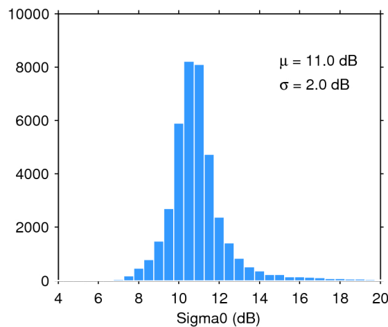
Figure 25. Histogram of flag-valid sigma0 over oceans and lakes for 26/10/2016. The mean ( \mu ) and standard deviation ( \sigma ) are also shown. Note that values outside [4 20] dB are excluded from the histogram for the sake of readability but not from the computation of \mu and \sigma .
