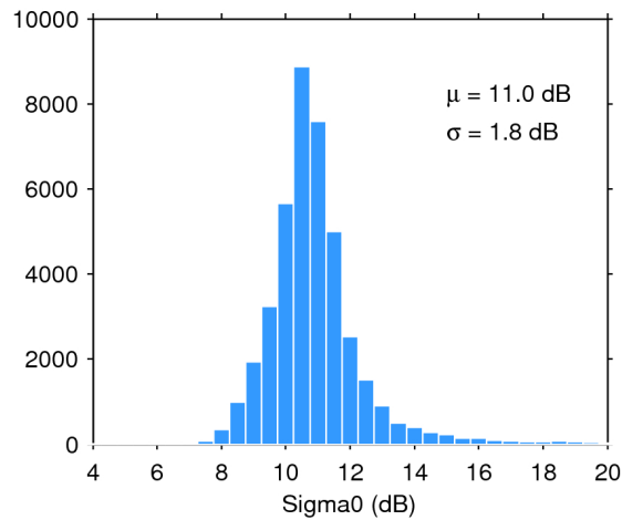
Figure 25. Histogram of flag-valid sigma0 over oceans and lakes for 25/10/2016. The mean ( \mu ) and standard deviation ( \sigma ) are also shown. Note that values outside [4 20] dB are excluded from the histogram for the sake of readability but not from the computation of \mu and \sigma .
