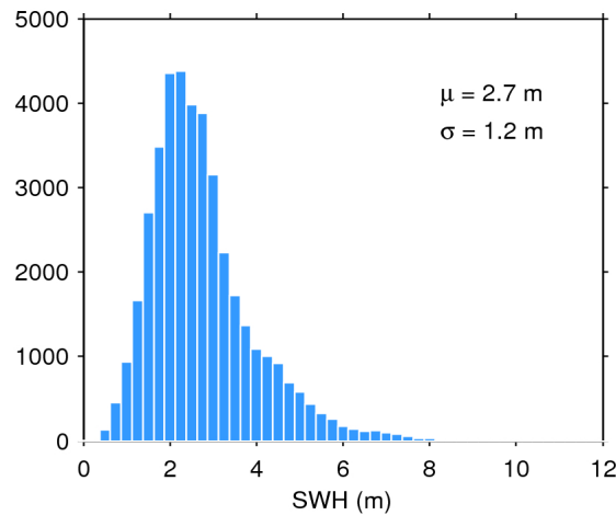
Figure 20. Histogram of science-valid SWH over oceans and lakes for 25/10/2016. The mean ( \mu ) and standard deviation ( \sigma ) are also shown. Note that values larger than 12 m are excluded from the histogram for the sake of readability but not from the computation of \mu and \sigma .
