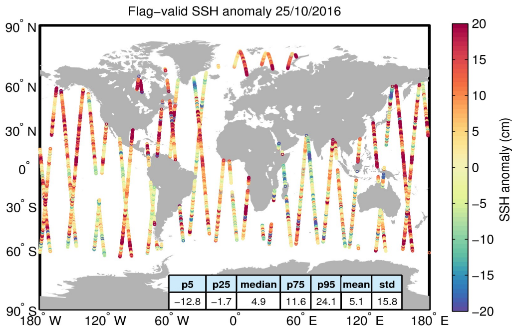
Figure 5. Geographical distribution of flag-valid 1-Hz SSH anomaly data over oceans and lakes for 25/10/2016. The statistical values shown in the table refer to the SSH anomaly in cm and are calculated over all measurements shown in the figure.
