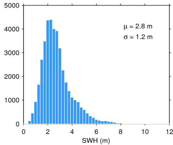
Figure 17. Histogram of flag-valid SWH over oceans and lakes for 25/10/2016. The mean ( \mu ) and standard deviation ( \sigma ) are also shown. Note that values larger than 12 m are excluded from the histogram for the sake of readability but not from the computation of \mu and \sigma .
