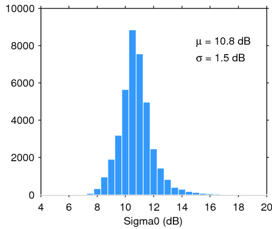
Figure 28. Histogram of science-valid sigma0 over oceans and lakes for 25/10/2016. The mean ( \mu ) and standard deviation ( \sigma ) are also shown. Note that values outside [4 20] dB are excluded from the histogram for the sake of readability but not from the computation of \mu and \sigma .
