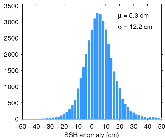
Figure 11. Histogram of science-valid SSH anomaly over oceans and lakes for 25/10/2016. The mean ( \mu ) and standard deviation ( \sigma ) are also shown. Note that values outside [-50 50] cm are excluded from the histogram for the sake of readability but not from the computation of \mu and \sigma .
