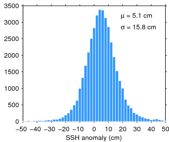
Figure 7. Histogram of flag-valid SSH anomaly over oceans and lakes for 25/10/2016. The mean ( \mu ) and standard deviation ( \sigma ) are also shown. Note that values outside [-50\ 50] cm are excluded from the histogram for the sake of readability but not from the computation of \mu and \sigma .
