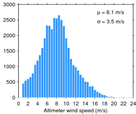
Figure 33. Histogram of flag-valid wind over oceans and lakes for 25/10/2016. The mean ( \mu ) and standard deviation ( \sigma ) are also shown. Note that values larger than 24 m/s are excluded from the histogram for the sake of readability but not from the computation of \mu and \sigma .
