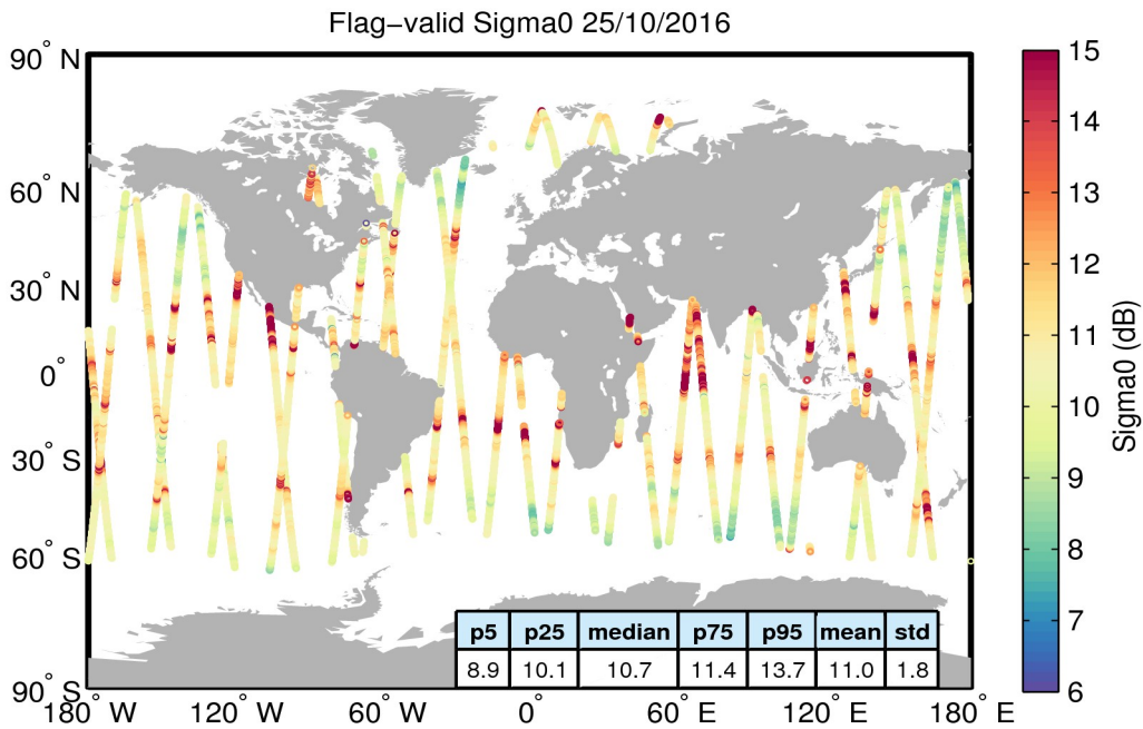
Figure 23. Geographical distribution of flag-valid sigma0 data over oceans and lakes for 25/10/2016. The statistical values shown in the table refer to the sigma0 in dB and are calculated over all measurements shown in the figure.
