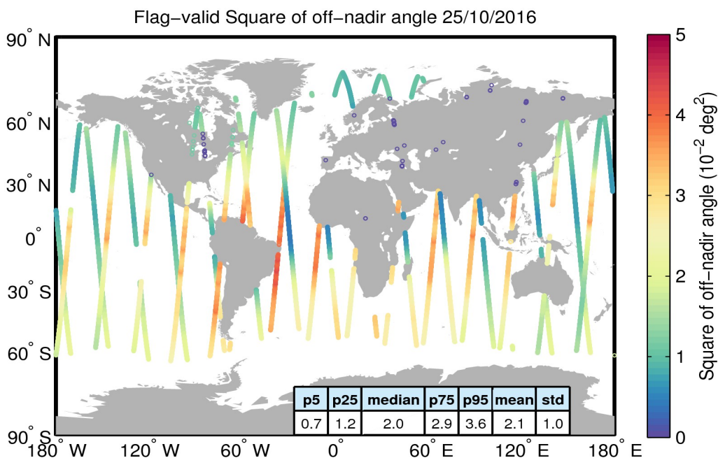
Figure 37. Geographical distribution of flag-valid mispointing data over oceans and lakes for 25/10/2016. The statistical values shown in the table refer to the mispointing in 10^{-2} deg 2 and are calculated over all measurements shown in the figure.
