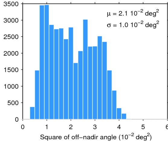
Figure 39. Histogram of flag-valid mispointing over oceans and lakes for 25/10/2016. The mean ( \mu ) and standard deviation ( \sigma ) are also shown. Note that values larger than 6 \cdot 10^{-2} \text{ deg}^2 are excluded from the histogram for the sake of readability but not from the computation of \mu and \sigma .
