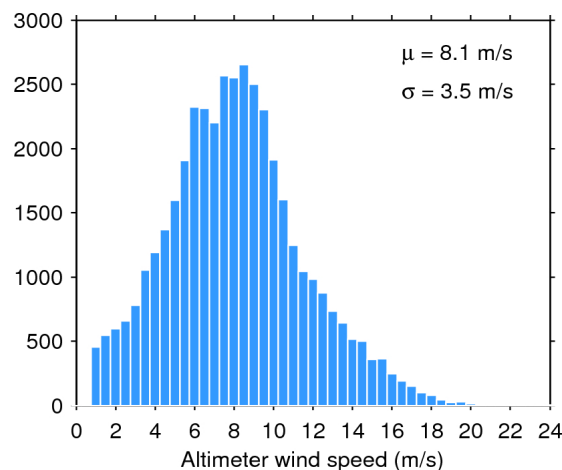
Figure 35. Histogram of science-valid wind over oceans and lakes for 25/10/2016. The mean ( \mu ) and standard deviation ( \sigma ) are also shown. Note that values larger than 24 m/s are excluded from the histogram for the sake of readability but not from the computation of \mu and \sigma .
