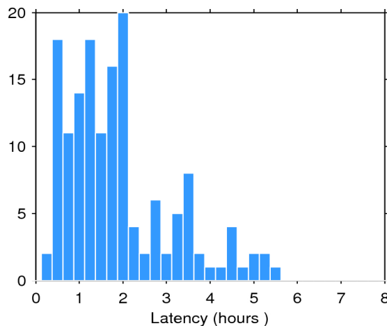
Figure 2. Histogram of the data latency for 25/10/2016. The y-axis denotes the number of files that are made available with a delay of x-hours with respect to the mean time of the records stored in the file.
