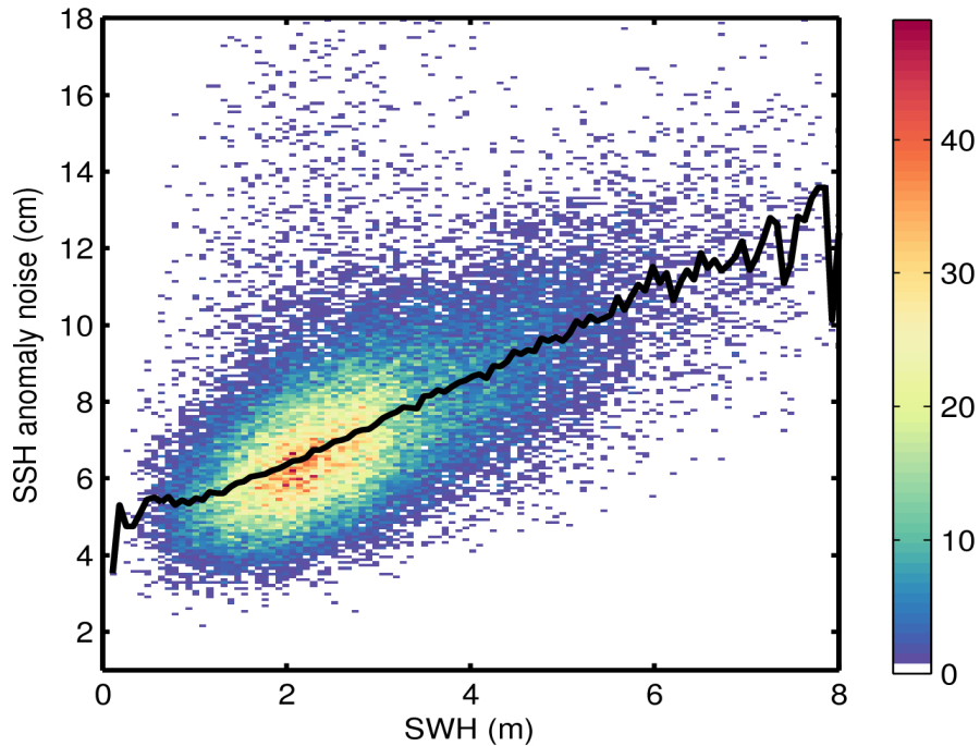
Figure 9. 2D histogram showing flag-valid SSH anomaly noise as a function of SWH for 25/10/2016. The black line denotes the median SSH anomaly noise as a function of SWH.
