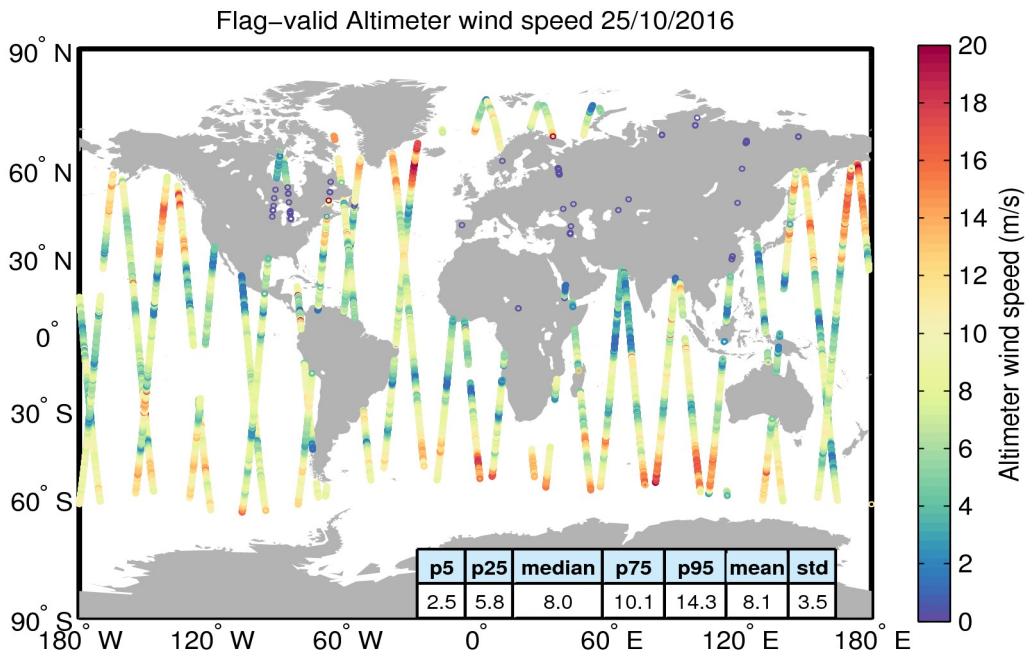
Figure 31. Geographical distribution of flag-valid wind data over oceans and lakes for 25/10/2016. The statistical values shown in the table refer to the wind in m/s and are calculated over all measurements shown in the figure.
