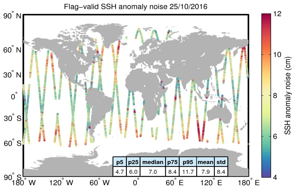
Figure 8. Geographical distribution of flag-valid 20-Hz SSH anomaly measurement noise over oceans and lakes for 25/10/2016. The statistical values shown in the table refer to the SSH anomaly noise and are calculated over all measurements shown in the figure.
