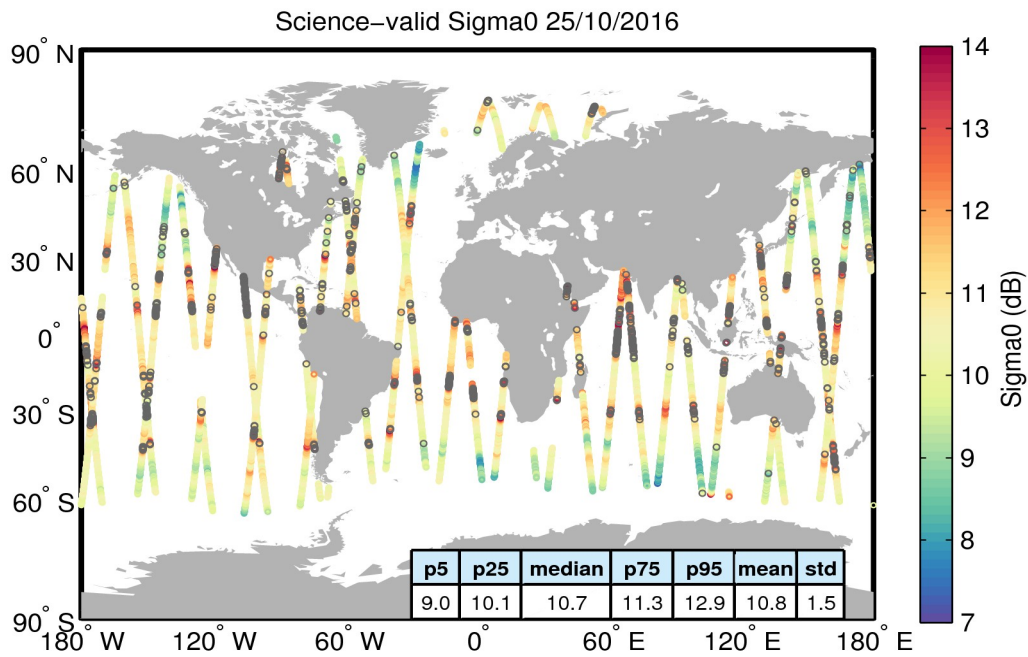
Figure 27. Geographical distribution of science-valid sigma0 data over oceans and lakes for 25/10/2016. The statistical values shown in the table refer to the sigma0 in dB and are calculated over all measurements shown in the figure. Gray circles denote records that have been rejected based on the editing criteria described in Table 4.
