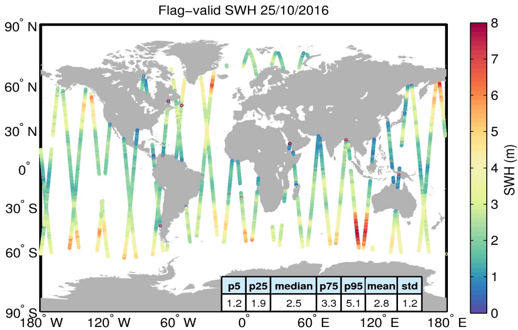
Figure 15. Geographical distribution of flag-valid SWH data over oceans and lakes for 25/10/2016. The statistical values shown in the table refer to the SWH in m and are calculated over all measurements shown in the figure.
