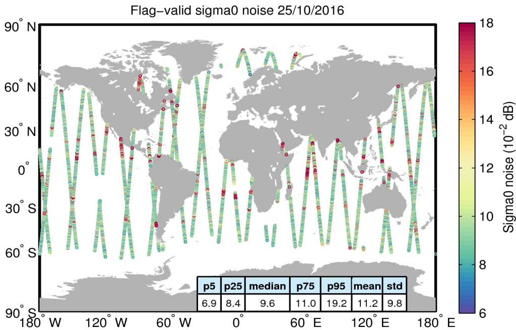
Figure 26. Geographical distribution of flag-valid 20-Hz sigma0 measurement noise over oceans and lakes for 25/10/2016. The statistical values shown in the table refer to the sigma0 noise and are calculated over all measurements shown in the figure.
