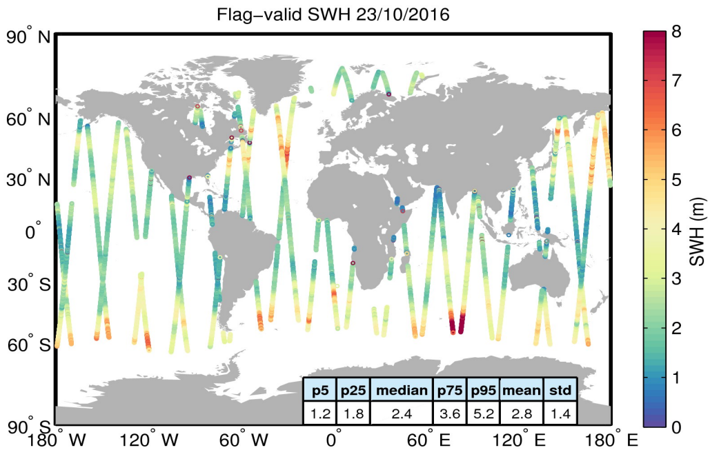
Figure 15. Geographical distribution of flag-valid SWH data over oceans and lakes for 23/10/2016. The statistical values shown in the table refer to the SWH in m and are calculated over all measurements shown in the figure.
