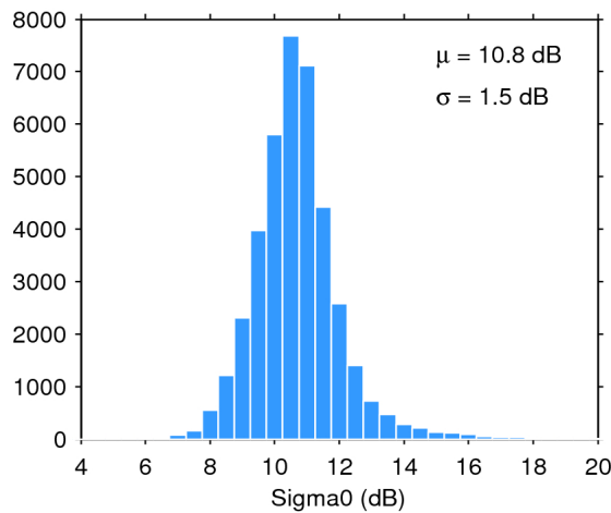
Figure 28. Histogram of science-valid sigma0 over oceans and lakes for 23/10/2016. The mean ( \mu ) and standard deviation ( \sigma ) are also shown. Note that values outside [4 20] dB are excluded from the histogram for the sake of readability but not from the computation of \mu and \sigma .
