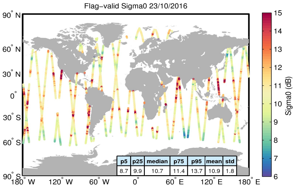
Figure 23. Geographical distribution of flag-valid sigma0 data over oceans and lakes for 23/10/2016. The statistical values shown in the table refer to the sigma0 in dB and are calculated over all measurements shown in the figure.
