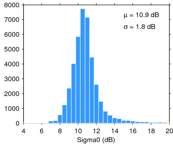
Figure 25. Histogram of flag-valid sigma0 over oceans and lakes for 23/10/2016. The mean ( \mu ) and standard deviation ( \sigma ) are also shown. Note that values outside [4 20] dB are excluded from the histogram for the sake of readability but not from the computation of \mu and \sigma .
