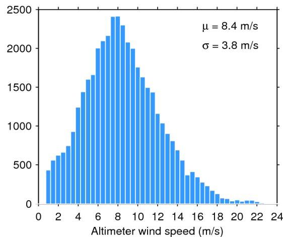
Figure 35. Histogram of science-valid wind over oceans and lakes for 23/10/2016. The mean ( \mu ) and standard deviation ( \sigma ) are also shown. Note that values larger than 24 m/s are excluded from the histogram for the sake of readability but not from the computation of \mu and \sigma .
