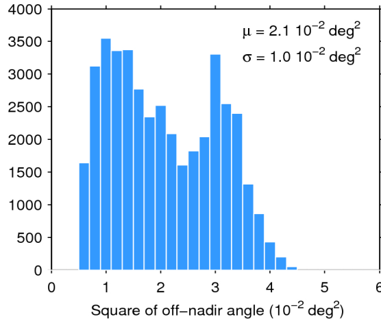
Figure 39. Histogram of flag-valid mispointing over oceans and lakes for 23/10/2016. The mean ( \mu ) and standard deviation ( \sigma ) are also shown. Note that values larger than 6 \cdot 10^{-2} \text{ deg}^2 are excluded from the histogram for the sake of readability but not from the computation of \mu and \sigma .
