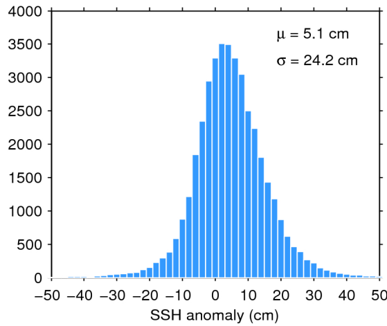
Figure 7. Histogram of flag-valid SSH anomaly over oceans and lakes for 23/10/2016. The mean ( \mu ) and standard deviation ( \sigma ) are also shown. Note that values outside [-50 50] cm are excluded from the histogram for the sake of readability but not from the computation of \mu and \sigma .
