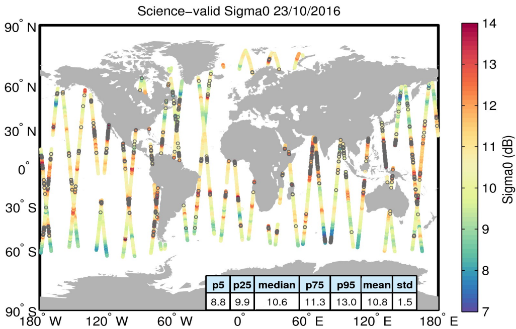
Figure 27. Geographical distribution of science-valid sigma0 data over oceans and lakes for 23/10/2016. The statistical values shown in the table refer to the sigma0 in dB and are calculated over all measurements shown in the figure. Gray circles denote records that have been rejected based on the editing criteria described in Table 4.
