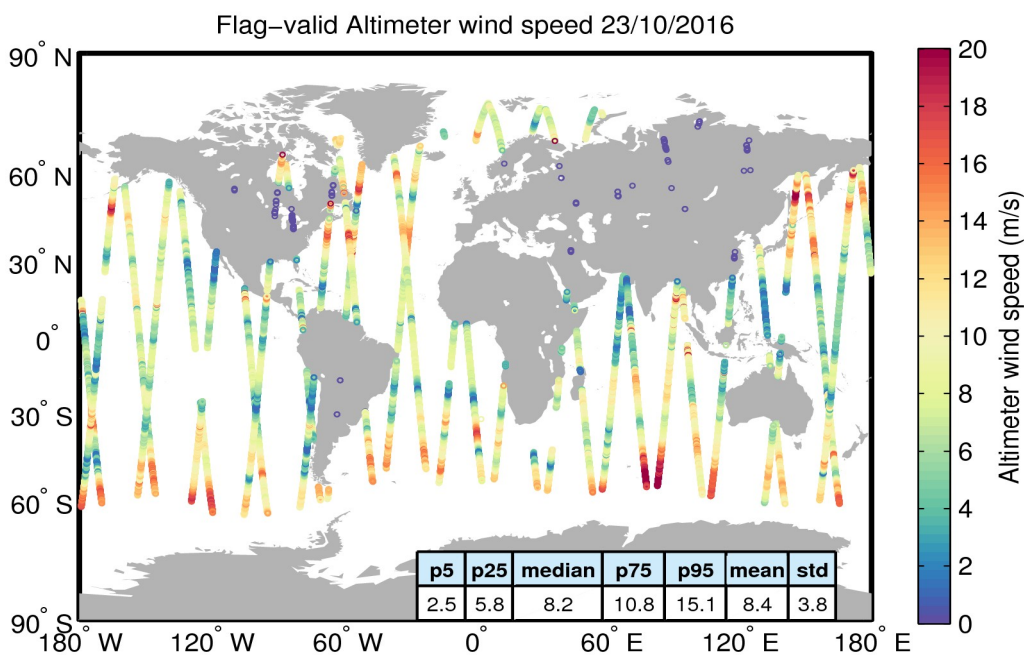
Figure 31. Geographical distribution of flag-valid wind data over oceans and lakes for 23/10/2016. The statistical values shown in the table refer to the wind in m/s and are calculated over all measurements shown in the figure.
