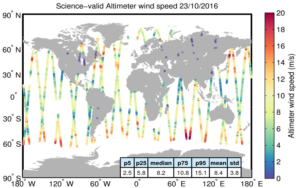
Figure 34. Geographical distribution of science-valid wind data over oceans and lakes for 23/10/2016. The statistical values shown in the table refer to the wind in m/s and are calculated over all measurements shown in the figure. Gray circles denote records that have been rejected based on the editing criteria described in Table 5.
