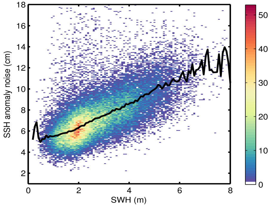
Figure 9. 2D histogram showing flag-valid SSH anomaly noise as a function of SWH for 23/10/2016. The black line denotes the median SSH anomaly noise as a function of SWH.
