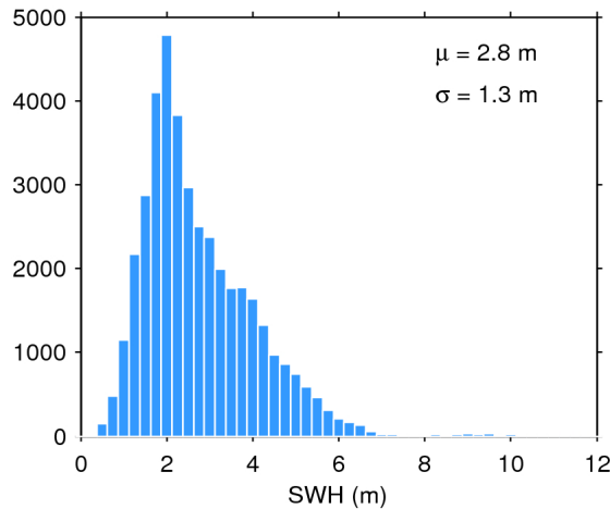
Figure 20. Histogram of science-valid SWH over oceans and lakes for 23/10/2016. The mean ( \mu ) and standard deviation ( \sigma ) are also shown. Note that values larger than 12 m are excluded from the histogram for the sake of readability but not from the computation of \mu and \sigma .
