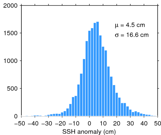
Figure 11. Histogram of science-valid SSH anomaly over oceans and lakes for 22/10/2016. The mean ( \mu ) and standard deviation ( \sigma ) are also shown. Note that values outside [-50 50] cm are excluded from the histogram for the sake of readability but not from the computation of \mu and \sigma .
