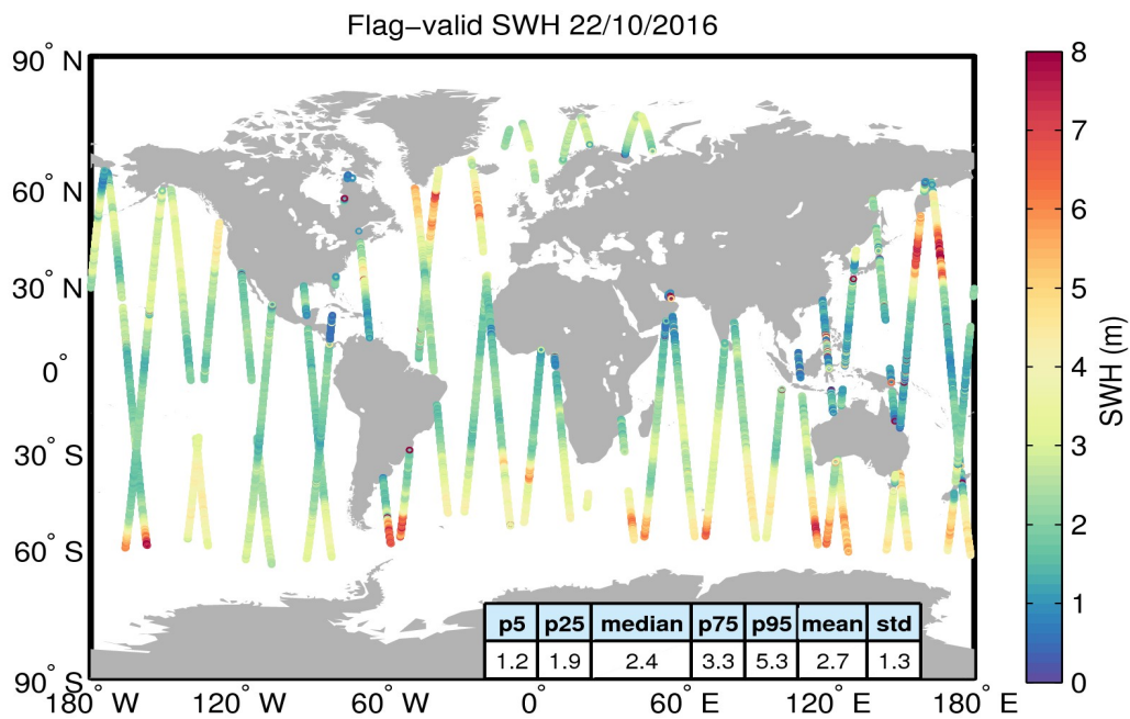
Figure 15. Geographical distribution of flag-valid SWH data over oceans and lakes for 22/10/2016. The statistical values shown in the table refer to the SWH in m and are calculated over all measurements shown in the figure.
