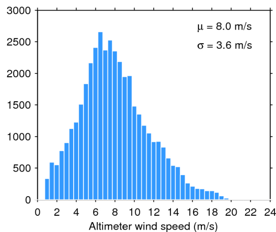
Figure 35. Histogram of science-valid wind over oceans and lakes for 22/10/2016. The mean ( \mu ) and standard deviation ( \sigma ) are also shown. Note that values larger than 24 m/s are excluded from the histogram for the sake of readability but not from the computation of \mu and \sigma .
