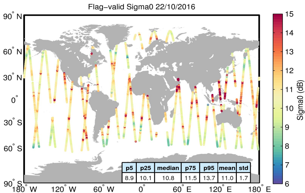
Figure 23. Geographical distribution of flag-valid sigma0 data over oceans and lakes for 22/10/2016. The statistical values shown in the table refer to the sigma0 in dB and are calculated over all measurements shown in the figure.
