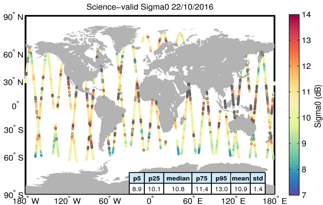
Figure 27. Geographical distribution of science-valid sigma0 data over oceans and lakes for 22/10/2016. The statistical values shown in the table refer to the sigma0 in dB and are calculated over all measurements shown in the figure. Gray circles denote records that have been rejected based on the editing criteria described in Table 4.
