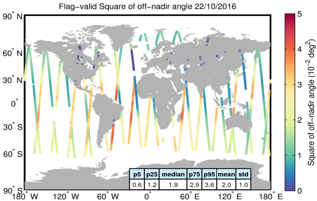
Figure 37. Geographical distribution of flag-valid mispointing data over oceans and lakes for 22/10/2016. The statistical values shown in the table refer to the mispointing in 10^{-2} deg 2 and are calculated over all measurements shown in the figure.
