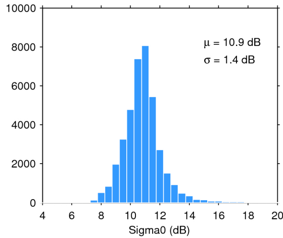
Figure 28. Histogram of science-valid sigma0 over oceans and lakes for 22/10/2016. The mean ( \mu ) and standard deviation ( \sigma ) are also shown. Note that values outside [4 20] dB are excluded from the histogram for the sake of readability but not from the computation of \mu and \sigma .
