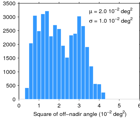
Figure 39. Histogram of flag-valid mispointing over oceans and lakes for 22/10/2016. The mean ( \mu ) and standard deviation ( \sigma ) are also shown. Note that values larger than 6 \cdot 10^{-2} \text{ deg}^2 are excluded from the histogram for the sake of readability but not from the computation of \mu and \sigma .
