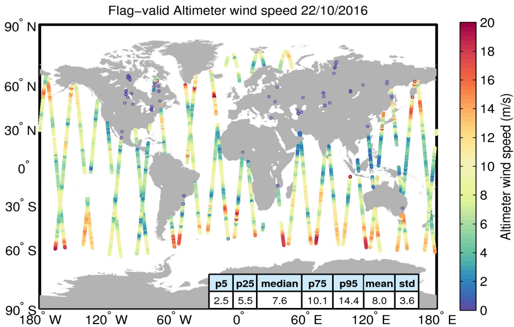
Figure 31. Geographical distribution of flag-valid wind data over oceans and lakes for 22/10/2016. The statistical values shown in the table refer to the wind in m/s and are calculated over all measurements shown in the figure.
