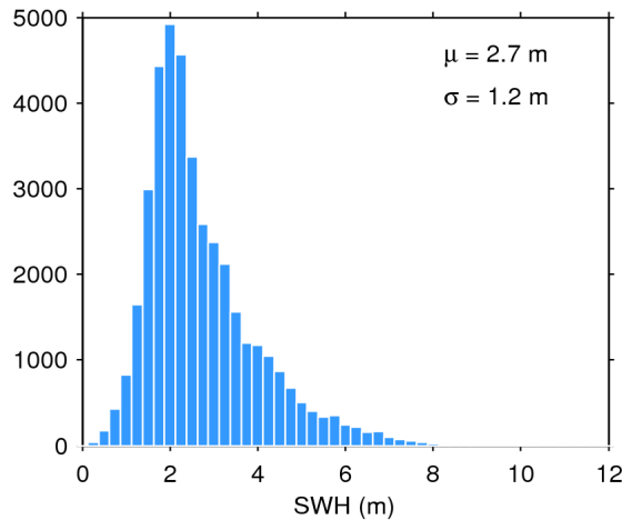
Figure 20. Histogram of science-valid SWH over oceans and lakes for 22/10/2016. The mean ( \mu ) and standard deviation ( \sigma ) are also shown. Note that values larger than 12 m are excluded from the histogram for the sake of readability but not from the computation of \mu and \sigma .
