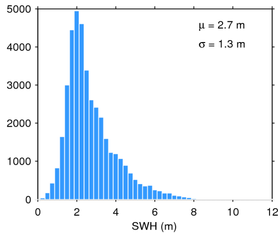
Figure 17. Histogram of flag-valid SWH over oceans and lakes for 22/10/2016. The mean ( \mu ) and standard deviation ( \sigma ) are also shown. Note that values larger than 12 m are excluded from the histogram for the sake of readability but not from the computation of \mu and \sigma .
