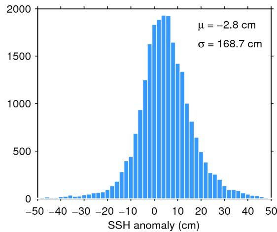
Figure 7. Histogram of flag-valid SSH anomaly over oceans and lakes for 22/10/2016. The mean ( \mu ) and standard deviation ( \sigma ) are also shown. Note that values outside [-50 50] cm are excluded from the histogram for the sake of readability but not from the computation of \mu and \sigma .
