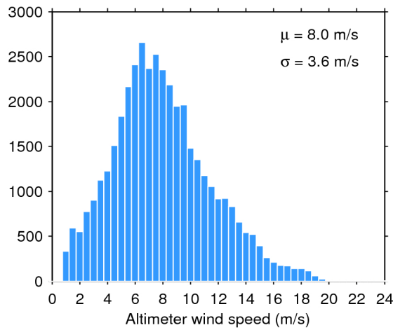
Figure 33. Histogram of flag-valid wind over oceans and lakes for 22/10/2016. The mean ( \mu ) and standard deviation ( \sigma ) are also shown. Note that values larger than 24 m/s are excluded from the histogram for the sake of readability but not from the computation of \mu and \sigma .
