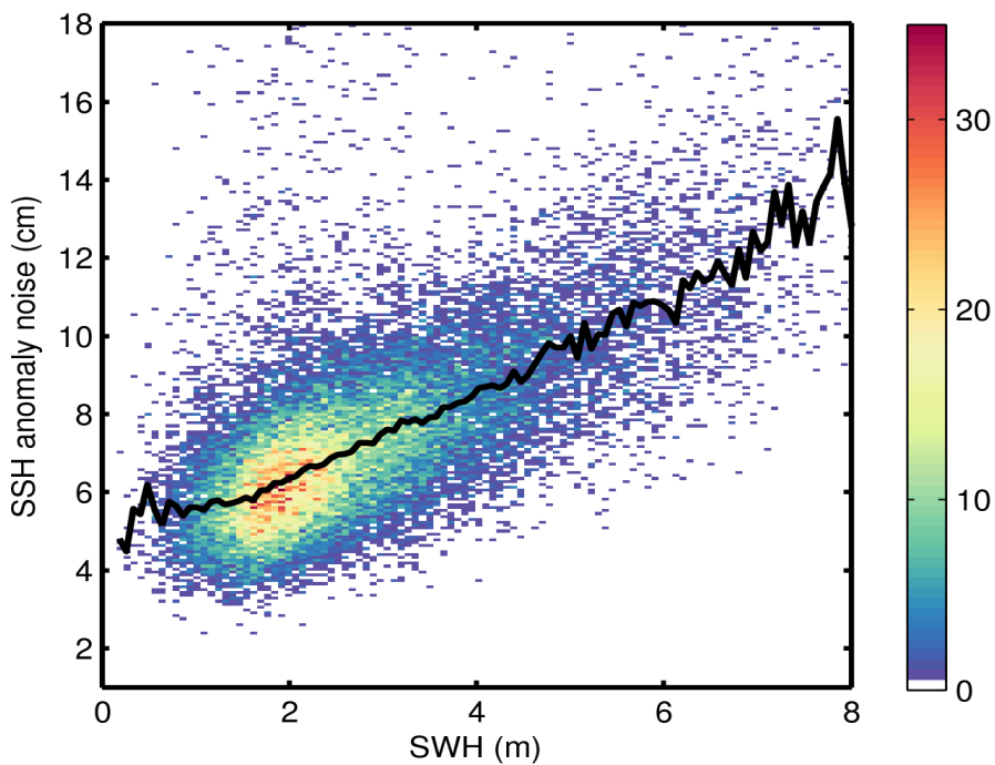
Figure 9. 2D histogram showing flag-valid SSH anomaly noise as a function of SWH for 22/10/2016. The black line denotes the median SSH anomaly noise as a function of SWH.
