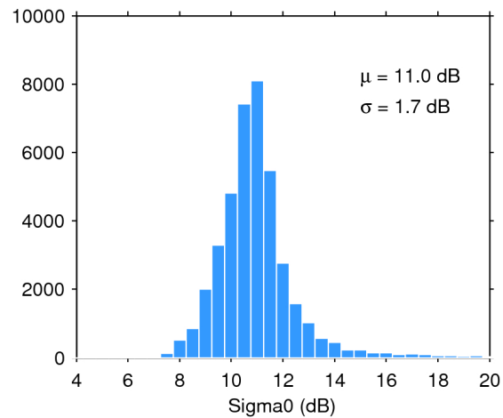
Figure 25. Histogram of flag-valid sigma0 over oceans and lakes for 22/10/2016. The mean ( \mu ) and standard deviation ( \sigma ) are also shown. Note that values outside [4 20] dB are excluded from the histogram for the sake of readability but not from the computation of \mu and \sigma .
