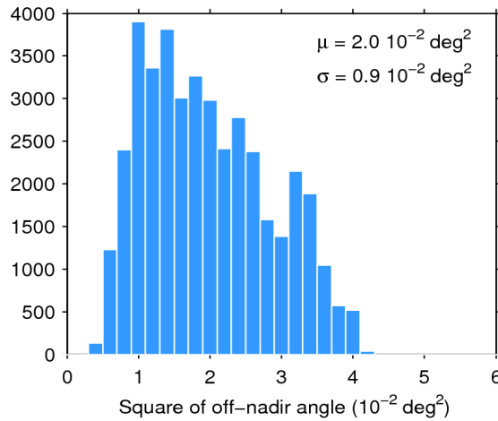
Figure 39. Histogram of flag-valid mispointing over oceans and lakes for 21/10/2016. The mean ( \mu ) and standard deviation ( \sigma ) are also shown. Note that values larger than 6 \cdot 10^{-2} \text{ deg}^2 are excluded from the histogram for the sake of readability but not from the computation of \mu and \sigma .
