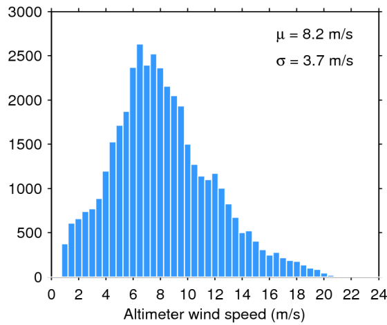
Figure 33. Histogram of flag-valid wind over oceans and lakes for 21/10/2016. The mean ( \mu ) and standard deviation ( \sigma ) are also shown. Note that values larger than 24 m/s are excluded from the histogram for the sake of readability but not from the computation of \mu and \sigma .
