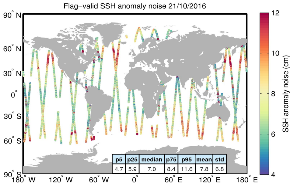
Figure 8. Geographical distribution of flag-valid 20-Hz SSH anomaly measurement noise over oceans and lakes for 21/10/2016. The statistical values shown in the table refer to the SSH anomaly noise and are calculated over all measurements shown in the figure.
