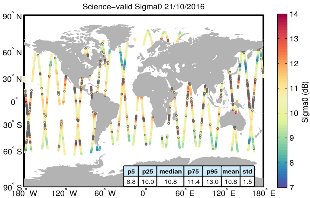
Figure 27. Geographical distribution of science-valid sigma0 data over oceans and lakes for 21/10/2016. The statistical values shown in the table refer to the sigma0 in dB and are calculated over all measurements shown in the figure. Gray circles denote records that have been rejected based on the editing criteria described in Table 4.
