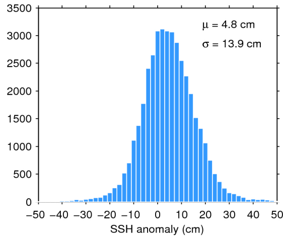
Figure 7. Histogram of flag-valid SSH anomaly over oceans and lakes for 21/10/2016. The mean ( \mu ) and standard deviation ( \sigma ) are also shown. Note that values outside [-50\ 50] cm are excluded from the histogram for the sake of readability but not from the computation of \mu and \sigma .
