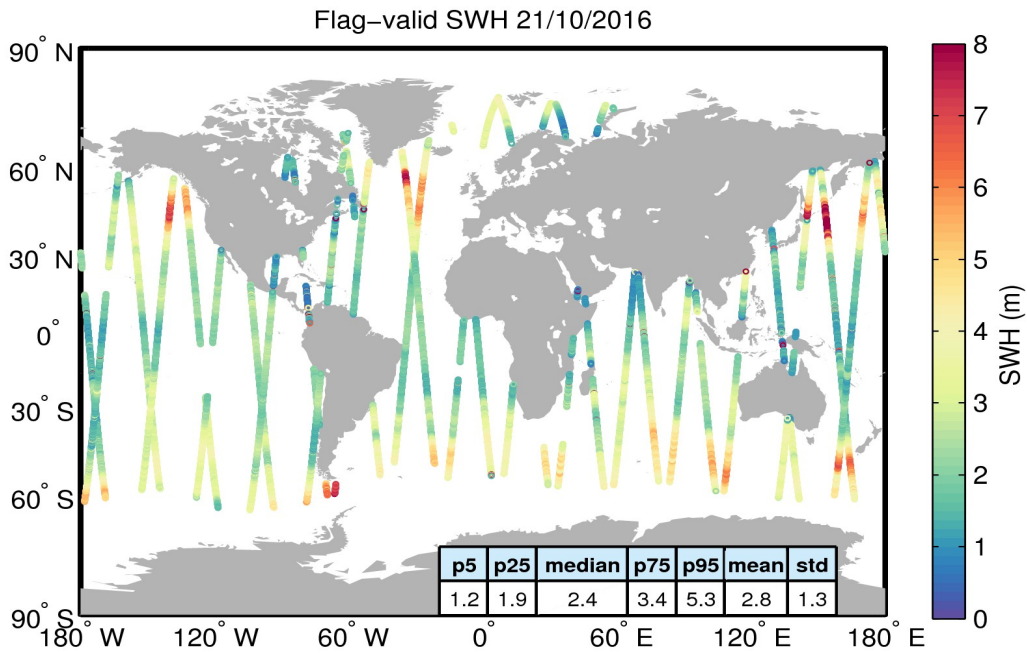
Figure 15. Geographical distribution of flag-valid SWH data over oceans and lakes for 21/10/2016. The statistical values shown in the table refer to the SWH in m and are calculated over all measurements shown in the figure.
