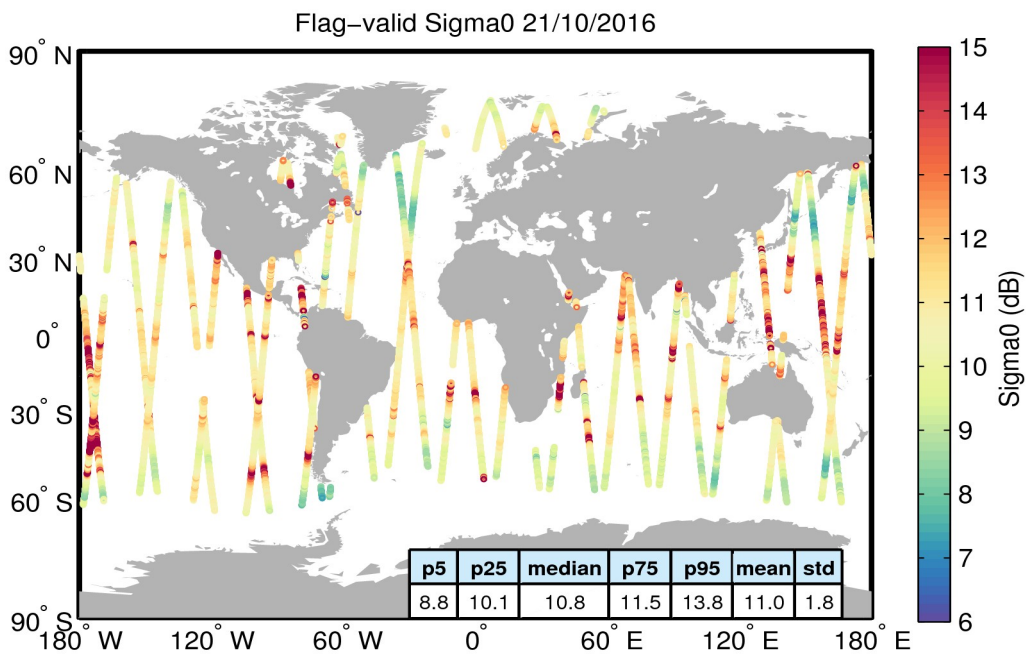
Figure 23. Geographical distribution of flag-valid sigma0 data over oceans and lakes for 21/10/2016. The statistical values shown in the table refer to the sigma0 in dB and are calculated over all measurements shown in the figure.
