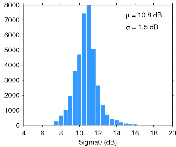
Figure 28. Histogram of science-valid sigma0 over oceans and lakes for 21/10/2016. The mean ( \mu ) and standard deviation ( \sigma ) are also shown. Note that values outside [4 20] dB are excluded from the histogram for the sake of readability but not from the computation of \mu and \sigma .
