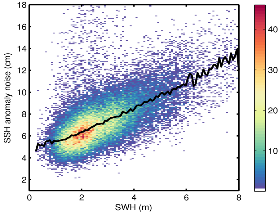
Figure 9. 2D histogram showing flag-valid SSH anomaly noise as a function of SWH for 21/10/2016. The black line denotes the median SSH anomaly noise as a function of SWH.
