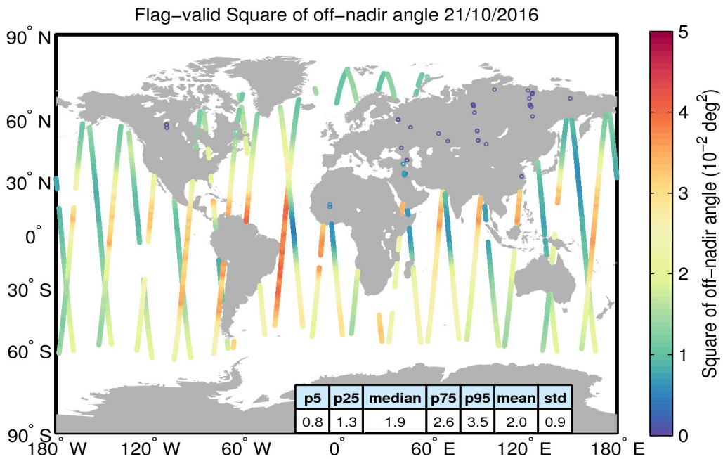
Figure 37. Geographical distribution of flag-valid mispointing data over oceans and lakes for 21/10/2016. The statistical values shown in the table refer to the mispointing in 10^{-2} deg 2 and are calculated over all measurements shown in the figure.
