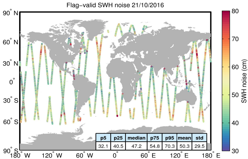
Figure 18. Geographical distribution of flag-valid 20-Hz SWH measurement noise over oceans and lakes for 21/10/2016. The statistical values shown in the table refer to the SWH noise and are calculated over all measurements shown in the figure.
