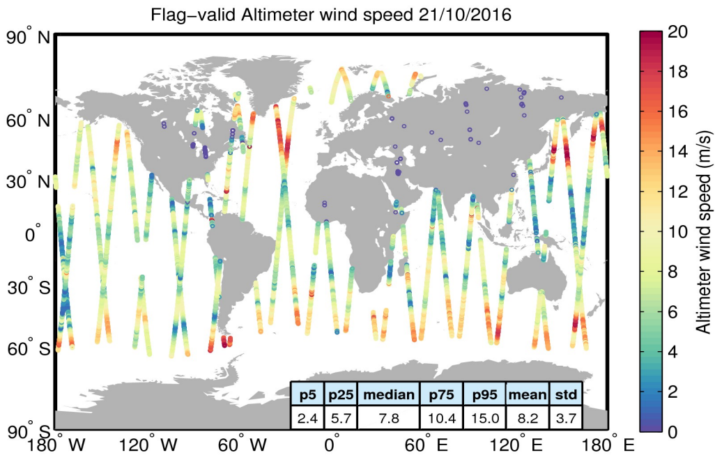
Figure 31. Geographical distribution of flag-valid wind data over oceans and lakes for 21/10/2016. The statistical values shown in the table refer to the wind in m/s and are calculated over all measurements shown in the figure.
