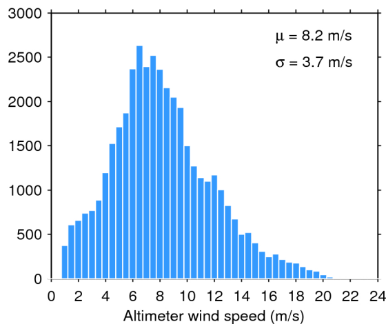
Figure 35. Histogram of science-valid wind over oceans and lakes for 21/10/2016. The mean ( \mu ) and standard deviation ( \sigma ) are also shown. Note that values larger than 24 m/s are excluded from the histogram for the sake of readability but not from the computation of \mu and \sigma .
