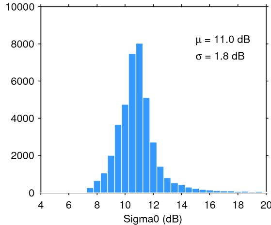
Figure 25. Histogram of flag-valid sigma0 over oceans and lakes for 21/10/2016. The mean ( \mu ) and standard deviation ( \sigma ) are also shown. Note that values outside [4 20] dB are excluded from the histogram for the sake of readability but not from the computation of \mu and \sigma .
