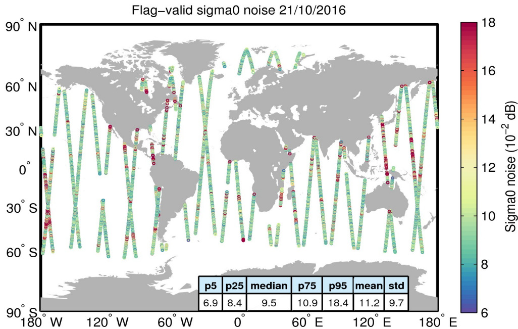
Figure 26. Geographical distribution of flag-valid 20-Hz sigma0 measurement noise over oceans and lakes for 21/10/2016. The statistical values shown in the table refer to the sigma0 noise and are calculated over all measurements shown in the figure.
