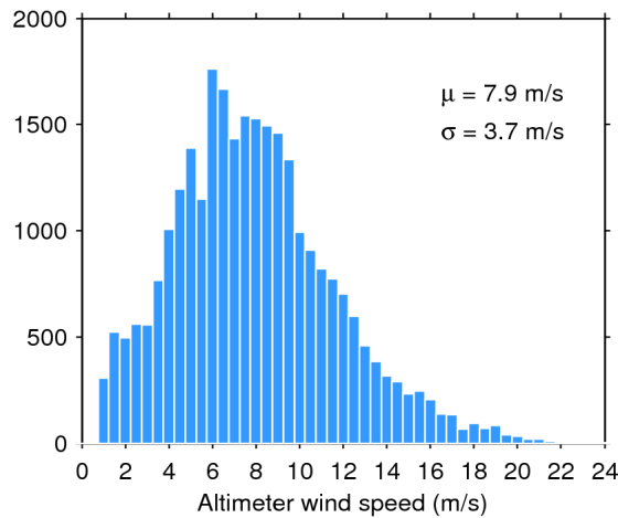
Figure 33. Histogram of flag-valid wind over oceans and lakes for 20/10/2016. The mean ( \mu ) and standard deviation ( \sigma ) are also shown. Note that values larger than 24 m/s are excluded from the histogram for the sake of readability but not from the computation of \mu and \sigma .
