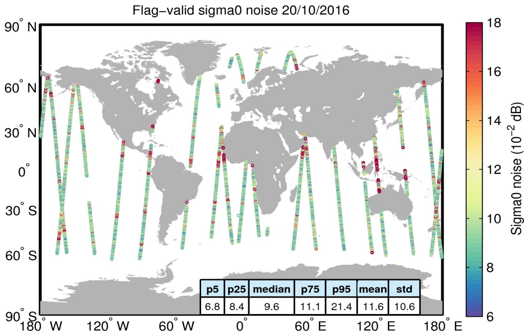
Figure 26. Geographical distribution of flag-valid 20-Hz sigma0 measurement noise over oceans and lakes for 20/10/2016. The statistical values shown in the table refer to the sigma0 noise and are calculated over all measurements shown in the figure.
