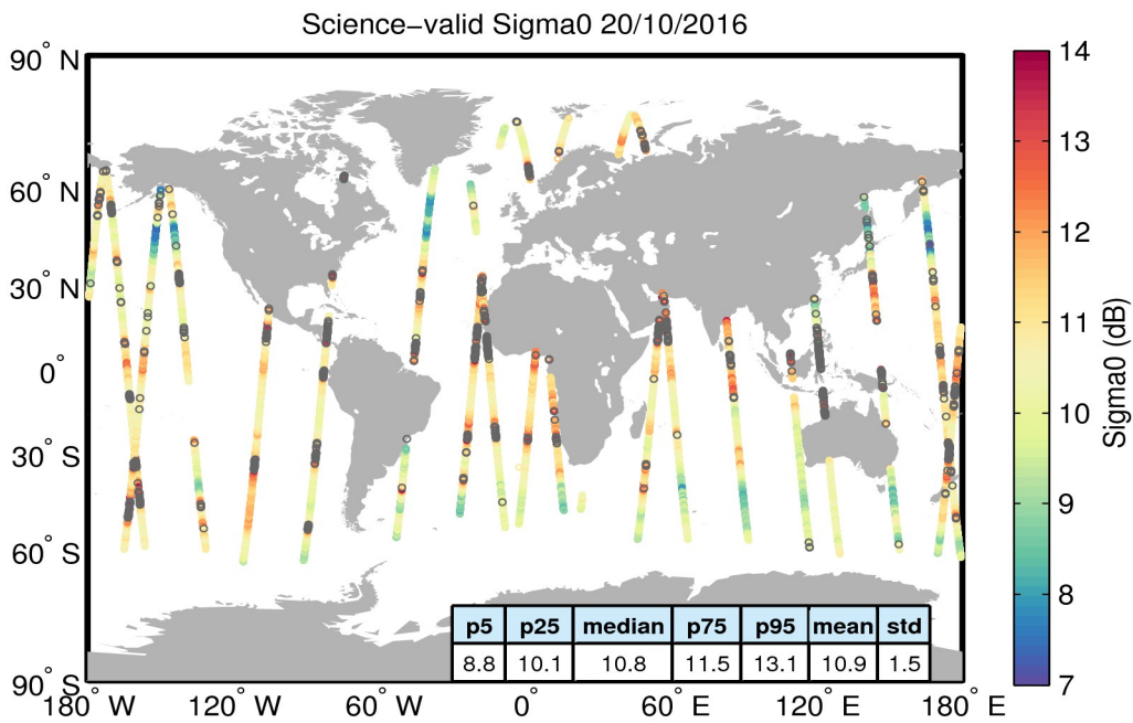
Figure 27. Geographical distribution of science-valid sigma0 data over oceans and lakes for 20/10/2016. The statistical values shown in the table refer to the sigma0 in dB and are calculated over all measurements shown in the figure. Gray circles denote records that have been rejected based on the editing criteria described in Table 4.
