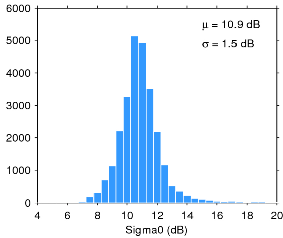
Figure 28. Histogram of science-valid sigma0 over oceans and lakes for 20/10/2016. The mean ( \mu ) and standard deviation ( \sigma ) are also shown. Note that values outside [4 20] dB are excluded from the histogram for the sake of readability but not from the computation of \mu and \sigma .
