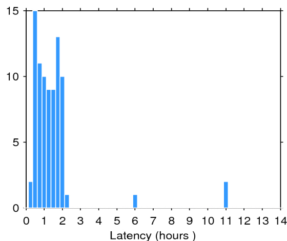
Figure 2. Histogram of the data latency for 20/10/2016. The y-axis denotes the number of files that are made available with a delay of x-hours with respect to the mean time of the records stored in the file.
