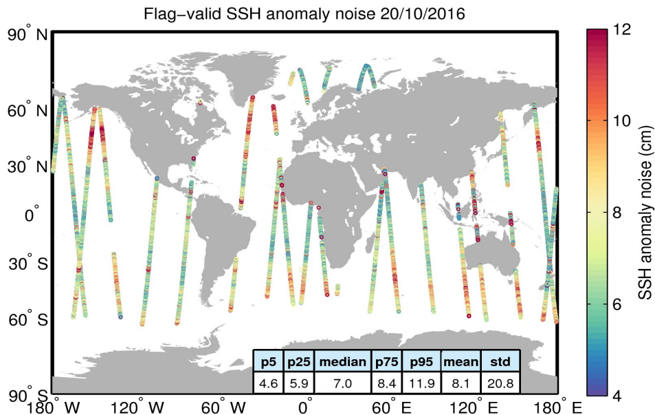
Figure 8. Geographical distribution of flag-valid 20-Hz SSH anomaly measurement noise over oceans and lakes for 20/10/2016. The statistical values shown in the table refer to the SSH anomaly noise and are calculated over all measurements shown in the figure.
