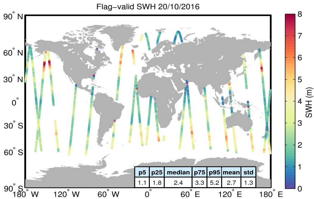
Figure 15. Geographical distribution of flag-valid SWH data over oceans and lakes for 20/10/2016. The statistical values shown in the table refer to the SWH in m and are calculated over all measurements shown in the figure.
