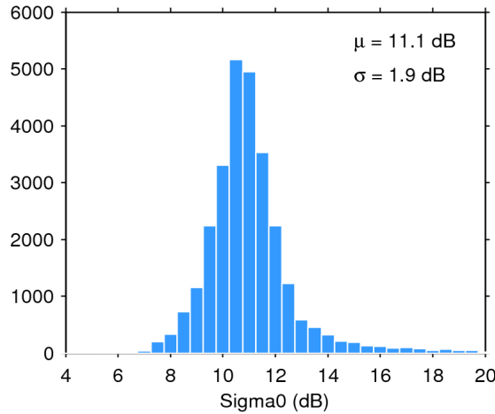
Figure 25. Histogram of flag-valid sigma0 over oceans and lakes for 20/10/2016. The mean ( \mu ) and standard deviation ( \sigma ) are also shown. Note that values outside [4 20] dB are excluded from the histogram for the sake of readability but not from the computation of \mu and \sigma .
