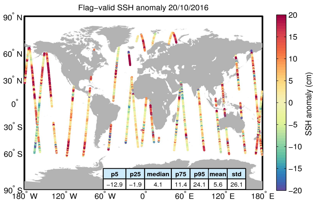
Figure 5. Geographical distribution of flag-valid 1-Hz SSH anomaly data over oceans and lakes for 20/10/2016. The statistical values shown in the table refer to the SSH anomaly in cm and are calculated over all measurements shown in the figure.
