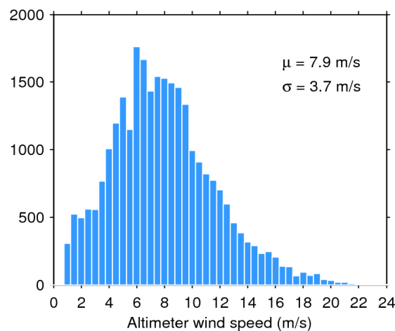
Figure 35. Histogram of science-valid wind over oceans and lakes for 20/10/2016. The mean ( \mu ) and standard deviation ( \sigma ) are also shown. Note that values larger than 24 m/s are excluded from the histogram for the sake of readability but not from the computation of \mu and \sigma .
