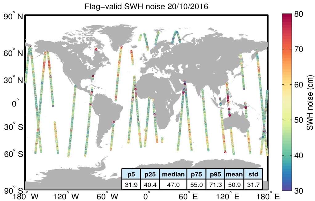
Figure 18. Geographical distribution of flag-valid 20-Hz SWH measurement noise over oceans and lakes for 20/10/2016. The statistical values shown in the table refer to the SWH noise and are calculated over all measurements shown in the figure.
