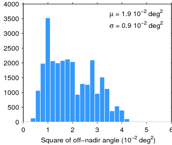
Figure 39. Histogram of flag-valid mispointing over oceans and lakes for 20/10/2016. The mean ( \mu ) and standard deviation ( \sigma ) are also shown. Note that values larger than 6 \cdot 10^{-2} \text{ deg}^2 are excluded from the histogram for the sake of readability but not from the computation of \mu and \sigma .
