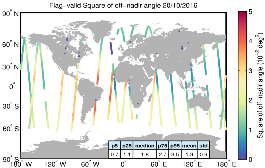
Figure 37. Geographical distribution of flag-valid mispointing data over oceans and lakes for 20/10/2016. The statistical values shown in the table refer to the mispointing in 10^{-2} \text{deg}^2 and are calculated over all measurements shown in the figure.
