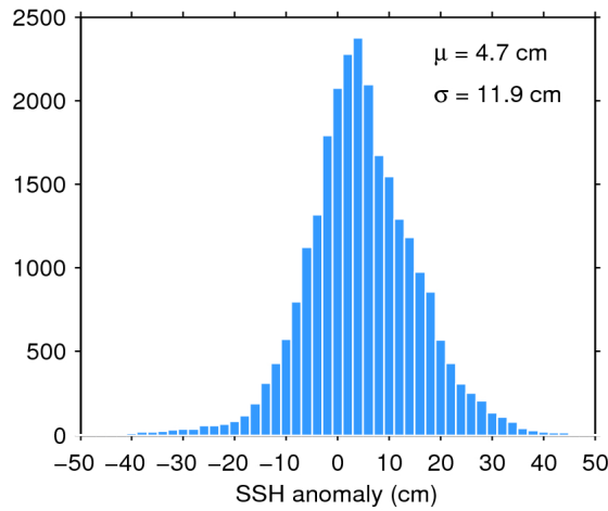
Figure 11. Histogram of science-valid SSH anomaly over oceans and lakes for 20/10/2016. The mean ( \mu ) and standard deviation ( \sigma ) are also shown. Note that values outside [-50 50] cm are excluded from the histogram for the sake of readability but not from the computation of \mu and \sigma .
