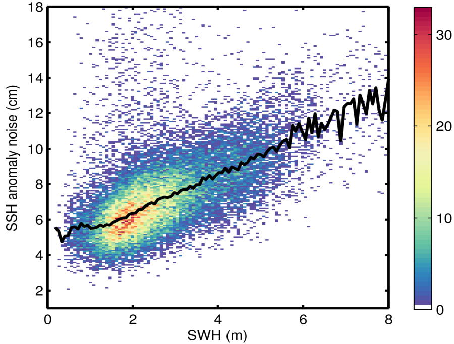
Figure 9. 2D histogram showing flag-valid SSH anomaly noise as a function of SWH for 20/10/2016. The black line denotes the median SSH anomaly noise as a function of SWH.
