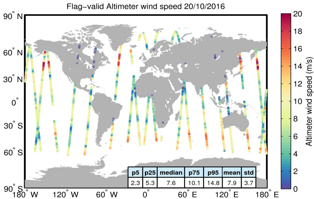
Figure 31. Geographical distribution of flag-valid wind data over oceans and lakes for 20/10/2016. The statistical values shown in the table refer to the wind in m/s and are calculated over all measurements shown in the figure.
