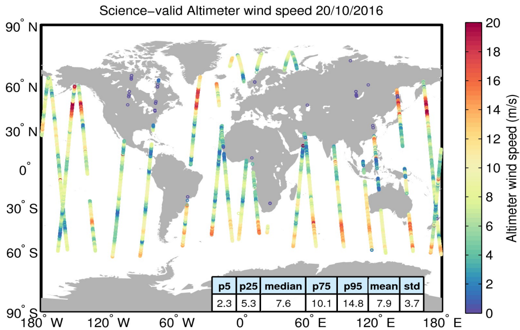
Figure 34. Geographical distribution of science-valid wind data over oceans and lakes for 20/10/2016. The statistical values shown in the table refer to the wind in m/s and are calculated over all measurements shown in the figure. Gray circles denote records that have been rejected based on the editing criteria described in Table 5.
