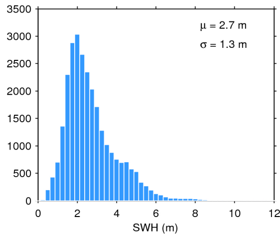
Figure 17. Histogram of flag-valid SWH over oceans and lakes for 20/10/2016. The mean ( \mu ) and standard deviation ( \sigma ) are also shown. Note that values larger than 12 m are excluded from the histogram for the sake of readability but not from the computation of \mu and \sigma .
