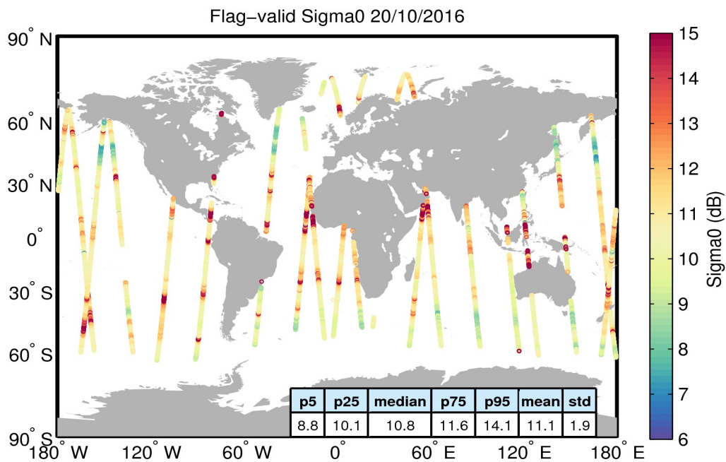
Figure 23. Geographical distribution of flag-valid sigma0 data over oceans and lakes for 20/10/2016. The statistical values shown in the table refer to the sigma0 in dB and are calculated over all measurements shown in the figure.
