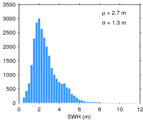
Figure 20. Histogram of science-valid SWH over oceans and lakes for 20/10/2016. The mean ( \mu ) and standard deviation ( \sigma ) are also shown. Note that values larger than 12 m are excluded from the histogram for the sake of readability but not from the computation of \mu and \sigma .
