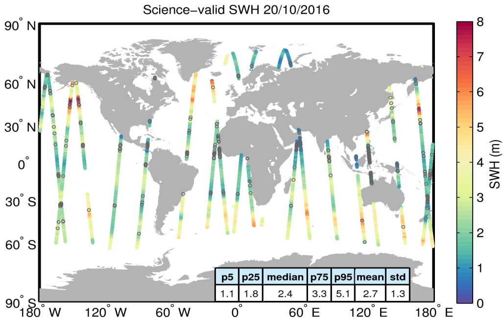
Figure 19. Geographical distribution of science-valid SWH data over oceans and lakes for 20/10/2016. The statistical values shown in the table refer to the SWH in m and are calculated over all measurements shown in the figure. Gray circles denote records that have been rejected based on the editing criteria described in Table 3.
