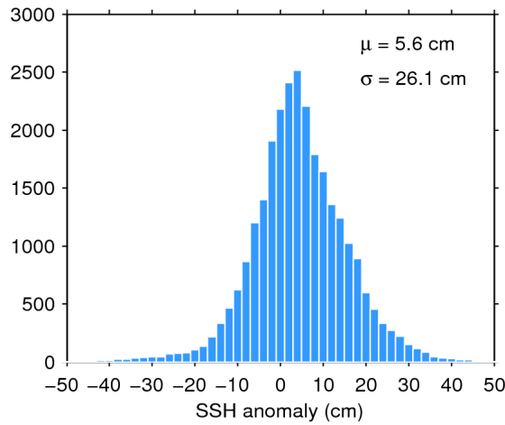
Figure 7. Histogram of flag-valid SSH anomaly over oceans and lakes for 20/10/2016. The mean ( \mu ) and standard deviation ( \sigma ) are also shown. Note that values outside [-50 50] cm are excluded from the histogram for the sake of readability but not from the computation of \mu and \sigma .
