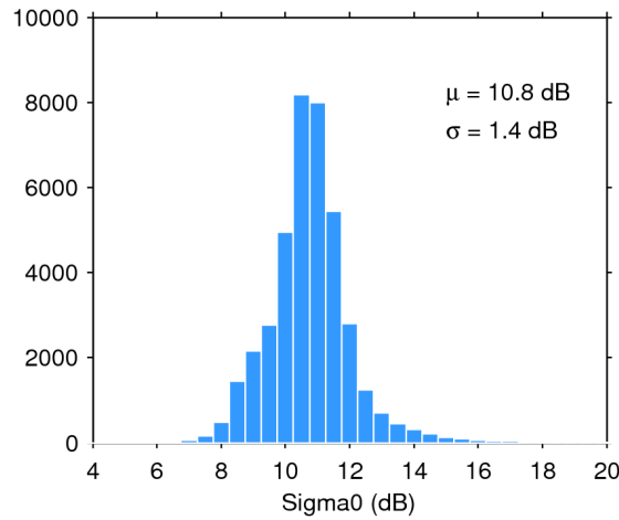
Figure 28. Histogram of science-valid sigma0 over oceans and lakes for 19/10/2016. The mean ( \mu ) and standard deviation ( \sigma ) are also shown. Note that values outside [4 20] dB are excluded from the histogram for the sake of readability but not from the computation of \mu and \sigma .
