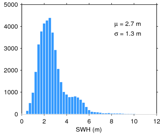
Figure 17. Histogram of flag-valid SWH over oceans and lakes for 19/10/2016. The mean ( \mu ) and standard deviation ( \sigma ) are also shown. Note that values larger than 12 m are excluded from the histogram for the sake of readability but not from the computation of \mu and \sigma .
