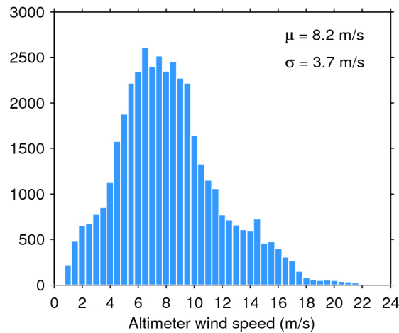
Figure 33. Histogram of flag-valid wind over oceans and lakes for 19/10/2016. The mean ( \mu ) and standard deviation ( \sigma ) are also shown. Note that values larger than 24 m/s are excluded from the histogram for the sake of readability but not from the computation of \mu and \sigma .
