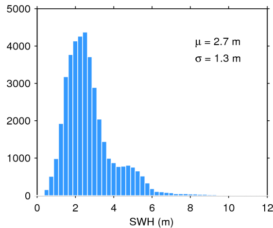
Figure 20. Histogram of science-valid SWH over oceans and lakes for 19/10/2016. The mean ( \mu ) and standard deviation ( \sigma ) are also shown. Note that values larger than 12 m are excluded from the histogram for the sake of readability but not from the computation of \mu and \sigma .
