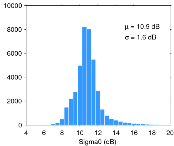
Figure 25. Histogram of flag-valid sigma0 over oceans and lakes for 19/10/2016. The mean ( \mu ) and standard deviation ( \sigma ) are also shown. Note that values outside [4 20] dB are excluded from the histogram for the sake of readability but not from the computation of \mu and \sigma .
