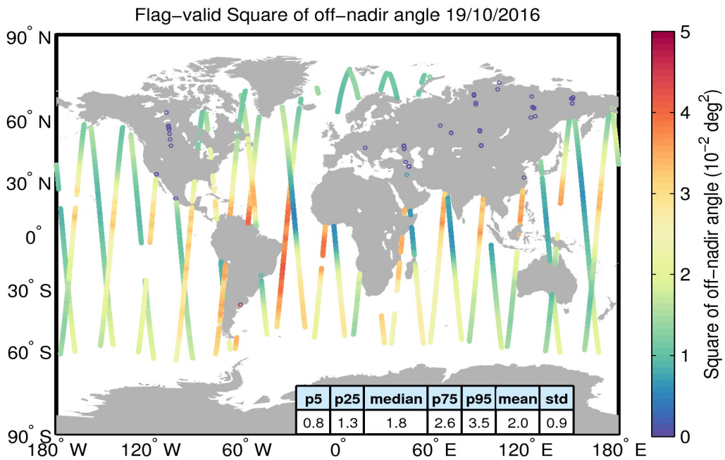
Figure 37. Geographical distribution of flag-valid mispointing data over oceans and lakes for 19/10/2016. The statistical values shown in the table refer to the mispointing in 10^{-2} deg 2 and are calculated over all measurements shown in the figure.
