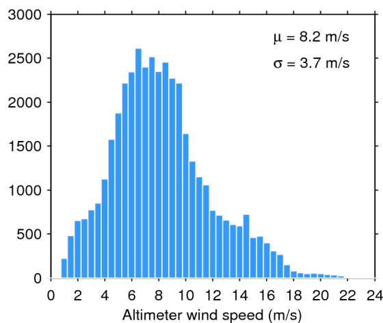
Figure 35. Histogram of science-valid wind over oceans and lakes for 19/10/2016. The mean ( \mu ) and standard deviation ( \sigma ) are also shown. Note that values larger than 24 m/s are excluded from the histogram for the sake of readability but not from the computation of \mu and \sigma .
