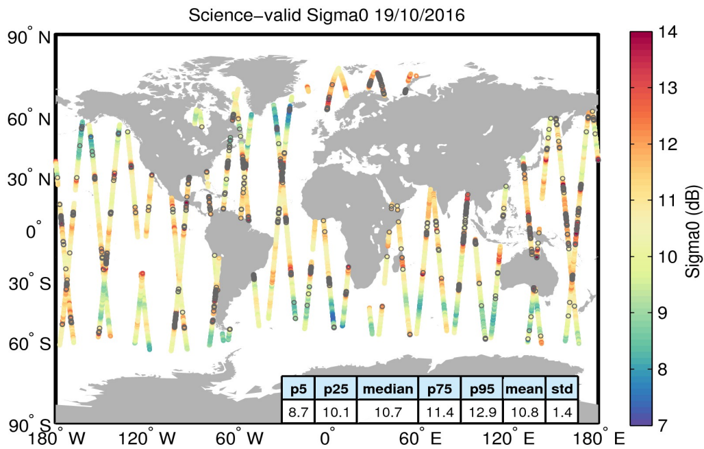
Figure 27. Geographical distribution of science-valid sigma0 data over oceans and lakes for 19/10/2016. The statistical values shown in the table refer to the sigma0 in dB and are calculated over all measurements shown in the figure. Gray circles denote records that have been rejected based on the editing criteria described in Table 4.
