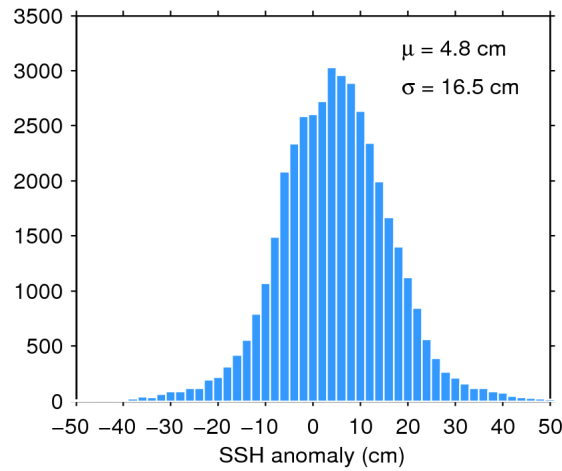
Figure 7. Histogram of flag-valid SSH anomaly over oceans and lakes for 19/10/2016. The mean ( \mu ) and standard deviation ( \sigma ) are also shown. Note that values outside [-50 50] cm are excluded from the histogram for the sake of readability but not from the computation of \mu and \sigma .
