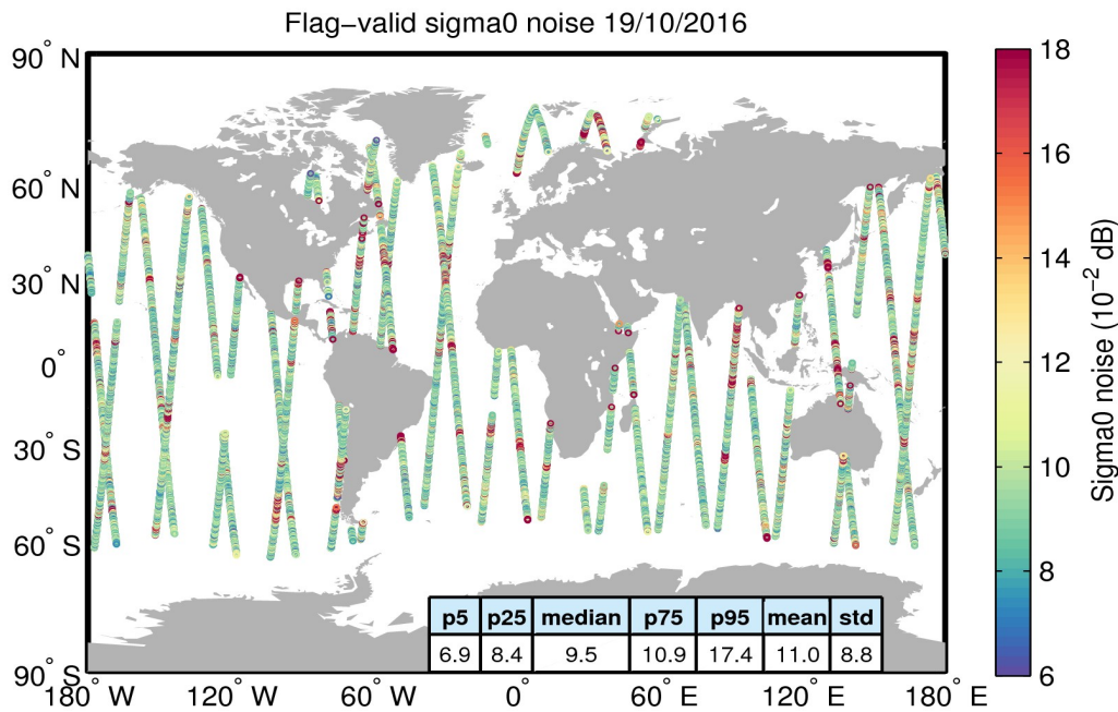
Figure 26. Geographical distribution of flag-valid 20-Hz sigma0 measurement noise over oceans and lakes for 19/10/2016. The statistical values shown in the table refer to the sigma0 noise and are calculated over all measurements shown in the figure.
