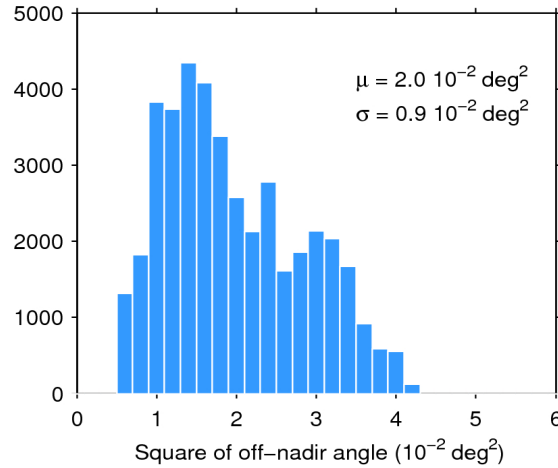
Figure 39. Histogram of flag-valid mispointing over oceans and lakes for 19/10/2016. The mean ( \mu ) and standard deviation ( \sigma ) are also shown. Note that values larger than 6 \cdot 10^{-2} \text{ deg}^2 are excluded from the histogram for the sake of readability but not from the computation of \mu and \sigma .
