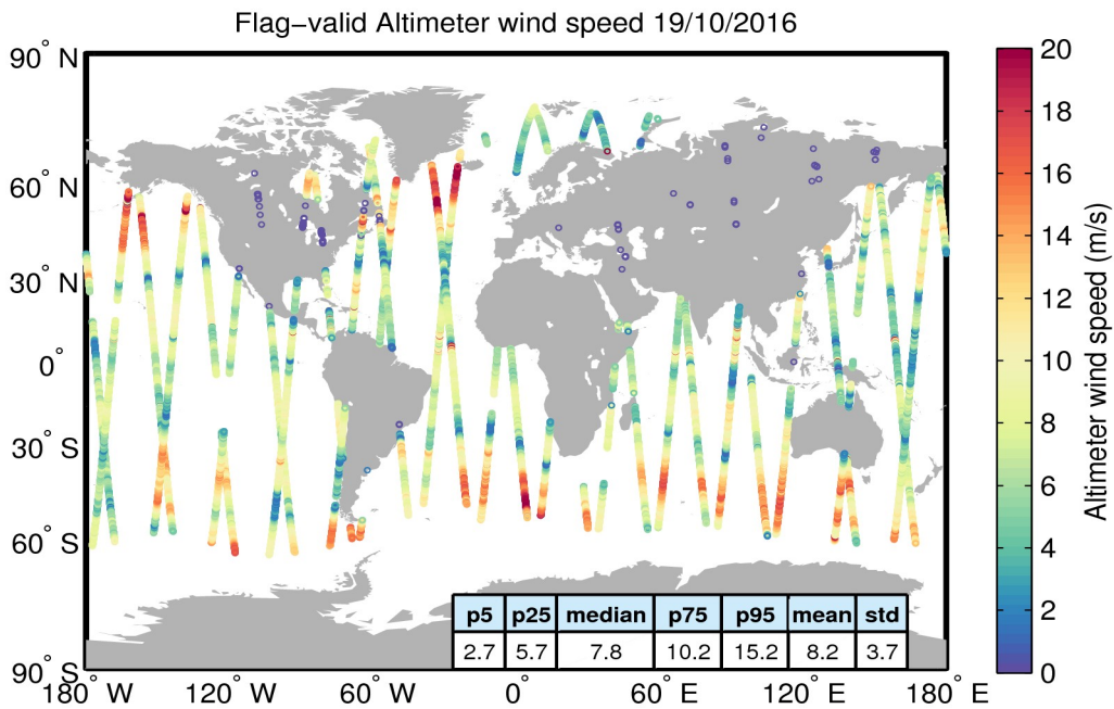
Figure 31. Geographical distribution of flag-valid wind data over oceans and lakes for 19/10/2016. The statistical values shown in the table refer to the wind in m/s and are calculated over all measurements shown in the figure.
