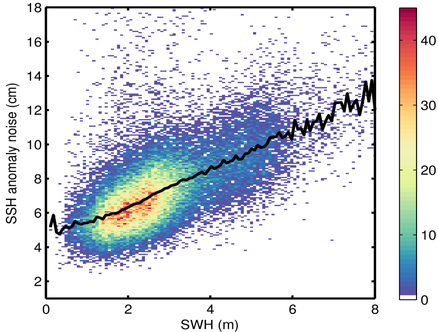
Figure 9. 2D histogram showing flag-valid SSH anomaly noise as a function of SWH for 19/10/2016. The black line denotes the median SSH anomaly noise as a function of SWH.
