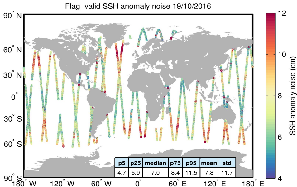
Figure 8. Geographical distribution of flag-valid 20-Hz SSH anomaly measurement noise over oceans and lakes for 19/10/2016. The statistical values shown in the table refer to the SSH anomaly noise and are calculated over all measurements shown in the figure.
