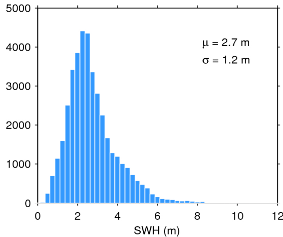
Figure 20. Histogram of science-valid SWH over oceans and lakes for 18/10/2016. The mean ( \mu ) and standard deviation ( \sigma ) are also shown. Note that values larger than 12 m are excluded from the histogram for the sake of readability but not from the computation of \mu and \sigma .
