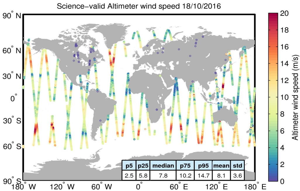
Figure 34. Geographical distribution of science-valid wind data over oceans and lakes for 18/10/2016. The statistical values shown in the table refer to the wind in m/s and are calculated over all measurements shown in the figure. Gray circles denote records that have been rejected based on the editing criteria described in Table 5.
