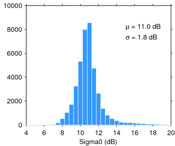
Figure 25. Histogram of flag-valid sigma0 over oceans and lakes for 18/10/2016. The mean ( \mu ) and standard deviation ( \sigma ) are also shown. Note that values outside [4 20] dB are excluded from the histogram for the sake of readability but not from the computation of \mu and \sigma .
