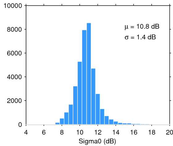
Figure 28. Histogram of science-valid sigma0 over oceans and lakes for 18/10/2016. The mean ( \mu ) and standard deviation ( \sigma ) are also shown. Note that values outside [4 20] dB are excluded from the histogram for the sake of readability but not from the computation of \mu and \sigma .
