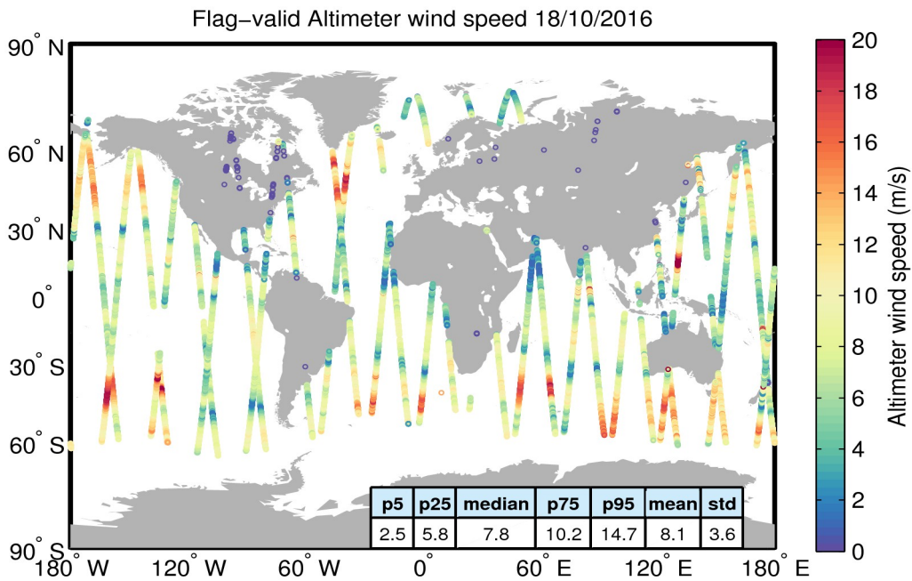
Figure 31. Geographical distribution of flag-valid wind data over oceans and lakes for 18/10/2016. The statistical values shown in the table refer to the wind in m/s and are calculated over all measurements shown in the figure.
