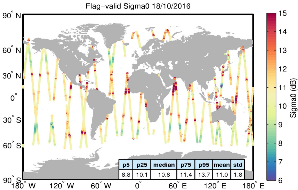
Figure 23. Geographical distribution of flag-valid sigma0 data over oceans and lakes for 18/10/2016. The statistical values shown in the table refer to the sigma0 in dB and are calculated over all measurements shown in the figure.
