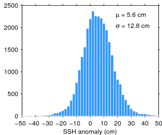
Figure 11. Histogram of science-valid SSH anomaly over oceans and lakes for 18/10/2016. The mean ( \mu ) and standard deviation ( \sigma ) are also shown. Note that values outside [-50 50] cm are excluded from the histogram for the sake of readability but not from the computation of \mu and \sigma .
