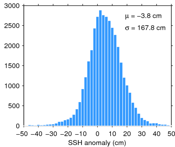
Figure 7. Histogram of flag-valid SSH anomaly over oceans and lakes for 18/10/2016. The mean ( \mu ) and standard deviation ( \sigma ) are also shown. Note that values outside [-50 50] cm are excluded from the histogram for the sake of readability but not from the computation of \mu and \sigma .
