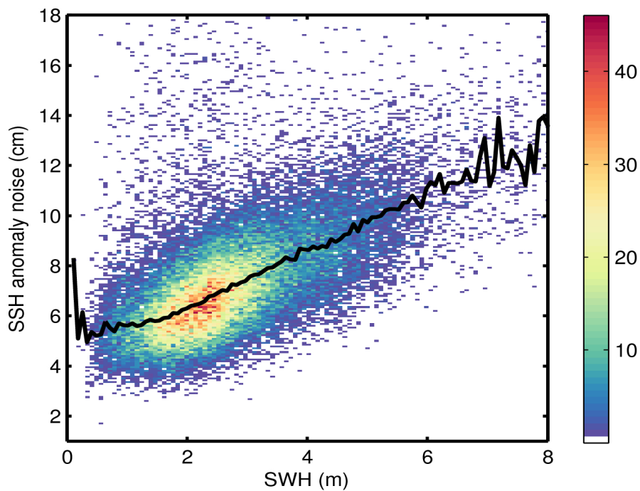
Figure 9. 2D histogram showing flag-valid SSH anomaly noise as a function of SWH for 18/10/2016. The black line denotes the median SSH anomaly noise as a function of SWH.
