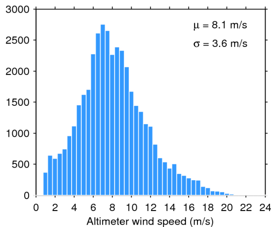
Figure 35. Histogram of science-valid wind over oceans and lakes for 18/10/2016. The mean ( \mu ) and standard deviation ( \sigma ) are also shown. Note that values larger than 24 m/s are excluded from the histogram for the sake of readability but not from the computation of \mu and \sigma .
