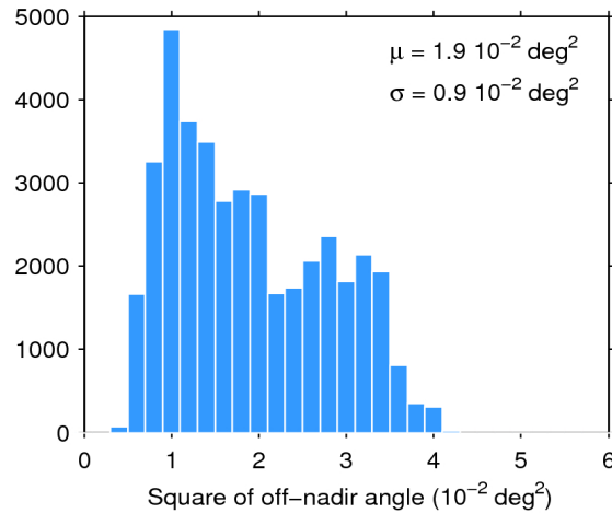
Figure 39. Histogram of flag-valid mispointing over oceans and lakes for 18/10/2016. The mean ( \mu ) and standard deviation ( \sigma ) are also shown. Note that values larger than 6 \cdot 10^{-2} \text{ deg}^2 are excluded from the histogram for the sake of readability but not from the computation of \mu and \sigma .
