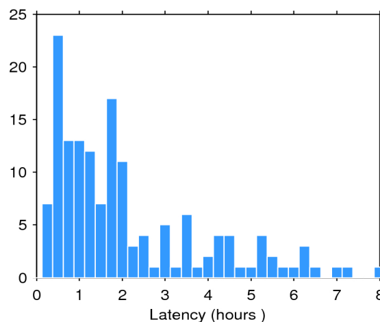
Figure 2. Histogram of the data latency for 18/10/2016. The y-axis denotes the number of files that are made available with a delay of x-hours with respect to the mean time of the records stored in the file.
