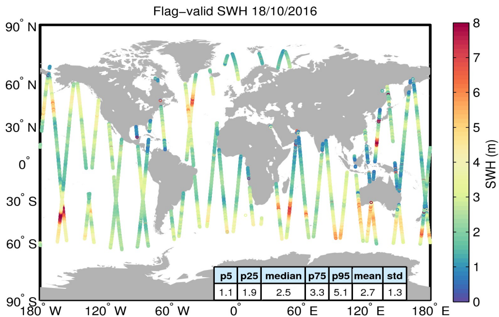
Figure 15. Geographical distribution of flag-valid SWH data over oceans and lakes for 18/10/2016. The statistical values shown in the table refer to the SWH in m and are calculated over all measurements shown in the figure.
