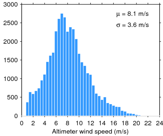
Figure 33. Histogram of flag-valid wind over oceans and lakes for 18/10/2016. The mean ( \mu ) and standard deviation ( \sigma ) are also shown. Note that values larger than 24 m/s are excluded from the histogram for the sake of readability but not from the computation of \mu and \sigma .
