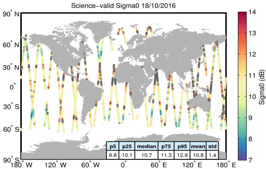
Figure 27. Geographical distribution of science-valid sigma0 data over oceans and lakes for 18/10/2016. The statistical values shown in the table refer to the sigma0 in dB and are calculated over all measurements shown in the figure. Gray circles denote records that have been rejected based on the editing criteria described in Table 4.
