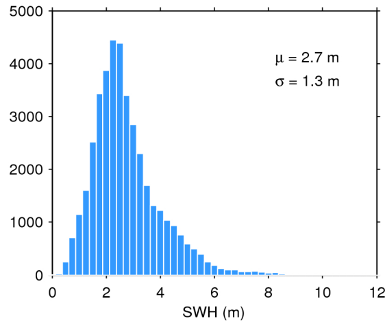
Figure 17. Histogram of flag-valid SWH over oceans and lakes for 18/10/2016. The mean ( \mu ) and standard deviation ( \sigma ) are also shown. Note that values larger than 12 m are excluded from the histogram for the sake of readability but not from the computation of \mu and \sigma .
