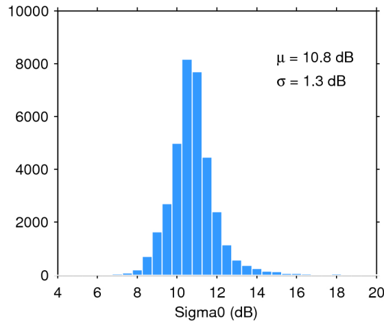
Figure 28. Histogram of science-valid sigma0 over oceans and lakes for 17/10/2016. The mean ( \mu ) and standard deviation ( \sigma ) are also shown. Note that values outside [4 20] dB are excluded from the histogram for the sake of readability but not from the computation of \mu and \sigma .
