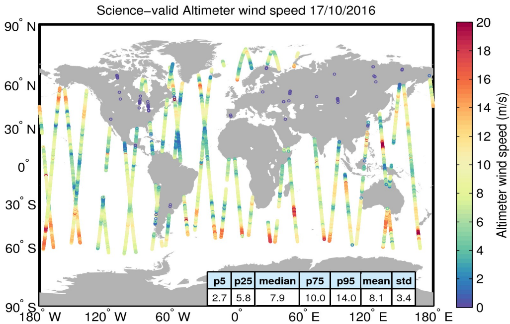
Figure 34. Geographical distribution of science-valid wind data over oceans and lakes for 17/10/2016. The statistical values shown in the table refer to the wind in m/s and are calculated over all measurements shown in the figure. Gray circles denote records that have been rejected based on the editing criteria described in Table 5.
