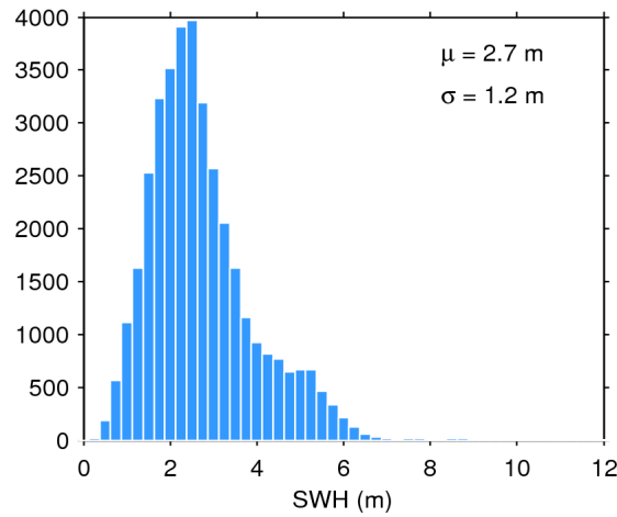
Figure 17. Histogram of flag-valid SWH over oceans and lakes for 17/10/2016. The mean ( \mu ) and standard deviation ( \sigma ) are also shown. Note that values larger than 12 m are excluded from the histogram for the sake of readability but not from the computation of \mu and \sigma .
