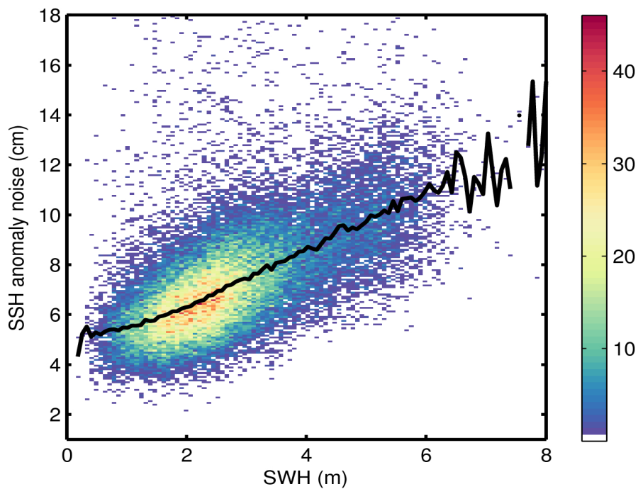
Figure 9. 2D histogram showing flag-valid SSH anomaly noise as a function of SWH for 17/10/2016. The black line denotes the median SSH anomaly noise as a function of SWH.
