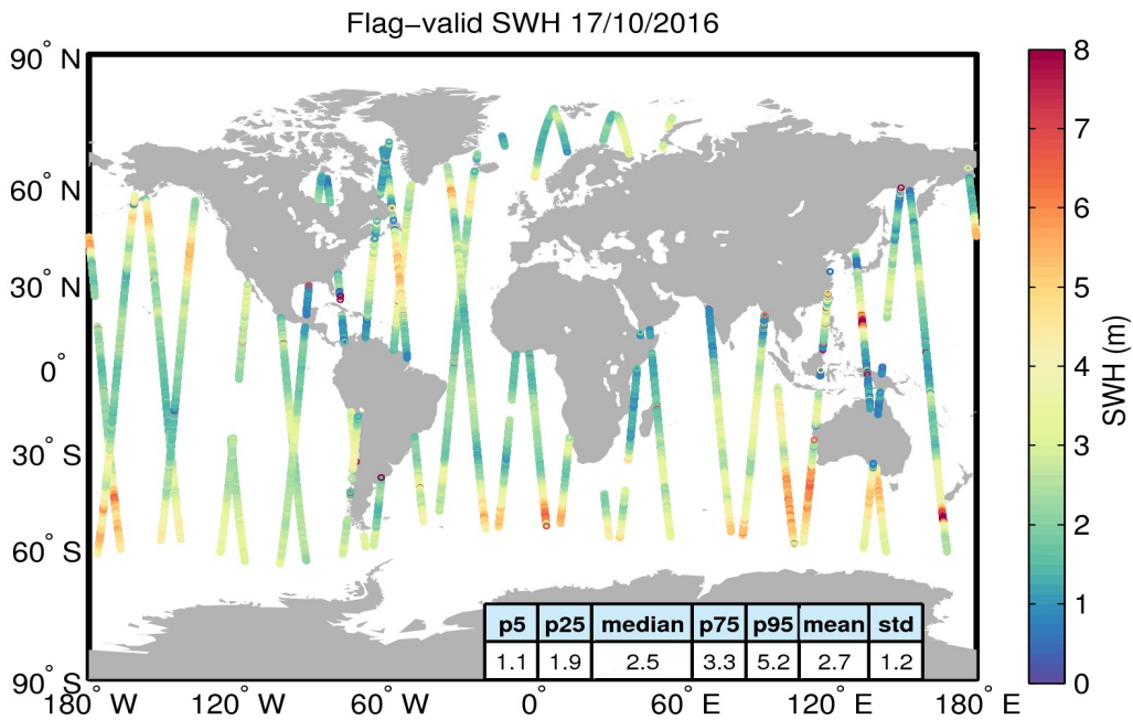
Figure 15. Geographical distribution of flag-valid SWH data over oceans and lakes for 17/10/2016. The statistical values shown in the table refer to the SWH in m and are calculated over all measurements shown in the figure.
