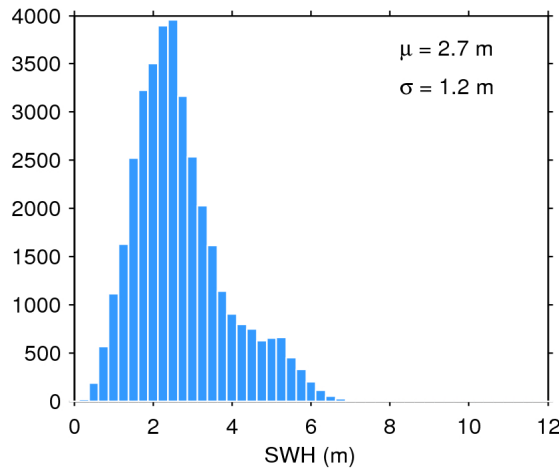
Figure 20. Histogram of science-valid SWH over oceans and lakes for 17/10/2016. The mean ( \mu ) and standard deviation ( \sigma ) are also shown. Note that values larger than 12 m are excluded from the histogram for the sake of readability but not from the computation of \mu and \sigma .
