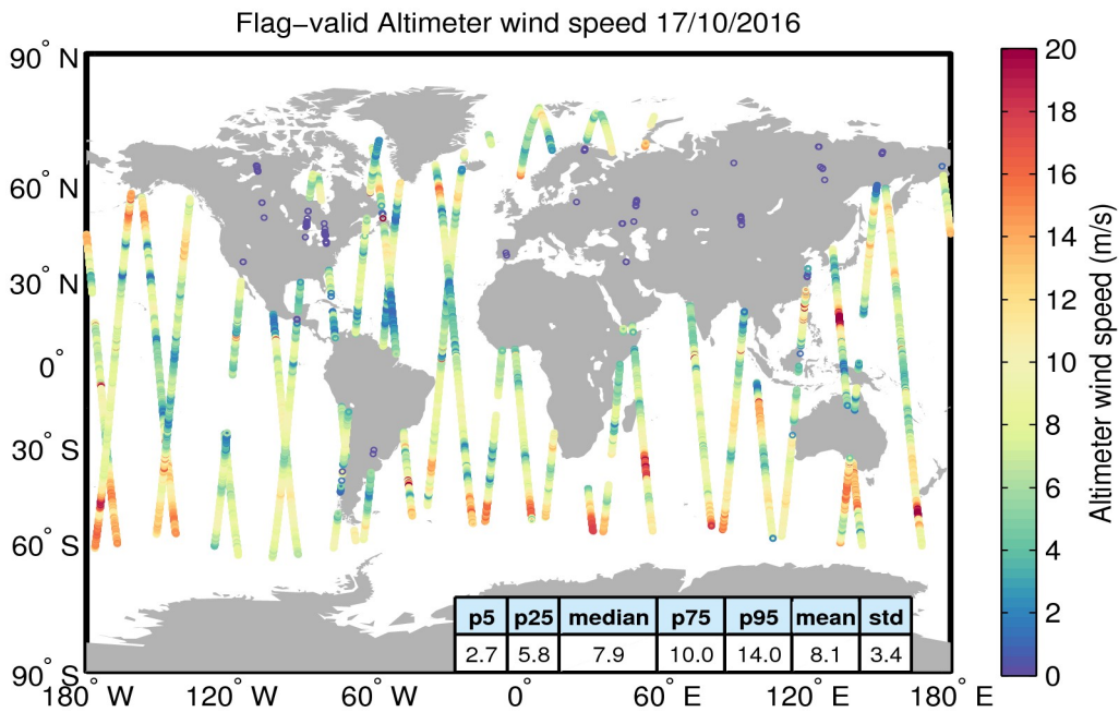
Figure 31. Geographical distribution of flag-valid wind data over oceans and lakes for 17/10/2016. The statistical values shown in the table refer to the wind in m/s and are calculated over all measurements shown in the figure.
