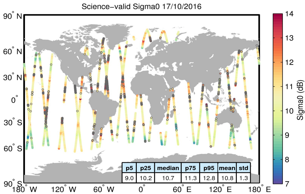
Figure 27. Geographical distribution of science-valid sigma0 data over oceans and lakes for 17/10/2016. The statistical values shown in the table refer to the sigma0 in dB and are calculated over all measurements shown in the figure. Gray circles denote records that have been rejected based on the editing criteria described in Table 4.
