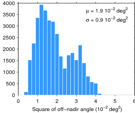
Figure 39. Histogram of flag-valid mispointing over oceans and lakes for 17/10/2016. The mean ( \mu ) and standard deviation ( \sigma ) are also shown. Note that values larger than 6 \cdot 10^{-2} \text{ deg}^2 are excluded from the histogram for the sake of readability but not from the computation of \mu and \sigma .
