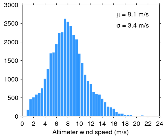
Figure 33. Histogram of flag-valid wind over oceans and lakes for 17/10/2016. The mean ( \mu ) and standard deviation ( \sigma ) are also shown. Note that values larger than 24 m/s are excluded from the histogram for the sake of readability but not from the computation of \mu and \sigma .
