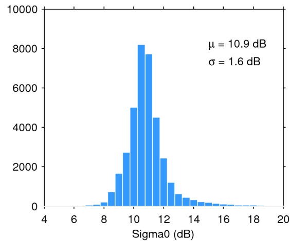
Figure 25. Histogram of flag-valid sigma0 over oceans and lakes for 17/10/2016. The mean ( \mu ) and standard deviation ( \sigma ) are also shown. Note that values outside [4 20] dB are excluded from the histogram for the sake of readability but not from the computation of \mu and \sigma .
