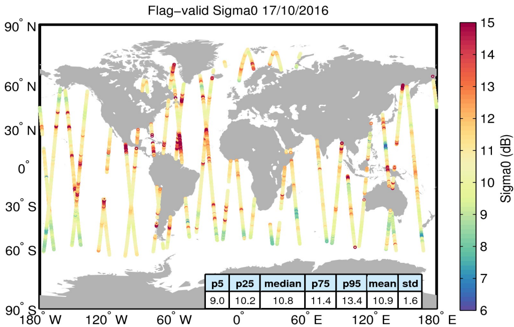
Figure 23. Geographical distribution of flag-valid sigma0 data over oceans and lakes for 17/10/2016. The statistical values shown in the table refer to the sigma0 in dB and are calculated over all measurements shown in the figure.
