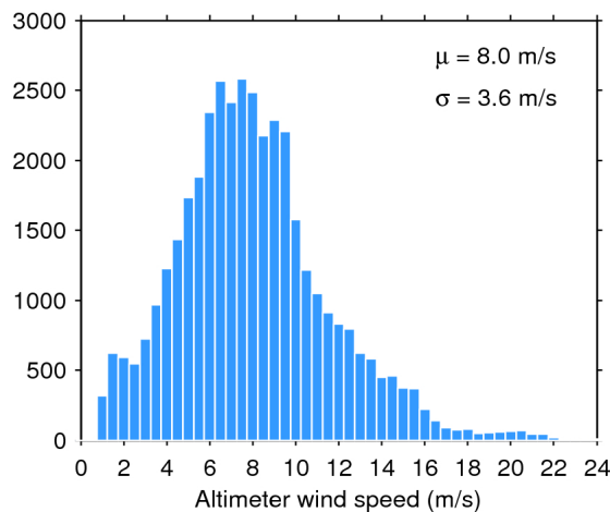
Figure 35. Histogram of science-valid wind over oceans and lakes for 15/10/2016. The mean ( \mu ) and standard deviation ( \sigma ) are also shown. Note that values larger than 24 m/s are excluded from the histogram for the sake of readability but not from the computation of \mu and \sigma .
