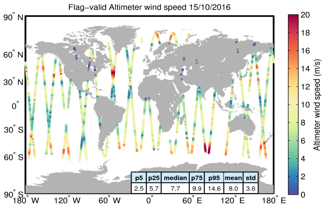
Figure 31. Geographical distribution of flag-valid wind data over oceans and lakes for 15/10/2016. The statistical values shown in the table refer to the wind in m/s and are calculated over all measurements shown in the figure.
