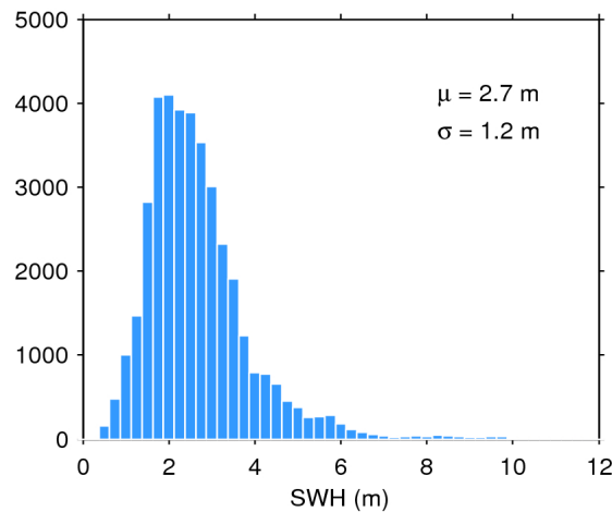
Figure 20. Histogram of science-valid SWH over oceans and lakes for 15/10/2016. The mean ( \mu ) and standard deviation ( \sigma ) are also shown. Note that values larger than 12 m are excluded from the histogram for the sake of readability but not from the computation of \mu and \sigma .
