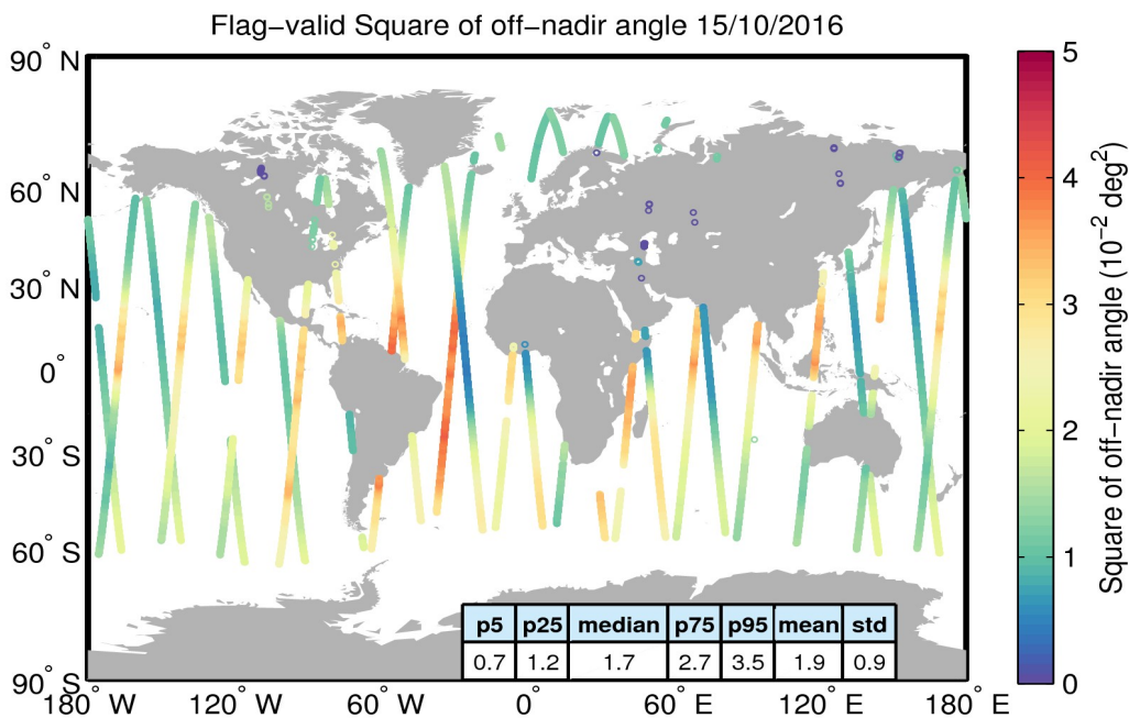
Figure 37. Geographical distribution of flag-valid mispointing data over oceans and lakes for 15/10/2016. The statistical values shown in the table refer to the mispointing in 10^{-2} deg 2 and are calculated over all measurements shown in the figure.
