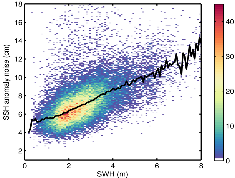
Figure 9. 2D histogram showing flag-valid SSH anomaly noise as a function of SWH for 15/10/2016. The black line denotes the median SSH anomaly noise as a function of SWH.
