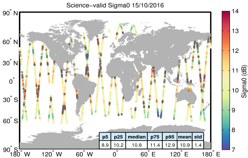
Figure 27. Geographical distribution of science-valid sigma0 data over oceans and lakes for 15/10/2016. The statistical values shown in the table refer to the sigma0 in dB and are calculated over all measurements shown in the figure. Gray circles denote records that have been rejected based on the editing criteria described in Table 4.
