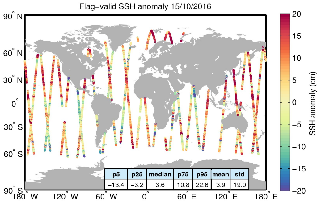
Figure 5. Geographical distribution of flag-valid 1-Hz SSH anomaly data over oceans and lakes for 15/10/2016. The statistical values shown in the table refer to the SSH anomaly in cm and are calculated over all measurements shown in the figure.
