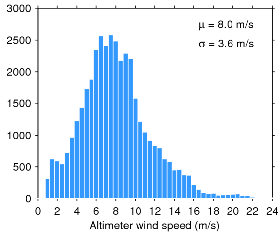
Figure 33. Histogram of flag-valid wind over oceans and lakes for 15/10/2016. The mean ( \mu ) and standard deviation ( \sigma ) are also shown. Note that values larger than 24 m/s are excluded from the histogram for the sake of readability but not from the computation of \mu and \sigma .
