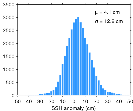
Figure 11. Histogram of science-valid SSH anomaly over oceans and lakes for 15/10/2016. The mean ( \mu ) and standard deviation ( \sigma ) are also shown. Note that values outside [-50 50] cm are excluded from the histogram for the sake of readability but not from the computation of \mu and \sigma .
