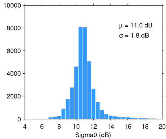
Figure 25. Histogram of flag-valid sigma0 over oceans and lakes for 15/10/2016. The mean ( \mu ) and standard deviation ( \sigma ) are also shown. Note that values outside [4 20] dB are excluded from the histogram for the sake of readability but not from the computation of \mu and \sigma .
