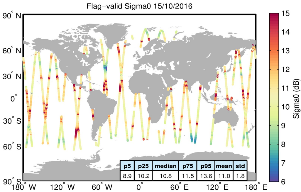
Figure 23. Geographical distribution of flag-valid sigma0 data over oceans and lakes for 15/10/2016. The statistical values shown in the table refer to the sigma0 in dB and are calculated over all measurements shown in the figure.
