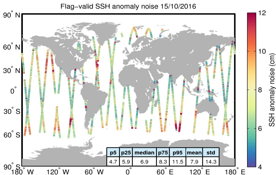
Figure 8. Geographical distribution of flag-valid 20-Hz SSH anomaly measurement noise over oceans and lakes for 15/10/2016. The statistical values shown in the table refer to the SSH anomaly noise and are calculated over all measurements shown in the figure.
