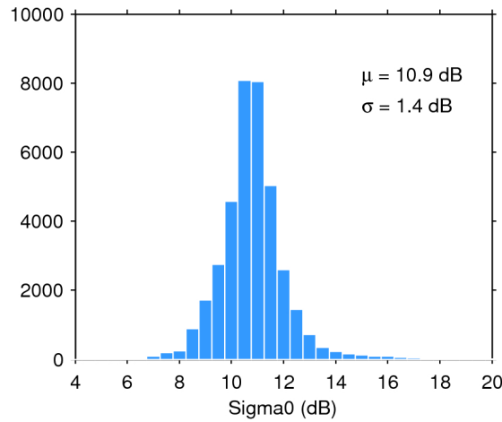
Figure 28. Histogram of science-valid sigma0 over oceans and lakes for 15/10/2016. The mean ( \mu ) and standard deviation ( \sigma ) are also shown. Note that values outside [4 20] dB are excluded from the histogram for the sake of readability but not from the computation of \mu and \sigma .
