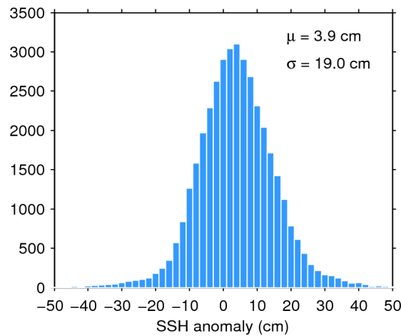
Figure 7. Histogram of flag-valid SSH anomaly over oceans and lakes for 15/10/2016. The mean ( \mu ) and standard deviation ( \sigma ) are also shown. Note that values outside [-50 50] cm are excluded from the histogram for the sake of readability but not from the computation of \mu and \sigma .
