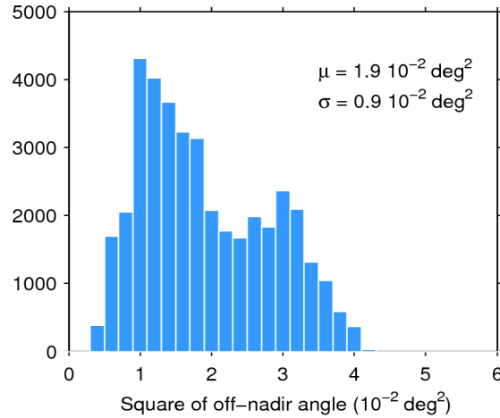
Figure 39. Histogram of flag-valid mispointing over oceans and lakes for 15/10/2016. The mean ( \mu ) and standard deviation ( \sigma ) are also shown. Note that values larger than 6 \cdot 10^{-2} \text{ deg}^2 are excluded from the histogram for the sake of readability but not from the computation of \mu and \sigma .
