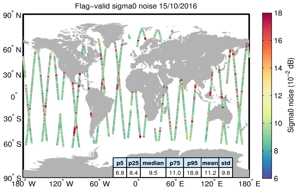
Figure 26. Geographical distribution of flag-valid 20-Hz sigma0 measurement noise over oceans and lakes for 15/10/2016. The statistical values shown in the table refer to the sigma0 noise and are calculated over all measurements shown in the figure.
