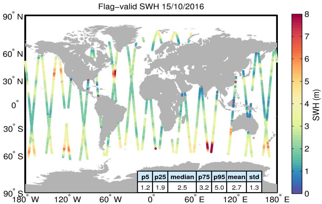
Figure 15. Geographical distribution of flag-valid SWH data over oceans and lakes for 15/10/2016. The statistical values shown in the table refer to the SWH in m and are calculated over all measurements shown in the figure.
