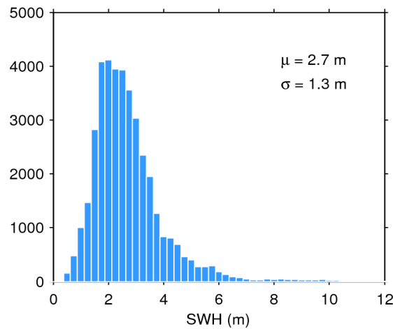
Figure 17. Histogram of flag-valid SWH over oceans and lakes for 15/10/2016. The mean ( \mu ) and standard deviation ( \sigma ) are also shown. Note that values larger than 12 m are excluded from the histogram for the sake of readability but not from the computation of \mu and \sigma .
