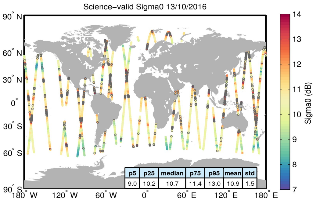
Figure 27. Geographical distribution of science-valid sigma0 data over oceans and lakes for 13/10/2016. The statistical values shown in the table refer to the sigma0 in dB and are calculated over all measurements shown in the figure. Gray circles denote records that have been rejected based on the editing criteria described in Table 4.
