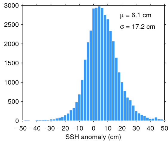
Figure 7. Histogram of flag-valid SSH anomaly over oceans and lakes for 13/10/2016. The mean ( \mu ) and standard deviation ( \sigma ) are also shown. Note that values outside [-50\ 50] cm are excluded from the histogram for the sake of readability but not from the computation of \mu and \sigma .
