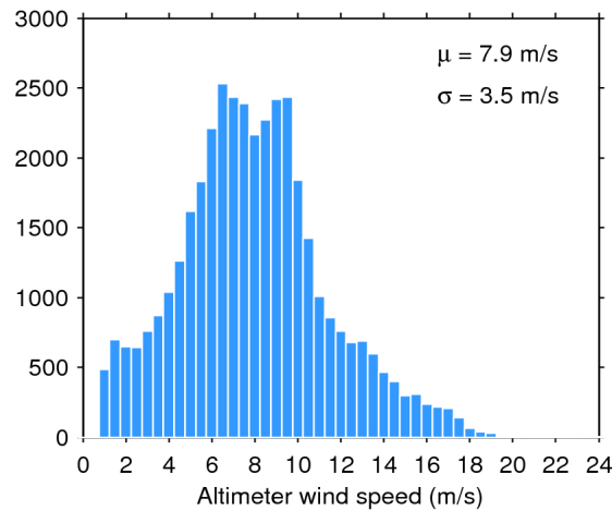
Figure 33. Histogram of flag-valid wind over oceans and lakes for 13/10/2016. The mean ( \mu ) and standard deviation ( \sigma ) are also shown. Note that values larger than 24 m/s are excluded from the histogram for the sake of readability but not from the computation of \mu and \sigma .
