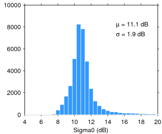
Figure 25. Histogram of flag-valid sigma0 over oceans and lakes for 13/10/2016. The mean ( \mu ) and standard deviation ( \sigma ) are also shown. Note that values outside [4 20] dB are excluded from the histogram for the sake of readability but not from the computation of \mu and \sigma .
