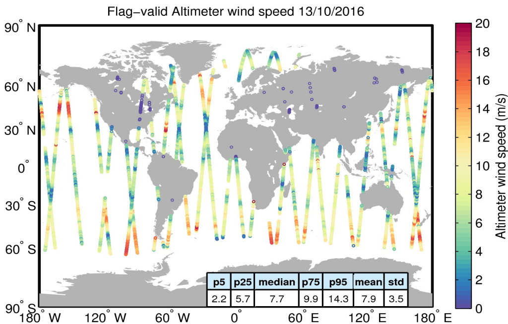
Figure 31. Geographical distribution of flag-valid wind data over oceans and lakes for 13/10/2016. The statistical values shown in the table refer to the wind in m/s and are calculated over all measurements shown in the figure.
