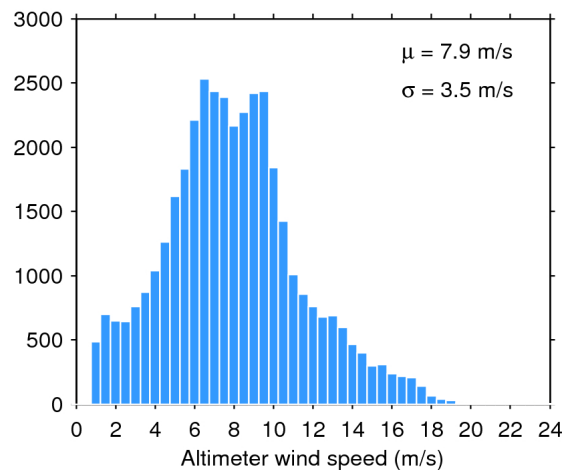
Figure 35. Histogram of science-valid wind over oceans and lakes for 13/10/2016. The mean ( \mu ) and standard deviation ( \sigma ) are also shown. Note that values larger than 24 m/s are excluded from the histogram for the sake of readability but not from the computation of \mu and \sigma .
