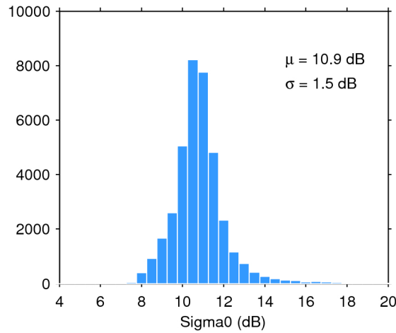
Figure 28. Histogram of science-valid sigma0 over oceans and lakes for 13/10/2016. The mean ( \mu ) and standard deviation ( \sigma ) are also shown. Note that values outside [4 20] dB are excluded from the histogram for the sake of readability but not from the computation of \mu and \sigma .
