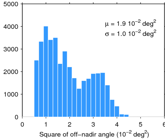
Figure 39. Histogram of flag-valid mispointing over oceans and lakes for 13/10/2016. The mean ( \mu ) and standard deviation ( \sigma ) are also shown. Note that values larger than 6 \cdot 10^{-2} \text{ deg}^2 are excluded from the histogram for the sake of readability but not from the computation of \mu and \sigma .
