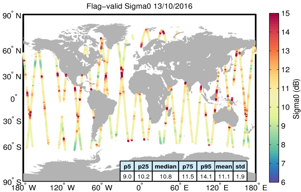
Figure 23. Geographical distribution of flag-valid sigma0 data over oceans and lakes for 13/10/2016. The statistical values shown in the table refer to the sigma0 in dB and are calculated over all measurements shown in the figure.
