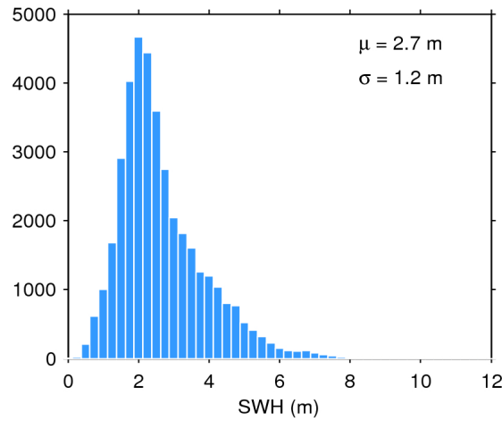
Figure 17. Histogram of flag-valid SWH over oceans and lakes for 13/10/2016. The mean ( \mu ) and standard deviation ( \sigma ) are also shown. Note that values larger than 12 m are excluded from the histogram for the sake of readability but not from the computation of \mu and \sigma .
