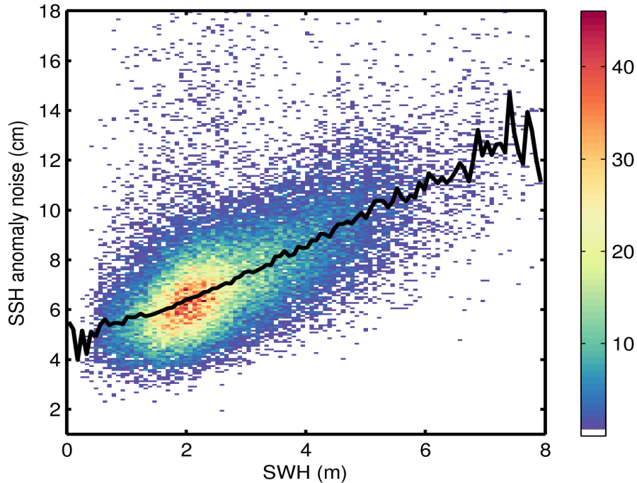
Figure 9. 2D histogram showing flag-valid SSH anomaly noise as a function of SWH for 13/10/2016. The black line denotes the median SSH anomaly noise as a function of SWH.
