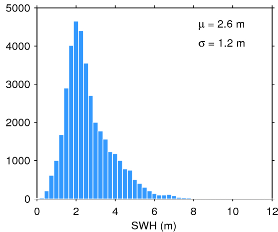
Figure 20. Histogram of science-valid SWH over oceans and lakes for 13/10/2016. The mean ( \mu ) and standard deviation ( \sigma ) are also shown. Note that values larger than 12 m are excluded from the histogram for the sake of readability but not from the computation of \mu and \sigma .
