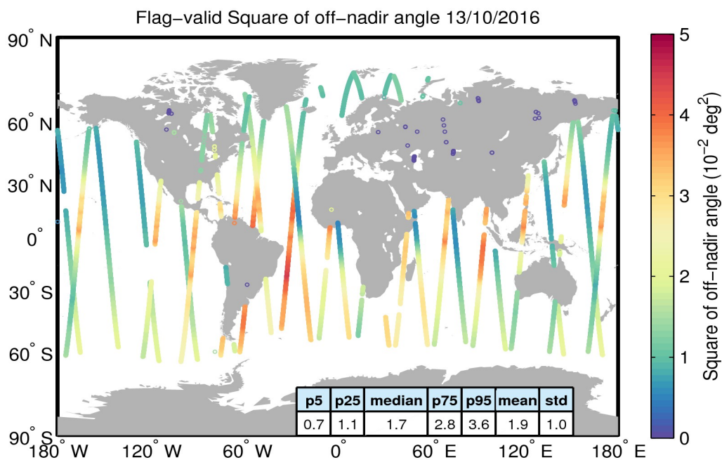
Figure 37. Geographical distribution of flag-valid mispointing data over oceans and lakes for 13/10/2016. The statistical values shown in the table refer to the mispointing in 10^{-2} deg 2 and are calculated over all measurements shown in the figure.
