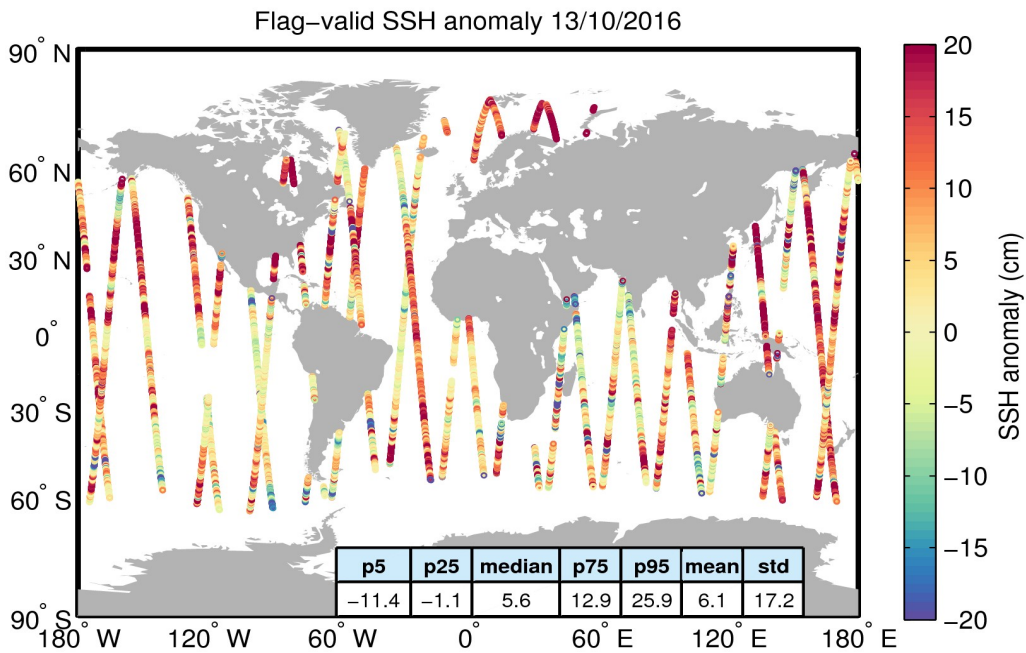
Figure 5. Geographical distribution of flag-valid 1-Hz SSH anomaly data over oceans and lakes for 13/10/2016. The statistical values shown in the table refer to the SSH anomaly in cm and are calculated over all measurements shown in the figure.
