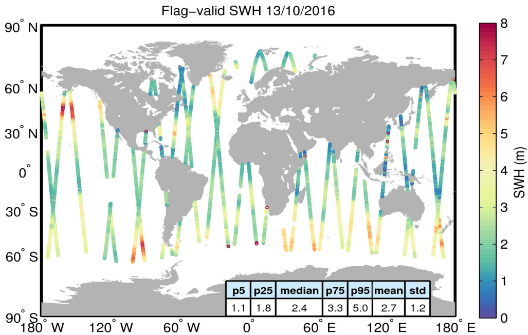
Figure 15. Geographical distribution of flag-valid SWH data over oceans and lakes for 13/10/2016. The statistical values shown in the table refer to the SWH in m and are calculated over all measurements shown in the figure.
