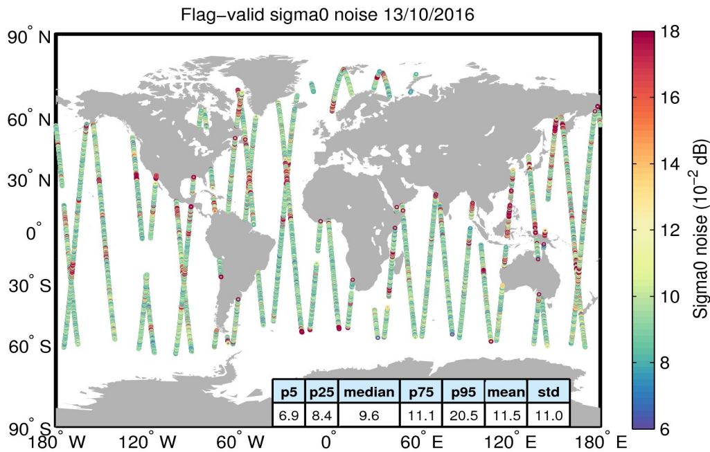
Figure 26. Geographical distribution of flag-valid 20-Hz sigma0 measurement noise over oceans and lakes for 13/10/2016. The statistical values shown in the table refer to the sigma0 noise and are calculated over all measurements shown in the figure.
