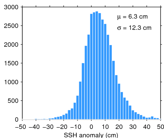
Figure 11. Histogram of science-valid SSH anomaly over oceans and lakes for 13/10/2016. The mean ( \mu ) and standard deviation ( \sigma ) are also shown. Note that values outside [-50 50] cm are excluded from the histogram for the sake of readability but not from the computation of \mu and \sigma .
