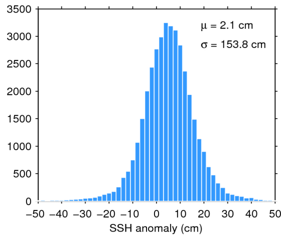
Figure 7. Histogram of flag-valid SSH anomaly over oceans and lakes for 12/10/2016. The mean ( \mu ) and standard deviation ( \sigma ) are also shown. Note that values outside [-50 50] cm are excluded from the histogram for the sake of readability but not from the computation of \mu and \sigma .
