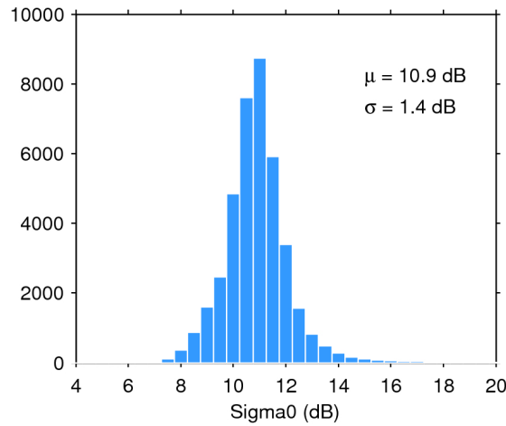
Figure 28. Histogram of science-valid sigma0 over oceans and lakes for 12/10/2016. The mean ( \mu ) and standard deviation ( \sigma ) are also shown. Note that values outside [4 20] dB are excluded from the histogram for the sake of readability but not from the computation of \mu and \sigma .
