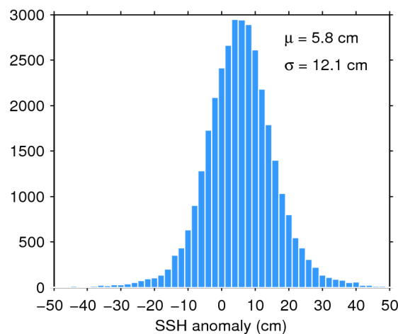
Figure 11. Histogram of science-valid SSH anomaly over oceans and lakes for 12/10/2016. The mean ( \mu ) and standard deviation ( \sigma ) are also shown. Note that values outside [-50 50] cm are excluded from the histogram for the sake of readability but not from the computation of \mu and \sigma .
