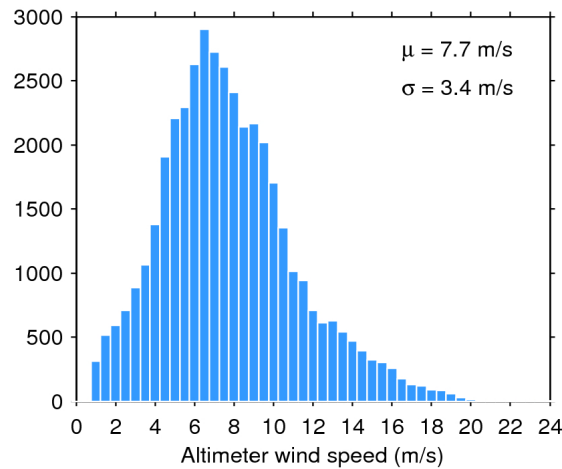
Figure 33. Histogram of flag-valid wind over oceans and lakes for 12/10/2016. The mean ( \mu ) and standard deviation ( \sigma ) are also shown. Note that values larger than 24 m/s are excluded from the histogram for the sake of readability but not from the computation of \mu and \sigma .
