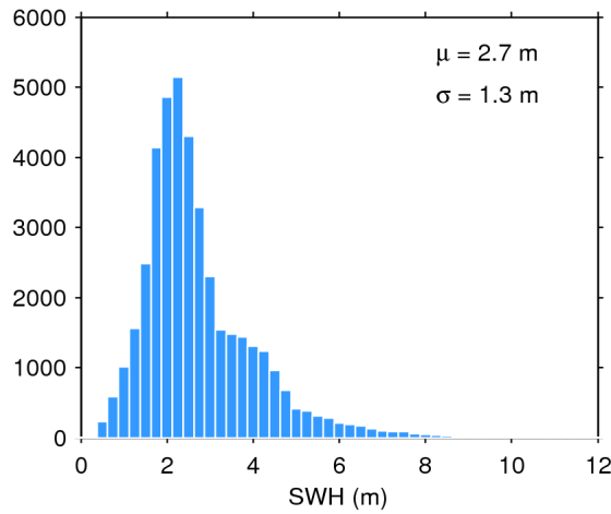
Figure 17. Histogram of flag-valid SWH over oceans and lakes for 12/10/2016. The mean ( \mu ) and standard deviation ( \sigma ) are also shown. Note that values larger than 12 m are excluded from the histogram for the sake of readability but not from the computation of \mu and \sigma .
