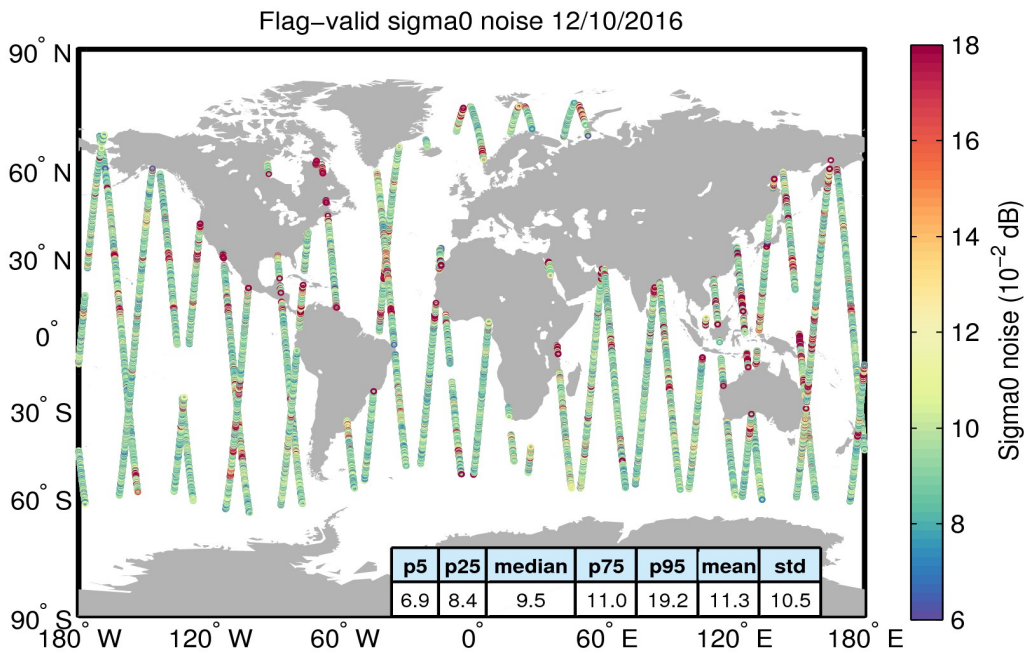
Figure 26. Geographical distribution of flag-valid 20-Hz sigma0 measurement noise over oceans and lakes for 12/10/2016. The statistical values shown in the table refer to the sigma0 noise and are calculated over all measurements shown in the figure.
