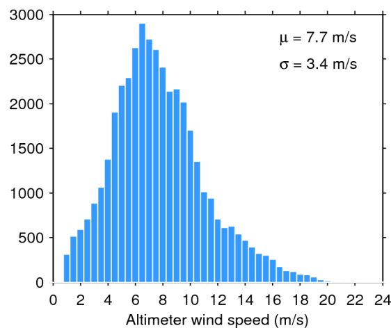
Figure 35. Histogram of science-valid wind over oceans and lakes for 12/10/2016. The mean ( \mu ) and standard deviation ( \sigma ) are also shown. Note that values larger than 24 m/s are excluded from the histogram for the sake of readability but not from the computation of \mu and \sigma .
