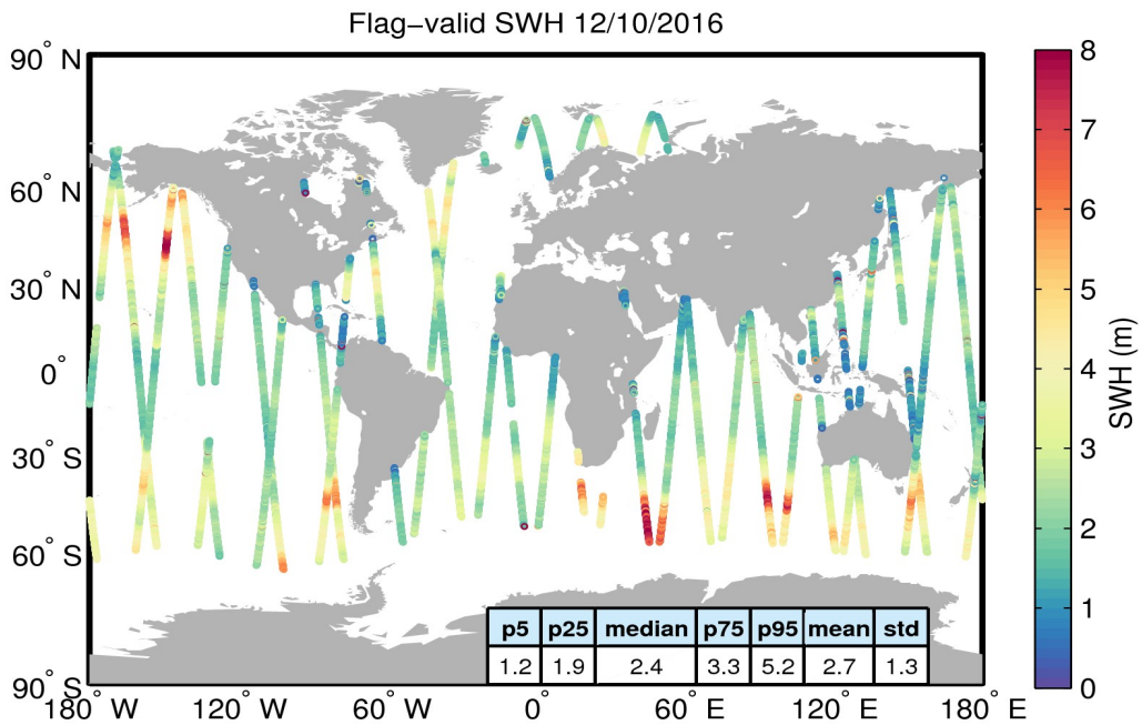
Figure 15. Geographical distribution of flag-valid SWH data over oceans and lakes for 12/10/2016. The statistical values shown in the table refer to the SWH in m and are calculated over all measurements shown in the figure.
