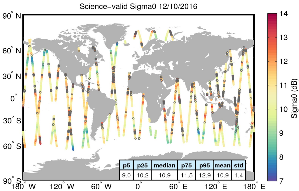
Figure 27. Geographical distribution of science-valid sigma0 data over oceans and lakes for 12/10/2016. The statistical values shown in the table refer to the sigma0 in dB and are calculated over all measurements shown in the figure. Gray circles denote records that have been rejected based on the editing criteria described in Table 4.
