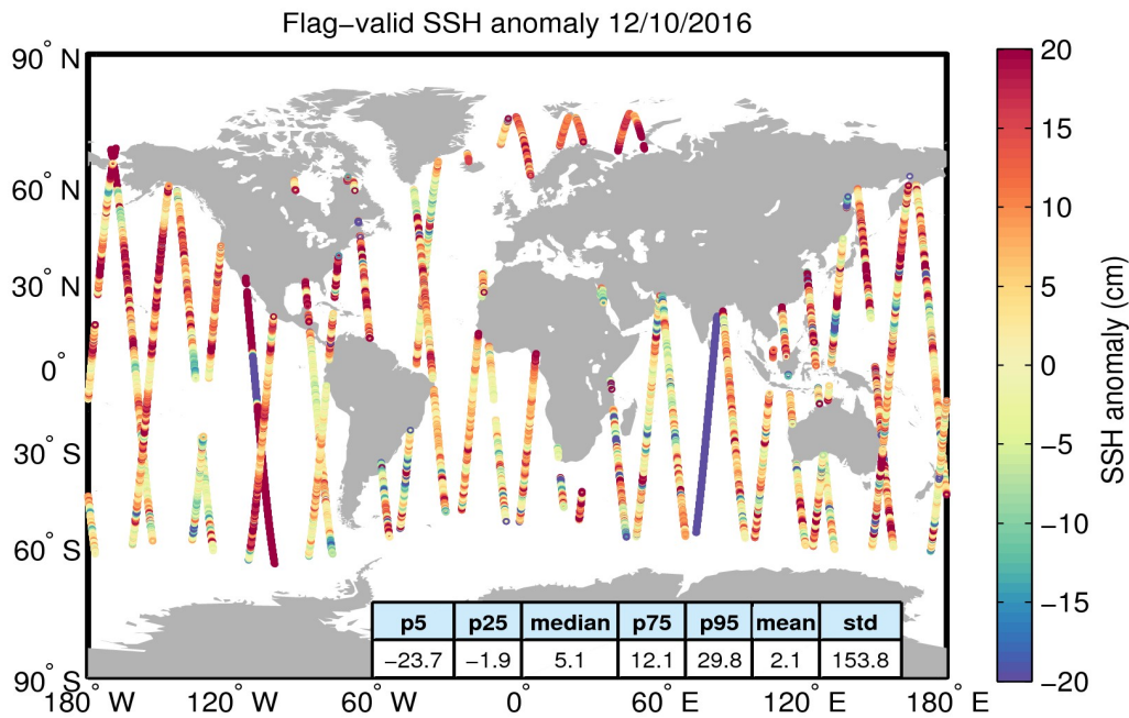
Figure 5. Geographical distribution of flag-valid 1-Hz SSH anomaly data over oceans and lakes for 12/10/2016. The statistical values shown in the table refer to the SSH anomaly in cm and are calculated over all measurements shown in the figure.
