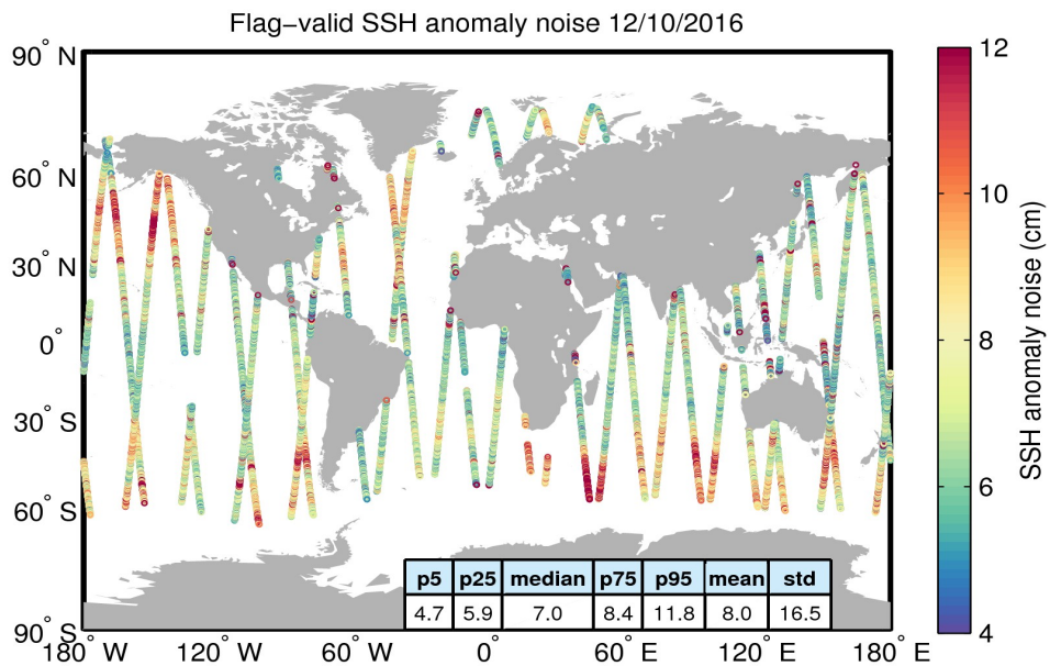
Figure 8. Geographical distribution of flag-valid 20-Hz SSH anomaly measurement noise over oceans and lakes for 12/10/2016. The statistical values shown in the table refer to the SSH anomaly noise and are calculated over all measurements shown in the figure.
