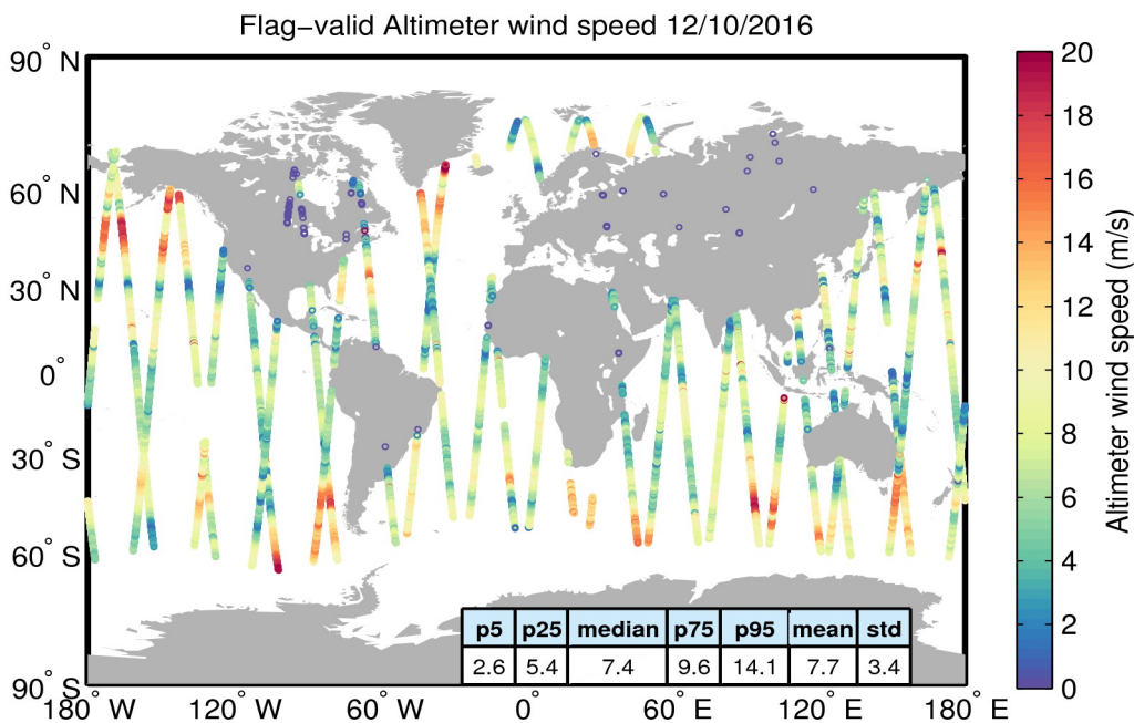
Figure 31. Geographical distribution of flag-valid wind data over oceans and lakes for 12/10/2016. The statistical values shown in the table refer to the wind in m/s and are calculated over all measurements shown in the figure.
