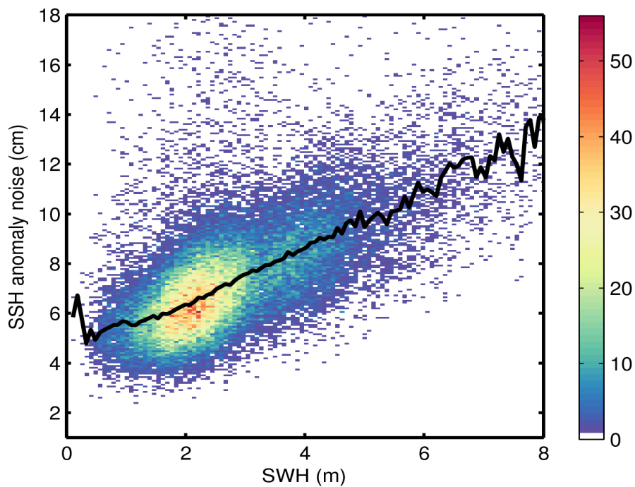
Figure 9. 2D histogram showing flag-valid SSH anomaly noise as a function of SWH for 12/10/2016. The black line denotes the median SSH anomaly noise as a function of SWH.
