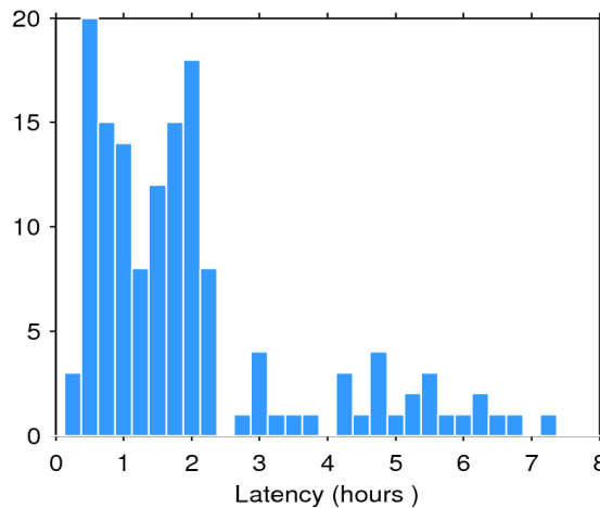
Figure 2. Histogram of the data latency for 12/10/2016. The y-axis denotes the number of files that are made available with a delay of x-hours with respect to the mean time of the records stored in the file.
