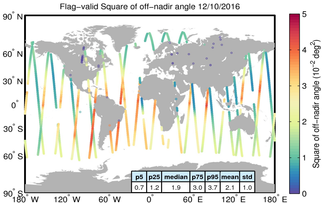
Figure 37. Geographical distribution of flag-valid mispointing data over oceans and lakes for 12/10/2016. The statistical values shown in the table refer to the mispointing in 10^{-2} deg 2 and are calculated over all measurements shown in the figure.
