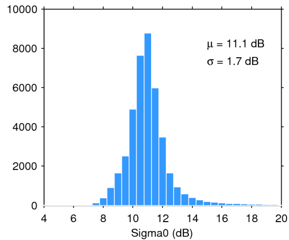
Figure 25. Histogram of flag-valid sigma0 over oceans and lakes for 12/10/2016. The mean ( \mu ) and standard deviation ( \sigma ) are also shown. Note that values outside [4 20] dB are excluded from the histogram for the sake of readability but not from the computation of \mu and \sigma .
