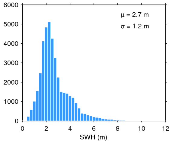
Figure 20. Histogram of science-valid SWH over oceans and lakes for 12/10/2016. The mean ( \mu ) and standard deviation ( \sigma ) are also shown. Note that values larger than 12 m are excluded from the histogram for the sake of readability but not from the computation of \mu and \sigma .
