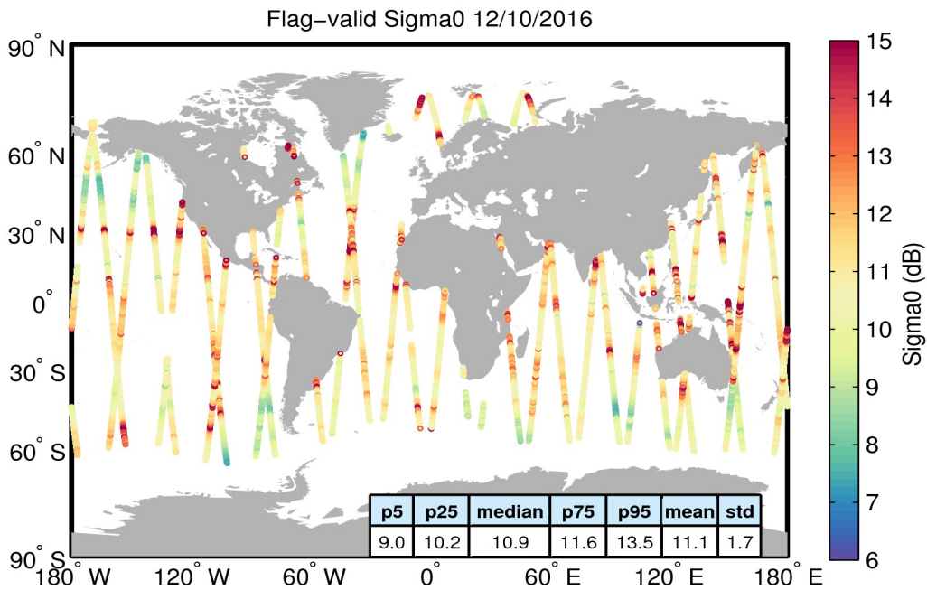
Figure 23. Geographical distribution of flag-valid sigma0 data over oceans and lakes for 12/10/2016. The statistical values shown in the table refer to the sigma0 in dB and are calculated over all measurements shown in the figure.
