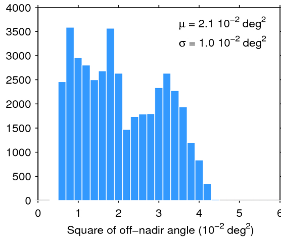
Figure 39. Histogram of flag-valid mispointing over oceans and lakes for 12/10/2016. The mean ( \mu ) and standard deviation ( \sigma ) are also shown. Note that values larger than 6 \cdot 10^{-2} \text{ deg}^2 are excluded from the histogram for the sake of readability but not from the computation of \mu and \sigma .
