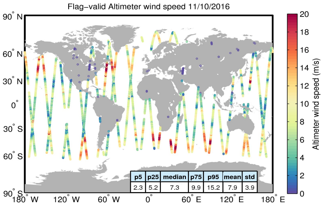
Figure 31. Geographical distribution of flag-valid wind data over oceans and lakes for 11/10/2016. The statistical values shown in the table refer to the wind in m/s and are calculated over all measurements shown in the figure.
