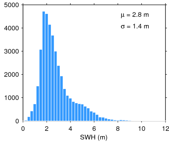
Figure 17. Histogram of flag-valid SWH over oceans and lakes for 11/10/2016. The mean ( \mu ) and standard deviation ( \sigma ) are also shown. Note that values larger than 12 m are excluded from the histogram for the sake of readability but not from the computation of \mu and \sigma .
