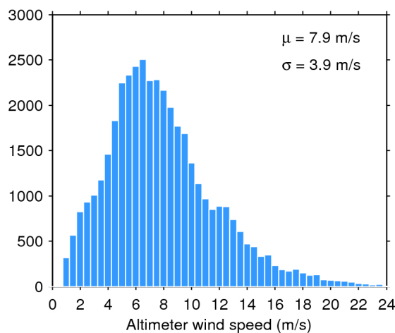
Figure 35. Histogram of science-valid wind over oceans and lakes for 11/10/2016. The mean ( \mu ) and standard deviation ( \sigma ) are also shown. Note that values larger than 24 m/s are excluded from the histogram for the sake of readability but not from the computation of \mu and \sigma .
