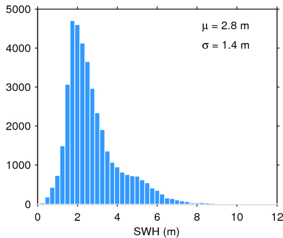
Figure 20. Histogram of science-valid SWH over oceans and lakes for 11/10/2016. The mean ( \mu ) and standard deviation ( \sigma ) are also shown. Note that values larger than 12 m are excluded from the histogram for the sake of readability but not from the computation of \mu and \sigma .
