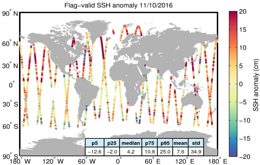
Figure 5. Geographical distribution of flag-valid 1-Hz SSH anomaly data over oceans and lakes for 11/10/2016. The statistical values shown in the table refer to the SSH anomaly in cm and are calculated over all measurements shown in the figure.
