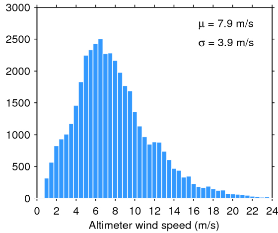
Figure 33. Histogram of flag-valid wind over oceans and lakes for 11/10/2016. The mean ( \mu ) and standard deviation ( \sigma ) are also shown. Note that values larger than 24 m/s are excluded from the histogram for the sake of readability but not from the computation of \mu and \sigma .
