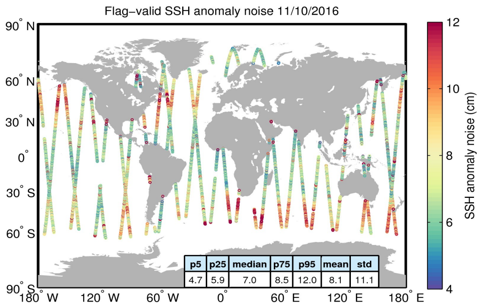
Figure 8. Geographical distribution of flag-valid 20-Hz SSH anomaly measurement noise over oceans and lakes for 11/10/2016. The statistical values shown in the table refer to the SSH anomaly noise and are calculated over all measurements shown in the figure.
