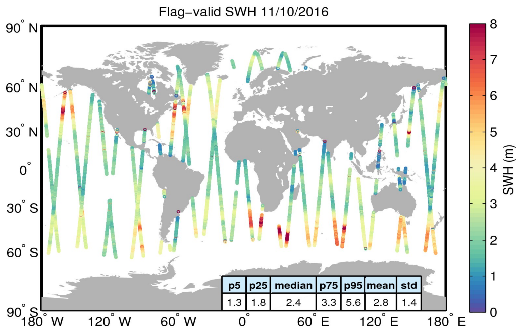
Figure 15. Geographical distribution of flag-valid SWH data over oceans and lakes for 11/10/2016. The statistical values shown in the table refer to the SWH in m and are calculated over all measurements shown in the figure.
