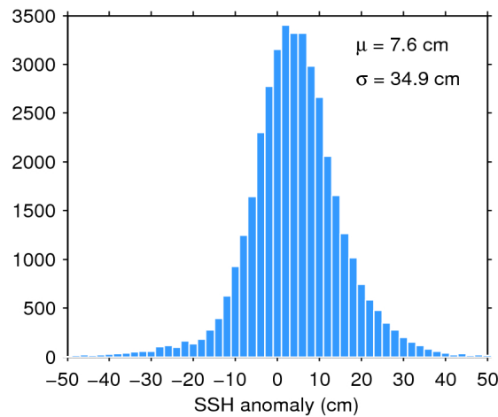
Figure 7. Histogram of flag-valid SSH anomaly over oceans and lakes for 11/10/2016. The mean ( \mu ) and standard deviation ( \sigma ) are also shown. Note that values outside [-50 50] cm are excluded from the histogram for the sake of readability but not from the computation of \mu and \sigma .
