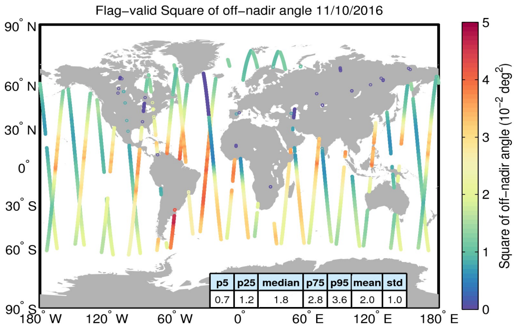
Figure 37. Geographical distribution of flag-valid mispointing data over oceans and lakes for 11/10/2016. The statistical values shown in the table refer to the mispointing in 10^{-2} deg 2 and are calculated over all measurements shown in the figure.
