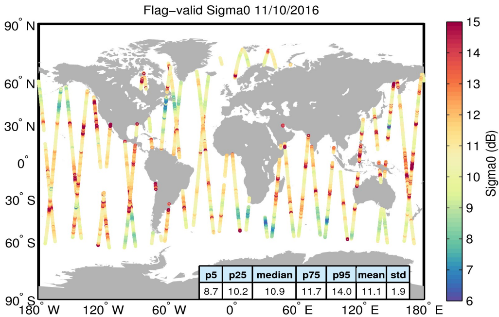
Figure 23. Geographical distribution of flag-valid sigma0 data over oceans and lakes for 11/10/2016. The statistical values shown in the table refer to the sigma0 in dB and are calculated over all measurements shown in the figure.
