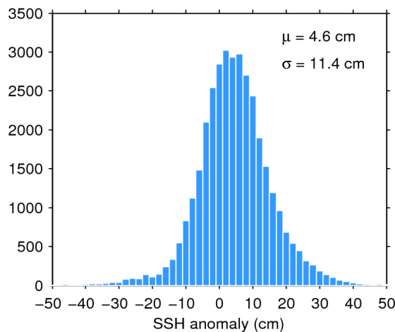
Figure 11. Histogram of science-valid SSH anomaly over oceans and lakes for 11/10/2016. The mean ( \mu ) and standard deviation ( \sigma ) are also shown. Note that values outside [-50 50] cm are excluded from the histogram for the sake of readability but not from the computation of \mu and \sigma .
