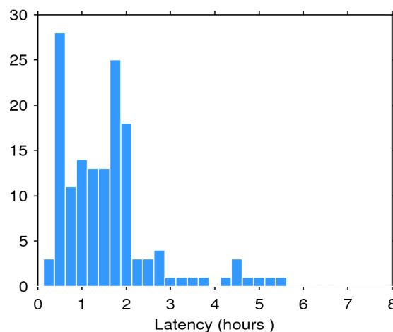
Figure 2. Histogram of the data latency for 11/10/2016. The y-axis denotes the number of files that are made available with a delay of x-hours with respect to the mean time of the records stored in the file.
