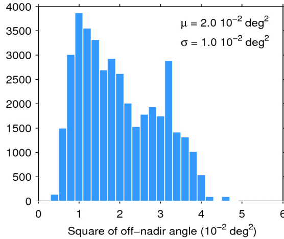
Figure 39. Histogram of flag-valid mispointing over oceans and lakes for 11/10/2016. The mean ( \mu ) and standard deviation ( \sigma ) are also shown. Note that values larger than 6 \cdot 10^{-2} \text{ deg}^2 are excluded from the histogram for the sake of readability but not from the computation of \mu and \sigma .
