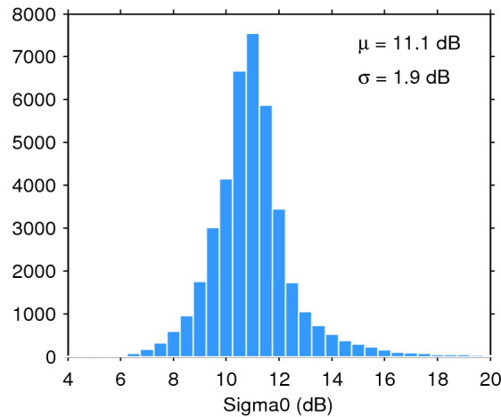
Figure 25. Histogram of flag-valid sigma0 over oceans and lakes for 11/10/2016. The mean ( \mu ) and standard deviation ( \sigma ) are also shown. Note that values outside [4 20] dB are excluded from the histogram for the sake of readability but not from the computation of \mu and \sigma .
