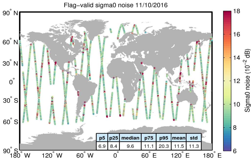
Figure 26. Geographical distribution of flag-valid 20-Hz sigma0 measurement noise over oceans and lakes for 11/10/2016. The statistical values shown in the table refer to the sigma0 noise and are calculated over all measurements shown in the figure.
