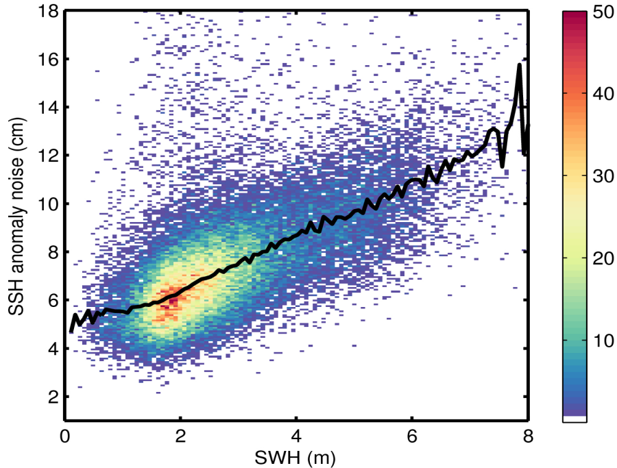
Figure 9. 2D histogram showing flag-valid SSH anomaly noise as a function of SWH for 11/10/2016. The black line denotes the median SSH anomaly noise as a function of SWH.
