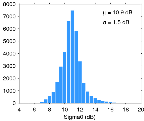
Figure 28. Histogram of science-valid sigma0 over oceans and lakes for 11/10/2016. The mean ( \mu ) and standard deviation ( \sigma ) are also shown. Note that values outside [4 20] dB are excluded from the histogram for the sake of readability but not from the computation of \mu and \sigma .
