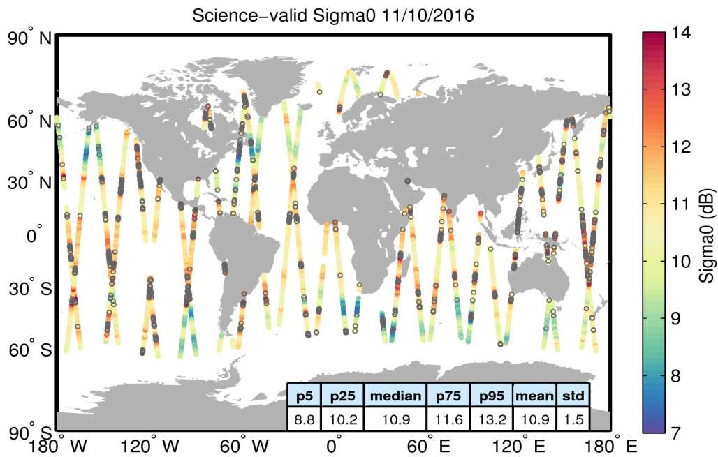
Figure 27. Geographical distribution of science-valid sigma0 data over oceans and lakes for 11/10/2016. The statistical values shown in the table refer to the sigma0 in dB and are calculated over all measurements shown in the figure. Gray circles denote records that have been rejected based on the editing criteria described in Table 4.
