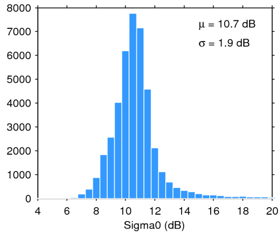
Figure 25. Histogram of flag-valid sigma0 over oceans and lakes for 10/10/2016. The mean ( \mu ) and standard deviation ( \sigma ) are also shown. Note that values outside [4 20] dB are excluded from the histogram for the sake of readability but not from the computation of \mu and \sigma .
