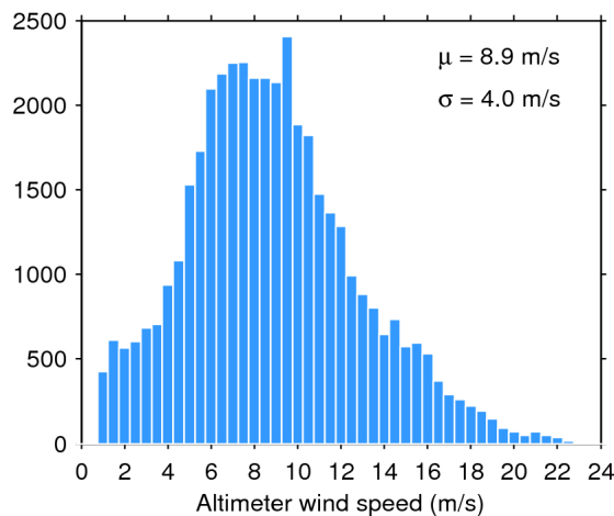
Figure 35. Histogram of science-valid wind over oceans and lakes for 10/10/2016. The mean ( \mu ) and standard deviation ( \sigma ) are also shown. Note that values larger than 24 m/s are excluded from the histogram for the sake of readability but not from the computation of \mu and \sigma .
