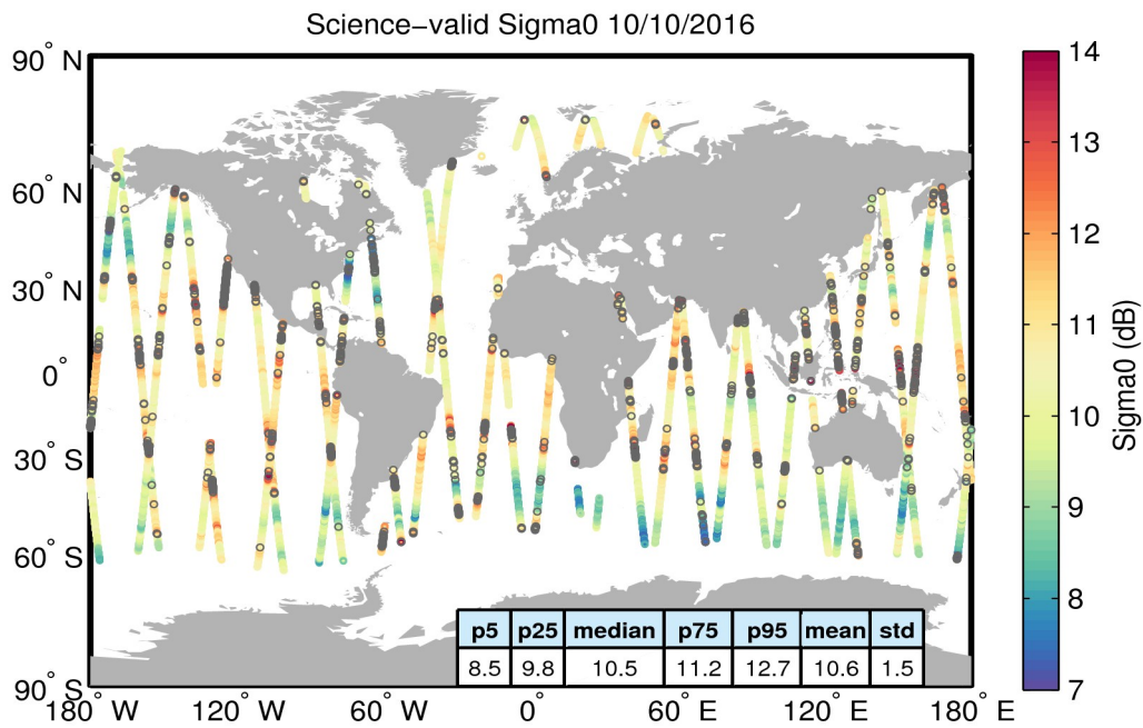
Figure 27. Geographical distribution of science-valid sigma0 data over oceans and lakes for 10/10/2016. The statistical values shown in the table refer to the sigma0 in dB and are calculated over all measurements shown in the figure. Gray circles denote records that have been rejected based on the editing criteria described in Table 4.
