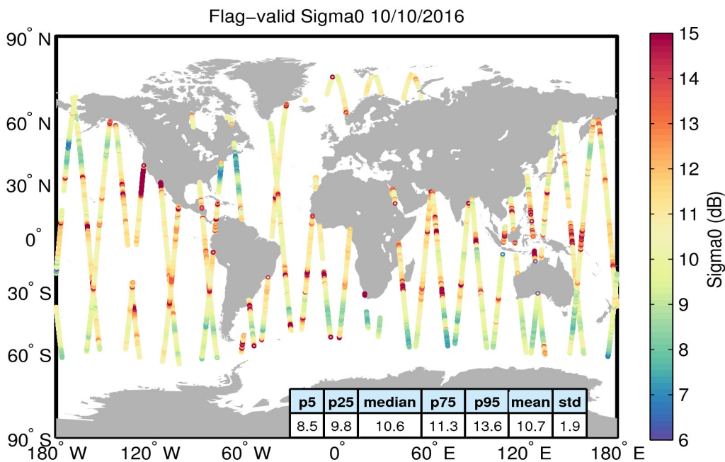
Figure 23. Geographical distribution of flag-valid sigma0 data over oceans and lakes for 10/10/2016. The statistical values shown in the table refer to the sigma0 in dB and are calculated over all measurements shown in the figure.
