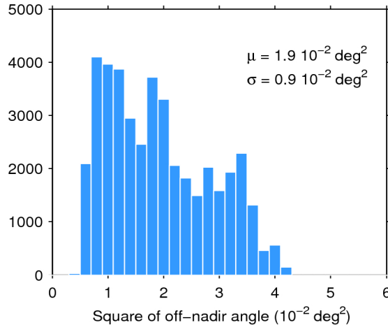
Figure 39. Histogram of flag-valid mispointing over oceans and lakes for 10/10/2016. The mean ( \mu ) and standard deviation ( \sigma ) are also shown. Note that values larger than 6 \cdot 10^{-2} \text{ deg}^2 are excluded from the histogram for the sake of readability but not from the computation of \mu and \sigma .
