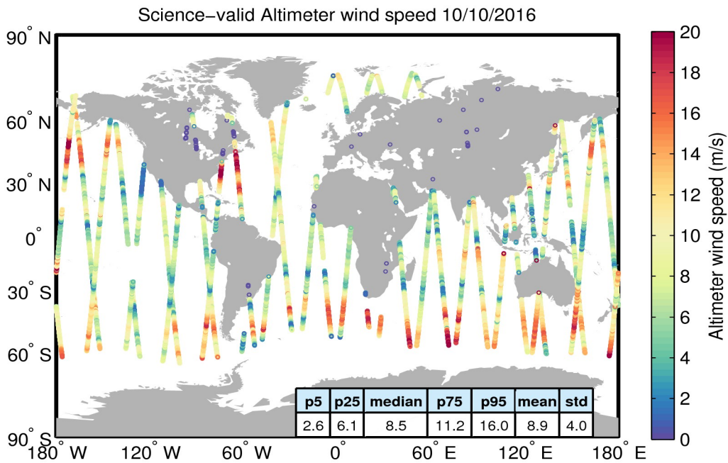
Figure 34. Geographical distribution of science-valid wind data over oceans and lakes for 10/10/2016. The statistical values shown in the table refer to the wind in m/s and are calculated over all measurements shown in the figure. Gray circles denote records that have been rejected based on the editing criteria described in Table 5.
