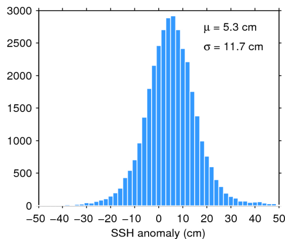
Figure 11. Histogram of science-valid SSH anomaly over oceans and lakes for 10/10/2016. The mean ( \mu ) and standard deviation ( \sigma ) are also shown. Note that values outside [-50 50] cm are excluded from the histogram for the sake of readability but not from the computation of \mu and \sigma .
