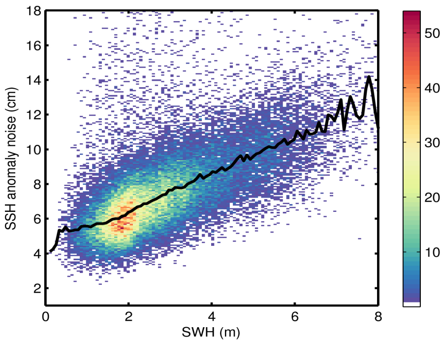
Figure 9. 2D histogram showing flag-valid SSH anomaly noise as a function of SWH for 10/10/2016. The black line denotes the median SSH anomaly noise as a function of SWH.
