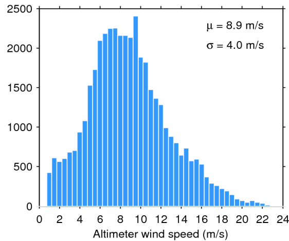
Figure 33. Histogram of flag-valid wind over oceans and lakes for 10/10/2016. The mean ( \mu ) and standard deviation ( \sigma ) are also shown. Note that values larger than 24 m/s are excluded from the histogram for the sake of readability but not from the computation of \mu and \sigma .
