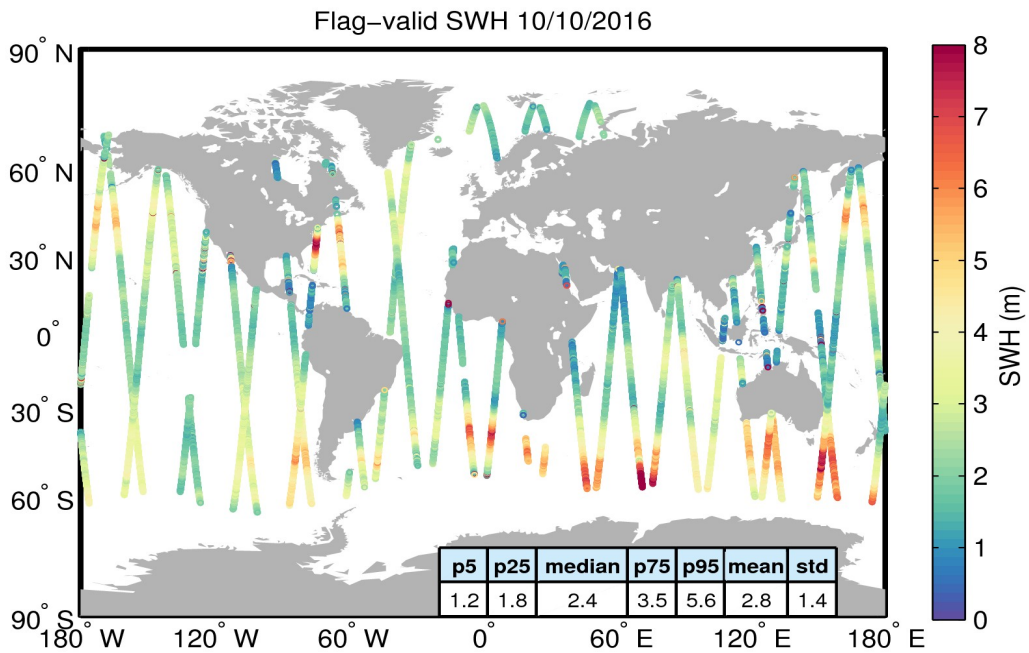
Figure 15. Geographical distribution of flag-valid SWH data over oceans and lakes for 10/10/2016. The statistical values shown in the table refer to the SWH in m and are calculated over all measurements shown in the figure.
