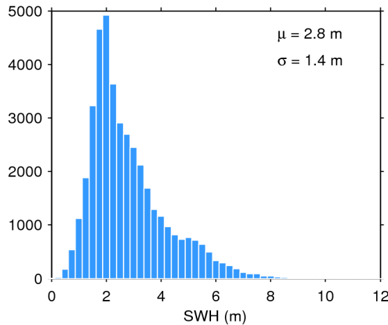
Figure 20. Histogram of science-valid SWH over oceans and lakes for 10/10/2016. The mean ( \mu ) and standard deviation ( \sigma ) are also shown. Note that values larger than 12 m are excluded from the histogram for the sake of readability but not from the computation of \mu and \sigma .
