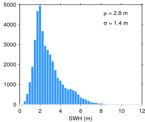
Figure 17. Histogram of flag-valid SWH over oceans and lakes for 10/10/2016. The mean ( \mu ) and standard deviation ( \sigma ) are also shown. Note that values larger than 12 m are excluded from the histogram for the sake of readability but not from the computation of \mu and \sigma .
