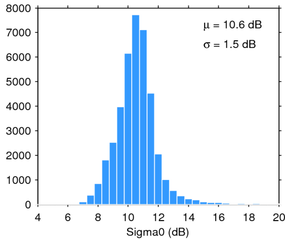
Figure 28. Histogram of science-valid sigma0 over oceans and lakes for 10/10/2016. The mean ( \mu ) and standard deviation ( \sigma ) are also shown. Note that values outside [4 20] dB are excluded from the histogram for the sake of readability but not from the computation of \mu and \sigma .
