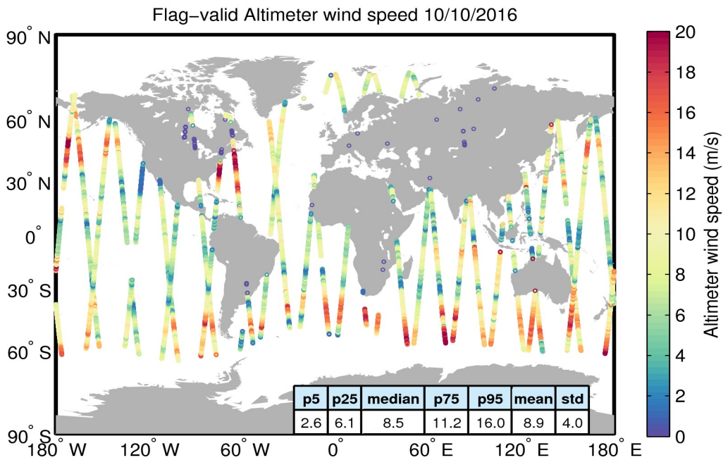
Figure 31. Geographical distribution of flag-valid wind data over oceans and lakes for 10/10/2016. The statistical values shown in the table refer to the wind in m/s and are calculated over all measurements shown in the figure.
