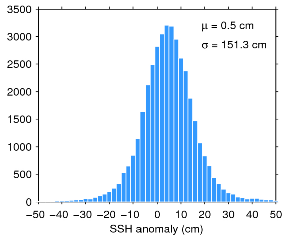
Figure 7. Histogram of flag-valid SSH anomaly over oceans and lakes for 10/10/2016. The mean ( \mu ) and standard deviation ( \sigma ) are also shown. Note that values outside [-50 50] cm are excluded from the histogram for the sake of readability but not from the computation of \mu and \sigma .
