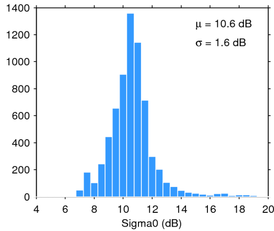
Figure 28. Histogram of science-valid sigma0 over oceans and lakes for 09/10/2016. The mean ( \mu ) and standard deviation ( \sigma ) are also shown. Note that values outside [4 20] dB are excluded from the histogram for the sake of readability but not from the computation of \mu and \sigma .
