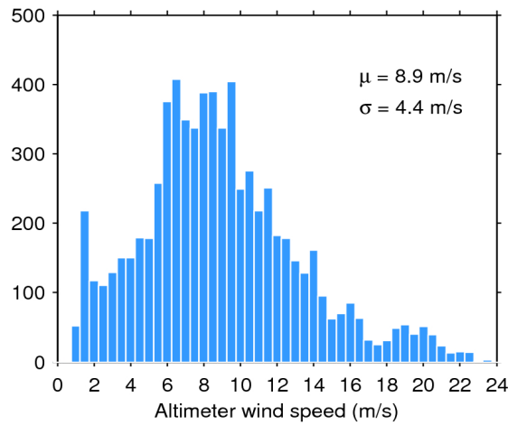
Figure 33. Histogram of flag-valid wind over oceans and lakes for 09/10/2016. The mean ( \mu ) and standard deviation ( \sigma ) are also shown. Note that values larger than 24 m/s are excluded from the histogram for the sake of readability but not from the computation of \mu and \sigma .
