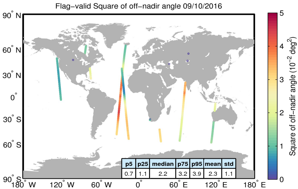
Figure 37. Geographical distribution of flag-valid mispointing data over oceans and lakes for 09/10/2016. The statistical values shown in the table refer to the mispointing in 10^{-2} deg 2 and are calculated over all measurements shown in the figure.
