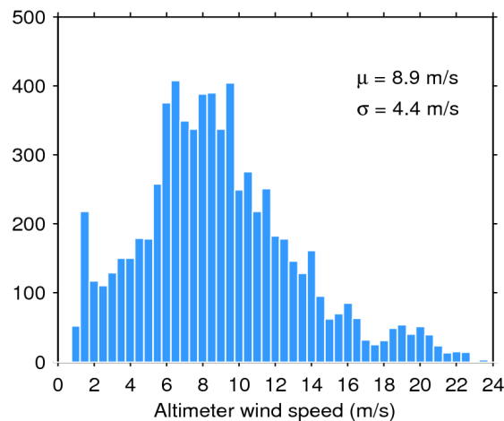
Figure 35. Histogram of science-valid wind over oceans and lakes for 09/10/2016. The mean ( \mu ) and standard deviation ( \sigma ) are also shown. Note that values larger than 24 m/s are excluded from the histogram for the sake of readability but not from the computation of \mu and \sigma .
