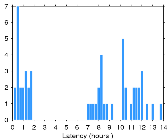
Figure 2. Histogram of the data latency for 09/10/2016. The y-axis denotes the number of files that are made available with a delay of x-hours with respect to the mean time of the records stored in the file.
