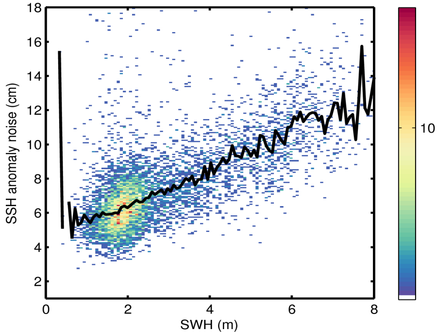
Figure 9. 2D histogram showing flag-valid SSH anomaly noise as a function of SWH for 09/10/2016. The black line denotes the median SSH anomaly noise as a function of SWH.
