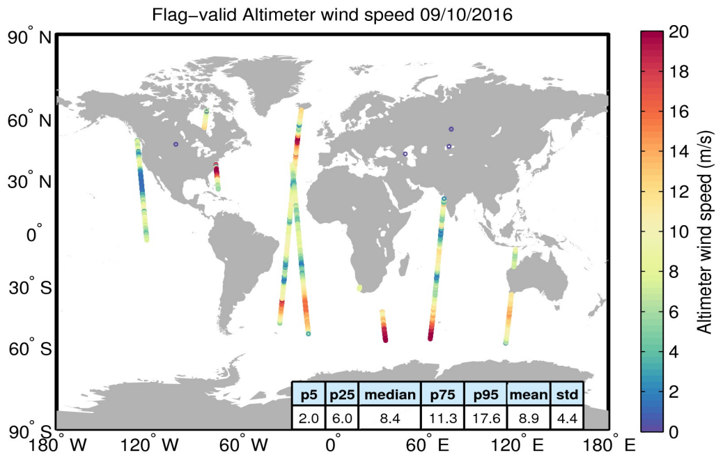
Figure 31. Geographical distribution of flag-valid wind data over oceans and lakes for 09/10/2016. The statistical values shown in the table refer to the wind in m/s and are calculated over all measurements shown in the figure.
