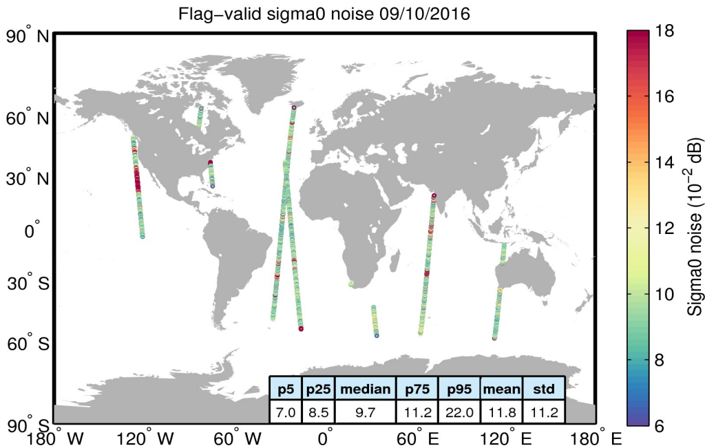
Figure 26. Geographical distribution of flag-valid 20-Hz sigma0 measurement noise over oceans and lakes for 09/10/2016. The statistical values shown in the table refer to the sigma0 noise and are calculated over all measurements shown in the figure.
