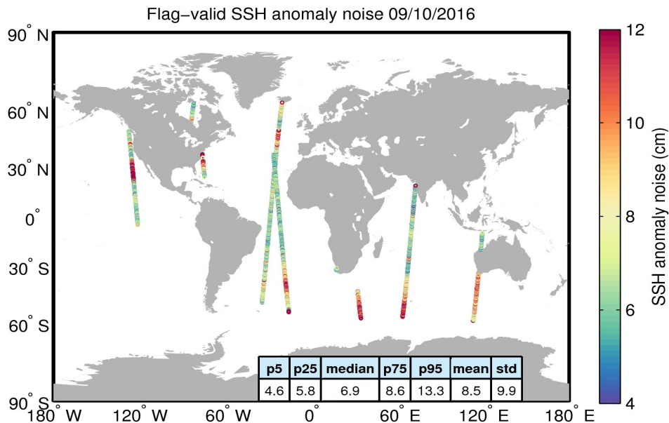
Figure 8. Geographical distribution of flag-valid 20-Hz SSH anomaly measurement noise over oceans and lakes for 09/10/2016. The statistical values shown in the table refer to the SSH anomaly noise and are calculated over all measurements shown in the figure.
