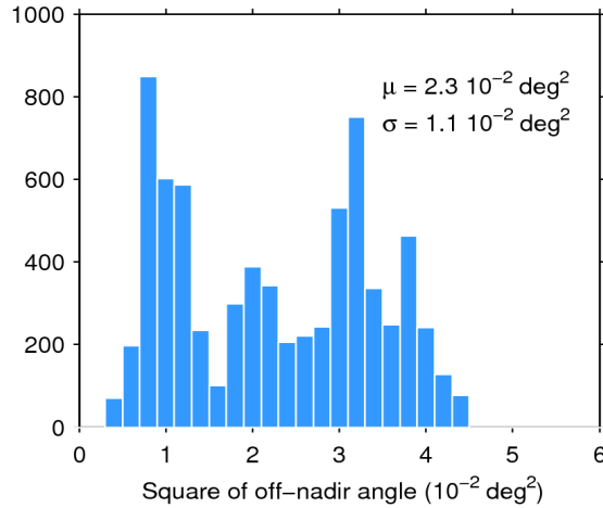
Figure 39. Histogram of flag-valid mispointing over oceans and lakes for 09/10/2016. The mean ( \mu ) and standard deviation ( \sigma ) are also shown. Note that values larger than 6 \cdot 10^{-2} \text{ deg}^2 are excluded from the histogram for the sake of readability but not from the computation of \mu and \sigma .
