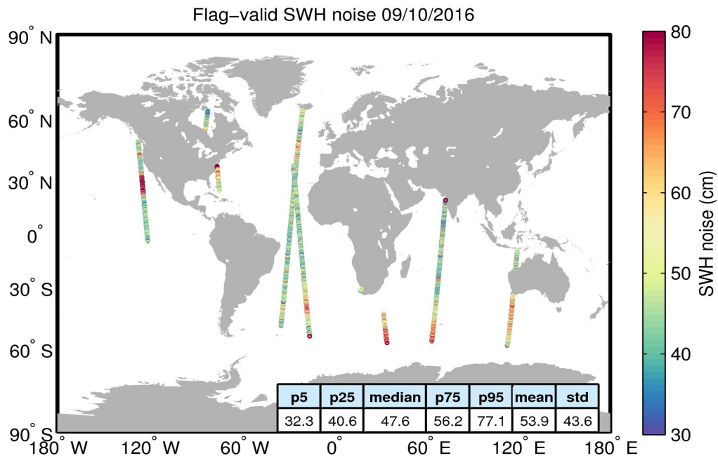
Figure 18. Geographical distribution of flag-valid 20-Hz SWH measurement noise over oceans and lakes for 09/10/2016. The statistical values shown in the table refer to the SWH noise and are calculated over all measurements shown in the figure.
