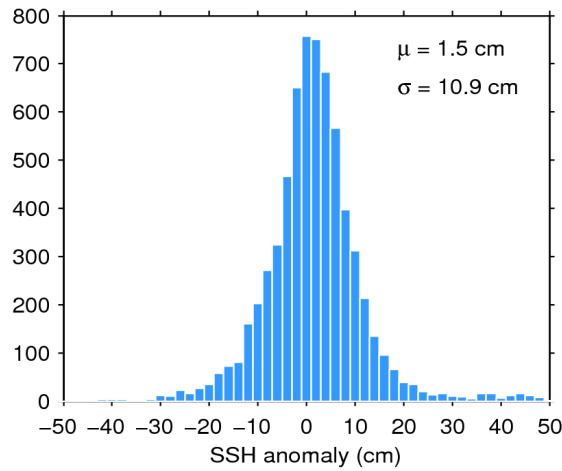
Figure 11. Histogram of science-valid SSH anomaly over oceans and lakes for 09/10/2016. The mean ( \mu ) and standard deviation ( \sigma ) are also shown. Note that values outside [-50 50] cm are excluded from the histogram for the sake of readability but not from the computation of \mu and \sigma .
