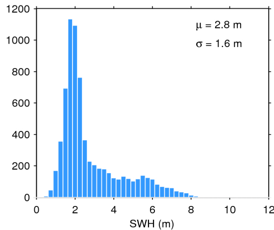
Figure 17. Histogram of flag-valid SWH over oceans and lakes for 09/10/2016. The mean ( \mu ) and standard deviation ( \sigma ) are also shown. Note that values larger than 12 m are excluded from the histogram for the sake of readability but not from the computation of \mu and \sigma .
