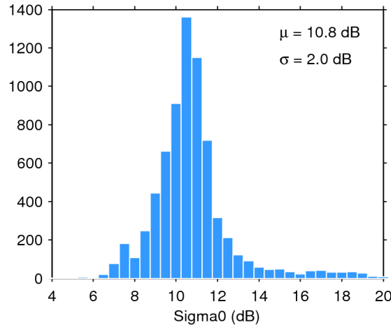
Figure 25. Histogram of flag-valid sigma0 over oceans and lakes for 09/10/2016. The mean ( \mu ) and standard deviation ( \sigma ) are also shown. Note that values outside [4 20] dB are excluded from the histogram for the sake of readability but not from the computation of \mu and \sigma .
