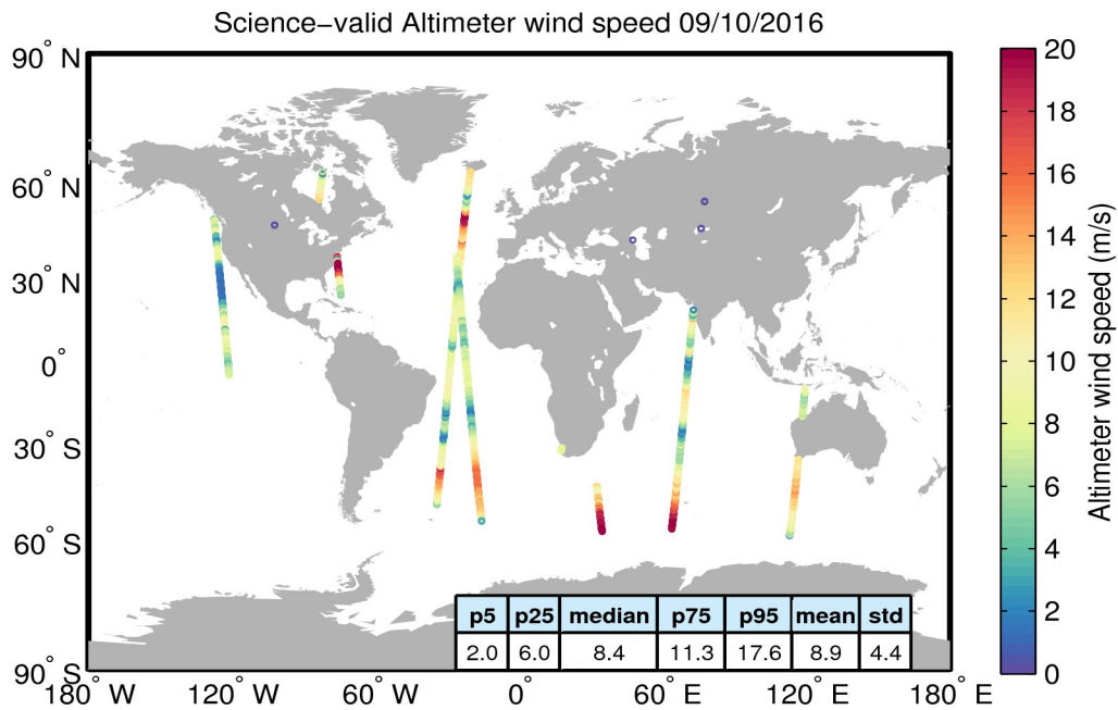
Figure 34. Geographical distribution of science-valid wind data over oceans and lakes for 09/10/2016. The statistical values shown in the table refer to the wind in m/s and are calculated over all measurements shown in the figure. Gray circles denote records that have been rejected based on the editing criteria described in Table 5.
