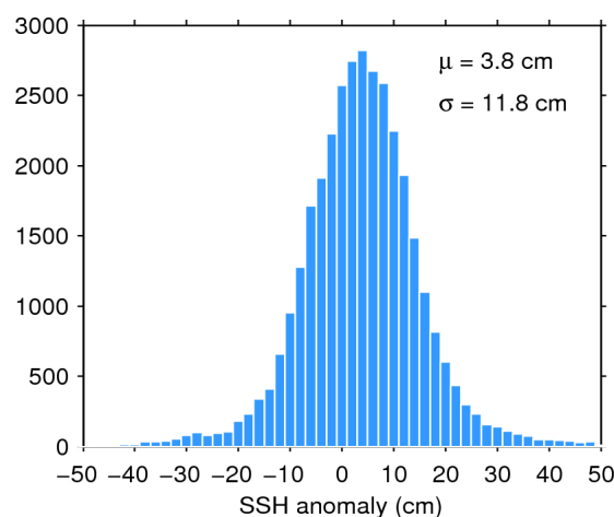
Figure 11. Histogram of science-valid SSH anomaly over oceans and lakes for 08/10/2016. The mean ( \mu ) and standard deviation ( \sigma ) are also shown. Note that values outside [-50 50] cm are excluded from the histogram for the sake of readability but not from the computation of \mu and \sigma .
