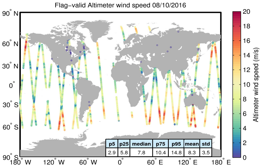
Figure 31. Geographical distribution of flag-valid wind data over oceans and lakes for 08/10/2016. The statistical values shown in the table refer to the wind in m/s and are calculated over all measurements shown in the figure.
