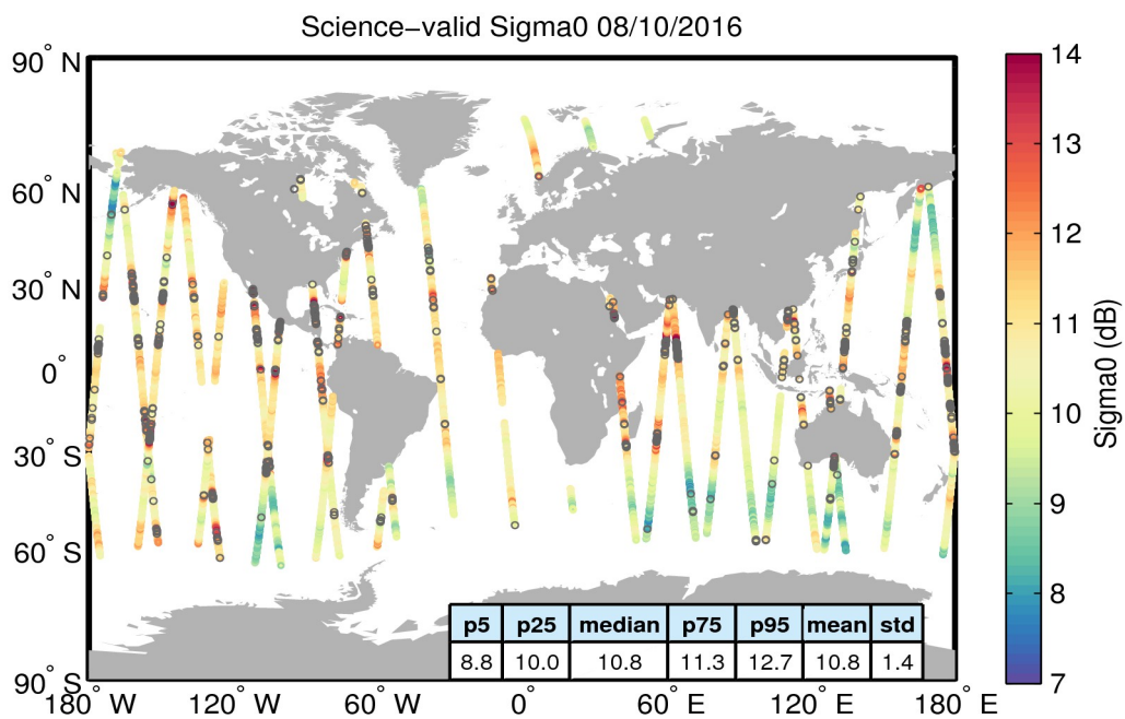
Figure 27. Geographical distribution of science-valid sigma0 data over oceans and lakes for 08/10/2016. The statistical values shown in the table refer to the sigma0 in dB and are calculated over all measurements shown in the figure. Gray circles denote records that have been rejected based on the editing criteria described in Table 4.
