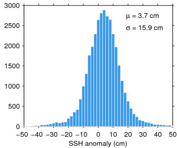
Figure 7. Histogram of flag-valid SSH anomaly over oceans and lakes for 08/10/2016. The mean ( \mu ) and standard deviation ( \sigma ) are also shown. Note that values outside [-50 50] cm are excluded from the histogram for the sake of readability but not from the computation of \mu and \sigma .
