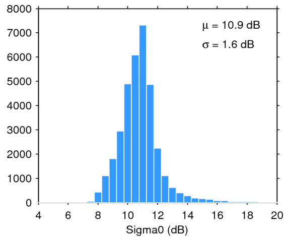
Figure 25. Histogram of flag-valid sigma0 over oceans and lakes for 08/10/2016. The mean ( \mu ) and standard deviation ( \sigma ) are also shown. Note that values outside [4 20] dB are excluded from the histogram for the sake of readability but not from the computation of \mu and \sigma .
