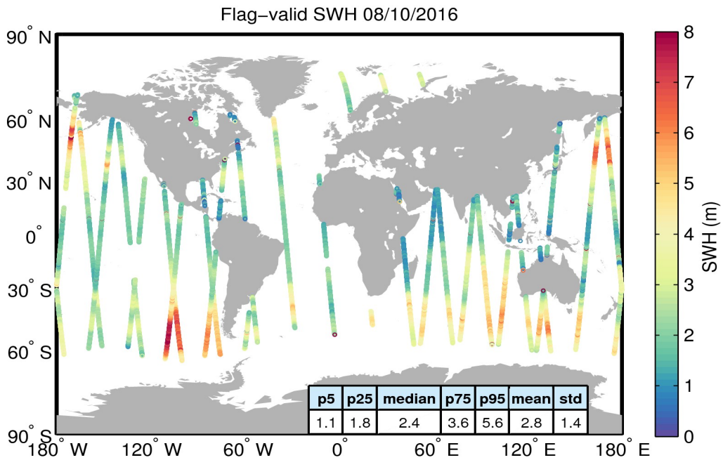
Figure 15. Geographical distribution of flag-valid SWH data over oceans and lakes for 08/10/2016. The statistical values shown in the table refer to the SWH in m and are calculated over all measurements shown in the figure.
