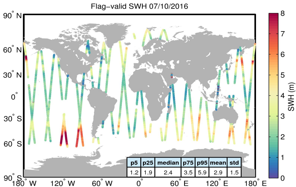
Figure 15. Geographical distribution of flag-valid SWH data over oceans and lakes for 07/10/2016. The statistical values shown in the table refer to the SWH in m and are calculated over all measurements shown in the figure.
