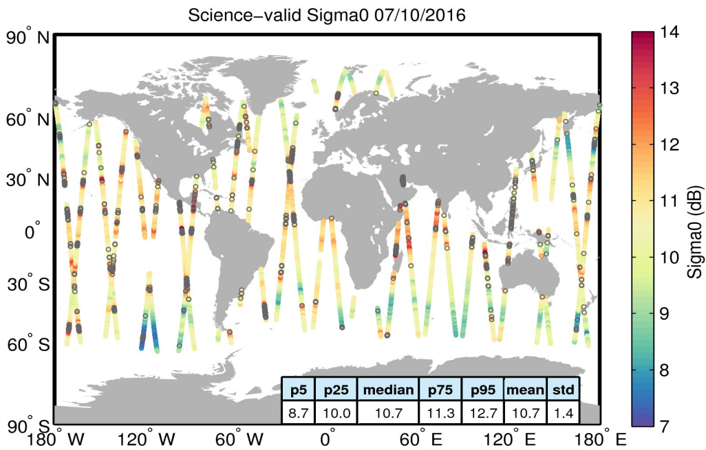
Figure 27. Geographical distribution of science-valid sigma0 data over oceans and lakes for 07/10/2016. The statistical values shown in the table refer to the sigma0 in dB and are calculated over all measurements shown in the figure. Gray circles denote records that have been rejected based on the editing criteria described in Table 4.
