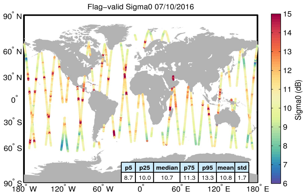
Figure 23. Geographical distribution of flag-valid sigma0 data over oceans and lakes for 07/10/2016. The statistical values shown in the table refer to the sigma0 in dB and are calculated over all measurements shown in the figure.
