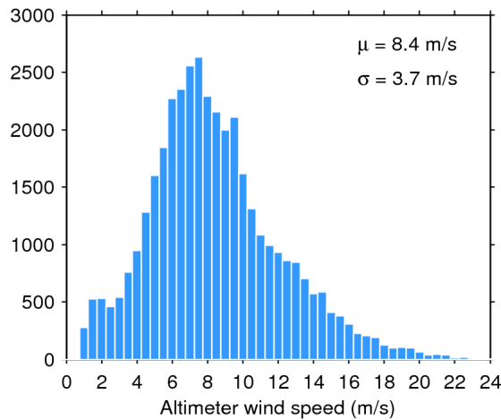
Figure 33. Histogram of flag-valid wind over oceans and lakes for 07/10/2016. The mean ( \mu ) and standard deviation ( \sigma ) are also shown. Note that values larger than 24 m/s are excluded from the histogram for the sake of readability but not from the computation of \mu and \sigma .
