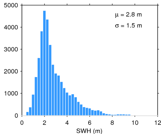
Figure 20. Histogram of science-valid SWH over oceans and lakes for 07/10/2016. The mean ( \mu ) and standard deviation ( \sigma ) are also shown. Note that values larger than 12 m are excluded from the histogram for the sake of readability but not from the computation of \mu and \sigma .
