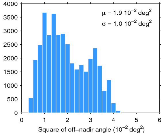
Figure 39. Histogram of flag-valid mispointing over oceans and lakes for 07/10/2016. The mean ( \mu ) and standard deviation ( \sigma ) are also shown. Note that values larger than 6 \cdot 10^{-2} \text{ deg}^2 are excluded from the histogram for the sake of readability but not from the computation of \mu and \sigma .
