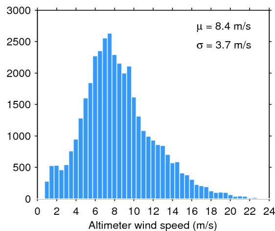
Figure 35. Histogram of science-valid wind over oceans and lakes for 07/10/2016. The mean ( \mu ) and standard deviation ( \sigma ) are also shown. Note that values larger than 24 m/s are excluded from the histogram for the sake of readability but not from the computation of \mu and \sigma .
