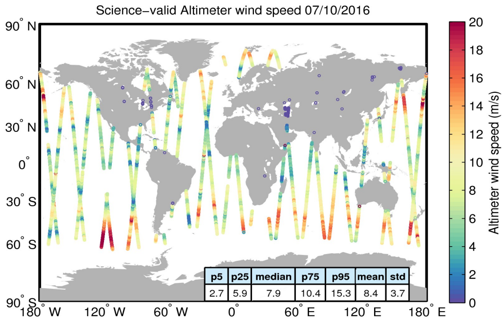
Figure 34. Geographical distribution of science-valid wind data over oceans and lakes for 07/10/2016. The statistical values shown in the table refer to the wind in m/s and are calculated over all measurements shown in the figure. Gray circles denote records that have been rejected based on the editing criteria described in Table 5.
