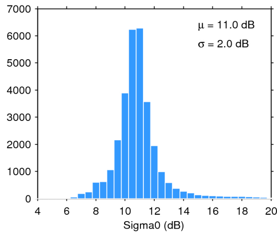
Figure 25. Histogram of flag-valid sigma0 over oceans and lakes for 06/10/2016. The mean ( \mu ) and standard deviation ( \sigma ) are also shown. Note that values outside [4 20] dB are excluded from the histogram for the sake of readability but not from the computation of \mu and \sigma .
