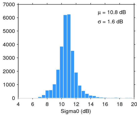
Figure 28. Histogram of science-valid sigma0 over oceans and lakes for 06/10/2016. The mean ( \mu ) and standard deviation ( \sigma ) are also shown. Note that values outside [4 20] dB are excluded from the histogram for the sake of readability but not from the computation of \mu and \sigma .
