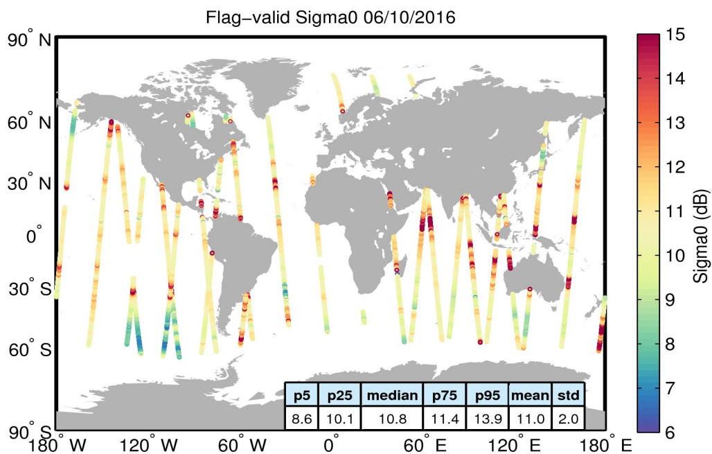
Figure 23. Geographical distribution of flag-valid sigma0 data over oceans and lakes for 06/10/2016. The statistical values shown in the table refer to the sigma0 in dB and are calculated over all measurements shown in the figure.
