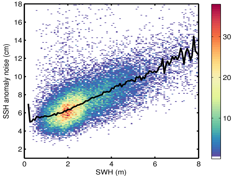
Figure 9. 2D histogram showing flag-valid SSH anomaly noise as a function of SWH for 06/10/2016. The black line denotes the median SSH anomaly noise as a function of SWH.
