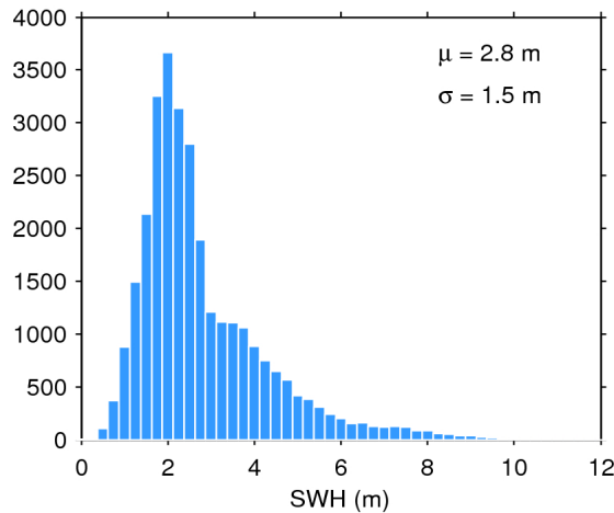
Figure 20. Histogram of science-valid SWH over oceans and lakes for 06/10/2016. The mean ( \mu ) and standard deviation ( \sigma ) are also shown. Note that values larger than 12 m are excluded from the histogram for the sake of readability but not from the computation of \mu and \sigma .
