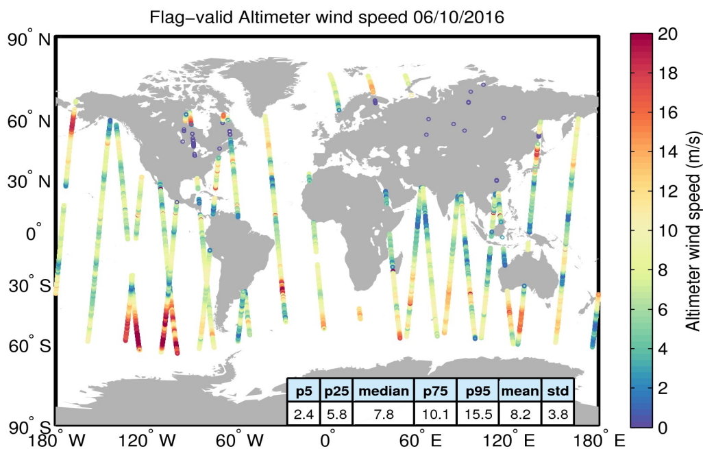
Figure 31. Geographical distribution of flag-valid wind data over oceans and lakes for 06/10/2016. The statistical values shown in the table refer to the wind in m/s and are calculated over all measurements shown in the figure.
