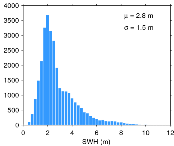
Figure 17. Histogram of flag-valid SWH over oceans and lakes for 06/10/2016. The mean ( \mu ) and standard deviation ( \sigma ) are also shown. Note that values larger than 12 m are excluded from the histogram for the sake of readability but not from the computation of \mu and \sigma .
