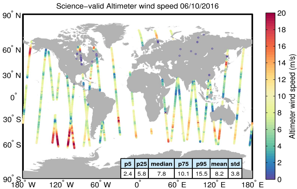
Figure 34. Geographical distribution of science-valid wind data over oceans and lakes for 06/10/2016. The statistical values shown in the table refer to the wind in m/s and are calculated over all measurements shown in the figure. Gray circles denote records that have been rejected based on the editing criteria described in Table 5.
