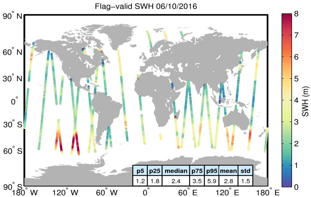
Figure 15. Geographical distribution of flag-valid SWH data over oceans and lakes for 06/10/2016. The statistical values shown in the table refer to the SWH in m and are calculated over all measurements shown in the figure.
