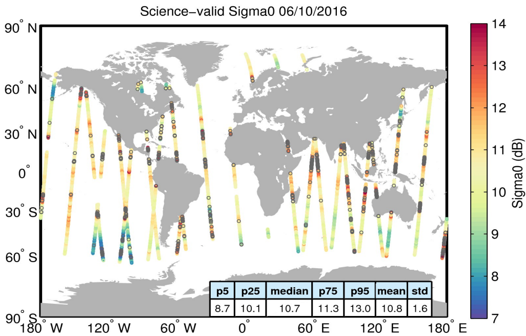
Figure 27. Geographical distribution of science-valid sigma0 data over oceans and lakes for 06/10/2016. The statistical values shown in the table refer to the sigma0 in dB and are calculated over all measurements shown in the figure. Gray circles denote records that have been rejected based on the editing criteria described in Table 4.
