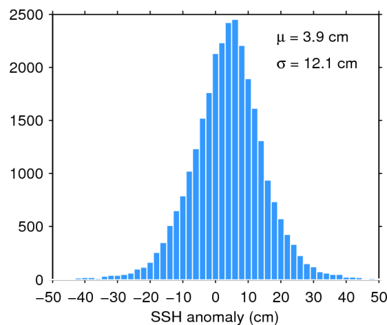
Figure 11. Histogram of science-valid SSH anomaly over oceans and lakes for 06/10/2016. The mean ( \mu ) and standard deviation ( \sigma ) are also shown. Note that values outside [-50 50] cm are excluded from the histogram for the sake of readability but not from the computation of \mu and \sigma .
