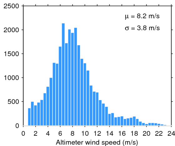
Figure 35. Histogram of science-valid wind over oceans and lakes for 06/10/2016. The mean ( \mu ) and standard deviation ( \sigma ) are also shown. Note that values larger than 24 m/s are excluded from the histogram for the sake of readability but not from the computation of \mu and \sigma .
