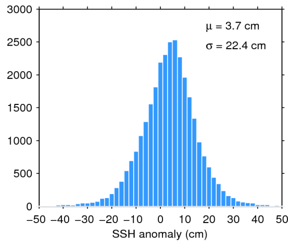
Figure 7. Histogram of flag-valid SSH anomaly over oceans and lakes for 06/10/2016. The mean ( \mu ) and standard deviation ( \sigma ) are also shown. Note that values outside [-50\ 50] cm are excluded from the histogram for the sake of readability but not from the computation of \mu and \sigma .
