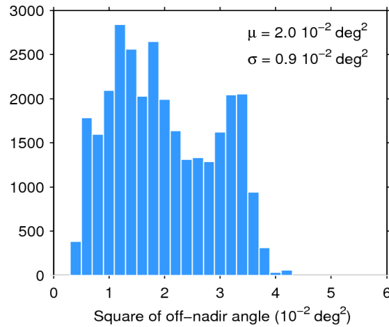
Figure 39. Histogram of flag-valid mispointing over oceans and lakes for 06/10/2016. The mean ( \mu ) and standard deviation ( \sigma ) are also shown. Note that values larger than 6 \cdot 10^{-2} \text{ deg}^2 are excluded from the histogram for the sake of readability but not from the computation of \mu and \sigma .
