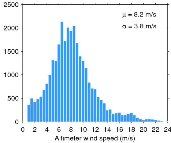
Figure 33. Histogram of flag-valid wind over oceans and lakes for 06/10/2016. The mean ( \mu ) and standard deviation ( \sigma ) are also shown. Note that values larger than 24 m/s are excluded from the histogram for the sake of readability but not from the computation of \mu and \sigma .
