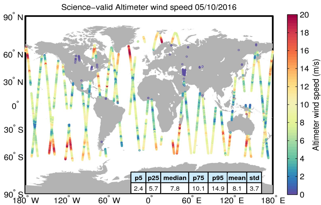
Figure 34. Geographical distribution of science-valid wind data over oceans and lakes for 05/10/2016. The statistical values shown in the table refer to the wind in m/s and are calculated over all measurements shown in the figure. Gray circles denote records that have been rejected based on the editing criteria described in Table 5.
