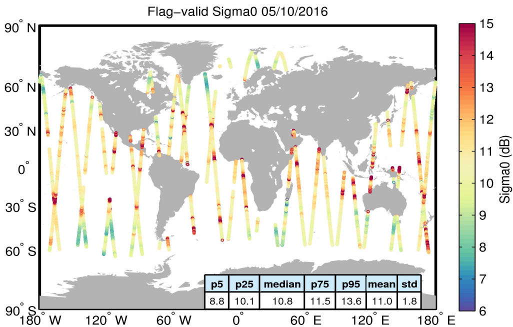
Figure 23. Geographical distribution of flag-valid sigma0 data over oceans and lakes for 05/10/2016. The statistical values shown in the table refer to the sigma0 in dB and are calculated over all measurements shown in the figure.
