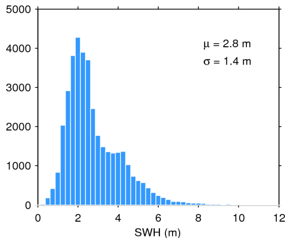
Figure 20. Histogram of science-valid SWH over oceans and lakes for 05/10/2016. The mean ( \mu ) and standard deviation ( \sigma ) are also shown. Note that values larger than 12 m are excluded from the histogram for the sake of readability but not from the computation of \mu and \sigma .
