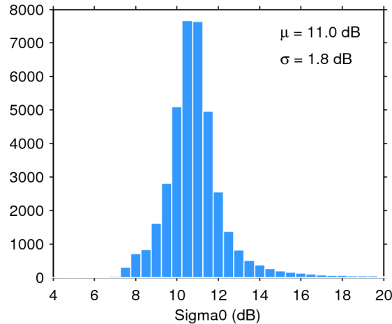
Figure 25. Histogram of flag-valid sigma0 over oceans and lakes for 05/10/2016. The mean ( \mu ) and standard deviation ( \sigma ) are also shown. Note that values outside [4 20] dB are excluded from the histogram for the sake of readability but not from the computation of \mu and \sigma .
