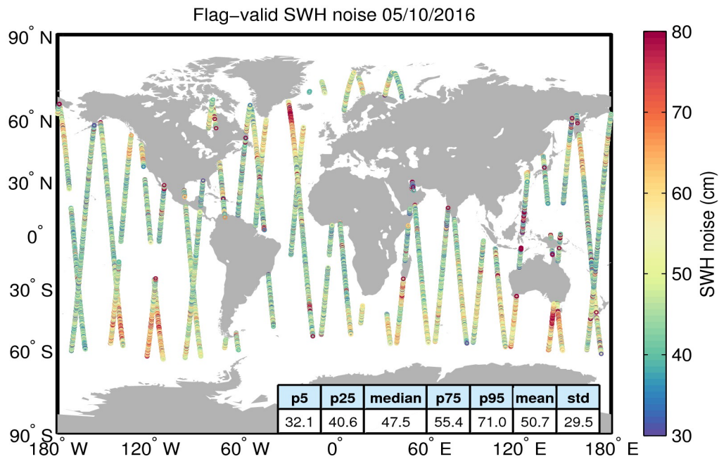
Figure 18. Geographical distribution of flag-valid 20-Hz SWH measurement noise over oceans and lakes for 05/10/2016. The statistical values shown in the table refer to the SWH noise and are calculated over all measurements shown in the figure.
