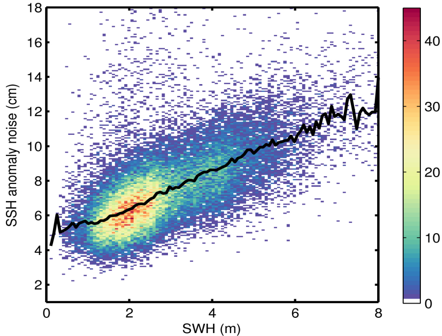
Figure 9. 2D histogram showing flag-valid SSH anomaly noise as a function of SWH for 05/10/2016. The black line denotes the median SSH anomaly noise as a function of SWH.
