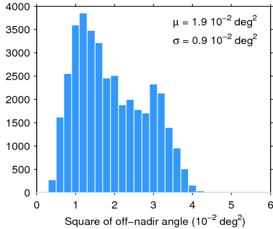
Figure 39. Histogram of flag-valid mispointing over oceans and lakes for 05/10/2016. The mean ( \mu ) and standard deviation ( \sigma ) are also shown. Note that values larger than 6 \cdot 10^{-2} \text{ deg}^2 are excluded from the histogram for the sake of readability but not from the computation of \mu and \sigma .
