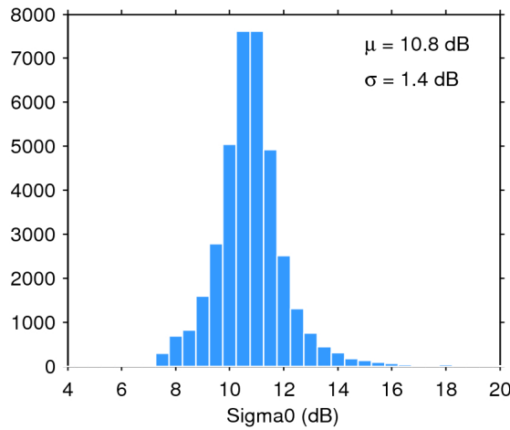
Figure 28. Histogram of science-valid sigma0 over oceans and lakes for 05/10/2016. The mean ( \mu ) and standard deviation ( \sigma ) are also shown. Note that values outside [4 20] dB are excluded from the histogram for the sake of readability but not from the computation of \mu and \sigma .
