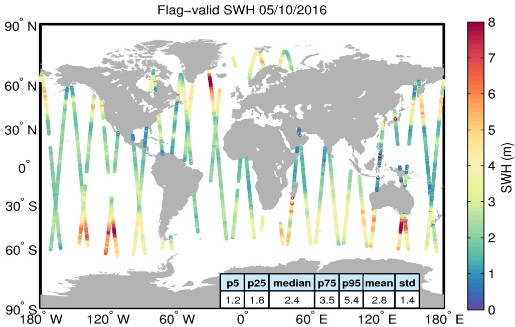
Figure 15. Geographical distribution of flag-valid SWH data over oceans and lakes for 05/10/2016. The statistical values shown in the table refer to the SWH in m and are calculated over all measurements shown in the figure.
