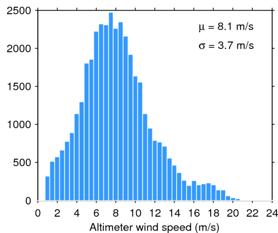
Figure 35. Histogram of science-valid wind over oceans and lakes for 05/10/2016. The mean ( \mu ) and standard deviation ( \sigma ) are also shown. Note that values larger than 24 m/s are excluded from the histogram for the sake of readability but not from the computation of \mu and \sigma .
