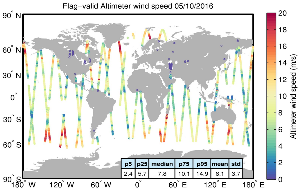
Figure 31. Geographical distribution of flag-valid wind data over oceans and lakes for 05/10/2016. The statistical values shown in the table refer to the wind in m/s and are calculated over all measurements shown in the figure.
