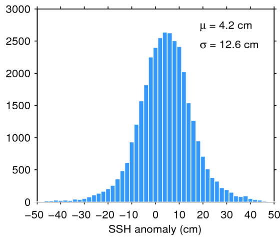
Figure 11. Histogram of science-valid SSH anomaly over oceans and lakes for 05/10/2016. The mean ( \mu ) and standard deviation ( \sigma ) are also shown. Note that values outside [-50 50] cm are excluded from the histogram for the sake of readability but not from the computation of \mu and \sigma .
