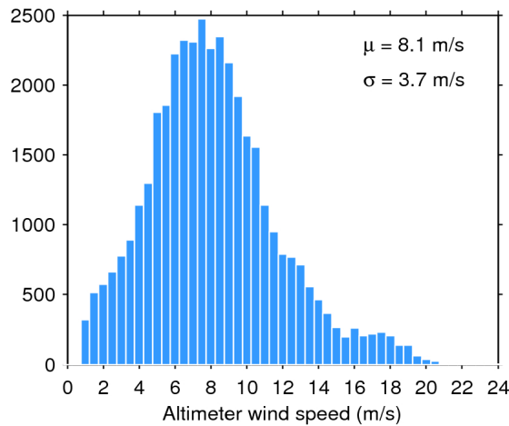
Figure 33. Histogram of flag-valid wind over oceans and lakes for 05/10/2016. The mean ( \mu ) and standard deviation ( \sigma ) are also shown. Note that values larger than 24 m/s are excluded from the histogram for the sake of readability but not from the computation of \mu and \sigma .
