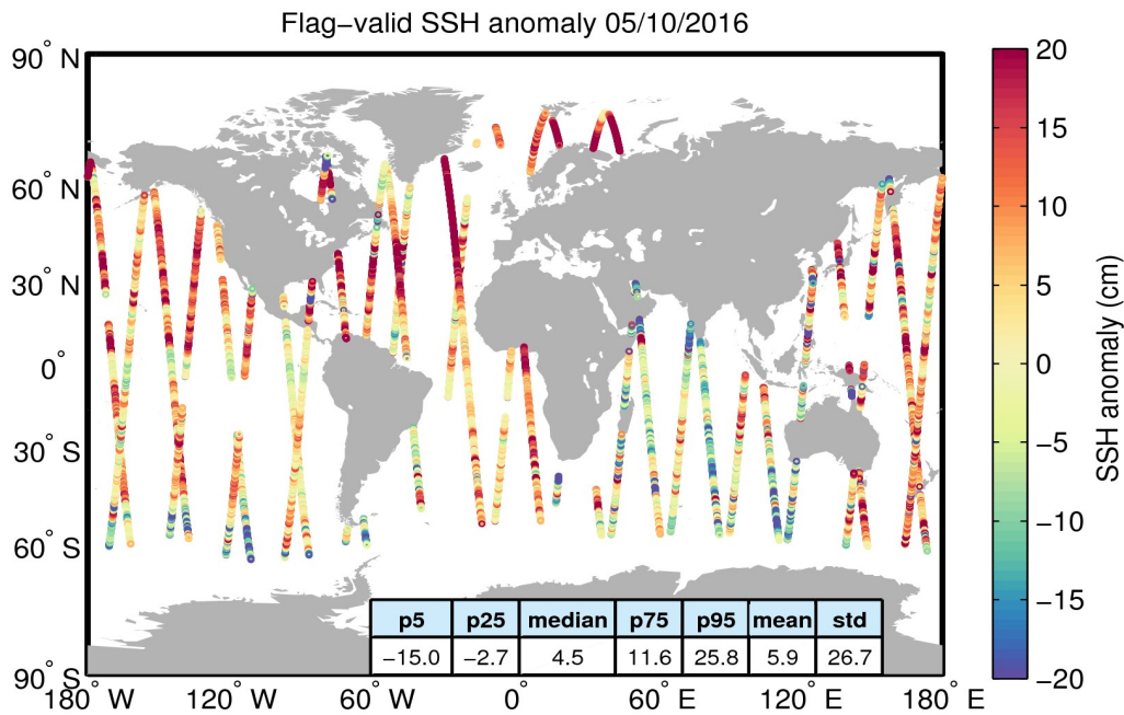
Figure 5. Geographical distribution of flag-valid 1-Hz SSH anomaly data over oceans and lakes for 05/10/2016. The statistical values shown in the table refer to the SSH anomaly in cm and are calculated over all measurements shown in the figure.
