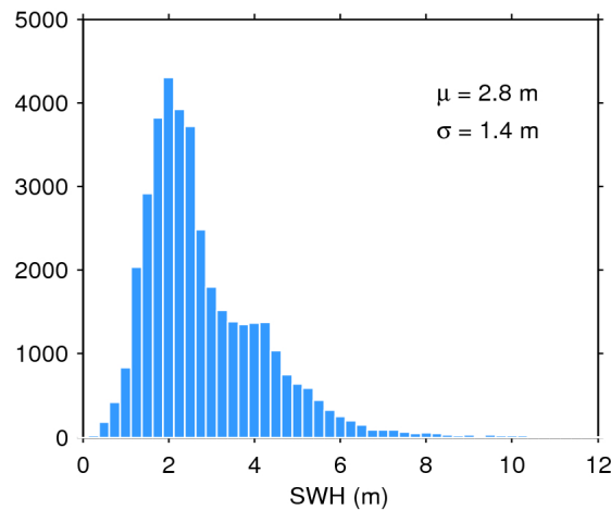
Figure 17. Histogram of flag-valid SWH over oceans and lakes for 05/10/2016. The mean ( \mu ) and standard deviation ( \sigma ) are also shown. Note that values larger than 12 m are excluded from the histogram for the sake of readability but not from the computation of \mu and \sigma .
