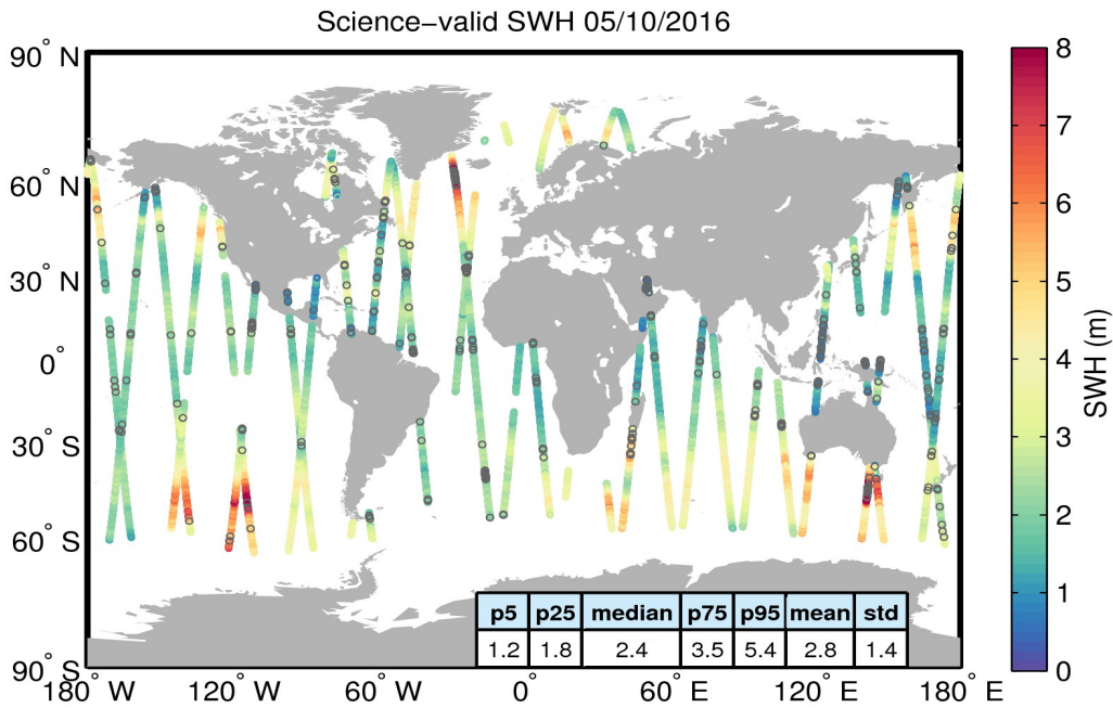
Figure 19. Geographical distribution of science-valid SWH data over oceans and lakes for 05/10/2016. The statistical values shown in the table refer to the SWH in m and are calculated over all measurements shown in the figure. Gray circles denote records that have been rejected based on the editing criteria described in Table 3.
