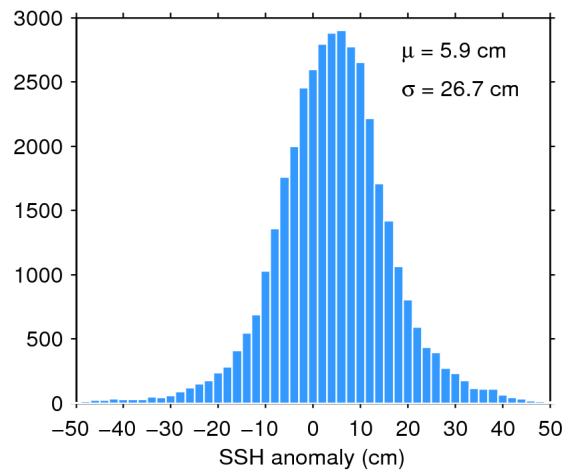
Figure 7. Histogram of flag-valid SSH anomaly over oceans and lakes for 05/10/2016. The mean ( \mu ) and standard deviation ( \sigma ) are also shown. Note that values outside [-50\ 50] cm are excluded from the histogram for the sake of readability but not from the computation of \mu and \sigma .
