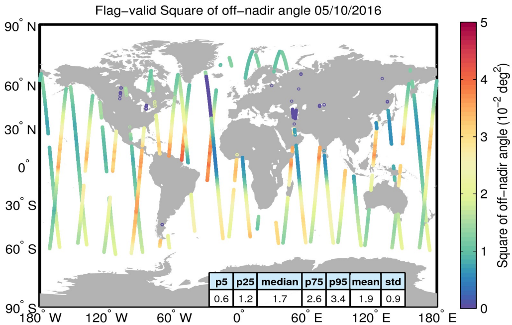
Figure 37. Geographical distribution of flag-valid mispointing data over oceans and lakes for 05/10/2016. The statistical values shown in the table refer to the mispointing in 10^{-2} deg 2 and are calculated over all measurements shown in the figure.
