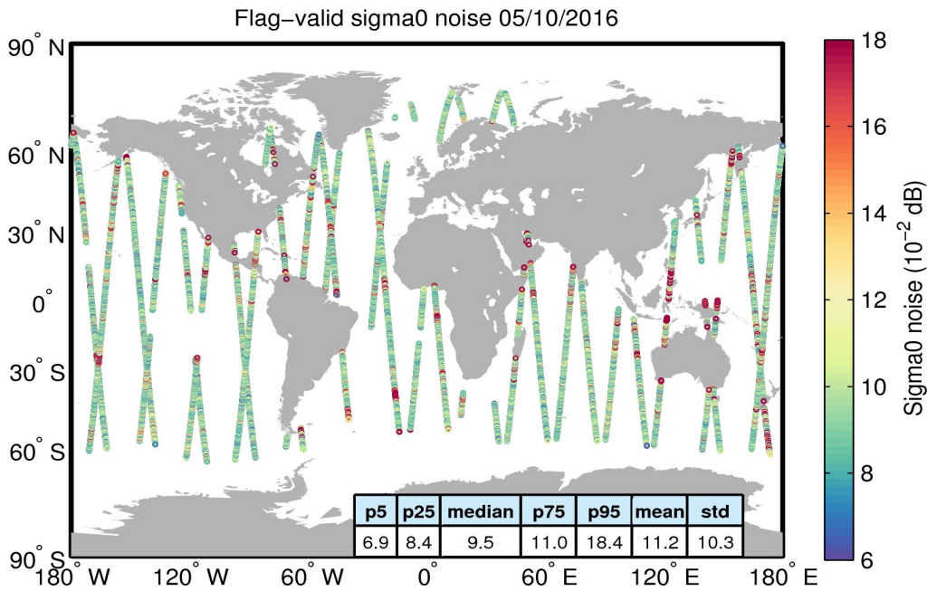
Figure 26. Geographical distribution of flag-valid 20-Hz sigma0 measurement noise over oceans and lakes for 05/10/2016. The statistical values shown in the table refer to the sigma0 noise and are calculated over all measurements shown in the figure.
