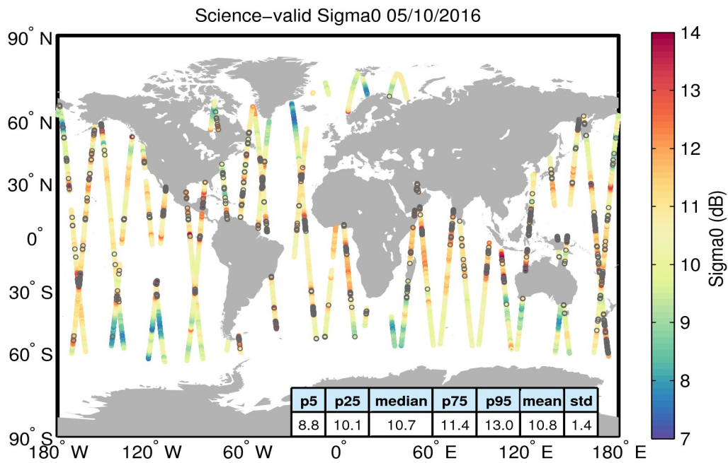
Figure 27. Geographical distribution of science-valid sigma0 data over oceans and lakes for 05/10/2016. The statistical values shown in the table refer to the sigma0 in dB and are calculated over all measurements shown in the figure. Gray circles denote records that have been rejected based on the editing criteria described in Table 4.
