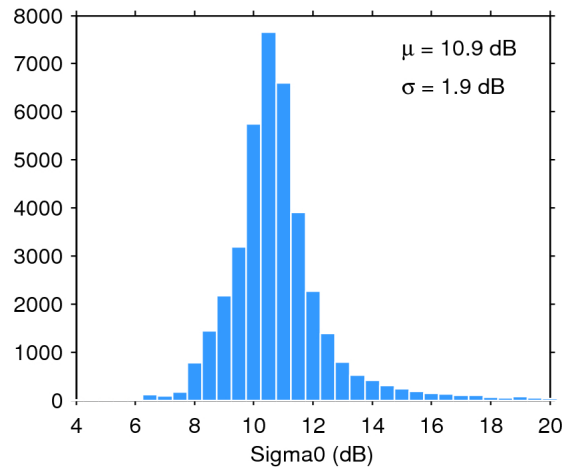
Figure 25. Histogram of flag-valid sigma0 over oceans and lakes for 03/10/2016. The mean ( \mu ) and standard deviation ( \sigma ) are also shown. Note that values outside [4 20] dB are excluded from the histogram for the sake of readability but not from the computation of \mu and \sigma .
