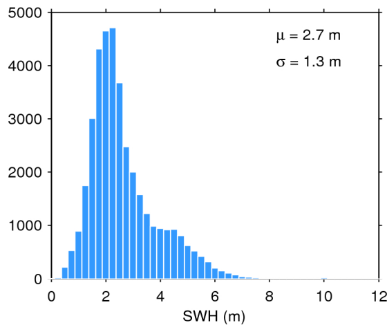
Figure 20. Histogram of science-valid SWH over oceans and lakes for 03/10/2016. The mean ( \mu ) and standard deviation ( \sigma ) are also shown. Note that values larger than 12 m are excluded from the histogram for the sake of readability but not from the computation of \mu and \sigma .
