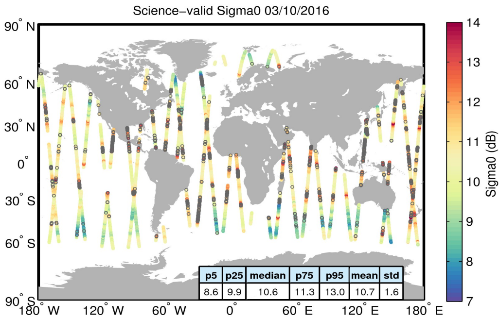
Figure 27. Geographical distribution of science-valid sigma0 data over oceans and lakes for 03/10/2016. The statistical values shown in the table refer to the sigma0 in dB and are calculated over all measurements shown in the figure. Gray circles denote records that have been rejected based on the editing criteria described in Table 4.
