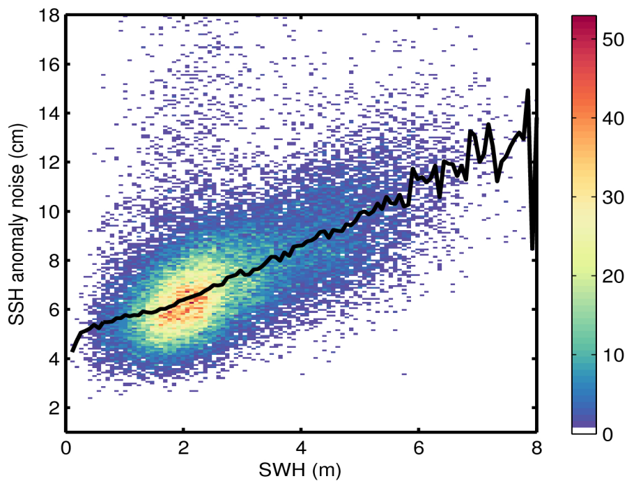
Figure 9. 2D histogram showing flag-valid SSH anomaly noise as a function of SWH for 03/10/2016. The black line denotes the median SSH anomaly noise as a function of SWH.
