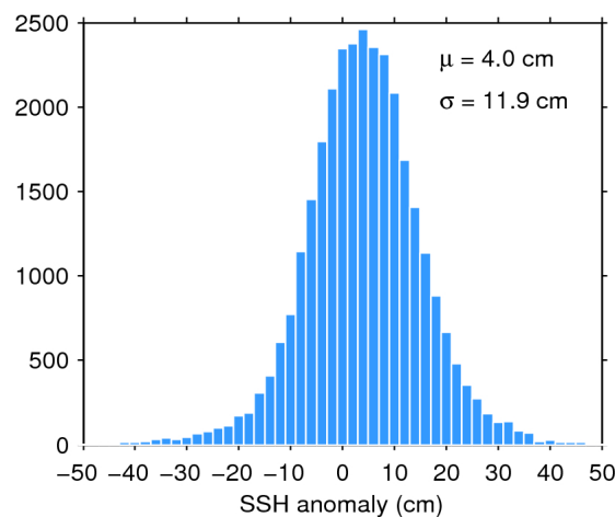
Figure 11. Histogram of science-valid SSH anomaly over oceans and lakes for 03/10/2016. The mean ( \mu ) and standard deviation ( \sigma ) are also shown. Note that values outside [-50 50] cm are excluded from the histogram for the sake of readability but not from the computation of \mu and \sigma .
