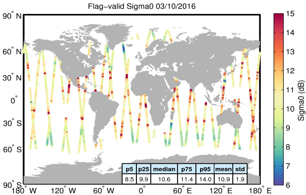
Figure 23. Geographical distribution of flag-valid sigma0 data over oceans and lakes for 03/10/2016. The statistical values shown in the table refer to the sigma0 in dB and are calculated over all measurements shown in the figure.
