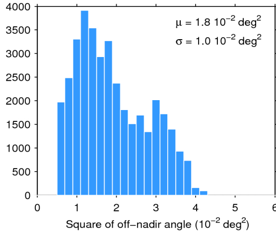
Figure 39. Histogram of flag-valid mispointing over oceans and lakes for 03/10/2016. The mean ( \mu ) and standard deviation ( \sigma ) are also shown. Note that values larger than 6 \cdot 10^{-2} \text{ deg}^2 are excluded from the histogram for the sake of readability but not from the computation of \mu and \sigma .
