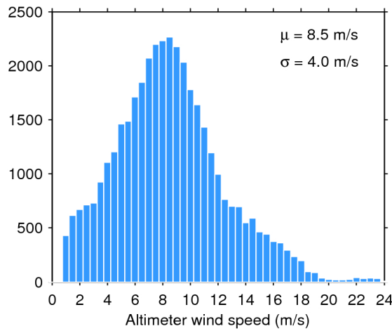
Figure 33. Histogram of flag-valid wind over oceans and lakes for 03/10/2016. The mean ( \mu ) and standard deviation ( \sigma ) are also shown. Note that values larger than 24 m/s are excluded from the histogram for the sake of readability but not from the computation of \mu and \sigma .
