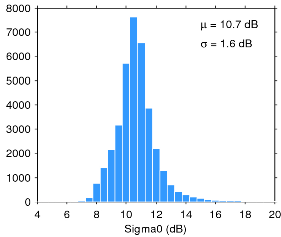
Figure 28. Histogram of science-valid sigma0 over oceans and lakes for 03/10/2016. The mean ( \mu ) and standard deviation ( \sigma ) are also shown. Note that values outside [4 20] dB are excluded from the histogram for the sake of readability but not from the computation of \mu and \sigma .
