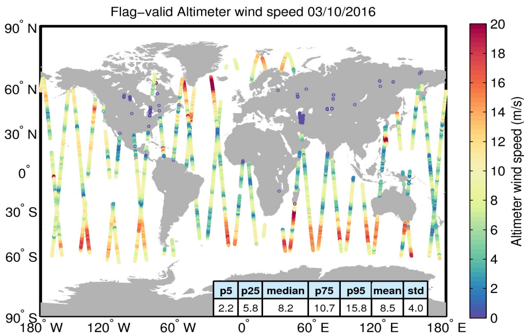
Figure 31. Geographical distribution of flag-valid wind data over oceans and lakes for 03/10/2016. The statistical values shown in the table refer to the wind in m/s and are calculated over all measurements shown in the figure.
