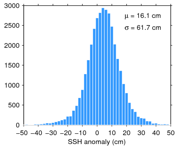
Figure 7. Histogram of flag-valid SSH anomaly over oceans and lakes for 03/10/2016. The mean ( \mu ) and standard deviation ( \sigma ) are also shown. Note that values outside [-50 50] cm are excluded from the histogram for the sake of readability but not from the computation of \mu and \sigma .
