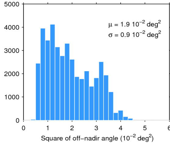
Figure 39. Histogram of flag-valid mispointing over oceans and lakes for 02/10/2016. The mean ( \mu ) and standard deviation ( \sigma ) are also shown. Note that values larger than 6 \cdot 10^{-2} \text{ deg}^2 are excluded from the histogram for the sake of readability but not from the computation of \mu and \sigma .
