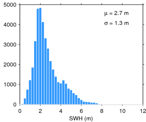
Figure 17. Histogram of flag-valid SWH over oceans and lakes for 02/10/2016. The mean ( \mu ) and standard deviation ( \sigma ) are also shown. Note that values larger than 12 m are excluded from the histogram for the sake of readability but not from the computation of \mu and \sigma .
