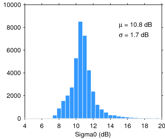
Figure 28. Histogram of science-valid sigma0 over oceans and lakes for 02/10/2016. The mean ( \mu ) and standard deviation ( \sigma ) are also shown. Note that values outside [4 20] dB are excluded from the histogram for the sake of readability but not from the computation of \mu and \sigma .
