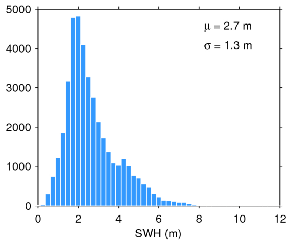
Figure 20. Histogram of science-valid SWH over oceans and lakes for 02/10/2016. The mean ( \mu ) and standard deviation ( \sigma ) are also shown. Note that values larger than 12 m are excluded from the histogram for the sake of readability but not from the computation of \mu and \sigma .
