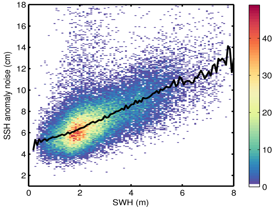
Figure 9. 2D histogram showing flag-valid SSH anomaly noise as a function of SWH for 02/10/2016. The black line denotes the median SSH anomaly noise as a function of SWH.
