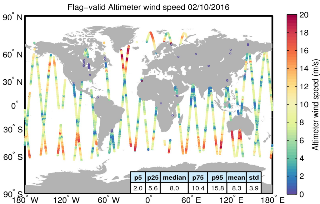
Figure 31. Geographical distribution of flag-valid wind data over oceans and lakes for 02/10/2016. The statistical values shown in the table refer to the wind in m/s and are calculated over all measurements shown in the figure.
