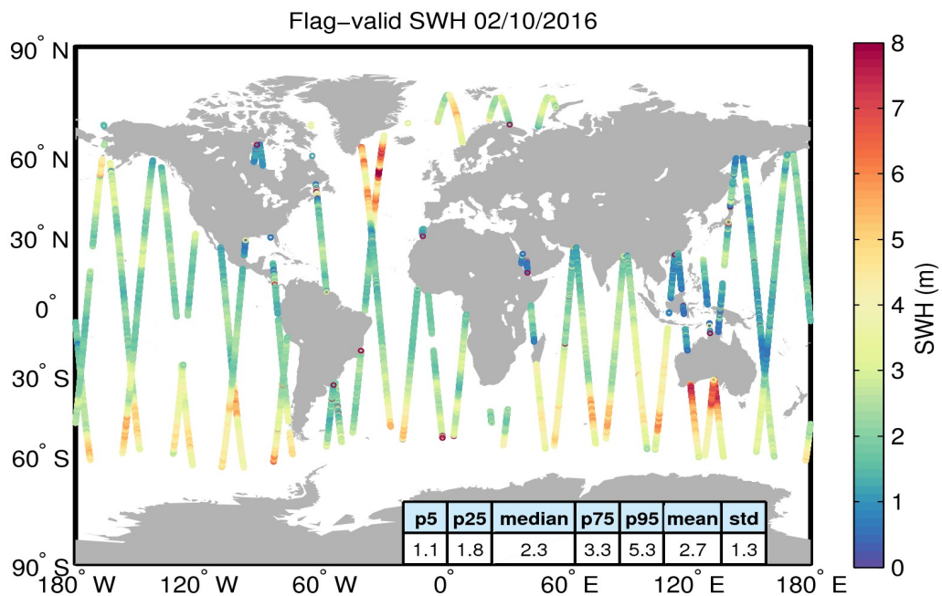
Figure 15. Geographical distribution of flag-valid SWH data over oceans and lakes for 02/10/2016. The statistical values shown in the table refer to the SWH in m and are calculated over all measurements shown in the figure.
