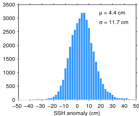
Figure 11. Histogram of science-valid SSH anomaly over oceans and lakes for 02/10/2016. The mean ( \mu ) and standard deviation ( \sigma ) are also shown. Note that values outside [-50 50] cm are excluded from the histogram for the sake of readability but not from the computation of \mu and \sigma .
