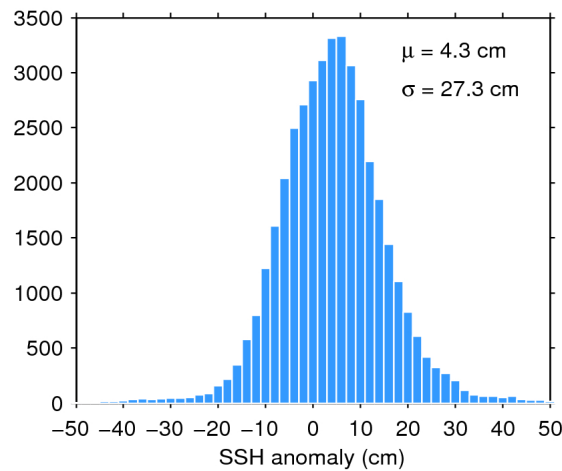
Figure 7. Histogram of flag-valid SSH anomaly over oceans and lakes for 02/10/2016. The mean ( \mu ) and standard deviation ( \sigma ) are also shown. Note that values outside [-50 50] cm are excluded from the histogram for the sake of readability but not from the computation of \mu and \sigma .
