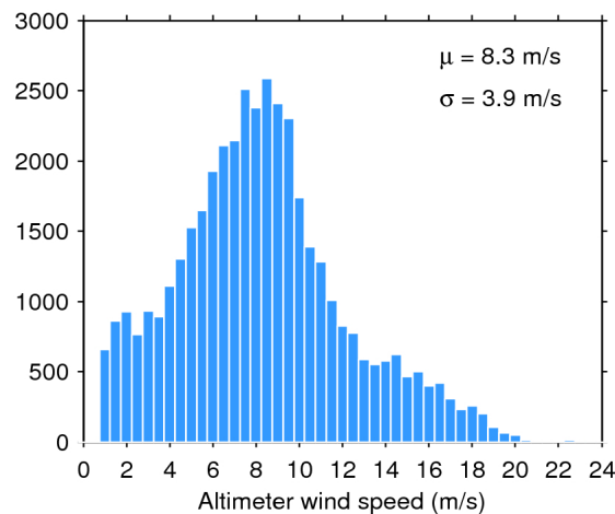
Figure 35. Histogram of science-valid wind over oceans and lakes for 02/10/2016. The mean ( \mu ) and standard deviation ( \sigma ) are also shown. Note that values larger than 24 m/s are excluded from the histogram for the sake of readability but not from the computation of \mu and \sigma .
