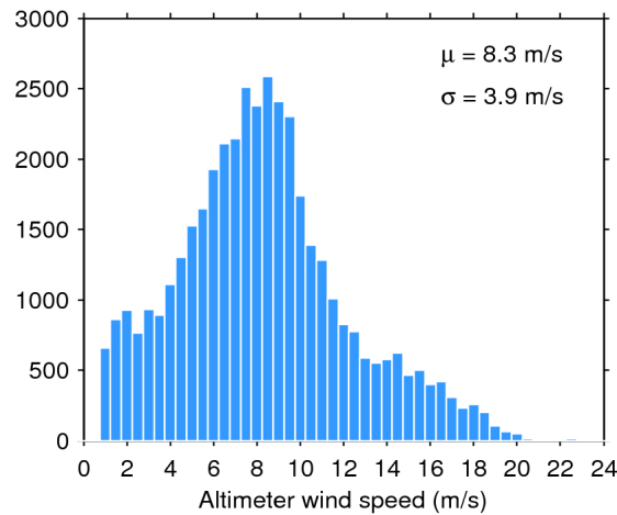
Figure 33. Histogram of flag-valid wind over oceans and lakes for 02/10/2016. The mean ( \mu ) and standard deviation ( \sigma ) are also shown. Note that values larger than 24 m/s are excluded from the histogram for the sake of readability but not from the computation of \mu and \sigma .
