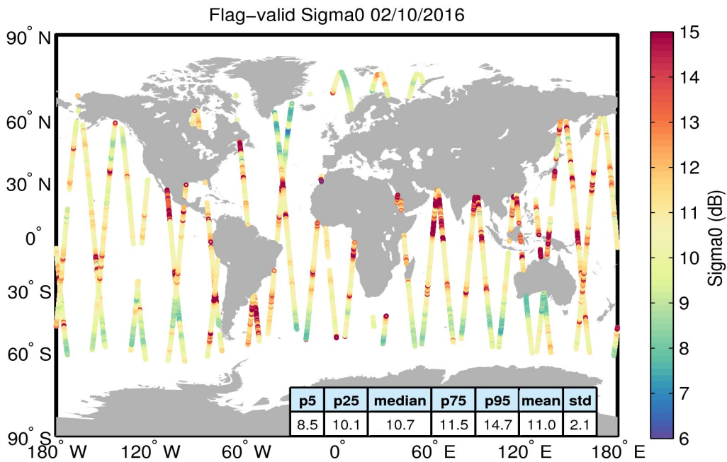
Figure 23. Geographical distribution of flag-valid sigma0 data over oceans and lakes for 02/10/2016. The statistical values shown in the table refer to the sigma0 in dB and are calculated over all measurements shown in the figure.
