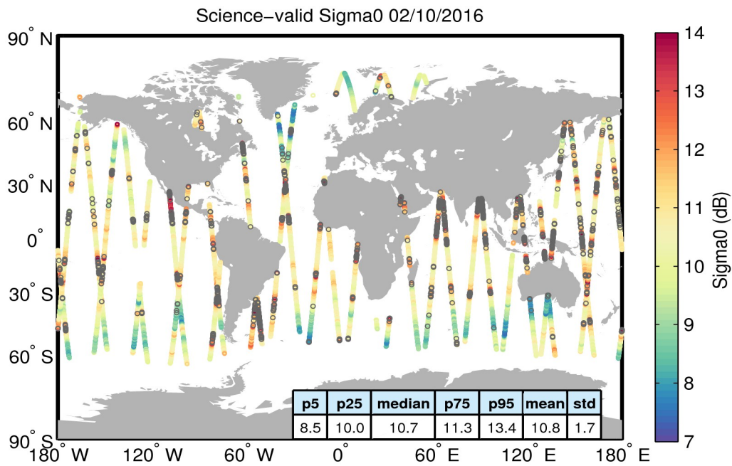
Figure 27. Geographical distribution of science-valid sigma0 data over oceans and lakes for 02/10/2016. The statistical values shown in the table refer to the sigma0 in dB and are calculated over all measurements shown in the figure. Gray circles denote records that have been rejected based on the editing criteria described in Table 4.
