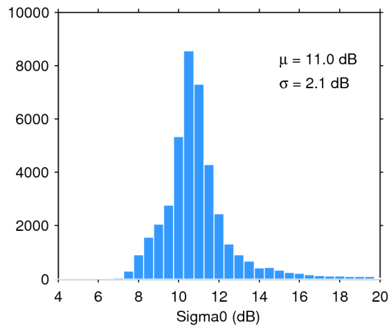
Figure 25. Histogram of flag-valid sigma0 over oceans and lakes for 02/10/2016. The mean ( \mu ) and standard deviation ( \sigma ) are also shown. Note that values outside [4 20] dB are excluded from the histogram for the sake of readability but not from the computation of \mu and \sigma .
