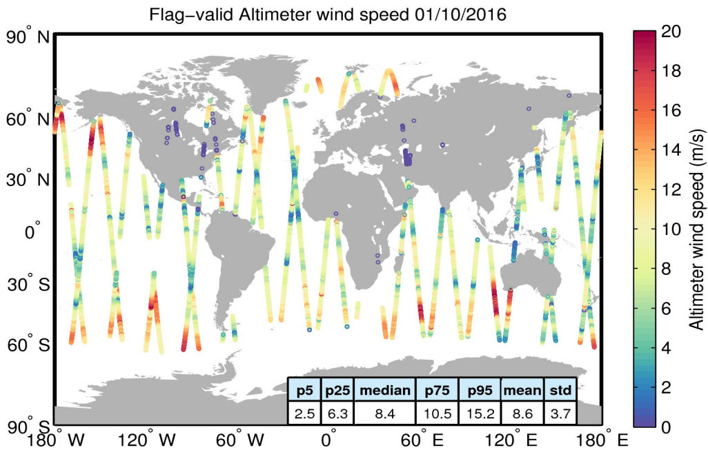
Figure 31. Geographical distribution of flag-valid wind data over oceans and lakes for 01/10/2016. The statistical values shown in the table refer to the wind in m/s and are calculated over all measurements shown in the figure.
