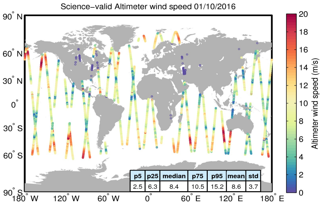
Figure 34. Geographical distribution of science-valid wind data over oceans and lakes for 01/10/2016. The statistical values shown in the table refer to the wind in m/s and are calculated over all measurements shown in the figure. Gray circles denote records that have been rejected based on the editing criteria described in Table 5.
