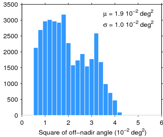
Figure 39. Histogram of flag-valid mispointing over oceans and lakes for 01/10/2016. The mean ( \mu ) and standard deviation ( \sigma ) are also shown. Note that values larger than 6 \cdot 10^{-2} \text{ deg}^2 are excluded from the histogram for the sake of readability but not from the computation of \mu and \sigma .
