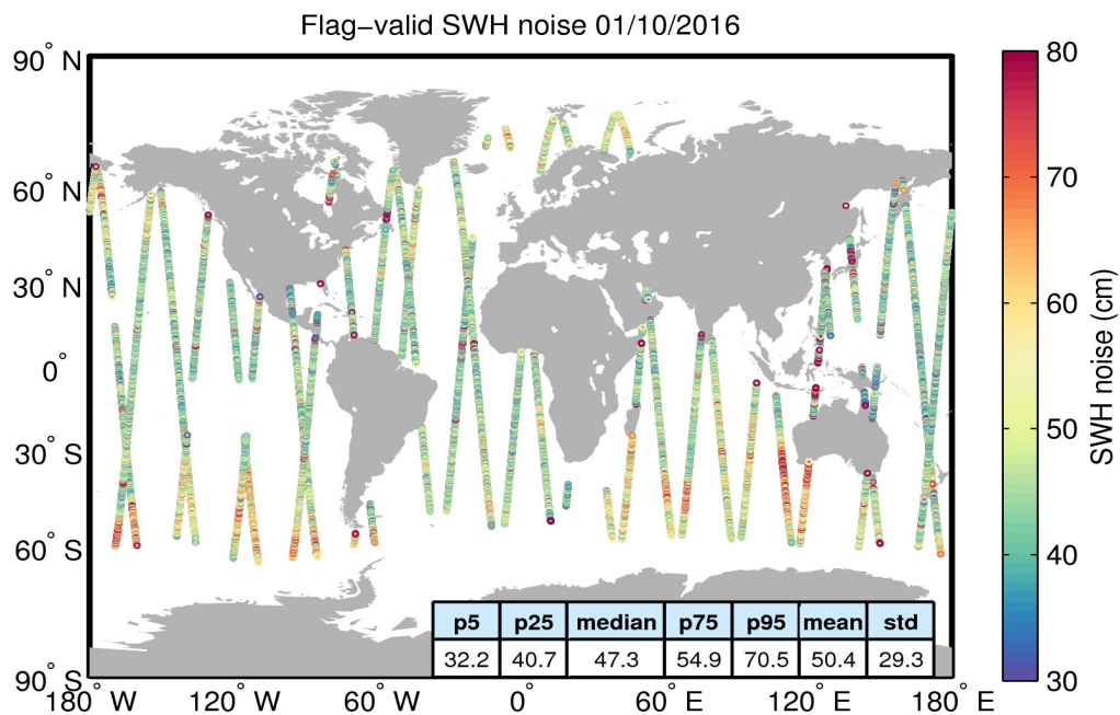
Figure 18. Geographical distribution of flag-valid 20-Hz SWH measurement noise over oceans and lakes for 01/10/2016. The statistical values shown in the table refer to the SWH noise and are calculated over all measurements shown in the figure.
