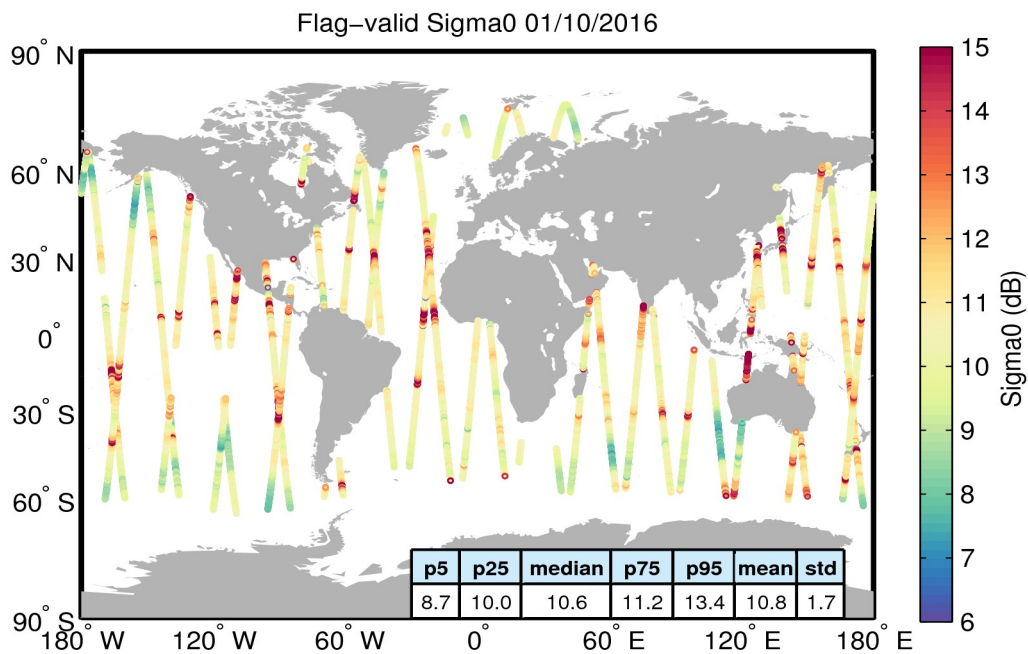
Figure 23. Geographical distribution of flag-valid sigma0 data over oceans and lakes for 01/10/2016. The statistical values shown in the table refer to the sigma0 in dB and are calculated over all measurements shown in the figure.
