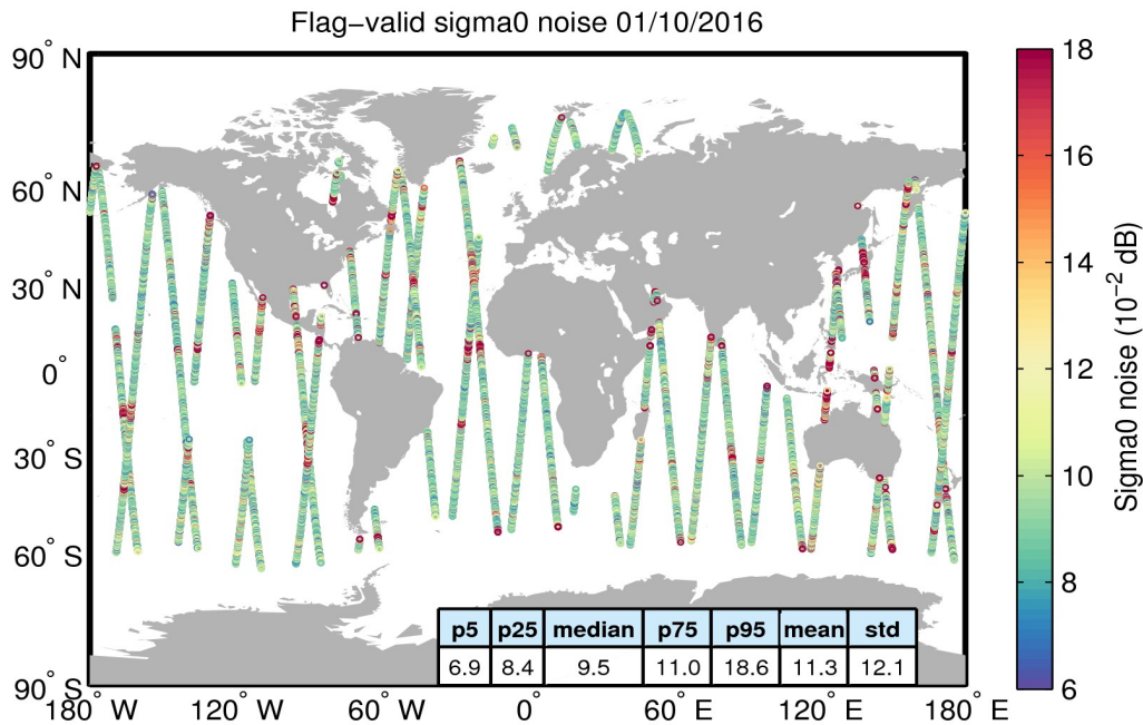
Figure 26. Geographical distribution of flag-valid 20-Hz sigma0 measurement noise over oceans and lakes for 01/10/2016. The statistical values shown in the table refer to the sigma0 noise and are calculated over all measurements shown in the figure.
