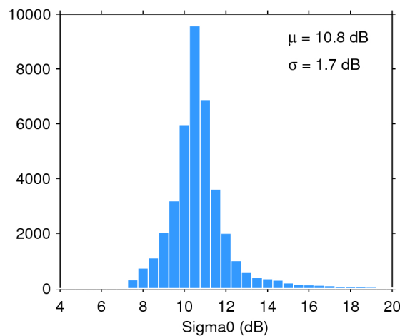
Figure 25. Histogram of flag-valid sigma0 over oceans and lakes for 01/10/2016. The mean ( \mu ) and standard deviation ( \sigma ) are also shown. Note that values outside [4 20] dB are excluded from the histogram for the sake of readability but not from the computation of \mu and \sigma .
