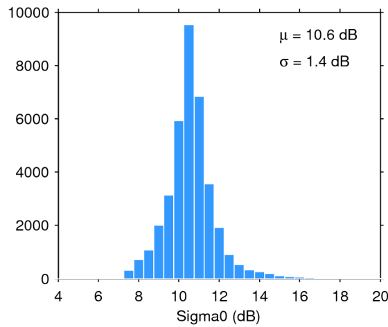
Figure 28. Histogram of science-valid sigma0 over oceans and lakes for 01/10/2016. The mean ( \mu ) and standard deviation ( \sigma ) are also shown. Note that values outside [4 20] dB are excluded from the histogram for the sake of readability but not from the computation of \mu and \sigma .
