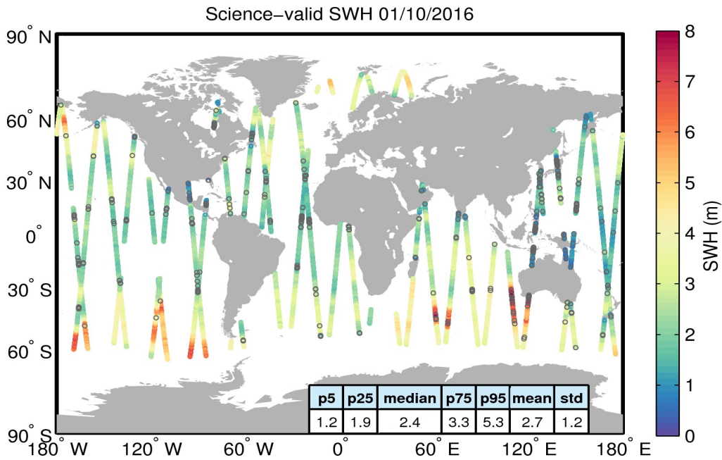
Figure 19. Geographical distribution of science-valid SWH data over oceans and lakes for 01/10/2016. The statistical values shown in the table refer to the SWH in m and are calculated over all measurements shown in the figure. Gray circles denote records that have been rejected based on the editing criteria described in Table 3.
