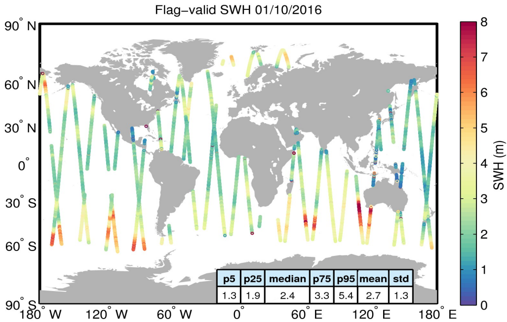
Figure 15. Geographical distribution of flag-valid SWH data over oceans and lakes for 01/10/2016. The statistical values shown in the table refer to the SWH in m and are calculated over all measurements shown in the figure.
