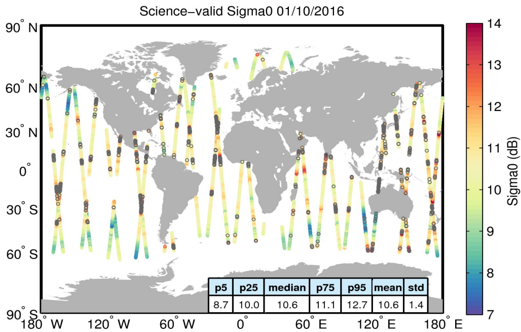
Figure 27. Geographical distribution of science-valid sigma0 data over oceans and lakes for 01/10/2016. The statistical values shown in the table refer to the sigma0 in dB and are calculated over all measurements shown in the figure. Gray circles denote records that have been rejected based on the editing criteria described in Table 4.
