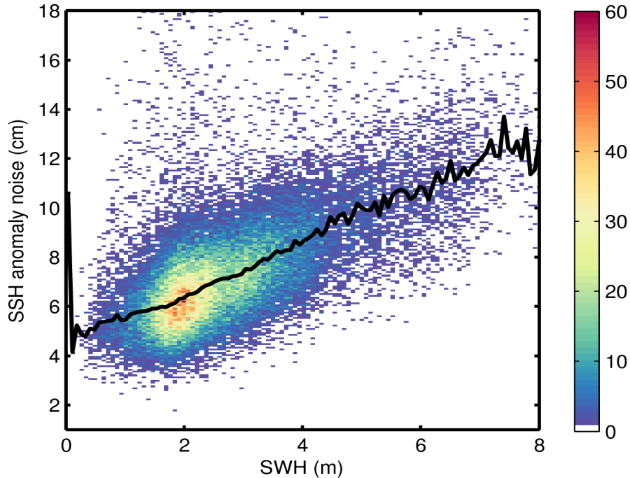
Figure 9. 2D histogram showing flag-valid SSH anomaly noise as a function of SWH for 01/10/2016. The black line denotes the median SSH anomaly noise as a function of SWH.
