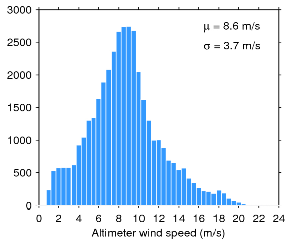
Figure 35. Histogram of science-valid wind over oceans and lakes for 01/10/2016. The mean ( \mu ) and standard deviation ( \sigma ) are also shown. Note that values larger than 24 m/s are excluded from the histogram for the sake of readability but not from the computation of \mu and \sigma .
