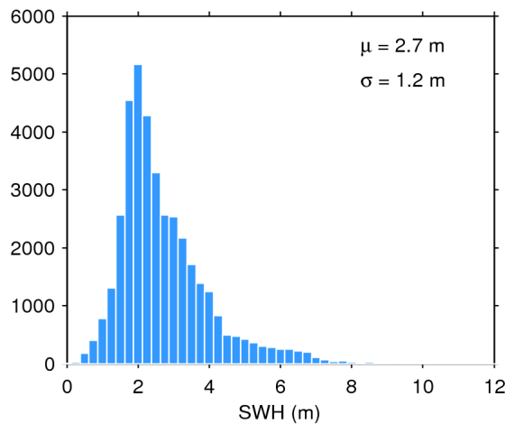
Figure 20. Histogram of science-valid SWH over oceans and lakes for 01/10/2016. The mean ( \mu ) and standard deviation ( \sigma ) are also shown. Note that values larger than 12 m are excluded from the histogram for the sake of readability but not from the computation of \mu and \sigma .
