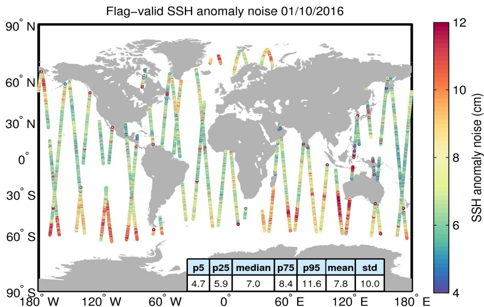
Figure 8. Geographical distribution of flag-valid 20-Hz SSH anomaly measurement noise over oceans and lakes for 01/10/2016. The statistical values shown in the table refer to the SSH anomaly noise and are calculated over all measurements shown in the figure.
