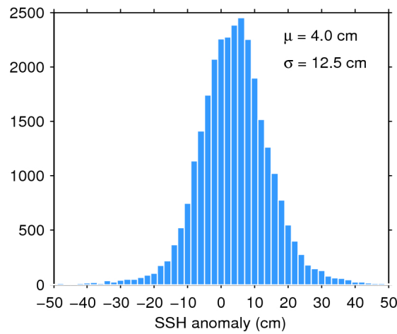
Figure 11. Histogram of science-valid SSH anomaly over oceans and lakes for 01/10/2016. The mean ( \mu ) and standard deviation ( \sigma ) are also shown. Note that values outside [-50 50] cm are excluded from the histogram for the sake of readability but not from the computation of \mu and \sigma .
