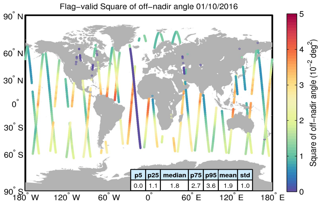
Figure 37. Geographical distribution of flag-valid mispointing data over oceans and lakes for 01/10/2016. The statistical values shown in the table refer to the mispointing in 10^{-2} deg 2 and are calculated over all measurements shown in the figure.
