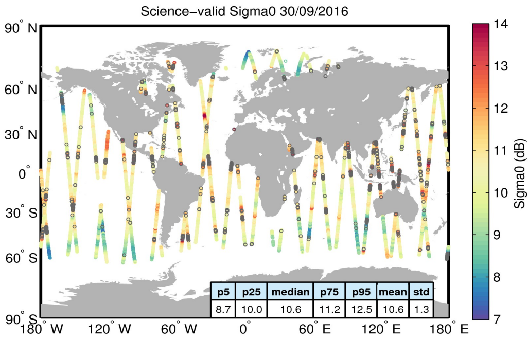
Figure 27. Geographical distribution of science-valid sigma0 data over oceans and lakes for 30/09/2016. The statistical values shown in the table refer to the sigma0 in dB and are calculated over all measurements shown in the figure. Gray circles denote records that have been rejected based on the editing criteria described in Table 4.
