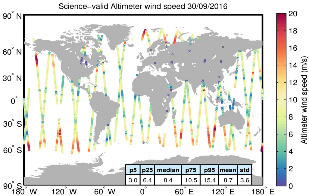
Figure 34. Geographical distribution of science-valid wind data over oceans and lakes for 30/09/2016. The statistical values shown in the table refer to the wind in m/s and are calculated over all measurements shown in the figure. Gray circles denote records that have been rejected based on the editing criteria described in Table 5.
