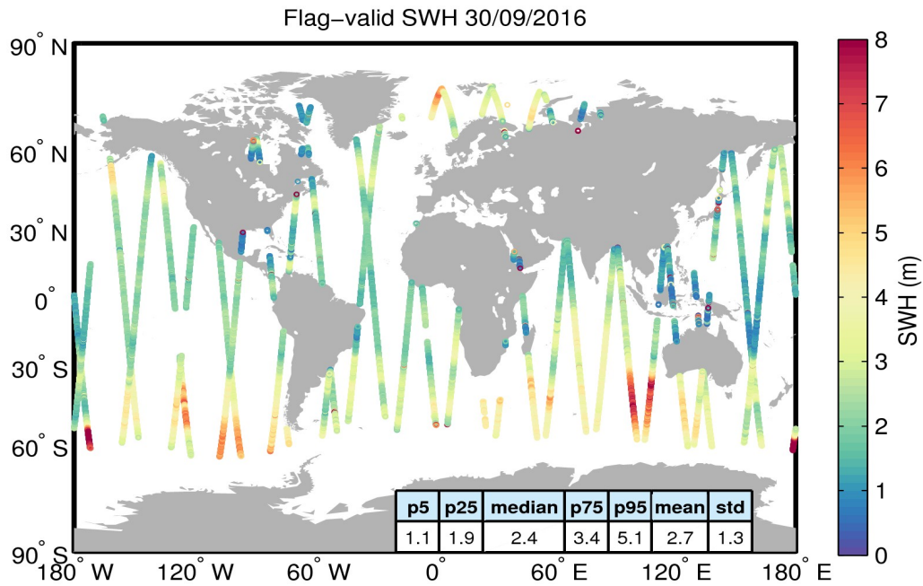
Figure 15. Geographical distribution of flag-valid SWH data over oceans and lakes for 30/09/2016. The statistical values shown in the table refer to the SWH in m and are calculated over all measurements shown in the figure.
