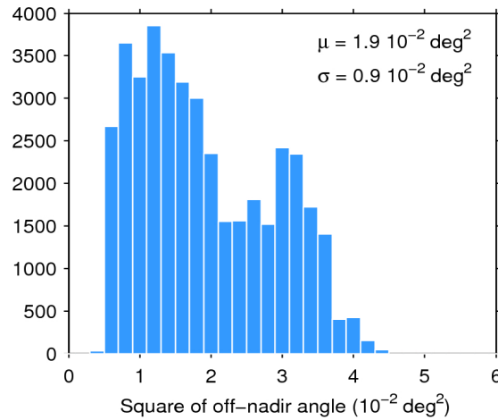
Figure 39. Histogram of flag-valid mispointing over oceans and lakes for 30/09/2016. The mean ( \mu ) and standard deviation ( \sigma ) are also shown. Note that values larger than 6 \cdot 10^{-2} \text{ deg}^2 are excluded from the histogram for the sake of readability but not from the computation of \mu and \sigma .
