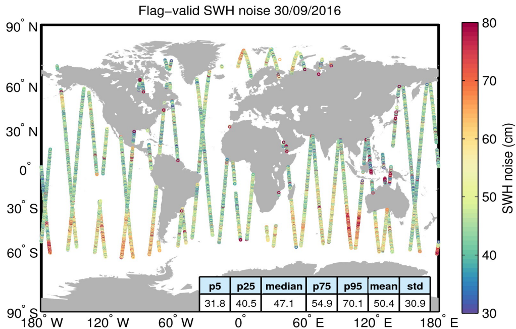
Figure 18. Geographical distribution of flag-valid 20-Hz SWH measurement noise over oceans and lakes for 30/09/2016. The statistical values shown in the table refer to the SWH noise and are calculated over all measurements shown in the figure.
