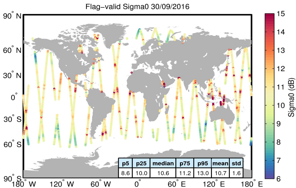
Figure 23. Geographical distribution of flag-valid sigma0 data over oceans and lakes for 30/09/2016. The statistical values shown in the table refer to the sigma0 in dB and are calculated over all measurements shown in the figure.
