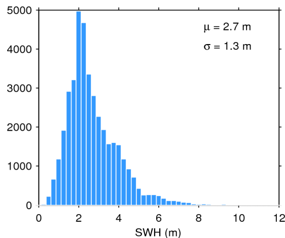
Figure 20. Histogram of science-valid SWH over oceans and lakes for 30/09/2016. The mean ( \mu ) and standard deviation ( \sigma ) are also shown. Note that values larger than 12 m are excluded from the histogram for the sake of readability but not from the computation of \mu and \sigma .
