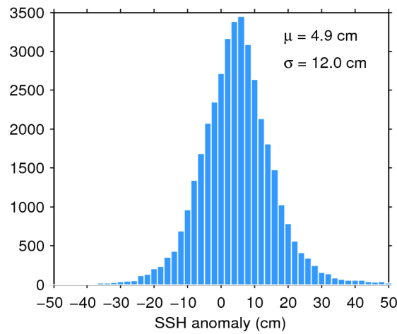
Figure 11. Histogram of science-valid SSH anomaly over oceans and lakes for 30/09/2016. The mean ( \mu ) and standard deviation ( \sigma ) are also shown. Note that values outside [-50 50] cm are excluded from the histogram for the sake of readability but not from the computation of \mu and \sigma .
