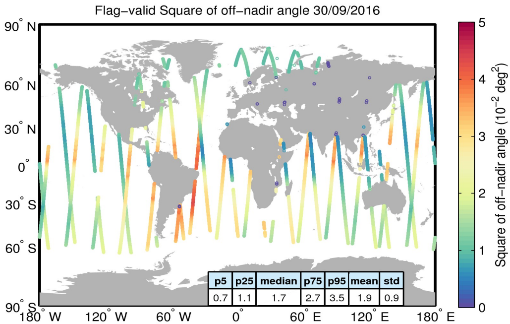
Figure 37. Geographical distribution of flag-valid mispointing data over oceans and lakes for 30/09/2016. The statistical values shown in the table refer to the mispointing in 10^{-2} deg 2 and are calculated over all measurements shown in the figure.
