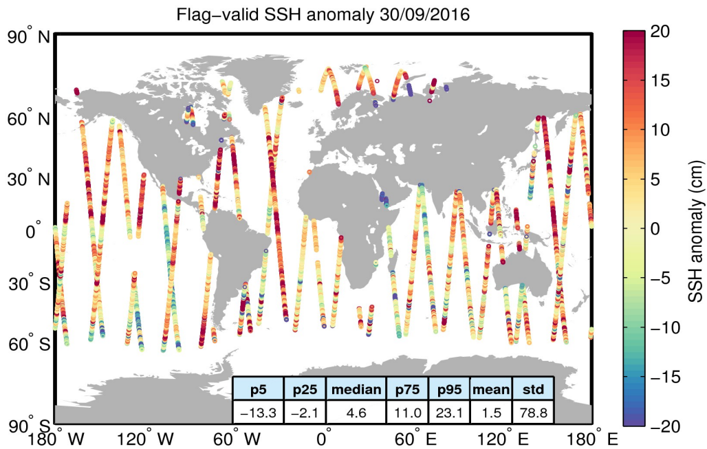
Figure 5. Geographical distribution of flag-valid 1-Hz SSH anomaly data over oceans and lakes for 30/09/2016. The statistical values shown in the table refer to the SSH anomaly in cm and are calculated over all measurements shown in the figure.
