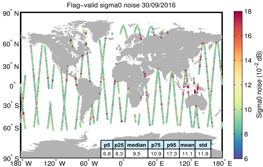
Figure 26. Geographical distribution of flag-valid 20-Hz sigma0 measurement noise over oceans and lakes for 30/09/2016. The statistical values shown in the table refer to the sigma0 noise and are calculated over all measurements shown in the figure.
