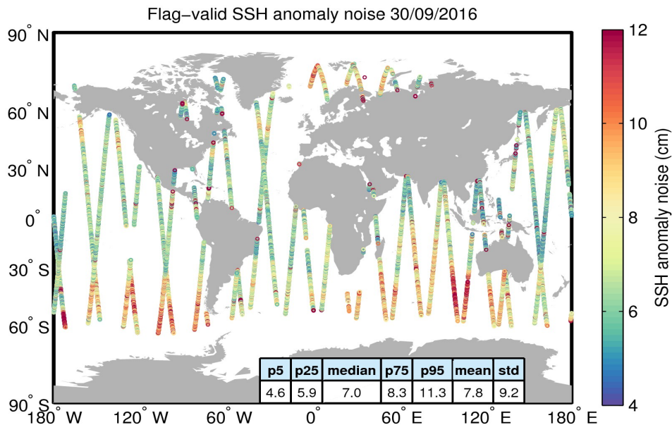
Figure 8. Geographical distribution of flag-valid 20-Hz SSH anomaly measurement noise over oceans and lakes for 30/09/2016. The statistical values shown in the table refer to the SSH anomaly noise and are calculated over all measurements shown in the figure.
