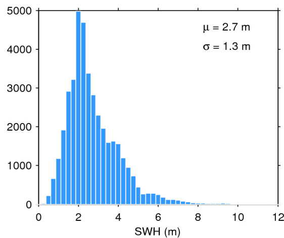
Figure 17. Histogram of flag-valid SWH over oceans and lakes for 30/09/2016. The mean ( \mu ) and standard deviation ( \sigma ) are also shown. Note that values larger than 12 m are excluded from the histogram for the sake of readability but not from the computation of \mu and \sigma .
