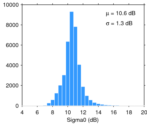
Figure 28. Histogram of science-valid sigma0 over oceans and lakes for 30/09/2016. The mean ( \mu ) and standard deviation ( \sigma ) are also shown. Note that values outside [4 20] dB are excluded from the histogram for the sake of readability but not from the computation of \mu and \sigma .
