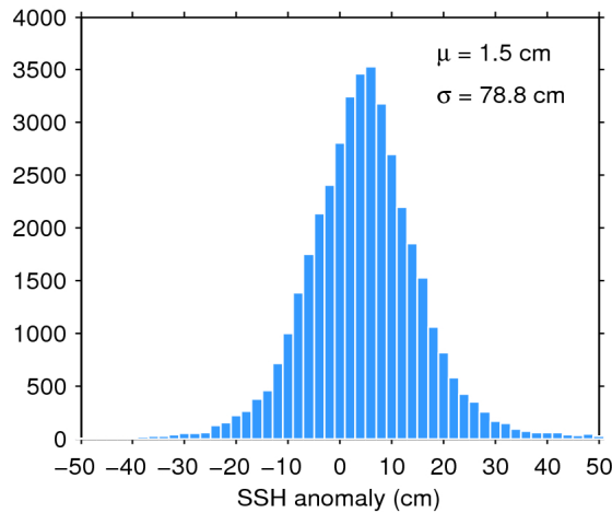
Figure 7. Histogram of flag-valid SSH anomaly over oceans and lakes for 30/09/2016. The mean ( \mu ) and standard deviation ( \sigma ) are also shown. Note that values outside [-50 50] cm are excluded from the histogram for the sake of readability but not from the computation of \mu and \sigma .
