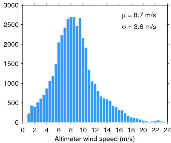
Figure 33. Histogram of flag-valid wind over oceans and lakes for 30/09/2016. The mean ( \mu ) and standard deviation ( \sigma ) are also shown. Note that values larger than 24 m/s are excluded from the histogram for the sake of readability but not from the computation of \mu and \sigma .
