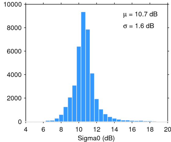
Figure 25. Histogram of flag-valid sigma0 over oceans and lakes for 30/09/2016. The mean ( \mu ) and standard deviation ( \sigma ) are also shown. Note that values outside [4 20] dB are excluded from the histogram for the sake of readability but not from the computation of \mu and \sigma .
