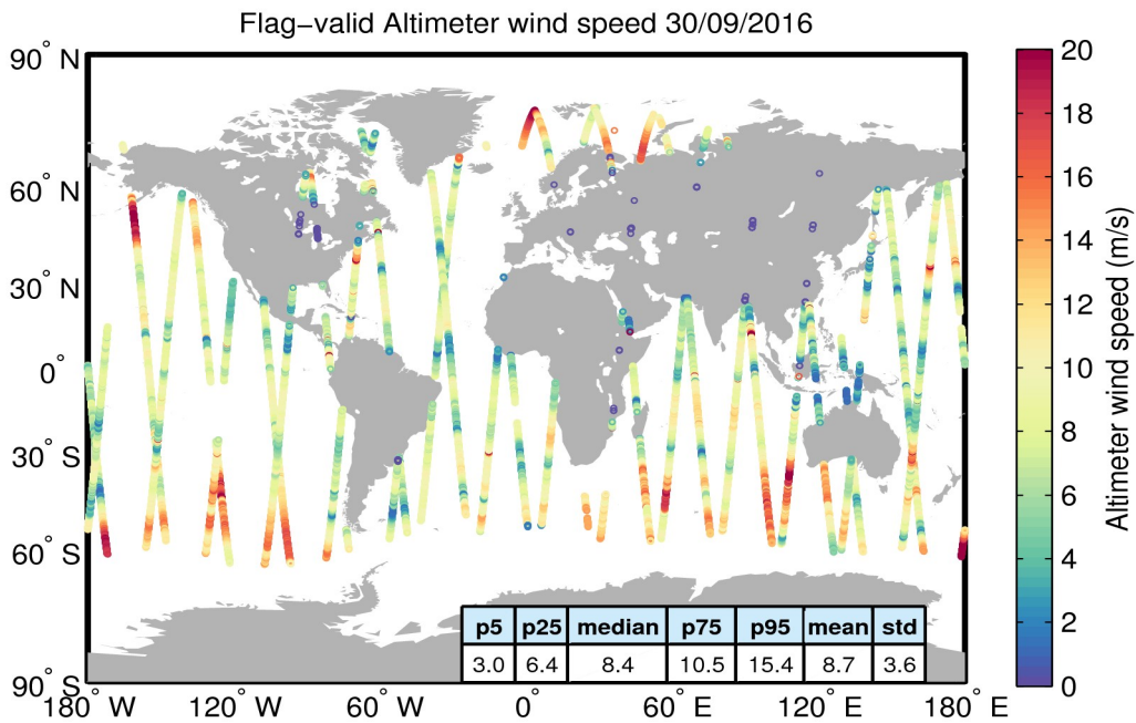
Figure 31. Geographical distribution of flag-valid wind data over oceans and lakes for 30/09/2016. The statistical values shown in the table refer to the wind in m/s and are calculated over all measurements shown in the figure.
