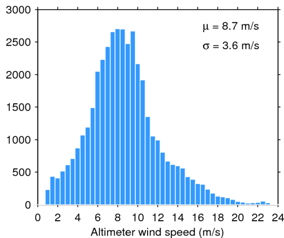
Figure 35. Histogram of science-valid wind over oceans and lakes for 30/09/2016. The mean ( \mu ) and standard deviation ( \sigma ) are also shown. Note that values larger than 24 m/s are excluded from the histogram for the sake of readability but not from the computation of \mu and \sigma .
