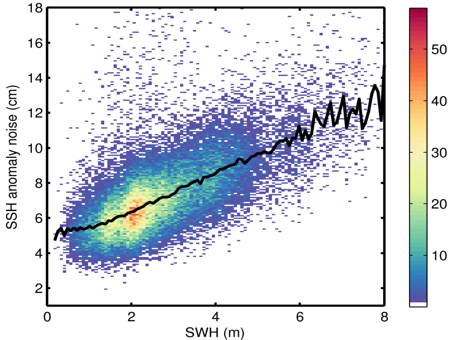
Figure 9. 2D histogram showing flag-valid SSH anomaly noise as a function of SWH for 30/09/2016. The black line denotes the median SSH anomaly noise as a function of SWH.
