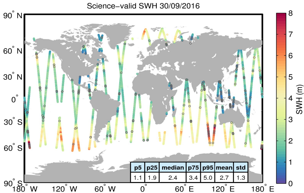
Figure 19. Geographical distribution of science-valid SWH data over oceans and lakes for 30/09/2016. The statistical values shown in the table refer to the SWH in m and are calculated over all measurements shown in the figure. Gray circles denote records that have been rejected based on the editing criteria described in Table 3.
