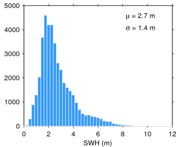
Figure 17. Histogram of flag-valid SWH over oceans and lakes for 24/09/2016. The mean ( \mu ) and standard deviation ( \sigma ) are also shown. Note that values larger than 12 m are excluded from the histogram for the sake of readability but not from the computation of \mu and \sigma .
