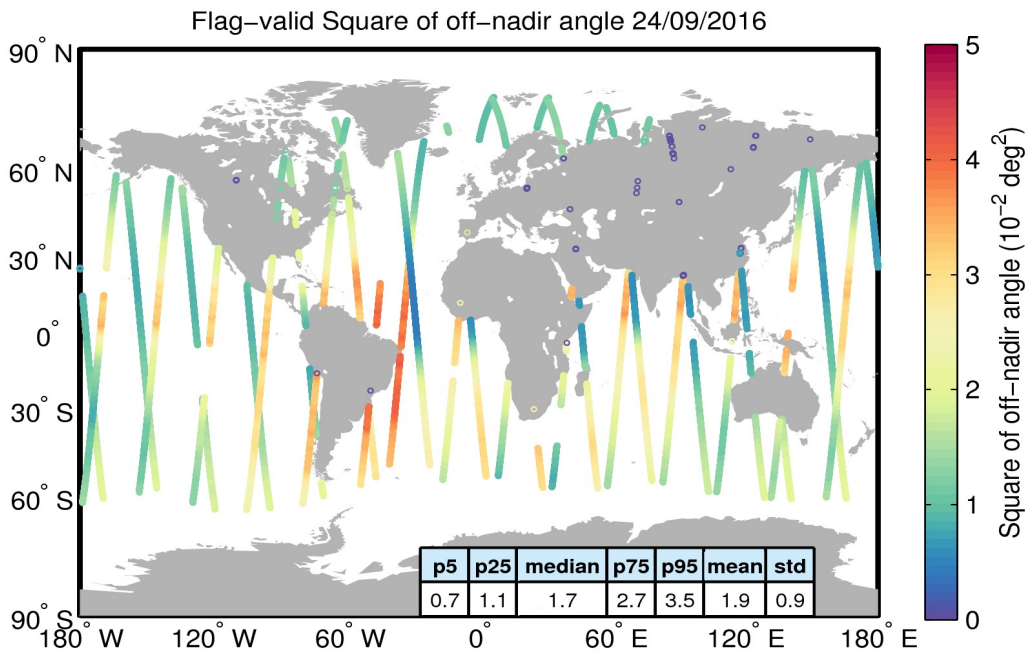
Figure 37. Geographical distribution of flag-valid mispointing data over oceans and lakes for 24/09/2016. The statistical values shown in the table refer to the mispointing in 10^{-2} deg 2 and are calculated over all measurements shown in the figure.
