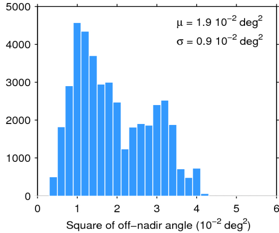
Figure 39. Histogram of flag-valid mispointing over oceans and lakes for 24/09/2016. The mean ( \mu ) and standard deviation ( \sigma ) are also shown. Note that values larger than 6 \cdot 10^{-2} \text{ deg}^2 are excluded from the histogram for the sake of readability but not from the computation of \mu and \sigma .
