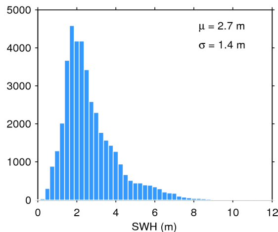
Figure 20. Histogram of science-valid SWH over oceans and lakes for 24/09/2016. The mean ( \mu ) and standard deviation ( \sigma ) are also shown. Note that values larger than 12 m are excluded from the histogram for the sake of readability but not from the computation of \mu and \sigma .
