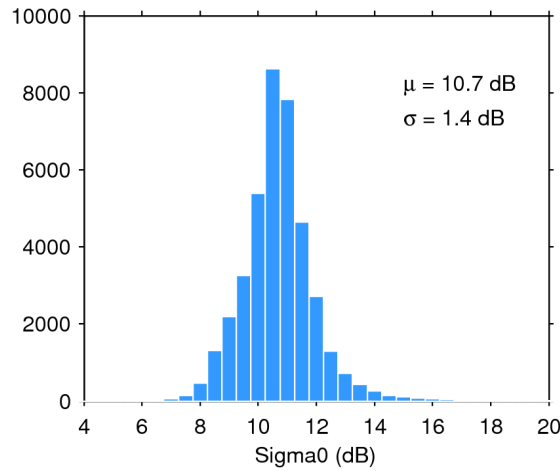
Figure 28. Histogram of science-valid sigma0 over oceans and lakes for 24/09/2016. The mean ( \mu ) and standard deviation ( \sigma ) are also shown. Note that values outside [4 20] dB are excluded from the histogram for the sake of readability but not from the computation of \mu and \sigma .
