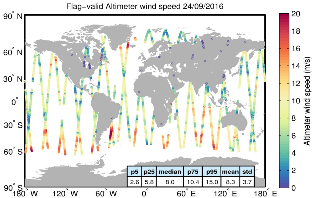
Figure 31. Geographical distribution of flag-valid wind data over oceans and lakes for 24/09/2016. The statistical values shown in the table refer to the wind in m/s and are calculated over all measurements shown in the figure.
