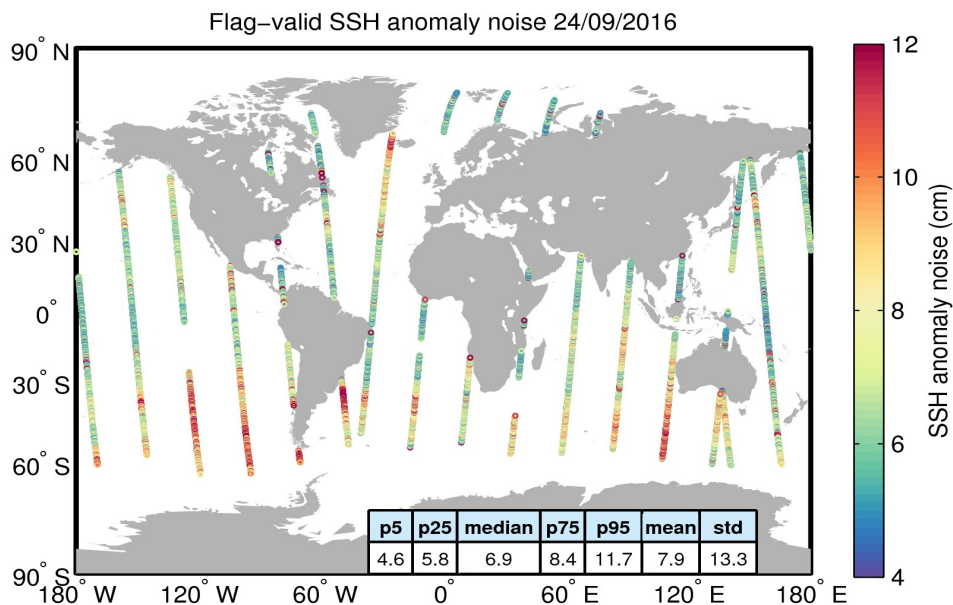
Figure 8. Geographical distribution of flag-valid 20-Hz SSH anomaly measurement noise over oceans and lakes for 24/09/2016. The statistical values shown in the table refer to the SSH anomaly noise and are calculated over all measurements shown in the figure.
