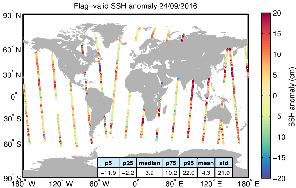
Figure 5. Geographical distribution of flag-valid 1-Hz SSH anomaly data over oceans and lakes for 24/09/2016. The statistical values shown in the table refer to the SSH anomaly in cm and are calculated over all measurements shown in the figure.
