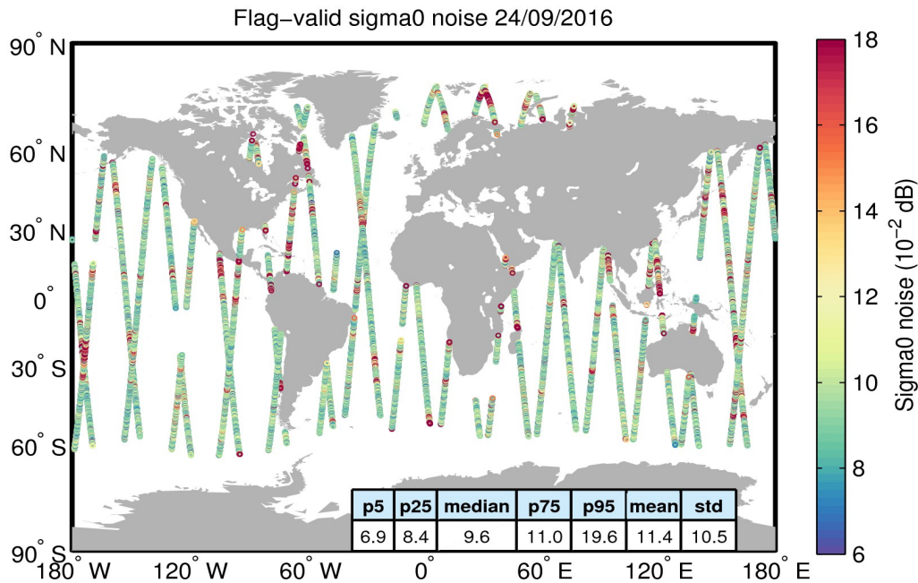
Figure 26. Geographical distribution of flag-valid 20-Hz sigma0 measurement noise over oceans and lakes for 24/09/2016. The statistical values shown in the table refer to the sigma0 noise and are calculated over all measurements shown in the figure.
