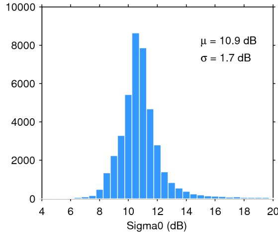
Figure 25. Histogram of flag-valid sigma0 over oceans and lakes for 24/09/2016. The mean ( \mu ) and standard deviation ( \sigma ) are also shown. Note that values outside [4 20] dB are excluded from the histogram for the sake of readability but not from the computation of \mu and \sigma .
