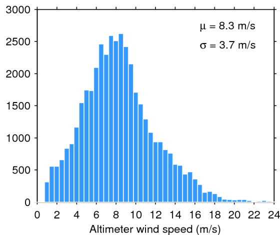
Figure 35. Histogram of science-valid wind over oceans and lakes for 24/09/2016. The mean ( \mu ) and standard deviation ( \sigma ) are also shown. Note that values larger than 24 m/s are excluded from the histogram for the sake of readability but not from the computation of \mu and \sigma .
