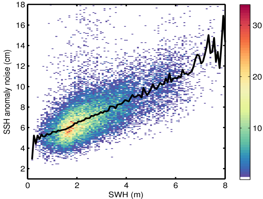
Figure 9. 2D histogram showing flag-valid SSH anomaly noise as a function of SWH for 24/09/2016. The black line denotes the median SSH anomaly noise as a function of SWH.
