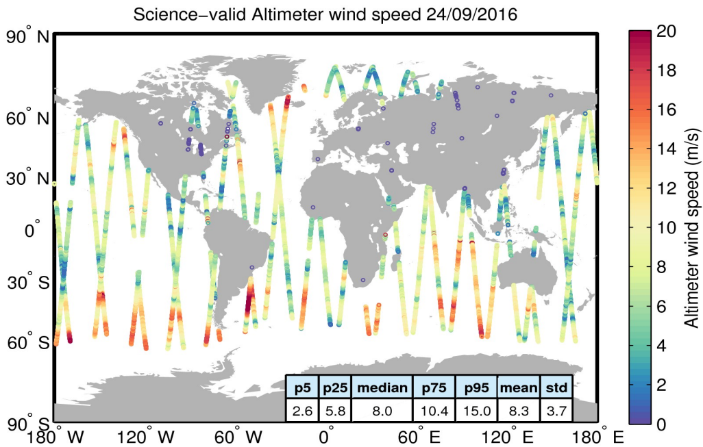
Figure 34. Geographical distribution of science-valid wind data over oceans and lakes for 24/09/2016. The statistical values shown in the table refer to the wind in m/s and are calculated over all measurements shown in the figure. Gray circles denote records that have been rejected based on the editing criteria described in Table 5.
