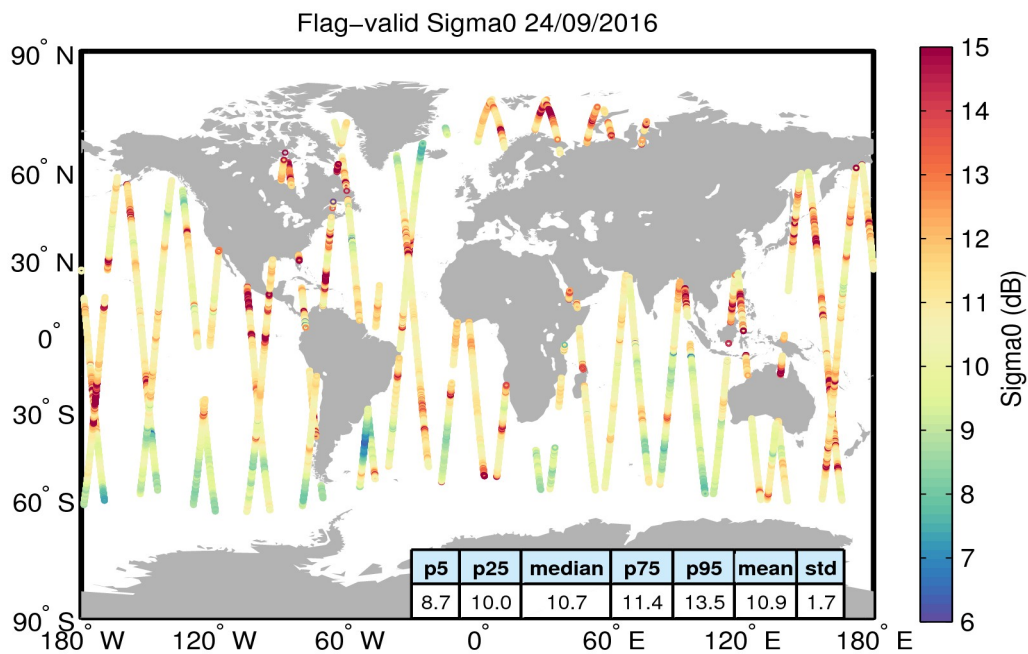
Figure 23. Geographical distribution of flag-valid sigma0 data over oceans and lakes for 24/09/2016. The statistical values shown in the table refer to the sigma0 in dB and are calculated over all measurements shown in the figure.
