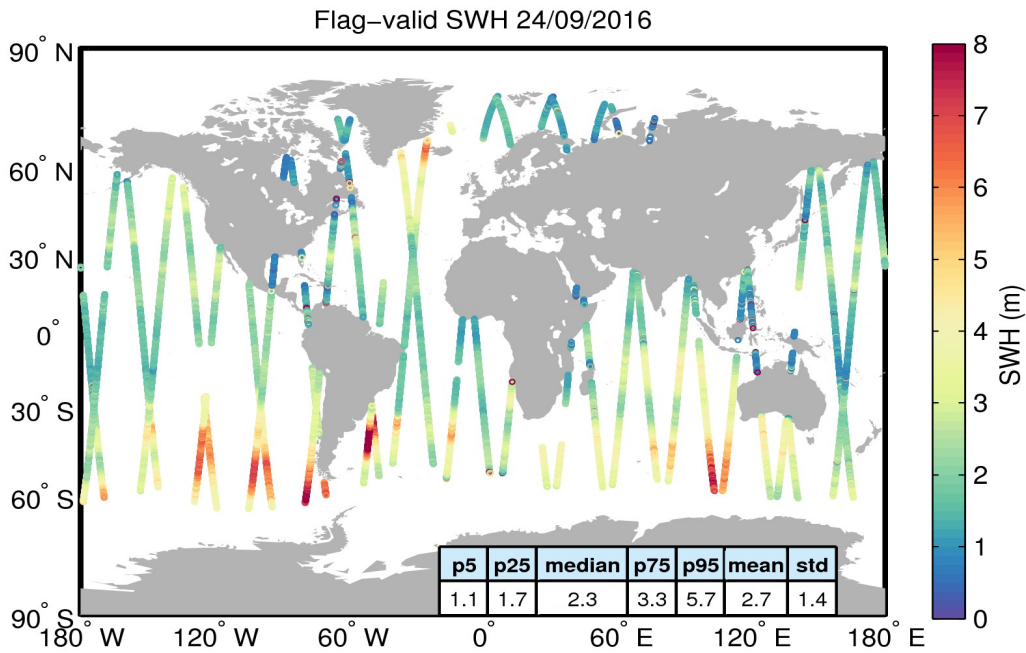
Figure 15. Geographical distribution of flag-valid SWH data over oceans and lakes for 24/09/2016. The statistical values shown in the table refer to the SWH in m and are calculated over all measurements shown in the figure.
