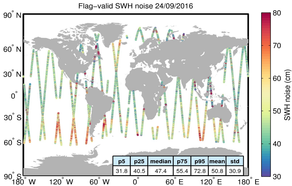
Figure 18. Geographical distribution of flag-valid 20-Hz SWH measurement noise over oceans and lakes for 24/09/2016. The statistical values shown in the table refer to the SWH noise and are calculated over all measurements shown in the figure.
