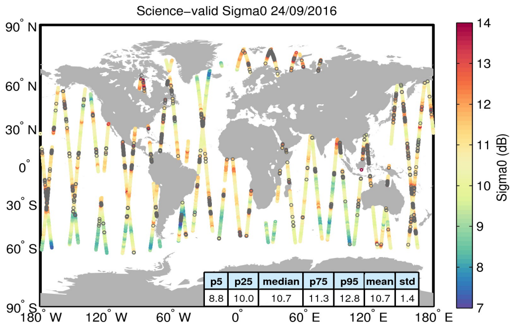
Figure 27. Geographical distribution of science-valid sigma0 data over oceans and lakes for 24/09/2016. The statistical values shown in the table refer to the sigma0 in dB and are calculated over all measurements shown in the figure. Gray circles denote records that have been rejected based on the editing criteria described in Table 4.
