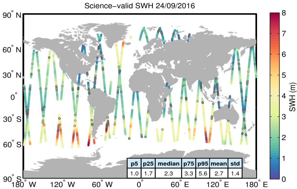
Figure 19. Geographical distribution of science-valid SWH data over oceans and lakes for 24/09/2016. The statistical values shown in the table refer to the SWH in m and are calculated over all measurements shown in the figure. Gray circles denote records that have been rejected based on the editing criteria described in Table 3.
