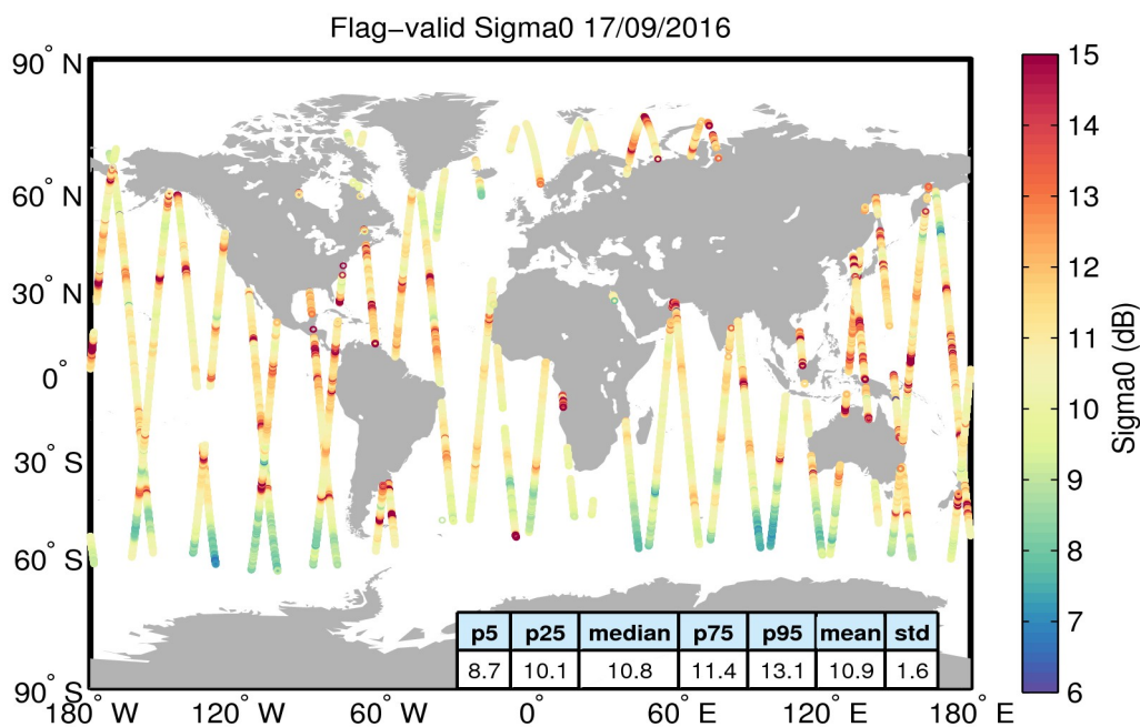
Figure 23. Geographical distribution of flag-valid sigma0 data over oceans and lakes for 17/09/2016. The statistical values shown in the table refer to the sigma0 in dB and are calculated over all measurements shown in the figure.
