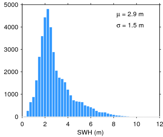
Figure 17. Histogram of flag-valid SWH over oceans and lakes for 17/09/2016. The mean ( \mu ) and standard deviation ( \sigma ) are also shown. Note that values larger than 12 m are excluded from the histogram for the sake of readability but not from the computation of \mu and \sigma .
