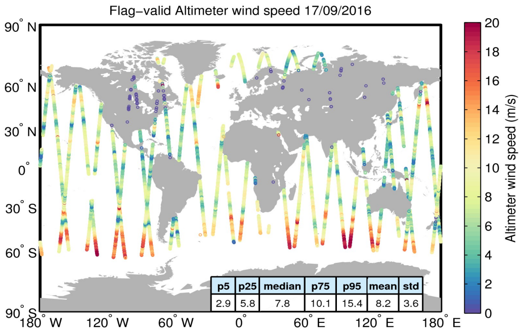
Figure 31. Geographical distribution of flag-valid wind data over oceans and lakes for 17/09/2016. The statistical values shown in the table refer to the wind in m/s and are calculated over all measurements shown in the figure.
