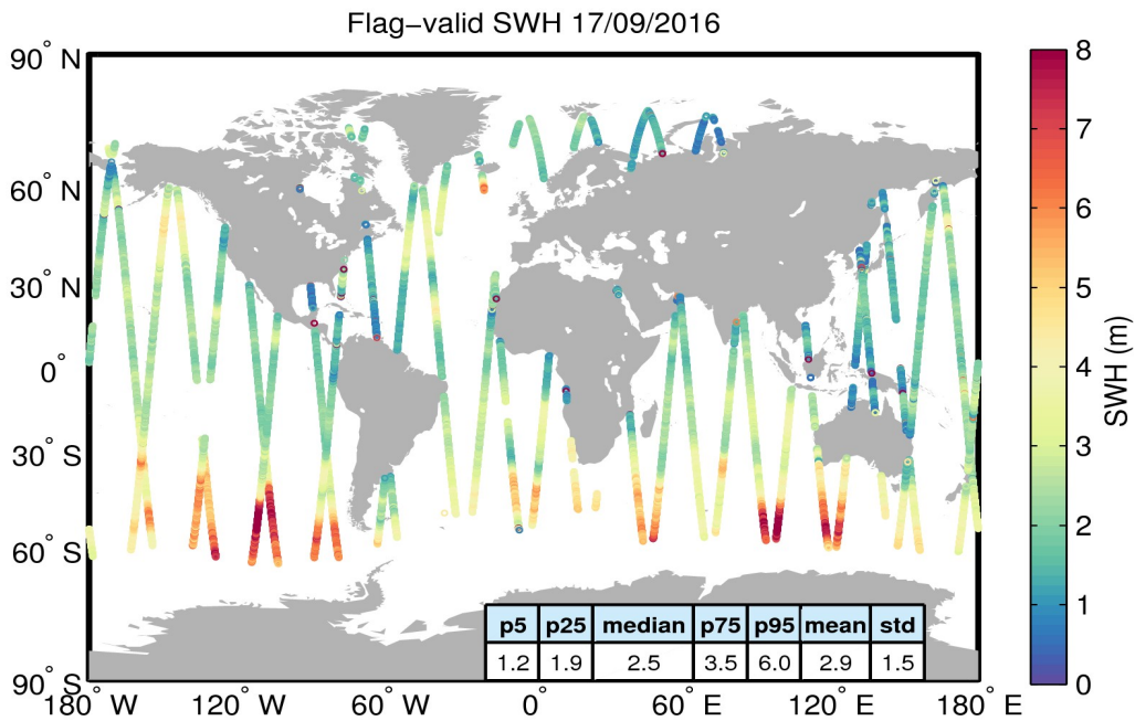
Figure 15. Geographical distribution of flag-valid SWH data over oceans and lakes for 17/09/2016. The statistical values shown in the table refer to the SWH in m and are calculated over all measurements shown in the figure.
