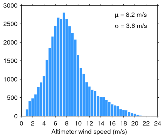
Figure 35. Histogram of science-valid wind over oceans and lakes for 17/09/2016. The mean ( \mu ) and standard deviation ( \sigma ) are also shown. Note that values larger than 24 m/s are excluded from the histogram for the sake of readability but not from the computation of \mu and \sigma .
