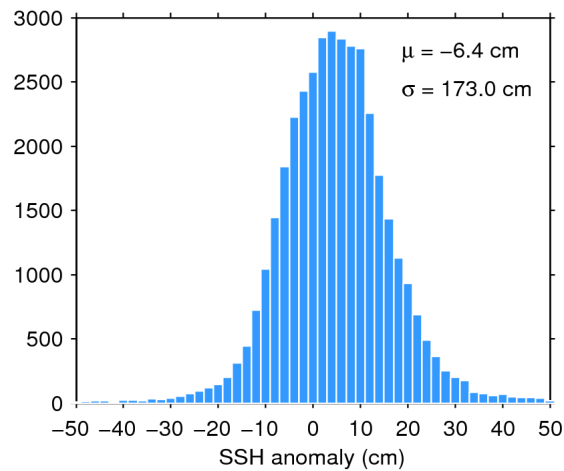
Figure 7. Histogram of flag-valid SSH anomaly over oceans and lakes for 17/09/2016. The mean ( \mu ) and standard deviation ( \sigma ) are also shown. Note that values outside [-50 50] cm are excluded from the histogram for the sake of readability but not from the computation of \mu and \sigma .
