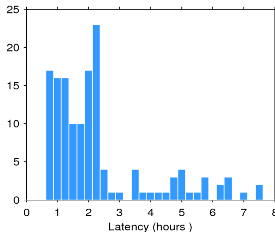
Figure 2. Histogram of the data latency for 17/09/2016. The y-axis denotes the number of files that are made available with a delay of x-hours with respect to the mean time of the records stored in the file.
