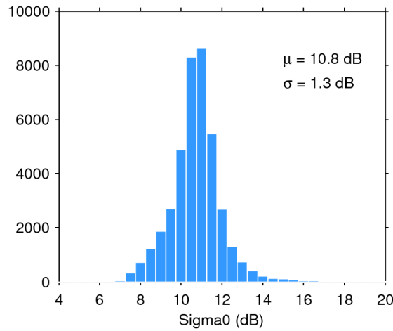
Figure 28. Histogram of science-valid sigma0 over oceans and lakes for 17/09/2016. The mean ( \mu ) and standard deviation ( \sigma ) are also shown. Note that values outside [4 20] dB are excluded from the histogram for the sake of readability but not from the computation of \mu and \sigma .
