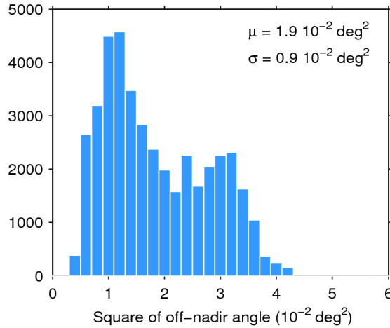
Figure 39. Histogram of flag-valid mispointing over oceans and lakes for 17/09/2016. The mean ( \mu ) and standard deviation ( \sigma ) are also shown. Note that values larger than 6 \cdot 10^{-2} \text{ deg}^2 are excluded from the histogram for the sake of readability but not from the computation of \mu and \sigma .
