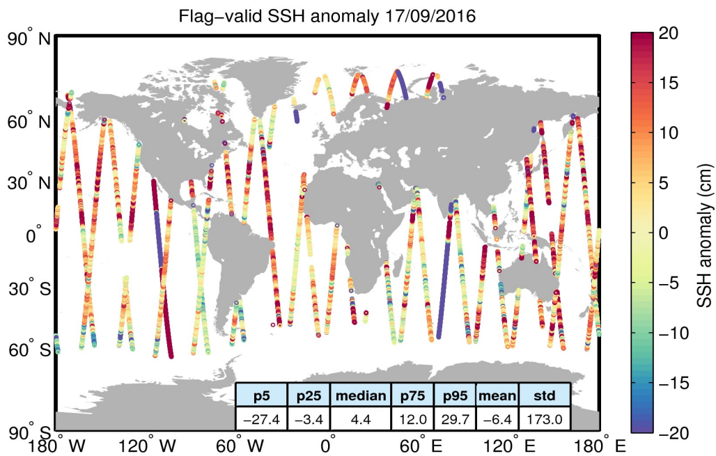
Figure 5. Geographical distribution of flag-valid 1-Hz SSH anomaly data over oceans and lakes for 17/09/2016. The statistical values shown in the table refer to the SSH anomaly in cm and are calculated over all measurements shown in the figure.
