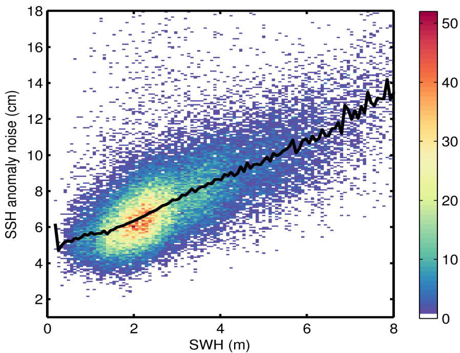
Figure 9. 2D histogram showing flag-valid SSH anomaly noise as a function of SWH for 17/09/2016. The black line denotes the median SSH anomaly noise as a function of SWH.
