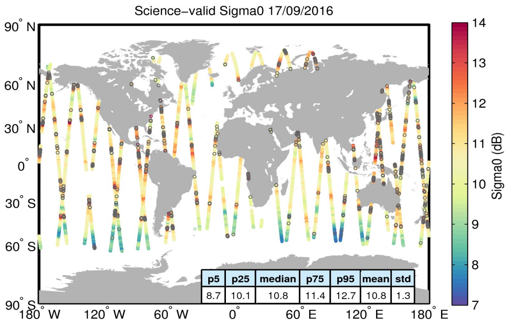
Figure 27. Geographical distribution of science-valid sigma0 data over oceans and lakes for 17/09/2016. The statistical values shown in the table refer to the sigma0 in dB and are calculated over all measurements shown in the figure. Gray circles denote records that have been rejected based on the editing criteria described in Table 4.
