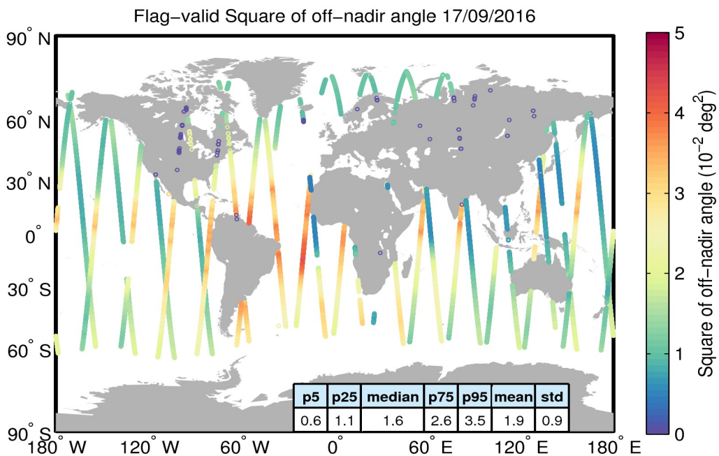
Figure 37. Geographical distribution of flag-valid mispointing data over oceans and lakes for 17/09/2016. The statistical values shown in the table refer to the mispointing in 10^{-2} \text{ deg}^2 and are calculated over all measurements shown in the figure.
