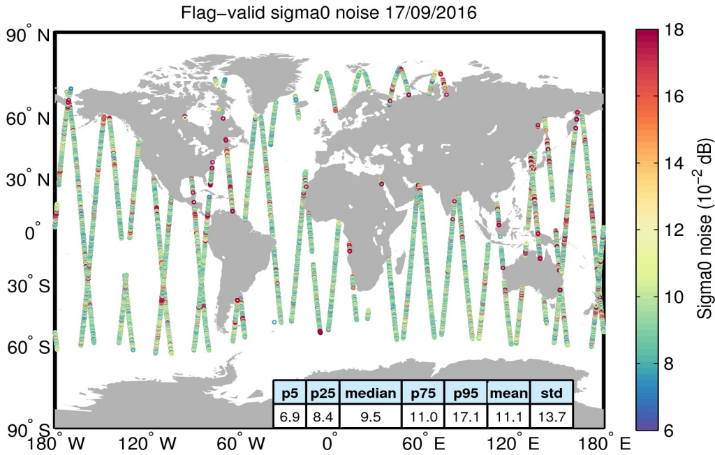
Figure 26. Geographical distribution of flag-valid 20-Hz sigma0 measurement noise over oceans and lakes for 17/09/2016. The statistical values shown in the table refer to the sigma0 noise and are calculated over all measurements shown in the figure.
