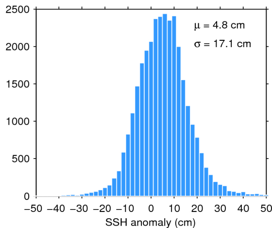
Figure 11. Histogram of science-valid SSH anomaly over oceans and lakes for 17/09/2016. The mean ( \mu ) and standard deviation ( \sigma ) are also shown. Note that values outside [-50 50] cm are excluded from the histogram for the sake of readability but not from the computation of \mu and \sigma .
