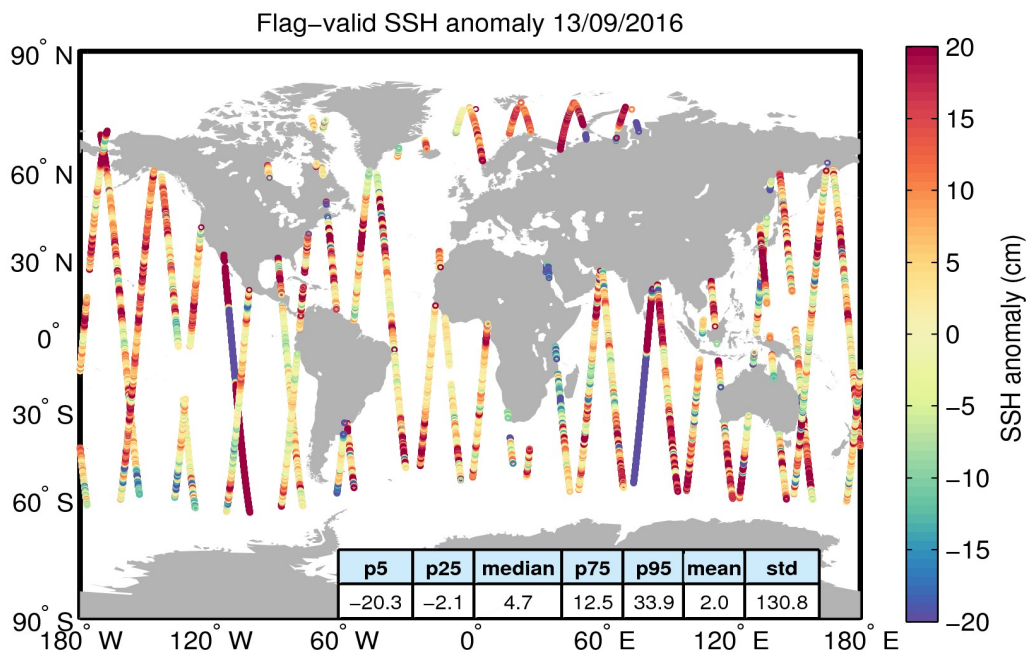
Figure 5. Geographical distribution of flag-valid 1-Hz SSH anomaly data over oceans and lakes for 13/09/2016. The statistical values shown in the table refer to the SSH anomaly in cm and are calculated over all measurements shown in the figure.
