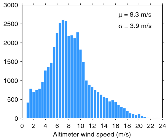
Figure 33. Histogram of flag-valid wind over oceans and lakes for 13/09/2016. The mean ( \mu ) and standard deviation ( \sigma ) are also shown. Note that values larger than 24 m/s are excluded from the histogram for the sake of readability but not from the computation of \mu and \sigma .
