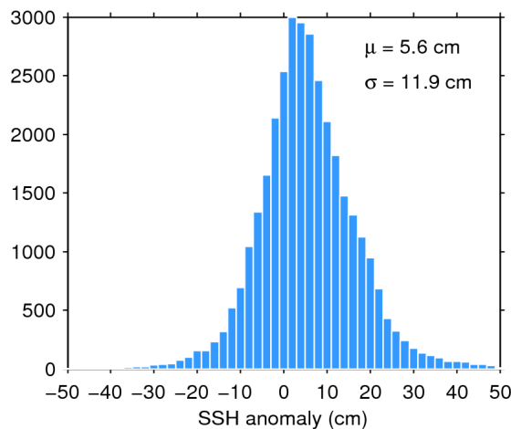
Figure 11. Histogram of science-valid SSH anomaly over oceans and lakes for 13/09/2016. The mean ( \mu ) and standard deviation ( \sigma ) are also shown. Note that values outside [-50 50] cm are excluded from the histogram for the sake of readability but not from the computation of \mu and \sigma .
