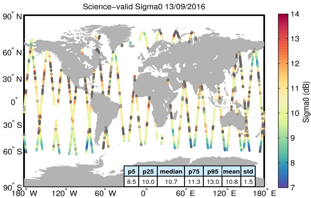
Figure 27. Geographical distribution of science-valid sigma0 data over oceans and lakes for 13/09/2016. The statistical values shown in the table refer to the sigma0 in dB and are calculated over all measurements shown in the figure. Gray circles denote records that have been rejected based on the editing criteria described in Table 4.
