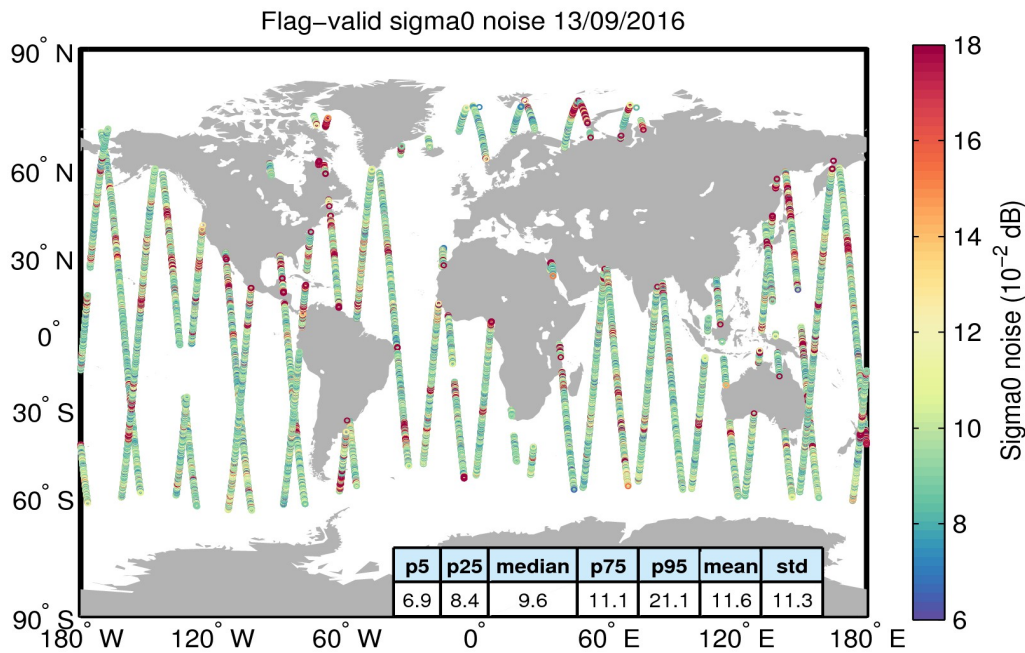
Figure 26. Geographical distribution of flag-valid 20-Hz sigma0 measurement noise over oceans and lakes for 13/09/2016. The statistical values shown in the table refer to the sigma0 noise and are calculated over all measurements shown in the figure.
