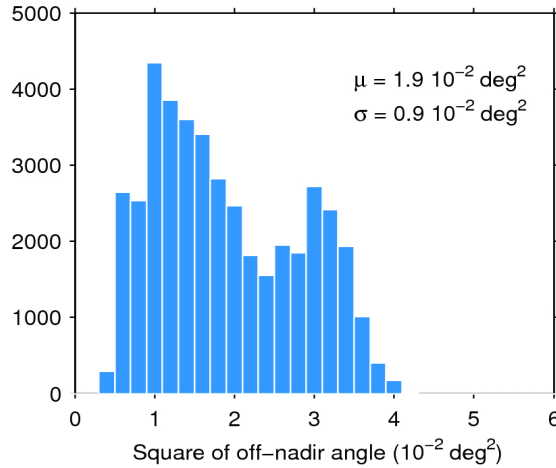
Figure 39. Histogram of flag-valid mispointing over oceans and lakes for 13/09/2016. The mean ( \mu ) and standard deviation ( \sigma ) are also shown. Note that values larger than 6 \cdot 10^{-2} \text{ deg}^2 are excluded from the histogram for the sake of readability but not from the computation of \mu and \sigma .
