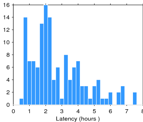
Figure 2. Histogram of the data latency for 13/09/2016. The y-axis denotes the number of files that are made available with a delay of x-hours with respect to the mean time of the records stored in the file.
