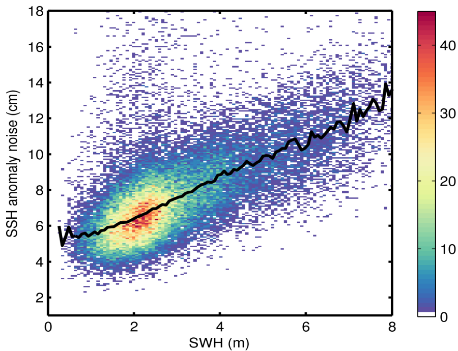
Figure 9. 2D histogram showing flag-valid SSH anomaly noise as a function of SWH for 13/09/2016. The black line denotes the median SSH anomaly noise as a function of SWH.
