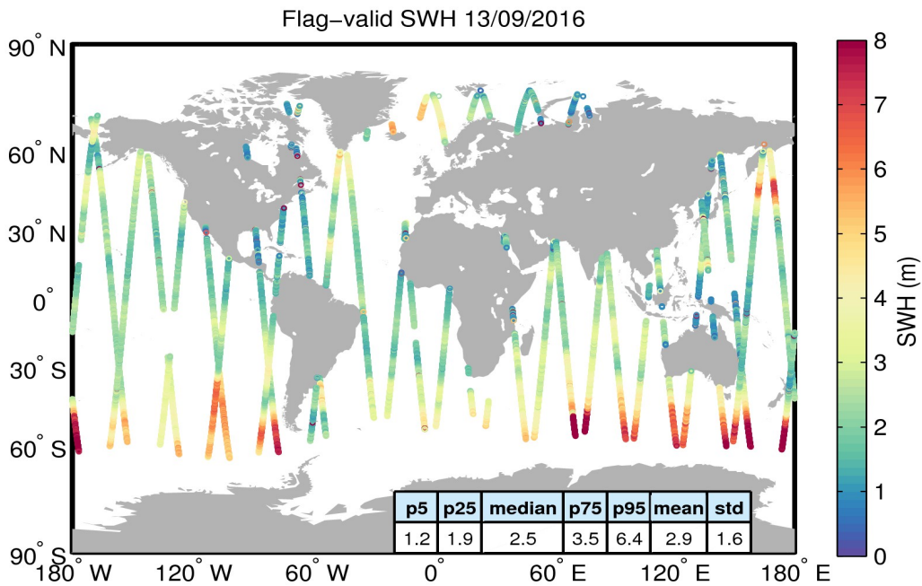
Figure 15. Geographical distribution of flag-valid SWH data over oceans and lakes for 13/09/2016. The statistical values shown in the table refer to the SWH in m and are calculated over all measurements shown in the figure.
