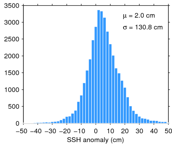
Figure 7. Histogram of flag-valid SSH anomaly over oceans and lakes for 13/09/2016. The mean ( \mu ) and standard deviation ( \sigma ) are also shown. Note that values outside [-50 50] cm are excluded from the histogram for the sake of readability but not from the computation of \mu and \sigma .
