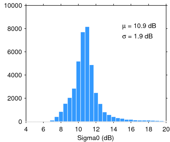
Figure 25. Histogram of flag-valid sigma0 over oceans and lakes for 13/09/2016. The mean ( \mu ) and standard deviation ( \sigma ) are also shown. Note that values outside [4 20] dB are excluded from the histogram for the sake of readability but not from the computation of \mu and \sigma .
