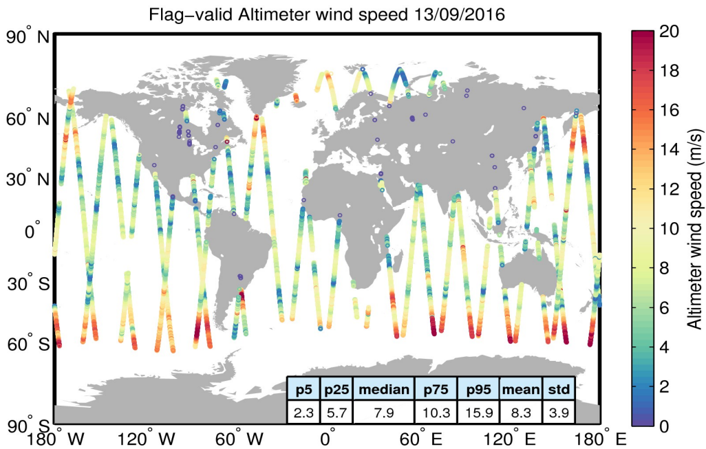
Figure 31. Geographical distribution of flag-valid wind data over oceans and lakes for 13/09/2016. The statistical values shown in the table refer to the wind in m/s and are calculated over all measurements shown in the figure.
