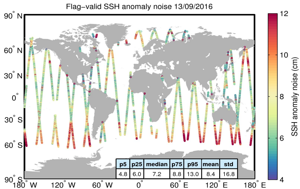
Figure 8. Geographical distribution of flag-valid 20-Hz SSH anomaly measurement noise over oceans and lakes for 13/09/2016. The statistical values shown in the table refer to the SSH anomaly noise and are calculated over all measurements shown in the figure.
