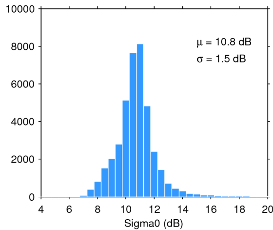
Figure 28. Histogram of science-valid sigma0 over oceans and lakes for 13/09/2016. The mean ( \mu ) and standard deviation ( \sigma ) are also shown. Note that values outside [4 20] dB are excluded from the histogram for the sake of readability but not from the computation of \mu and \sigma .
