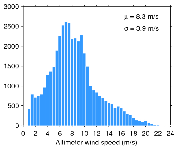
Figure 35. Histogram of science-valid wind over oceans and lakes for 13/09/2016. The mean ( \mu ) and standard deviation ( \sigma ) are also shown. Note that values larger than 24 m/s are excluded from the histogram for the sake of readability but not from the computation of \mu and \sigma .
