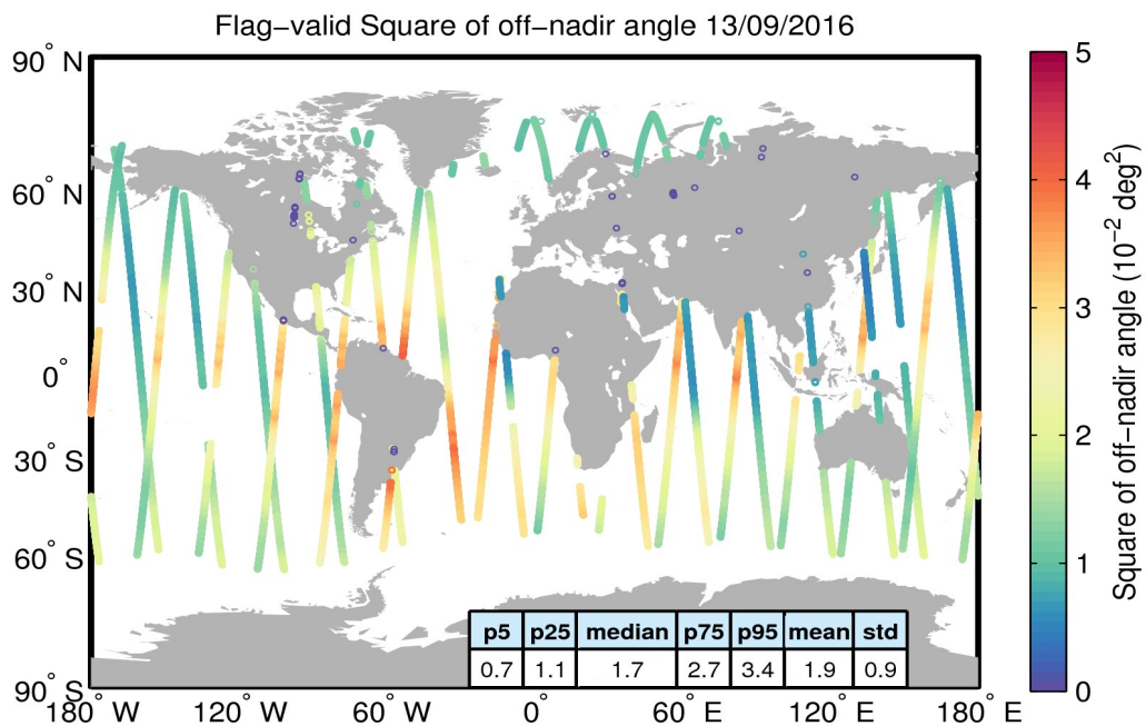
Figure 37. Geographical distribution of flag-valid mispointing data over oceans and lakes for 13/09/2016. The statistical values shown in the table refer to the mispointing in 10^{-2} deg 2 and are calculated over all measurements shown in the figure.
