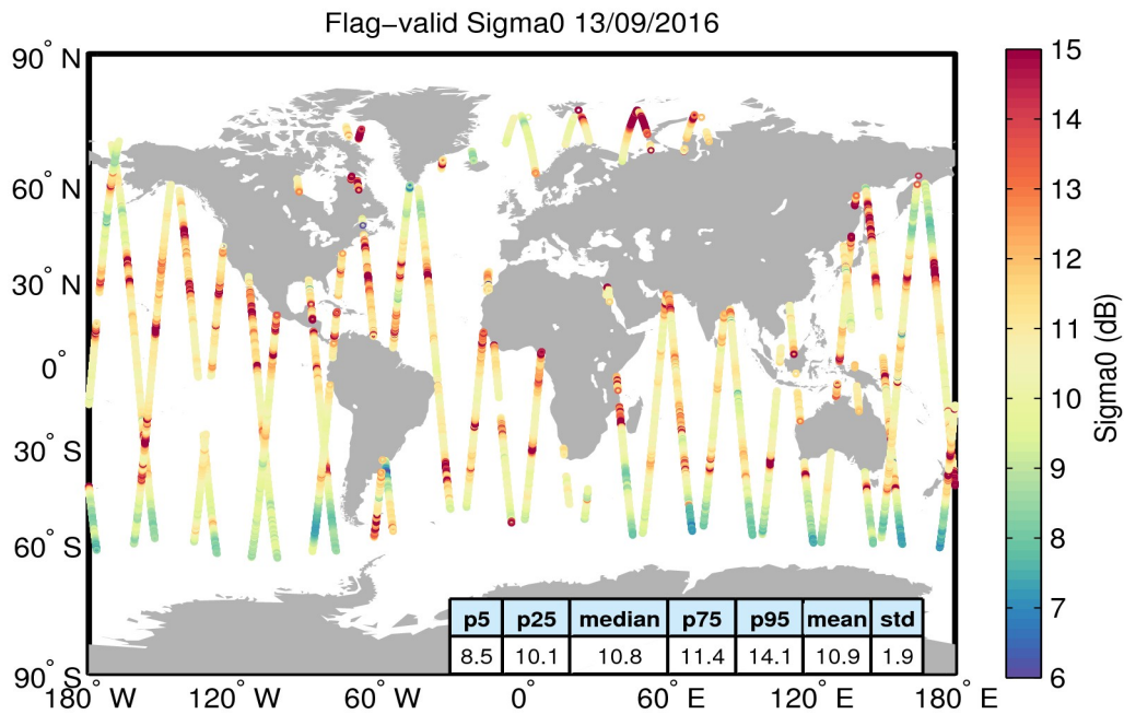
Figure 23. Geographical distribution of flag-valid sigma0 data over oceans and lakes for 13/09/2016. The statistical values shown in the table refer to the sigma0 in dB and are calculated over all measurements shown in the figure.
