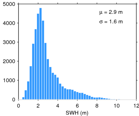
Figure 20. Histogram of science-valid SWH over oceans and lakes for 13/09/2016. The mean ( \mu ) and standard deviation ( \sigma ) are also shown. Note that values larger than 12 m are excluded from the histogram for the sake of readability but not from the computation of \mu and \sigma .
