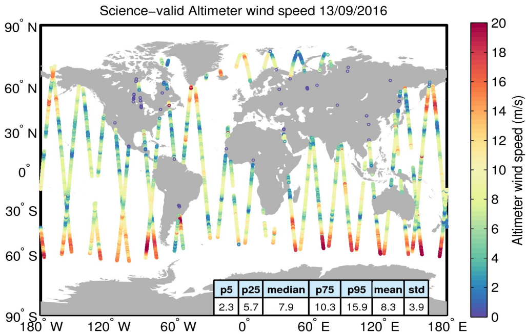
Figure 34. Geographical distribution of science-valid wind data over oceans and lakes for 13/09/2016. The statistical values shown in the table refer to the wind in m/s and are calculated over all measurements shown in the figure. Gray circles denote records that have been rejected based on the editing criteria described in Table 5.
