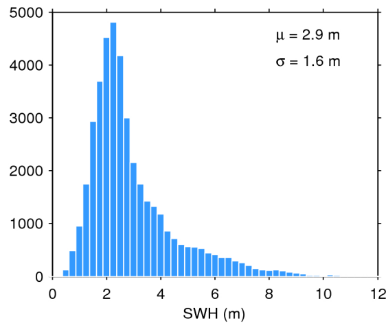
Figure 17. Histogram of flag-valid SWH over oceans and lakes for 13/09/2016. The mean ( \mu ) and standard deviation ( \sigma ) are also shown. Note that values larger than 12 m are excluded from the histogram for the sake of readability but not from the computation of \mu and \sigma .
