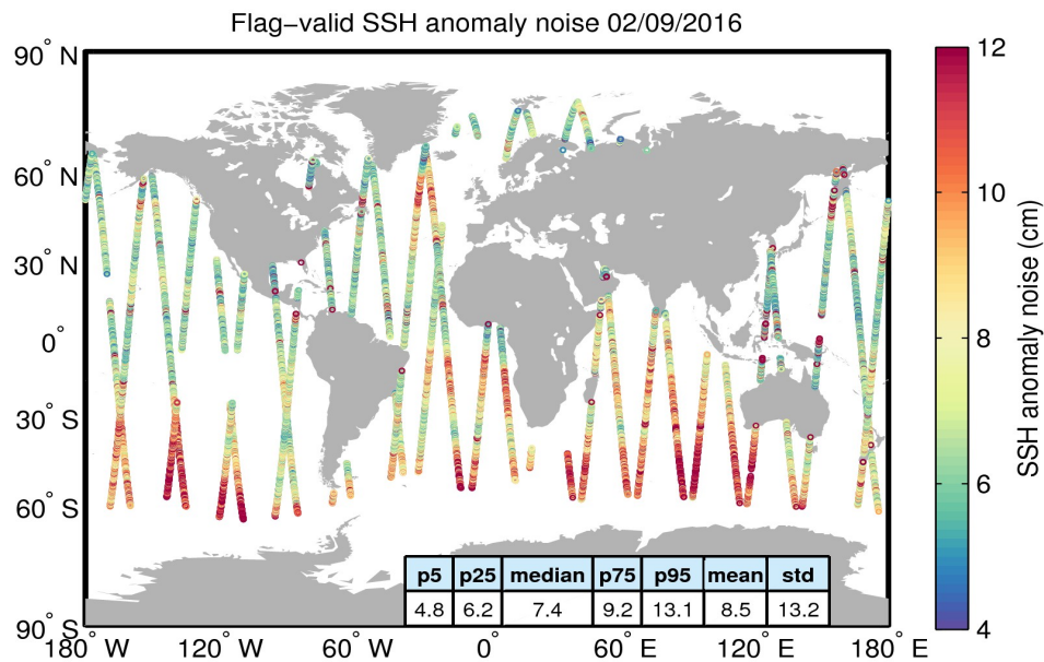
Figure 8. Geographical distribution of flag-valid 20-Hz SSH anomaly measurement noise over oceans and lakes for 02/09/2016. The statistical values shown in the table refer to the SSH anomaly noise and are calculated over all measurements shown in the figure.
