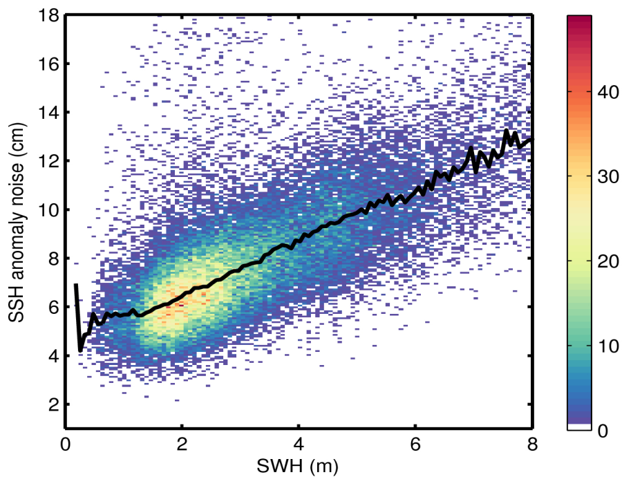
Figure 9. 2D histogram showing flag-valid SSH anomaly noise as a function of SWH for 02/09/2016. The black line denotes the median SSH anomaly noise as a function of SWH.
