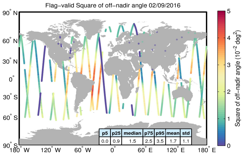
Figure 37. Geographical distribution of flag-valid mispointing data over oceans and lakes for 02/09/2016. The statistical values shown in the table refer to the mispointing in 10^{-2} deg 2 and are calculated over all measurements shown in the figure.
