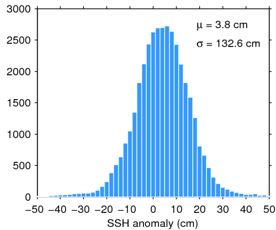
Figure 7. Histogram of flag-valid SSH anomaly over oceans and lakes for 02/09/2016. The mean ( \mu ) and standard deviation ( \sigma ) are also shown. Note that values outside [-50 50] cm are excluded from the histogram for the sake of readability but not from the computation of \mu and \sigma .
