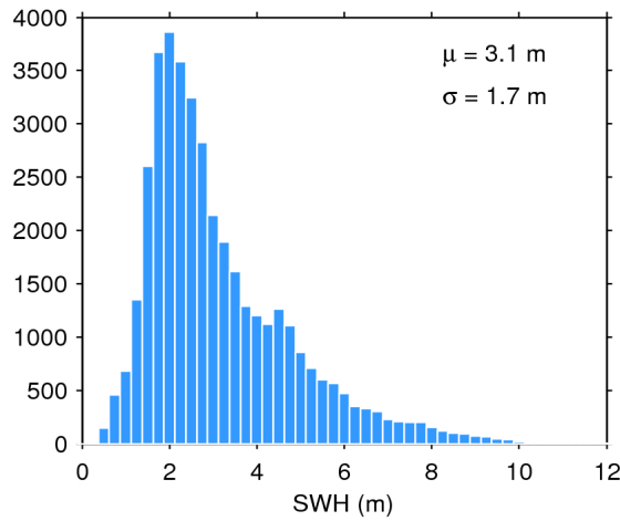
Figure 17. Histogram of flag-valid SWH over oceans and lakes for 02/09/2016. The mean ( \mu ) and standard deviation ( \sigma ) are also shown. Note that values larger than 12 m are excluded from the histogram for the sake of readability but not from the computation of \mu and \sigma .
