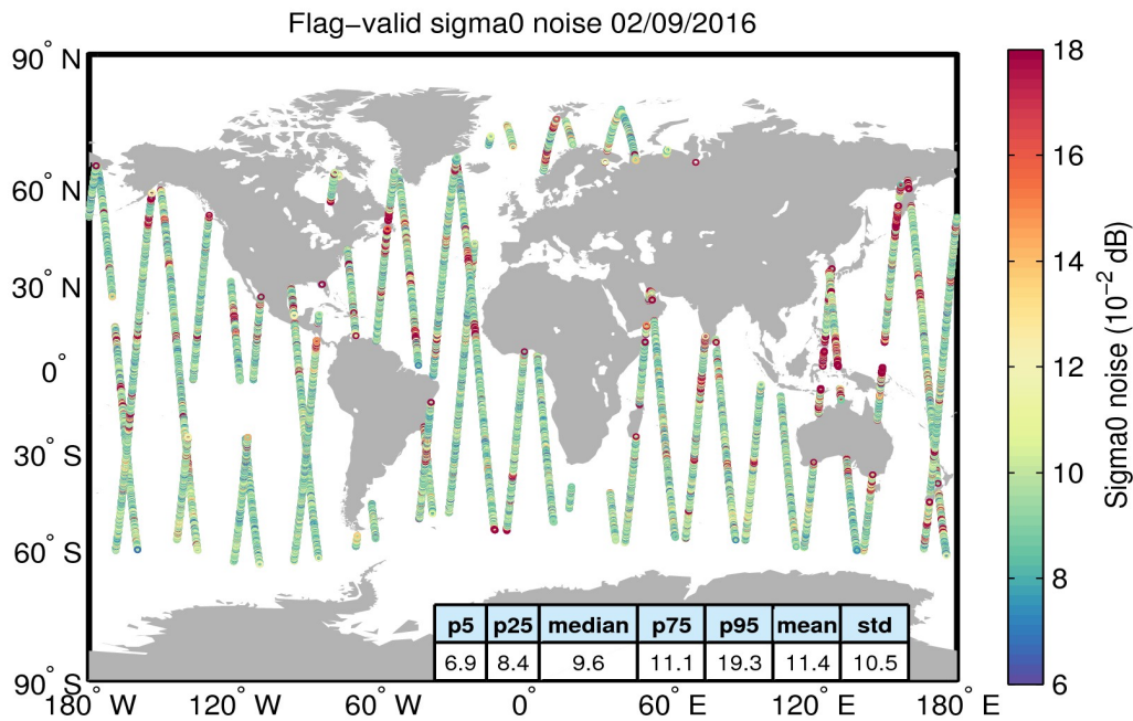
Figure 26. Geographical distribution of flag-valid 20-Hz sigma0 measurement noise over oceans and lakes for 02/09/2016. The statistical values shown in the table refer to the sigma0 noise and are calculated over all measurements shown in the figure.
