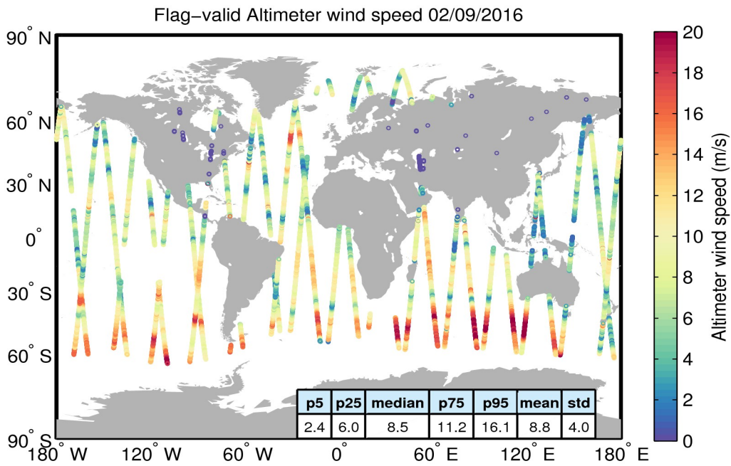
Figure 31. Geographical distribution of flag-valid wind data over oceans and lakes for 02/09/2016. The statistical values shown in the table refer to the wind in m/s and are calculated over all measurements shown in the figure.
