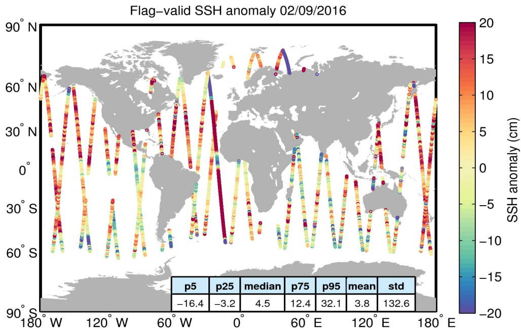
Figure 5. Geographical distribution of flag-valid 1-Hz SSH anomaly data over oceans and lakes for 02/09/2016. The statistical values shown in the table refer to the SSH anomaly in cm and are calculated over all measurements shown in the figure.
