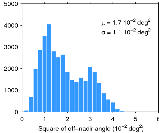
Figure 39. Histogram of flag-valid mispointing over oceans and lakes for 02/09/2016. The mean ( \mu ) and standard deviation ( \sigma ) are also shown. Note that values larger than 6 \cdot 10^{-2} \text{ deg}^2 are excluded from the histogram for the sake of readability but not from the computation of \mu and \sigma .
