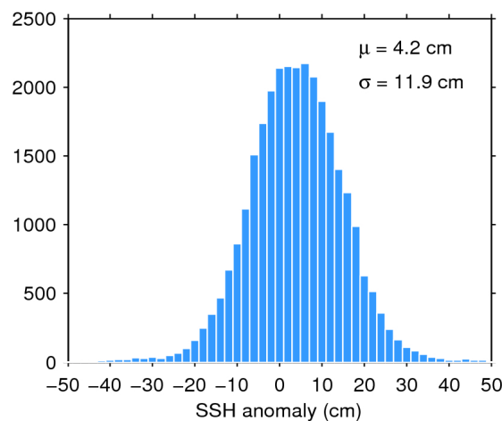
Figure 11. Histogram of science-valid SSH anomaly over oceans and lakes for 02/09/2016. The mean ( \mu ) and standard deviation ( \sigma ) are also shown. Note that values outside [-50 50] cm are excluded from the histogram for the sake of readability but not from the computation of \mu and \sigma .
