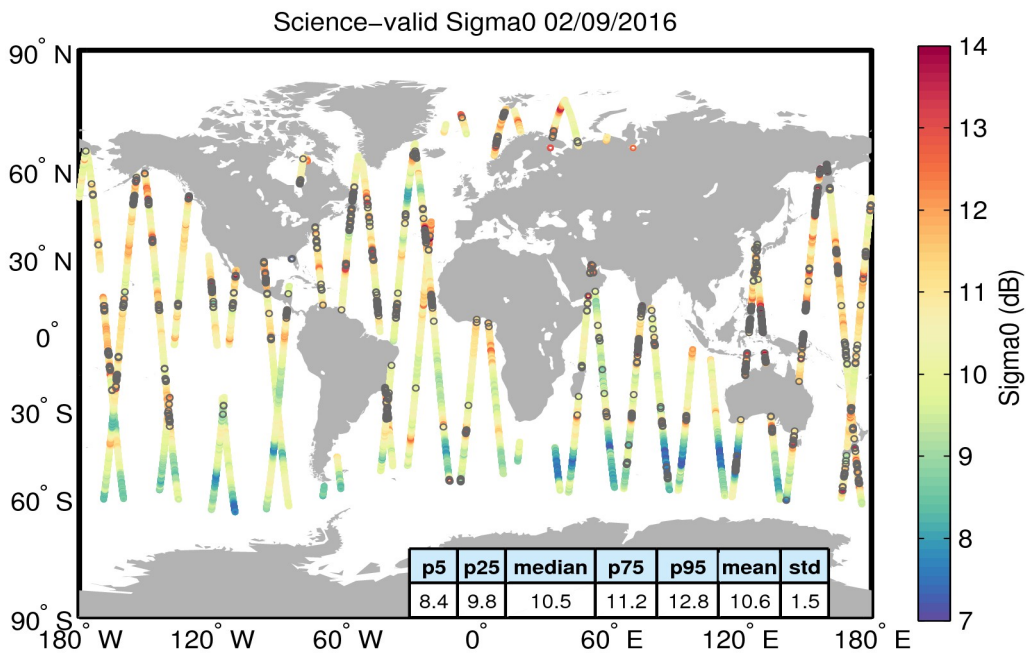
Figure 27. Geographical distribution of science-valid sigma0 data over oceans and lakes for 02/09/2016. The statistical values shown in the table refer to the sigma0 in dB and are calculated over all measurements shown in the figure. Gray circles denote records that have been rejected based on the editing criteria described in Table 4.
