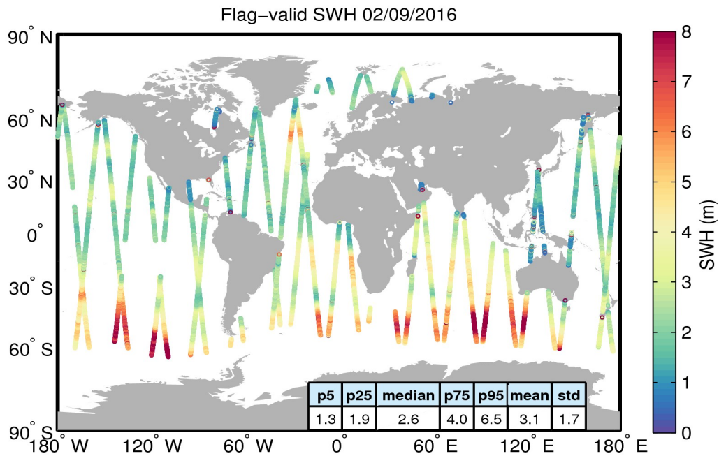
Figure 15. Geographical distribution of flag-valid SWH data over oceans and lakes for 02/09/2016. The statistical values shown in the table refer to the SWH in m and are calculated over all measurements shown in the figure.
