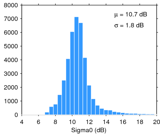
Figure 25. Histogram of flag-valid sigma0 over oceans and lakes for 02/09/2016. The mean ( \mu ) and standard deviation ( \sigma ) are also shown. Note that values outside [4 20] dB are excluded from the histogram for the sake of readability but not from the computation of \mu and \sigma .
