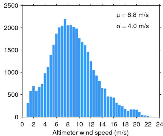
Figure 35. Histogram of science-valid wind over oceans and lakes for 02/09/2016. The mean ( \mu ) and standard deviation ( \sigma ) are also shown. Note that values larger than 24 m/s are excluded from the histogram for the sake of readability but not from the computation of \mu and \sigma .
