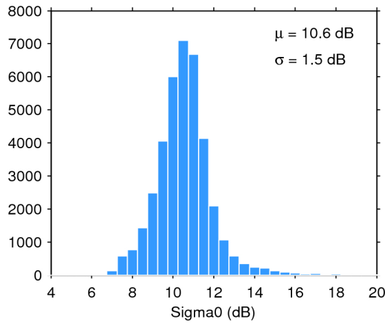
Figure 28. Histogram of science-valid sigma0 over oceans and lakes for 02/09/2016. The mean ( \mu ) and standard deviation ( \sigma ) are also shown. Note that values outside [4 20] dB are excluded from the histogram for the sake of readability but not from the computation of \mu and \sigma .
