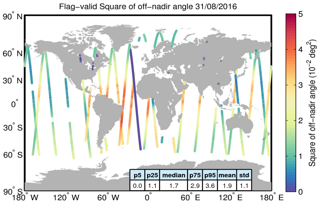
Figure 37. Geographical distribution of flag-valid mispointing data over oceans and lakes for 31/08/2016. The statistical values shown in the table refer to the mispointing in 10^{-2} \text{deg}^2 and are calculated over all measurements shown in the figure.
