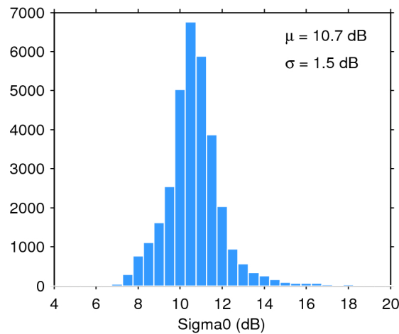
Figure 28. Histogram of science-valid sigma0 over oceans and lakes for 31/08/2016. The mean ( \mu ) and standard deviation ( \sigma ) are also shown. Note that values outside [4 20] dB are excluded from the histogram for the sake of readability but not from the computation of \mu and \sigma .
