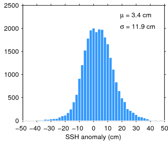
Figure 11. Histogram of science-valid SSH anomaly over oceans and lakes for 31/08/2016. The mean ( \mu ) and standard deviation ( \sigma ) are also shown. Note that values outside [-50 50] cm are excluded from the histogram for the sake of readability but not from the computation of \mu and \sigma .
