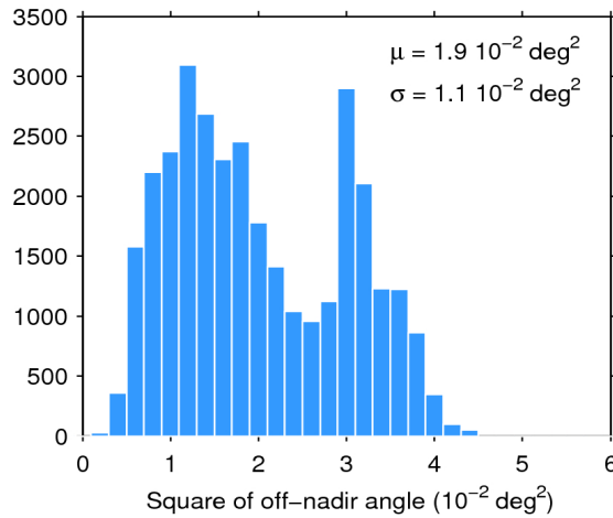
Figure 39. Histogram of flag-valid mispointing over oceans and lakes for 31/08/2016. The mean ( \mu ) and standard deviation ( \sigma ) are also shown. Note that values larger than 6 \cdot 10^{-2} \text{ deg}^2 are excluded from the histogram for the sake of readability but not from the computation of \mu and \sigma .
