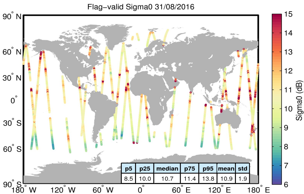
Figure 23. Geographical distribution of flag-valid sigma0 data over oceans and lakes for 31/08/2016. The statistical values shown in the table refer to the sigma0 in dB and are calculated over all measurements shown in the figure.
