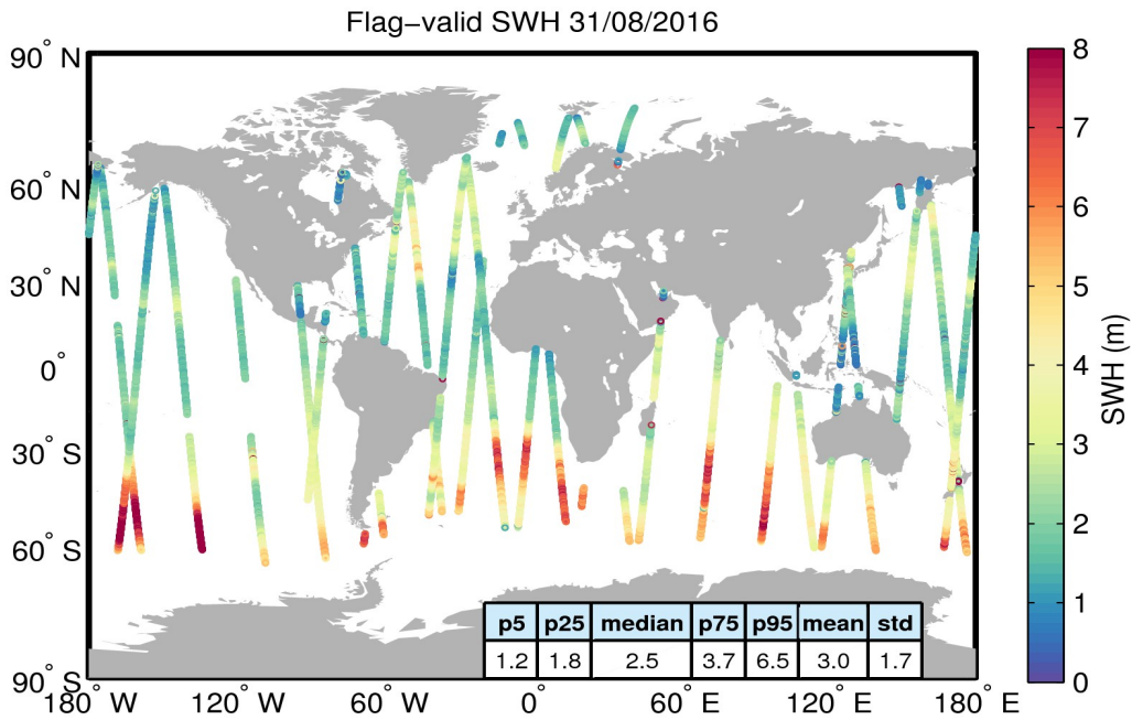
Figure 15. Geographical distribution of flag-valid SWH data over oceans and lakes for 31/08/2016. The statistical values shown in the table refer to the SWH in m and are calculated over all measurements shown in the figure.
