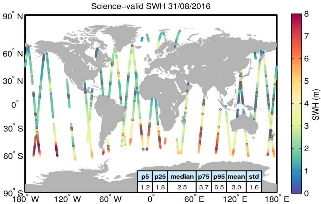
Figure 19. Geographical distribution of science-valid SWH data over oceans and lakes for 31/08/2016. The statistical values shown in the table refer to the SWH in m and are calculated over all measurements shown in the figure. Gray circles denote records that have been rejected based on the editing criteria described in Table 3.
