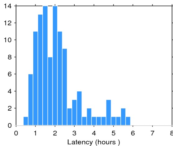
Figure 2. Histogram of the data latency for 31/08/2016. The y-axis denotes the number of files that are made available with a delay of x-hours with respect to the mean time of the records stored in the file.
