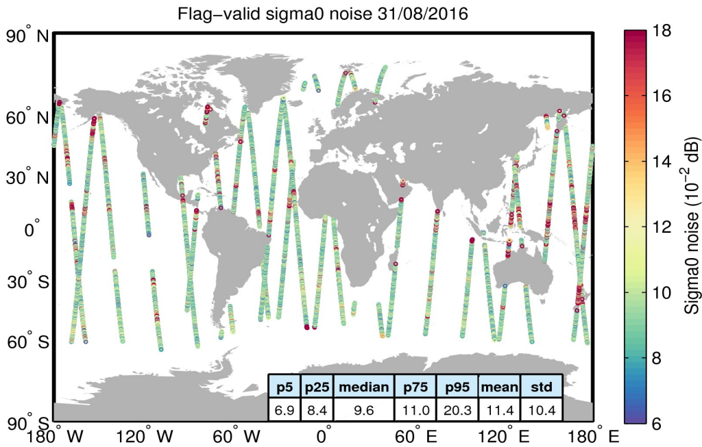
Figure 26. Geographical distribution of flag-valid 20-Hz sigma0 measurement noise over oceans and lakes for 31/08/2016. The statistical values shown in the table refer to the sigma0 noise and are calculated over all measurements shown in the figure.
