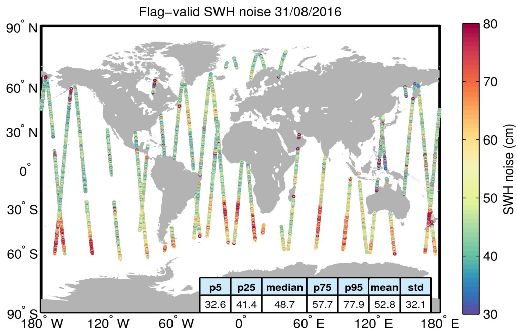
Figure 18. Geographical distribution of flag-valid 20-Hz SWH measurement noise over oceans and lakes for 31/08/2016. The statistical values shown in the table refer to the SWH noise and are calculated over all measurements shown in the figure.
