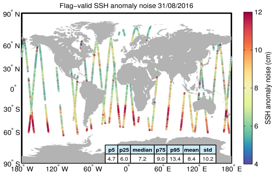
Figure 8. Geographical distribution of flag-valid 20-Hz SSH anomaly measurement noise over oceans and lakes for 31/08/2016. The statistical values shown in the table refer to the SSH anomaly noise and are calculated over all measurements shown in the figure.
