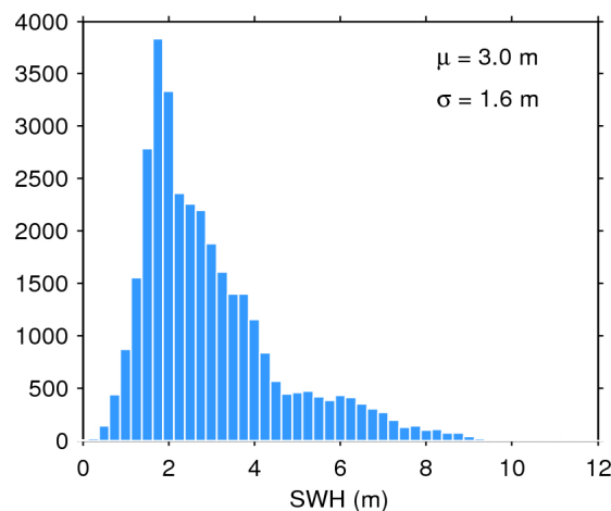
Figure 20. Histogram of science-valid SWH over oceans and lakes for 31/08/2016. The mean ( \mu ) and standard deviation ( \sigma ) are also shown. Note that values larger than 12 m are excluded from the histogram for the sake of readability but not from the computation of \mu and \sigma .
