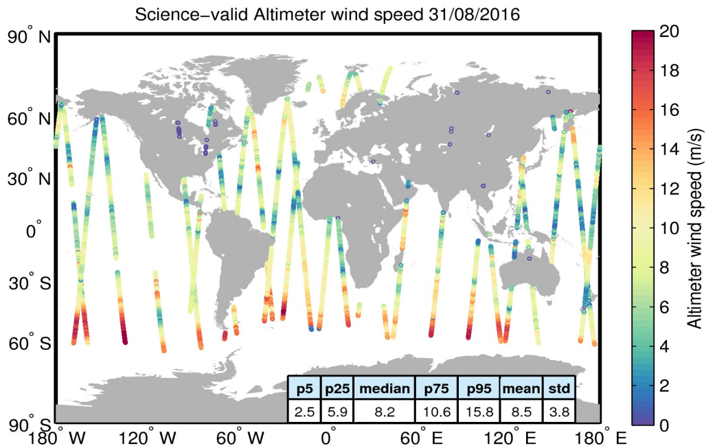
Figure 34. Geographical distribution of science-valid wind data over oceans and lakes for 31/08/2016. The statistical values shown in the table refer to the wind in m/s and are calculated over all measurements shown in the figure. Gray circles denote records that have been rejected based on the editing criteria described in Table 5.
