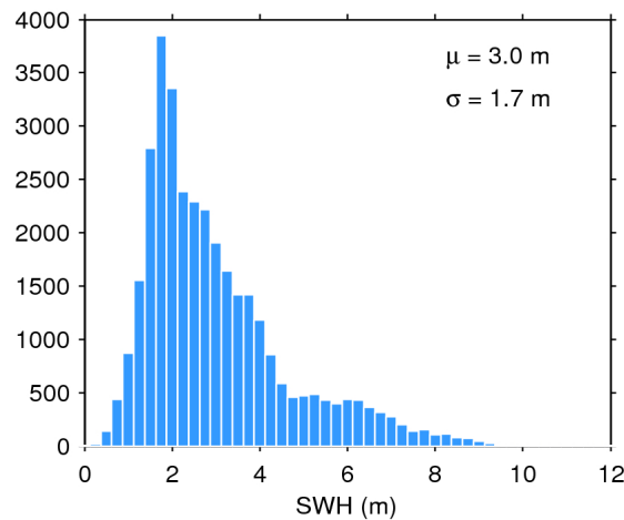
Figure 17. Histogram of flag-valid SWH over oceans and lakes for 31/08/2016. The mean ( \mu ) and standard deviation ( \sigma ) are also shown. Note that values larger than 12 m are excluded from the histogram for the sake of readability but not from the computation of \mu and \sigma .
