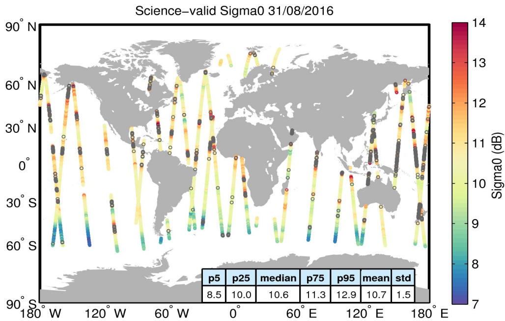
Figure 27. Geographical distribution of science-valid sigma0 data over oceans and lakes for 31/08/2016. The statistical values shown in the table refer to the sigma0 in dB and are calculated over all measurements shown in the figure. Gray circles denote records that have been rejected based on the editing criteria described in Table 4.
