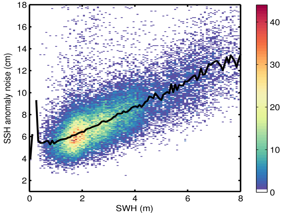
Figure 9. 2D histogram showing flag-valid SSH anomaly noise as a function of SWH for 31/08/2016. The black line denotes the median SSH anomaly noise as a function of SWH.
