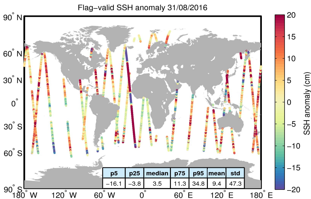
Figure 5. Geographical distribution of flag-valid 1-Hz SSH anomaly data over oceans and lakes for 31/08/2016. The statistical values shown in the table refer to the SSH anomaly in cm and are calculated over all measurements shown in the figure.
