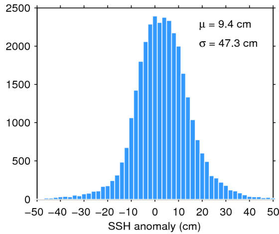
Figure 7. Histogram of flag-valid SSH anomaly over oceans and lakes for 31/08/2016. The mean ( \mu ) and standard deviation ( \sigma ) are also shown. Note that values outside [-50 50] cm are excluded from the histogram for the sake of readability but not from the computation of \mu and \sigma .
