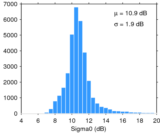
Figure 25. Histogram of flag-valid sigma0 over oceans and lakes for 31/08/2016. The mean ( \mu ) and standard deviation ( \sigma ) are also shown. Note that values outside [4 20] dB are excluded from the histogram for the sake of readability but not from the computation of \mu and \sigma .
