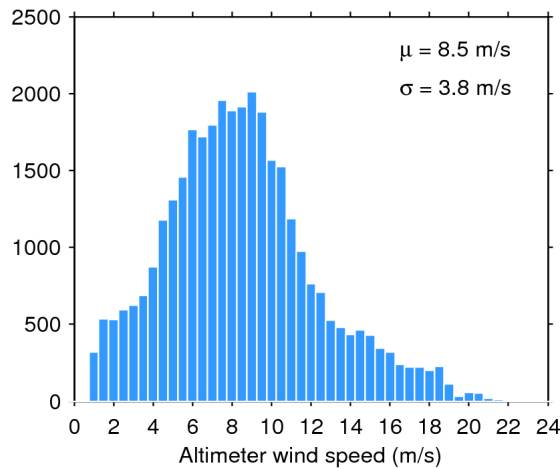
Figure 33. Histogram of flag-valid wind over oceans and lakes for 31/08/2016. The mean ( \mu ) and standard deviation ( \sigma ) are also shown. Note that values larger than 24 m/s are excluded from the histogram for the sake of readability but not from the computation of \mu and \sigma .
