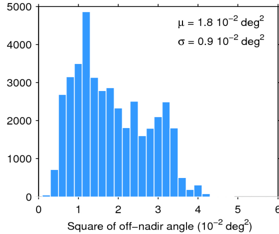
Figure 39. Histogram of flag-valid mispointing over oceans and lakes for 30/08/2016. The mean ( \mu ) and standard deviation ( \sigma ) are also shown. Note that values larger than 6 \cdot 10^{-2} \text{ deg}^2 are excluded from the histogram for the sake of readability but not from the computation of \mu and \sigma .
