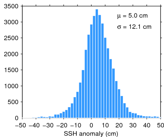
Figure 11. Histogram of science-valid SSH anomaly over oceans and lakes for 30/08/2016. The mean ( \mu ) and standard deviation ( \sigma ) are also shown. Note that values outside [-50 50] cm are excluded from the histogram for the sake of readability but not from the computation of \mu and \sigma .
