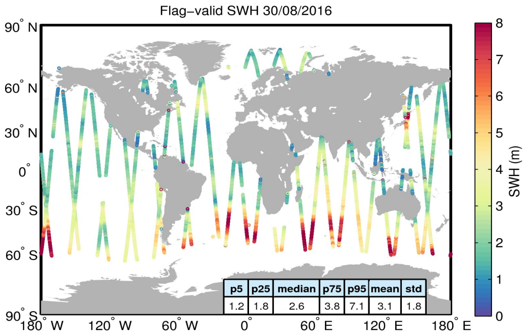
Figure 15. Geographical distribution of flag-valid SWH data over oceans and lakes for 30/08/2016. The statistical values shown in the table refer to the SWH in m and are calculated over all measurements shown in the figure.
