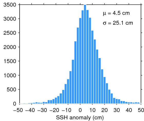
Figure 7. Histogram of flag-valid SSH anomaly over oceans and lakes for 30/08/2016. The mean ( \mu ) and standard deviation ( \sigma ) are also shown. Note that values outside [-50\ 50] cm are excluded from the histogram for the sake of readability but not from the computation of \mu and \sigma .
