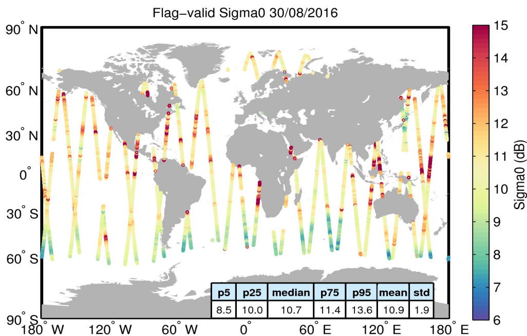
Figure 23. Geographical distribution of flag-valid sigma0 data over oceans and lakes for 30/08/2016. The statistical values shown in the table refer to the sigma0 in dB and are calculated over all measurements shown in the figure.
