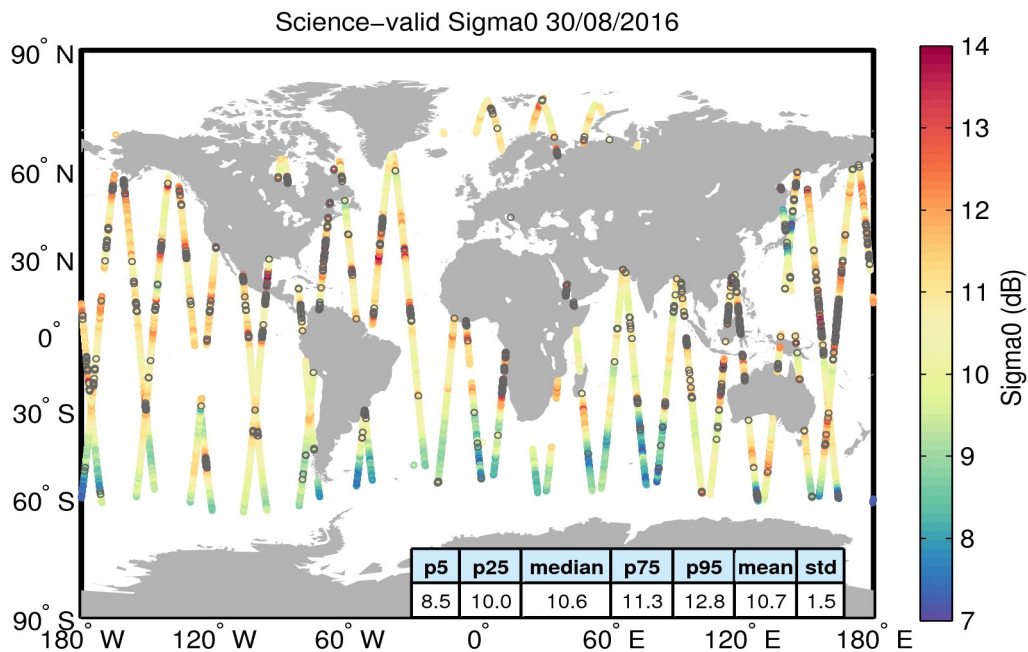
Figure 27. Geographical distribution of science-valid sigma0 data over oceans and lakes for 30/08/2016. The statistical values shown in the table refer to the sigma0 in dB and are calculated over all measurements shown in the figure. Gray circles denote records that have been rejected based on the editing criteria described in Table 4.
