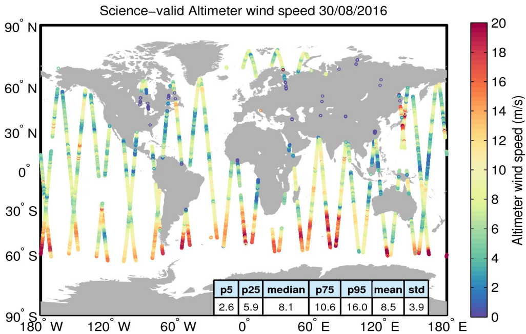
Figure 34. Geographical distribution of science-valid wind data over oceans and lakes for 30/08/2016. The statistical values shown in the table refer to the wind in m/s and are calculated over all measurements shown in the figure. Gray circles denote records that have been rejected based on the editing criteria described in Table 5.
