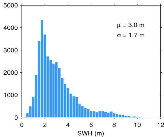
Figure 20. Histogram of science-valid SWH over oceans and lakes for 30/08/2016. The mean ( \mu ) and standard deviation ( \sigma ) are also shown. Note that values larger than 12 m are excluded from the histogram for the sake of readability but not from the computation of \mu and \sigma .
