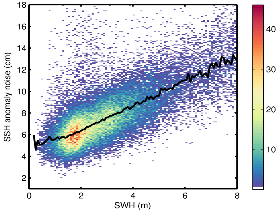
Figure 9. 2D histogram showing flag-valid SSH anomaly noise as a function of SWH for 30/08/2016. The black line denotes the median SSH anomaly noise as a function of SWH.
