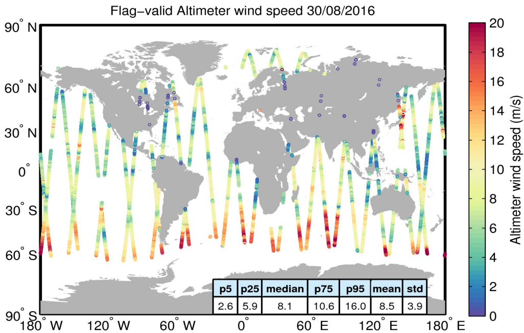
Figure 31. Geographical distribution of flag-valid wind data over oceans and lakes for 30/08/2016. The statistical values shown in the table refer to the wind in m/s and are calculated over all measurements shown in the figure.
