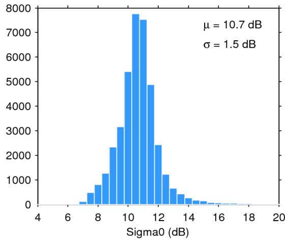
Figure 28. Histogram of science-valid sigma0 over oceans and lakes for 30/08/2016. The mean ( \mu ) and standard deviation ( \sigma ) are also shown. Note that values outside [4 20] dB are excluded from the histogram for the sake of readability but not from the computation of \mu and \sigma .
