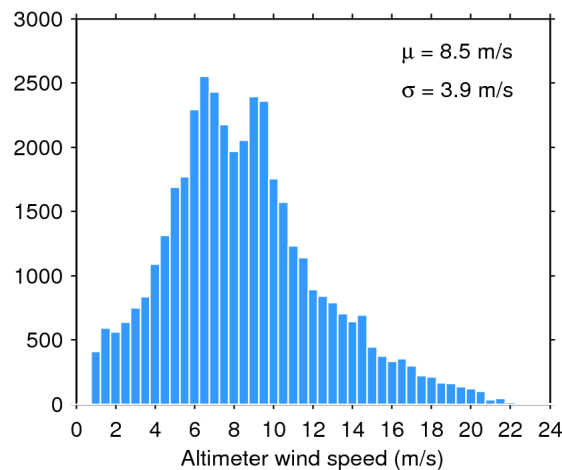
Figure 35. Histogram of science-valid wind over oceans and lakes for 30/08/2016. The mean ( \mu ) and standard deviation ( \sigma ) are also shown. Note that values larger than 24 m/s are excluded from the histogram for the sake of readability but not from the computation of \mu and \sigma .
