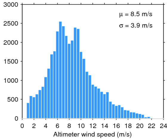
Figure 33. Histogram of flag-valid wind over oceans and lakes for 30/08/2016. The mean ( \mu ) and standard deviation ( \sigma ) are also shown. Note that values larger than 24 m/s are excluded from the histogram for the sake of readability but not from the computation of \mu and \sigma .
