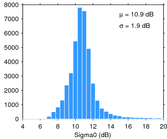
Figure 25. Histogram of flag-valid sigma0 over oceans and lakes for 30/08/2016. The mean ( \mu ) and standard deviation ( \sigma ) are also shown. Note that values outside [4 20] dB are excluded from the histogram for the sake of readability but not from the computation of \mu and \sigma .
