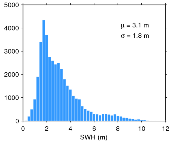
Figure 17. Histogram of flag-valid SWH over oceans and lakes for 30/08/2016. The mean ( \mu ) and standard deviation ( \sigma ) are also shown. Note that values larger than 12 m are excluded from the histogram for the sake of readability but not from the computation of \mu and \sigma .
