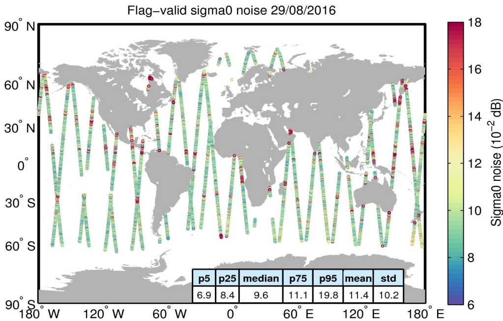
Figure 26. Geographical distribution of flag-valid 20-Hz sigma0 measurement noise over oceans and lakes for 29/08/2016. The statistical values shown in the table refer to the sigma0 noise and are calculated over all measurements shown in the figure.
