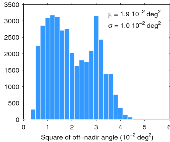
Figure 39. Histogram of flag-valid mispointing over oceans and lakes for 29/08/2016. The mean ( \mu ) and standard deviation ( \sigma ) are also shown. Note that values larger than 6 \cdot 10^{-2} \text{ deg}^2 are excluded from the histogram for the sake of readability but not from the computation of \mu and \sigma .
