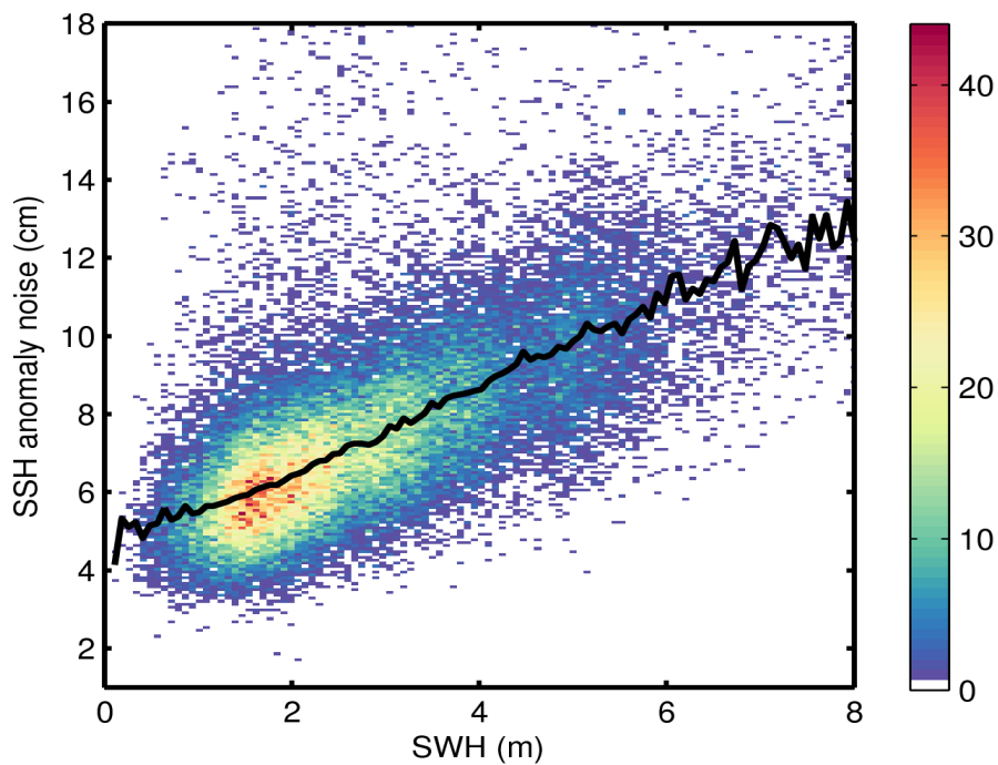
Figure 9. 2D histogram showing flag-valid SSH anomaly noise as a function of SWH for 29/08/2016. The black line denotes the median SSH anomaly noise as a function of SWH.
