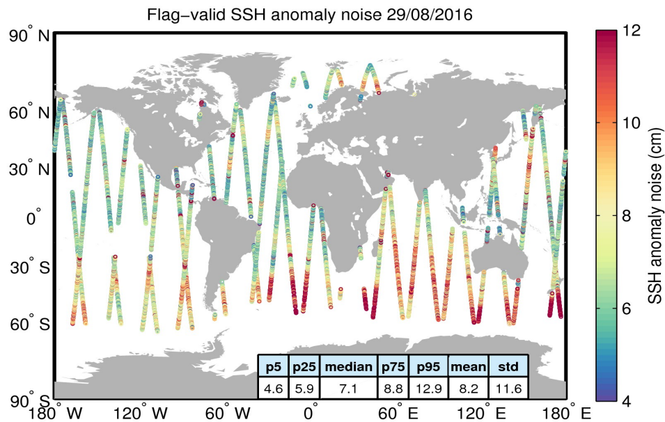
Figure 8. Geographical distribution of flag-valid 20-Hz SSH anomaly measurement noise over oceans and lakes for 29/08/2016. The statistical values shown in the table refer to the SSH anomaly noise and are calculated over all measurements shown in the figure.
