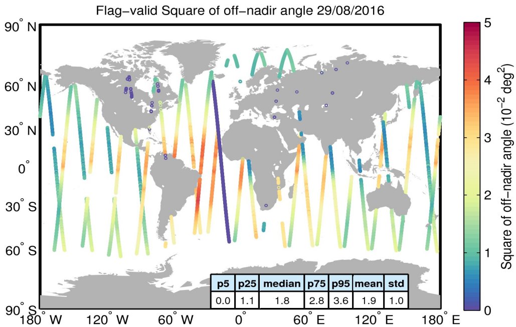
Figure 37. Geographical distribution of flag-valid mispointing data over oceans and lakes for 29/08/2016. The statistical values shown in the table refer to the mispointing in 10^{-2} deg 2 and are calculated over all measurements shown in the figure.
