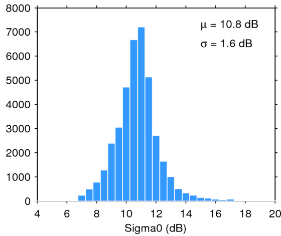
Figure 28. Histogram of science-valid sigma0 over oceans and lakes for 29/08/2016. The mean ( \mu ) and standard deviation ( \sigma ) are also shown. Note that values outside [4 20] dB are excluded from the histogram for the sake of readability but not from the computation of \mu and \sigma .
