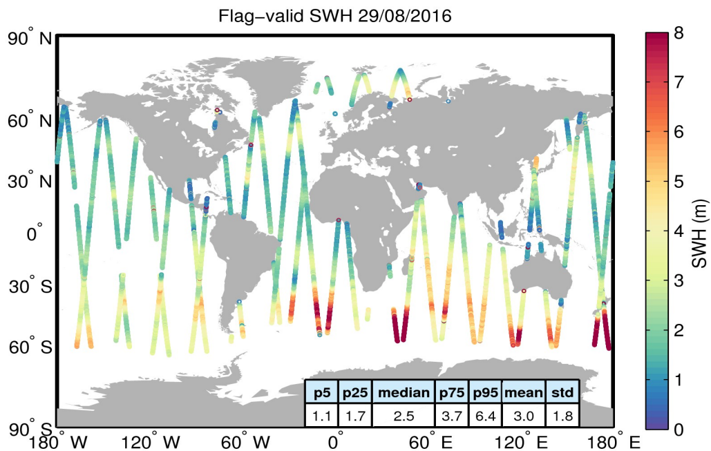
Figure 15. Geographical distribution of flag-valid SWH data over oceans and lakes for 29/08/2016. The statistical values shown in the table refer to the SWH in m and are calculated over all measurements shown in the figure.
