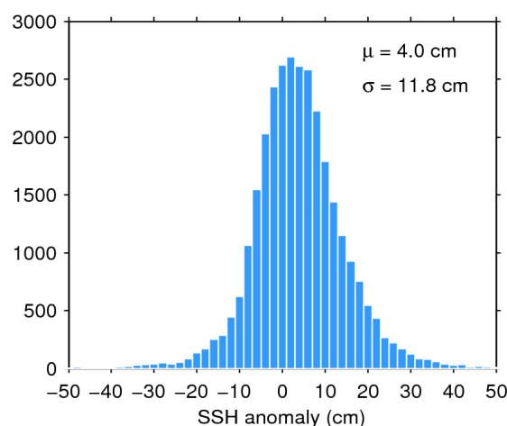
Figure 11. Histogram of science-valid SSH anomaly over oceans and lakes for 29/08/2016. The mean ( \mu ) and standard deviation ( \sigma ) are also shown. Note that values outside [-50 50] cm are excluded from the histogram for the sake of readability but not from the computation of \mu and \sigma .
