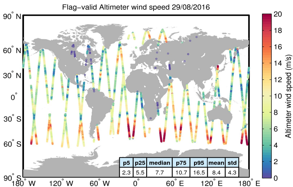
Figure 31. Geographical distribution of flag-valid wind data over oceans and lakes for 29/08/2016. The statistical values shown in the table refer to the wind in m/s and are calculated over all measurements shown in the figure.
