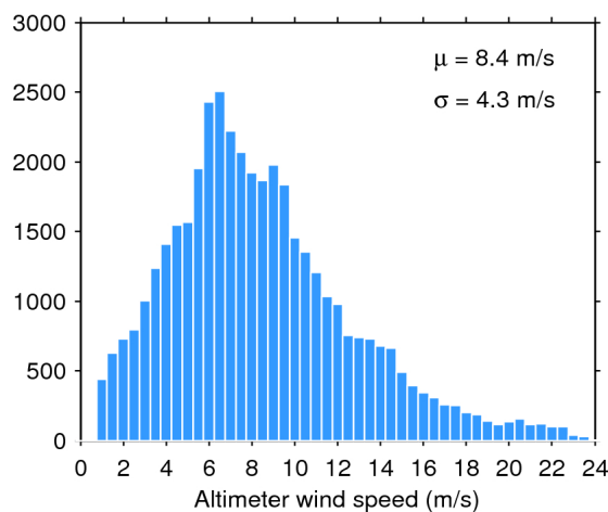
Figure 35. Histogram of science-valid wind over oceans and lakes for 29/08/2016. The mean ( \mu ) and standard deviation ( \sigma ) are also shown. Note that values larger than 24 m/s are excluded from the histogram for the sake of readability but not from the computation of \mu and \sigma .
