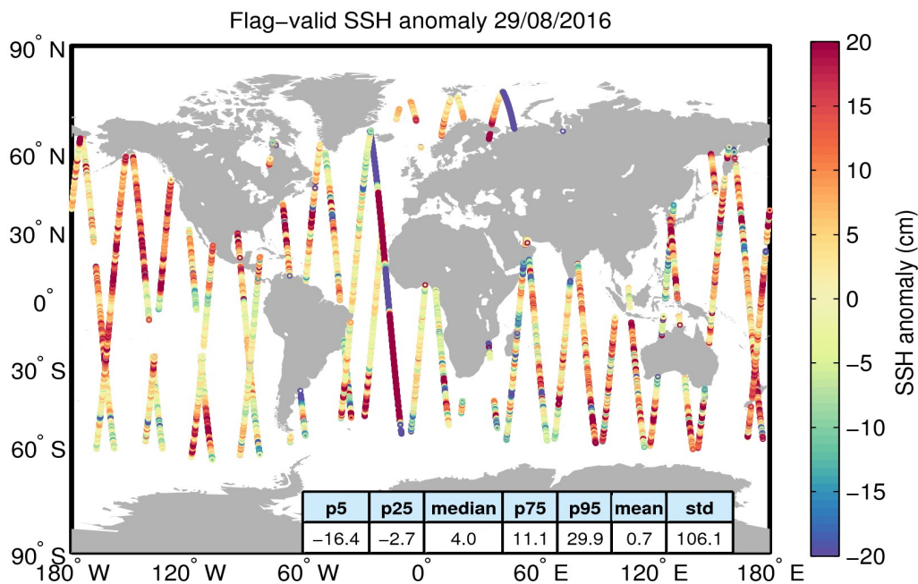
Figure 5. Geographical distribution of flag-valid 1-Hz SSH anomaly data over oceans and lakes for 29/08/2016. The statistical values shown in the table refer to the SSH anomaly in cm and are calculated over all measurements shown in the figure.
