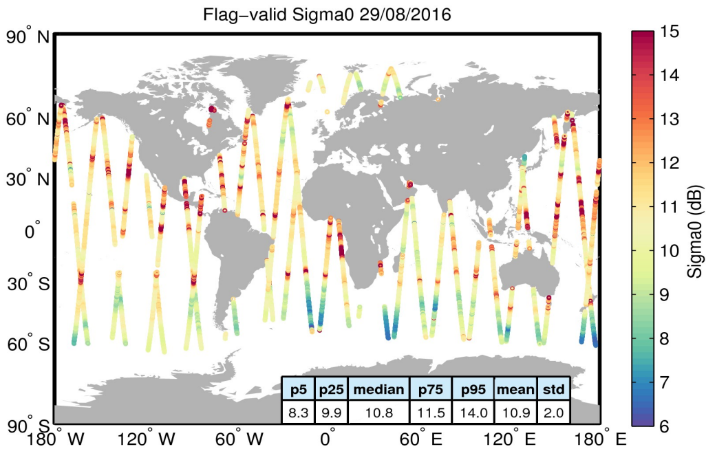
Figure 23. Geographical distribution of flag-valid sigma0 data over oceans and lakes for 29/08/2016. The statistical values shown in the table refer to the sigma0 in dB and are calculated over all measurements shown in the figure.
