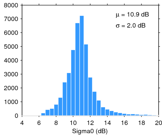
Figure 25. Histogram of flag-valid sigma0 over oceans and lakes for 29/08/2016. The mean ( \mu ) and standard deviation ( \sigma ) are also shown. Note that values outside [4 20] dB are excluded from the histogram for the sake of readability but not from the computation of \mu and \sigma .
