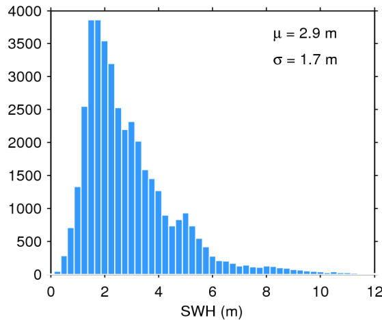
Figure 20. Histogram of science-valid SWH over oceans and lakes for 29/08/2016. The mean ( \mu ) and standard deviation ( \sigma ) are also shown. Note that values larger than 12 m are excluded from the histogram for the sake of readability but not from the computation of \mu and \sigma .
