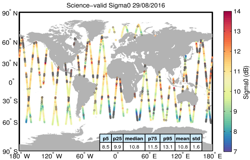
Figure 27. Geographical distribution of science-valid sigma0 data over oceans and lakes for 29/08/2016. The statistical values shown in the table refer to the sigma0 in dB and are calculated over all measurements shown in the figure. Gray circles denote records that have been rejected based on the editing criteria described in Table 4.
