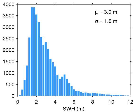
Figure 17. Histogram of flag-valid SWH over oceans and lakes for 29/08/2016. The mean ( \mu ) and standard deviation ( \sigma ) are also shown. Note that values larger than 12 m are excluded from the histogram for the sake of readability but not from the computation of \mu and \sigma .
