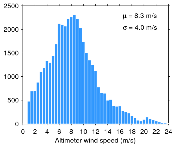
Figure 35. Histogram of science-valid wind over oceans and lakes for 28/08/2016. The mean ( \mu ) and standard deviation ( \sigma ) are also shown. Note that values larger than 24 m/s are excluded from the histogram for the sake of readability but not from the computation of \mu and \sigma .
