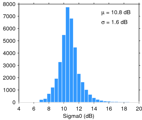
Figure 28. Histogram of science-valid sigma0 over oceans and lakes for 28/08/2016. The mean ( \mu ) and standard deviation ( \sigma ) are also shown. Note that values outside [4 20] dB are excluded from the histogram for the sake of readability but not from the computation of \mu and \sigma .
