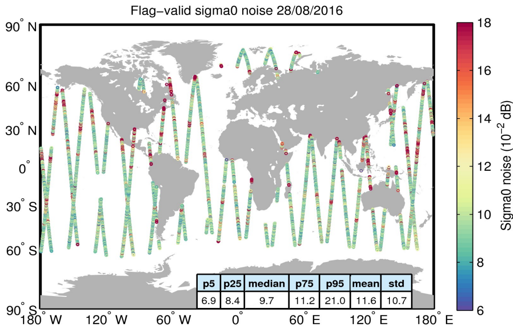
Figure 26. Geographical distribution of flag-valid 20-Hz sigma0 measurement noise over oceans and lakes for 28/08/2016. The statistical values shown in the table refer to the sigma0 noise and are calculated over all measurements shown in the figure.
