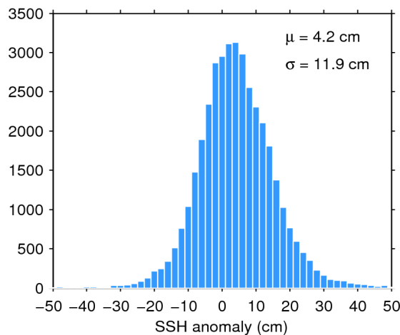
Figure 11. Histogram of science-valid SSH anomaly over oceans and lakes for 28/08/2016. The mean ( \mu ) and standard deviation ( \sigma ) are also shown. Note that values outside [-50 50] cm are excluded from the histogram for the sake of readability but not from the computation of \mu and \sigma .
