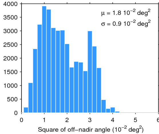
Figure 39. Histogram of flag-valid mispointing over oceans and lakes for 28/08/2016. The mean ( \mu ) and standard deviation ( \sigma ) are also shown. Note that values larger than 6 \cdot 10^{-2} \text{ deg}^2 are excluded from the histogram for the sake of readability but not from the computation of \mu and \sigma .
