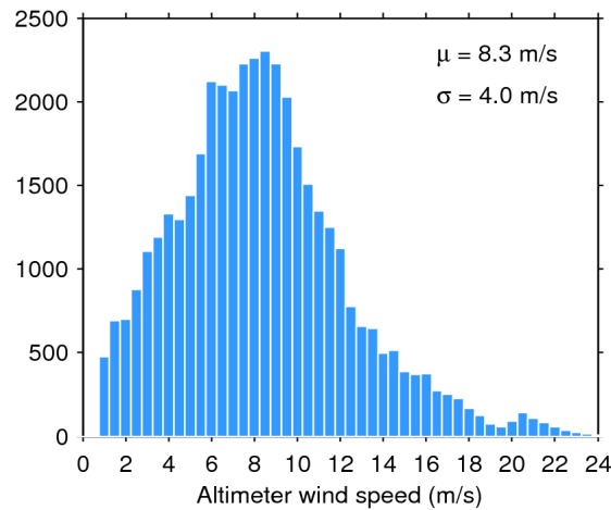
Figure 33. Histogram of flag-valid wind over oceans and lakes for 28/08/2016. The mean ( \mu ) and standard deviation ( \sigma ) are also shown. Note that values larger than 24 m/s are excluded from the histogram for the sake of readability but not from the computation of \mu and \sigma .
