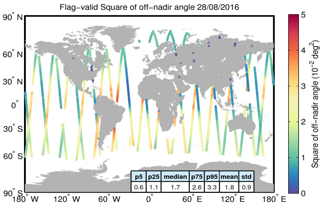
Figure 37. Geographical distribution of flag-valid mispointing data over oceans and lakes for 28/08/2016. The statistical values shown in the table refer to the mispointing in 10^{-2} deg 2 and are calculated over all measurements shown in the figure.
