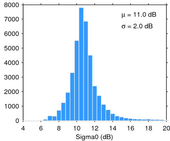
Figure 25. Histogram of flag-valid sigma0 over oceans and lakes for 28/08/2016. The mean ( \mu ) and standard deviation ( \sigma ) are also shown. Note that values outside [4 20] dB are excluded from the histogram for the sake of readability but not from the computation of \mu and \sigma .
