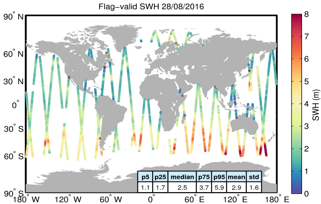
Figure 15. Geographical distribution of flag-valid SWH data over oceans and lakes for 28/08/2016. The statistical values shown in the table refer to the SWH in m and are calculated over all measurements shown in the figure.
