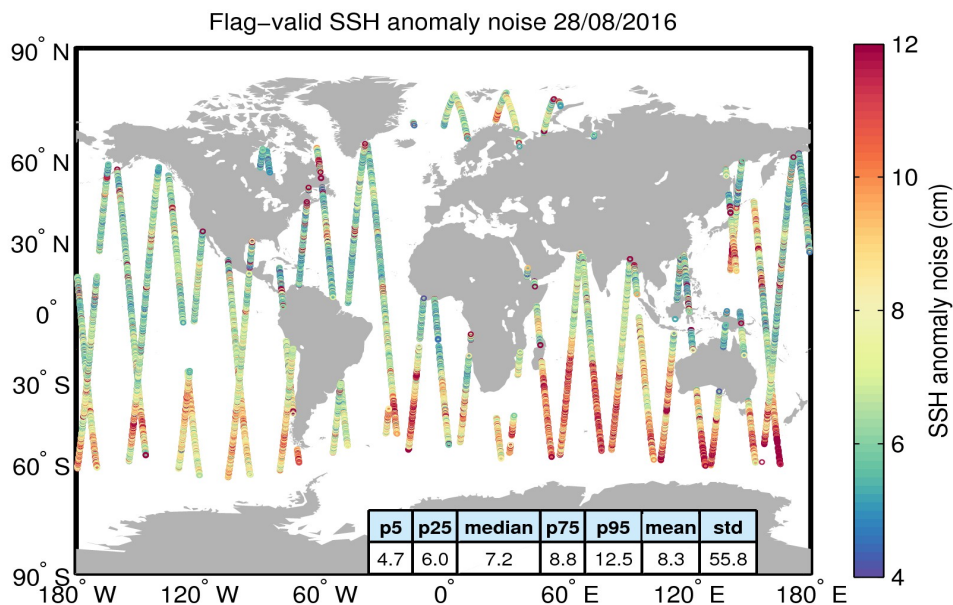
Figure 8. Geographical distribution of flag-valid 20-Hz SSH anomaly measurement noise over oceans and lakes for 28/08/2016. The statistical values shown in the table refer to the SSH anomaly noise and are calculated over all measurements shown in the figure.
