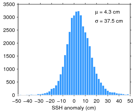
Figure 7. Histogram of flag-valid SSH anomaly over oceans and lakes for 28/08/2016. The mean ( \mu ) and standard deviation ( \sigma ) are also shown. Note that values outside [-50 50] cm are excluded from the histogram for the sake of readability but not from the computation of \mu and \sigma .
