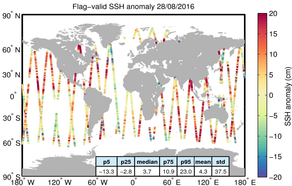
Figure 5. Geographical distribution of flag-valid 1-Hz SSH anomaly data over oceans and lakes for 28/08/2016. The statistical values shown in the table refer to the SSH anomaly in cm and are calculated over all measurements shown in the figure.
