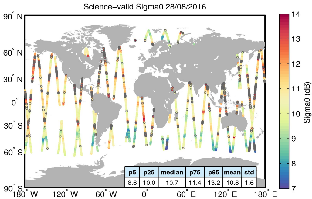
Figure 27. Geographical distribution of science-valid sigma0 data over oceans and lakes for 28/08/2016. The statistical values shown in the table refer to the sigma0 in dB and are calculated over all measurements shown in the figure. Gray circles denote records that have been rejected based on the editing criteria described in Table 4.
