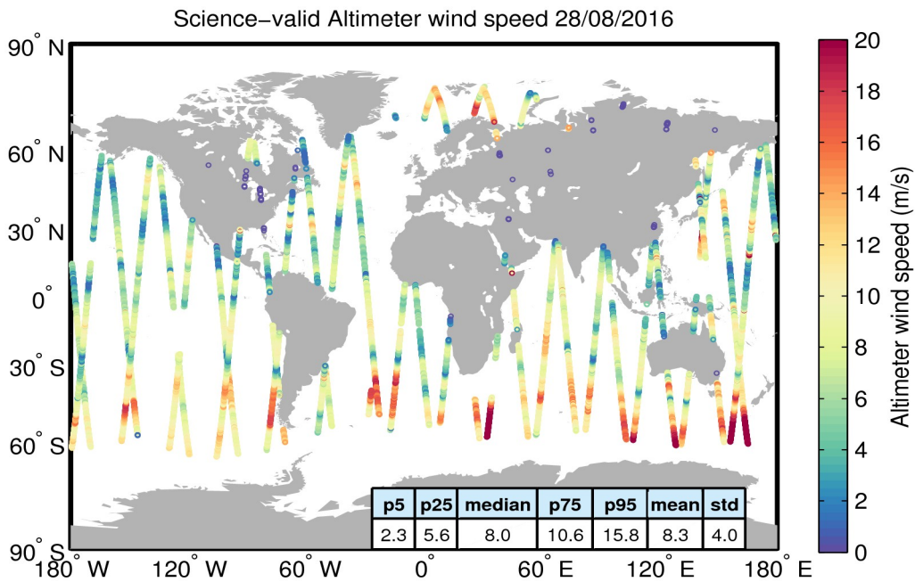
Figure 34. Geographical distribution of science-valid wind data over oceans and lakes for 28/08/2016. The statistical values shown in the table refer to the wind in m/s and are calculated over all measurements shown in the figure. Gray circles denote records that have been rejected based on the editing criteria described in Table 5.
