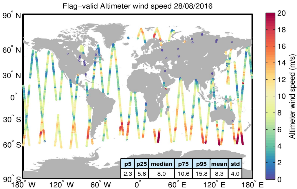
Figure 31. Geographical distribution of flag-valid wind data over oceans and lakes for 28/08/2016. The statistical values shown in the table refer to the wind in m/s and are calculated over all measurements shown in the figure.
