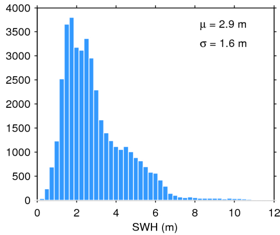
Figure 17. Histogram of flag-valid SWH over oceans and lakes for 28/08/2016. The mean ( \mu ) and standard deviation ( \sigma ) are also shown. Note that values larger than 12 m are excluded from the histogram for the sake of readability but not from the computation of \mu and \sigma .
