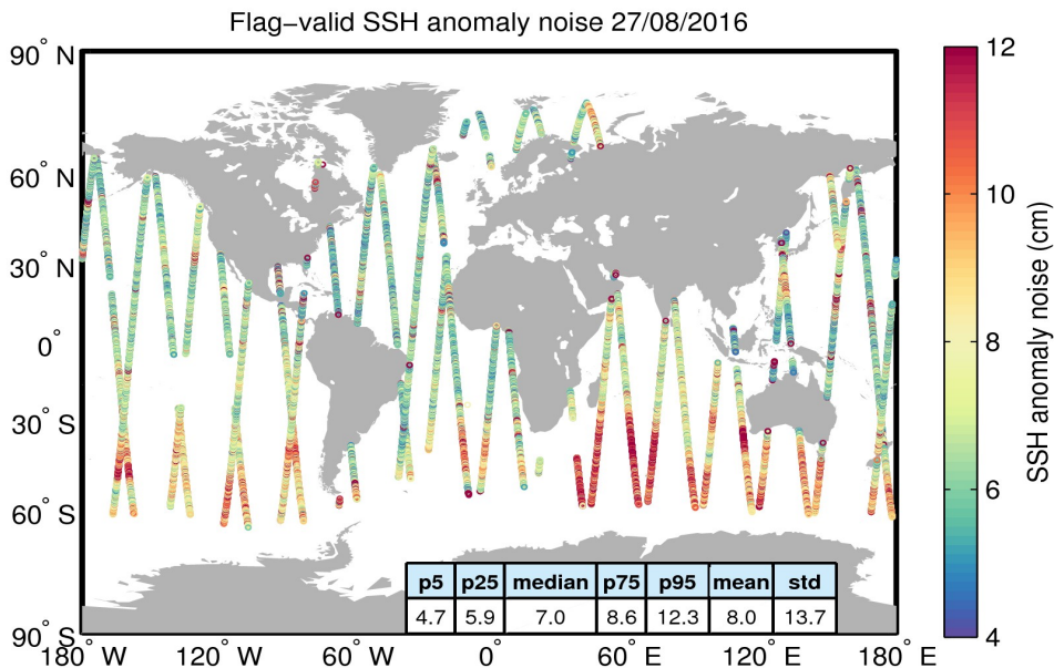
Figure 8. Geographical distribution of flag-valid 20-Hz SSH anomaly measurement noise over oceans and lakes for 27/08/2016. The statistical values shown in the table refer to the SSH anomaly noise and are calculated over all measurements shown in the figure.
