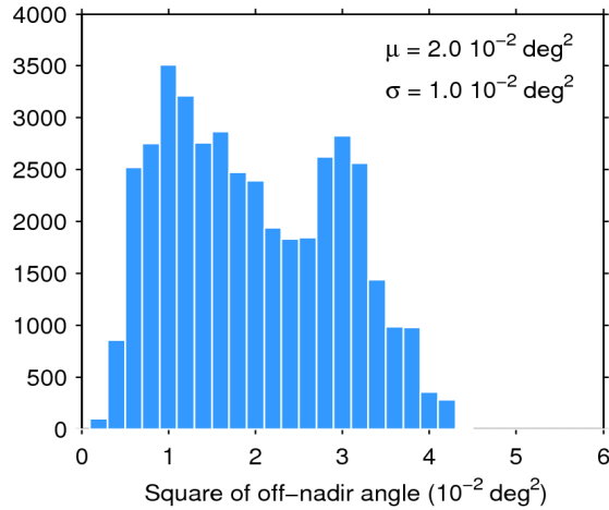
Figure 39. Histogram of flag-valid mispointing over oceans and lakes for 27/08/2016. The mean ( \mu ) and standard deviation ( \sigma ) are also shown. Note that values larger than 6 \cdot 10^{-2} \text{ deg}^2 are excluded from the histogram for the sake of readability but not from the computation of \mu and \sigma .
