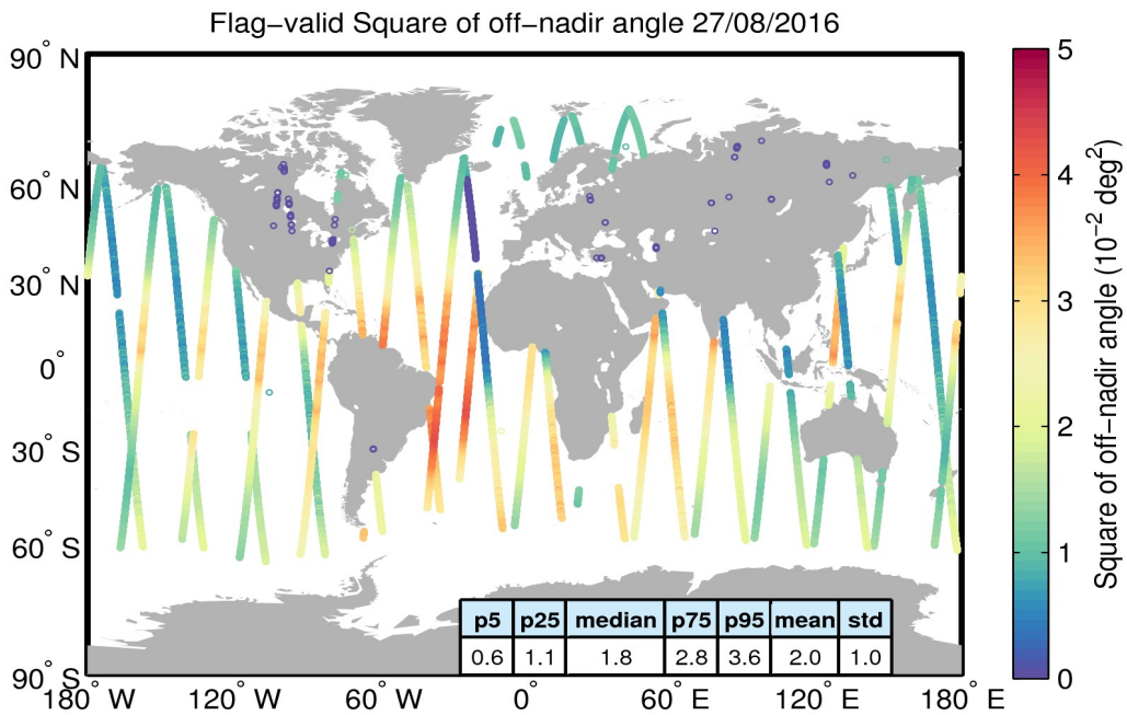
Figure 37. Geographical distribution of flag-valid mispointing data over oceans and lakes for 27/08/2016. The statistical values shown in the table refer to the mispointing in 10^{-2} deg 2 and are calculated over all measurements shown in the figure.
