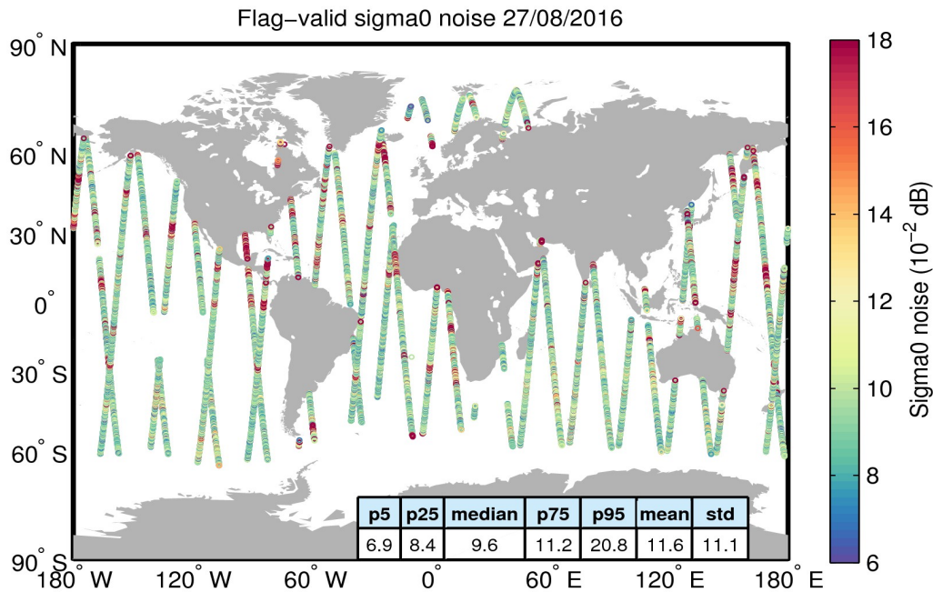
Figure 26. Geographical distribution of flag-valid 20-Hz sigma0 measurement noise over oceans and lakes for 27/08/2016. The statistical values shown in the table refer to the sigma0 noise and are calculated over all measurements shown in the figure.
