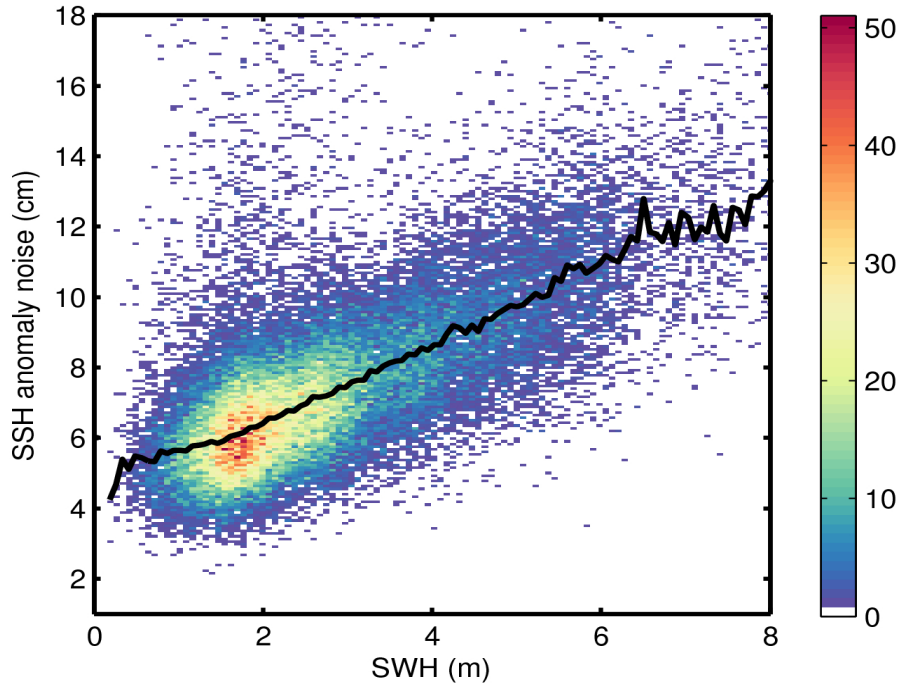
Figure 9. 2D histogram showing flag-valid SSH anomaly noise as a function of SWH for 27/08/2016. The black line denotes the median SSH anomaly noise as a function of SWH.
