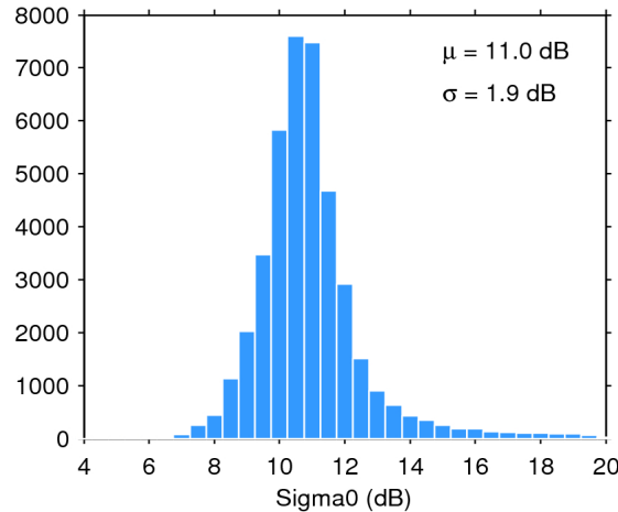
Figure 25. Histogram of flag-valid sigma0 over oceans and lakes for 27/08/2016. The mean ( \mu ) and standard deviation ( \sigma ) are also shown. Note that values outside [4 20] dB are excluded from the histogram for the sake of readability but not from the computation of \mu and \sigma .
