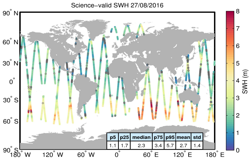
Figure 19. Geographical distribution of science-valid SWH data over oceans and lakes for 27/08/2016. The statistical values shown in the table refer to the SWH in m and are calculated over all measurements shown in the figure. Gray circles denote records that have been rejected based on the editing criteria described in Table 3.
