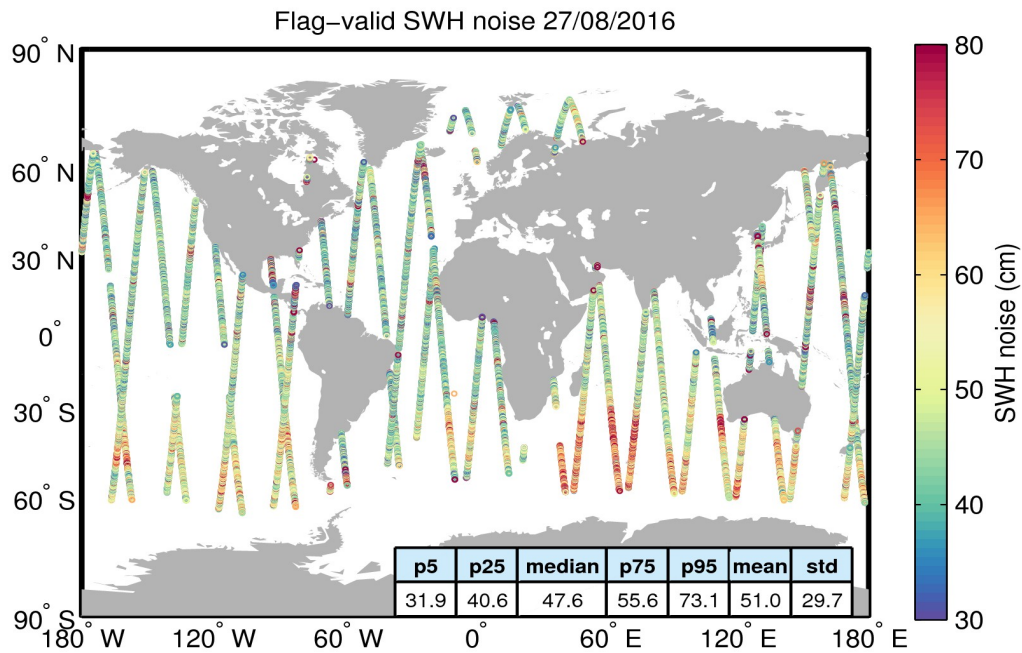
Figure 18. Geographical distribution of flag-valid 20-Hz SWH measurement noise over oceans and lakes for 27/08/2016. The statistical values shown in the table refer to the SWH noise and are calculated over all measurements shown in the figure.
