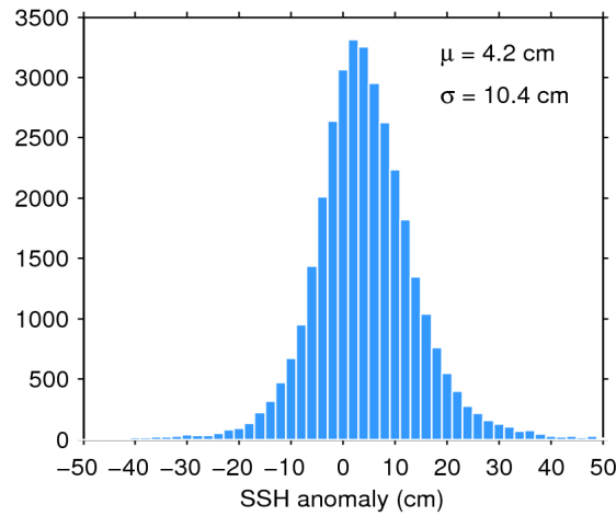
Figure 11. Histogram of science-valid SSH anomaly over oceans and lakes for 27/08/2016. The mean ( \mu ) and standard deviation ( \sigma ) are also shown. Note that values outside [-50 50] cm are excluded from the histogram for the sake of readability but not from the computation of \mu and \sigma .
