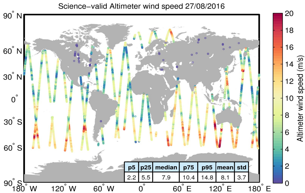
Figure 34. Geographical distribution of science-valid wind data over oceans and lakes for 27/08/2016. The statistical values shown in the table refer to the wind in m/s and are calculated over all measurements shown in the figure. Gray circles denote records that have been rejected based on the editing criteria described in Table 5.
