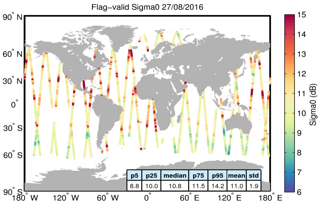
Figure 23. Geographical distribution of flag-valid sigma0 data over oceans and lakes for 27/08/2016. The statistical values shown in the table refer to the sigma0 in dB and are calculated over all measurements shown in the figure.
