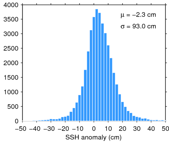
Figure 7. Histogram of flag-valid SSH anomaly over oceans and lakes for 27/08/2016. The mean ( \mu ) and standard deviation ( \sigma ) are also shown. Note that values outside [-50 50] cm are excluded from the histogram for the sake of readability but not from the computation of \mu and \sigma .
