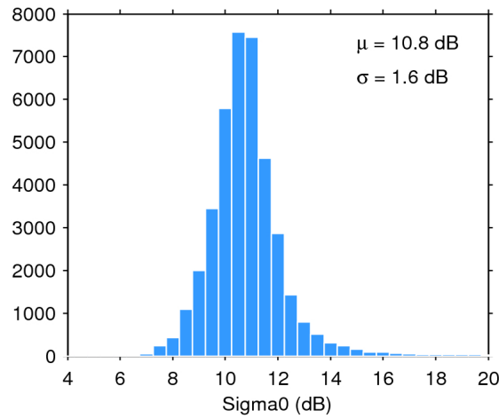
Figure 28. Histogram of science-valid sigma0 over oceans and lakes for 27/08/2016. The mean ( \mu ) and standard deviation ( \sigma ) are also shown. Note that values outside [4 20] dB are excluded from the histogram for the sake of readability but not from the computation of \mu and \sigma .
