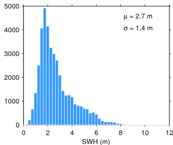
Figure 20. Histogram of science-valid SWH over oceans and lakes for 27/08/2016. The mean ( \mu ) and standard deviation ( \sigma ) are also shown. Note that values larger than 12 m are excluded from the histogram for the sake of readability but not from the computation of \mu and \sigma .
