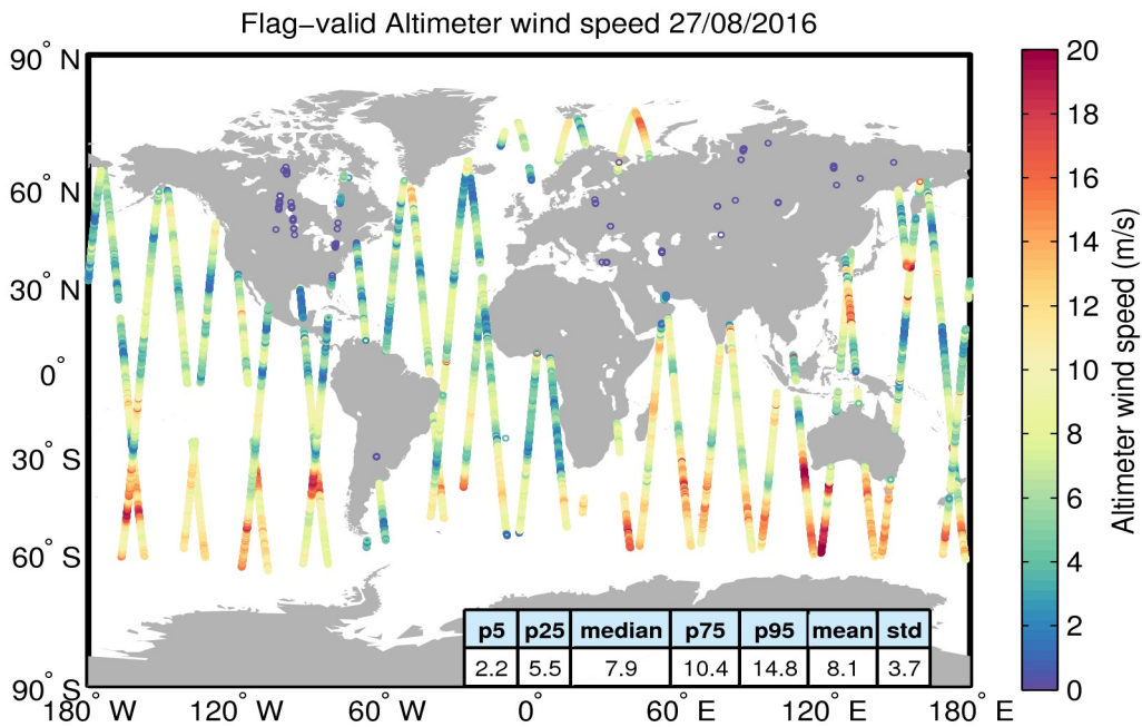
Figure 31. Geographical distribution of flag-valid wind data over oceans and lakes for 27/08/2016. The statistical values shown in the table refer to the wind in m/s and are calculated over all measurements shown in the figure.
