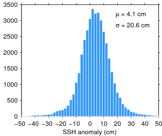
Figure 7. Histogram of flag-valid SSH anomaly over oceans and lakes for 26/08/2016. The mean ( \mu ) and standard deviation ( \sigma ) are also shown. Note that values outside [-50 50] cm are excluded from the histogram for the sake of readability but not from the computation of \mu and \sigma .
