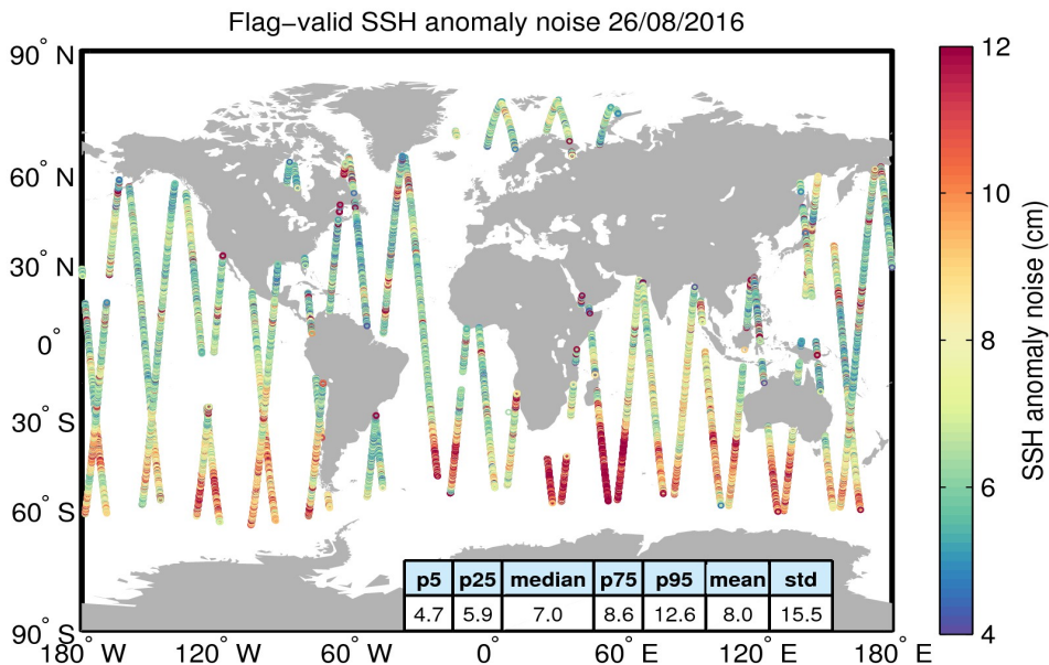
Figure 8. Geographical distribution of flag-valid 20-Hz SSH anomaly measurement noise over oceans and lakes for 26/08/2016. The statistical values shown in the table refer to the SSH anomaly noise and are calculated over all measurements shown in the figure.
