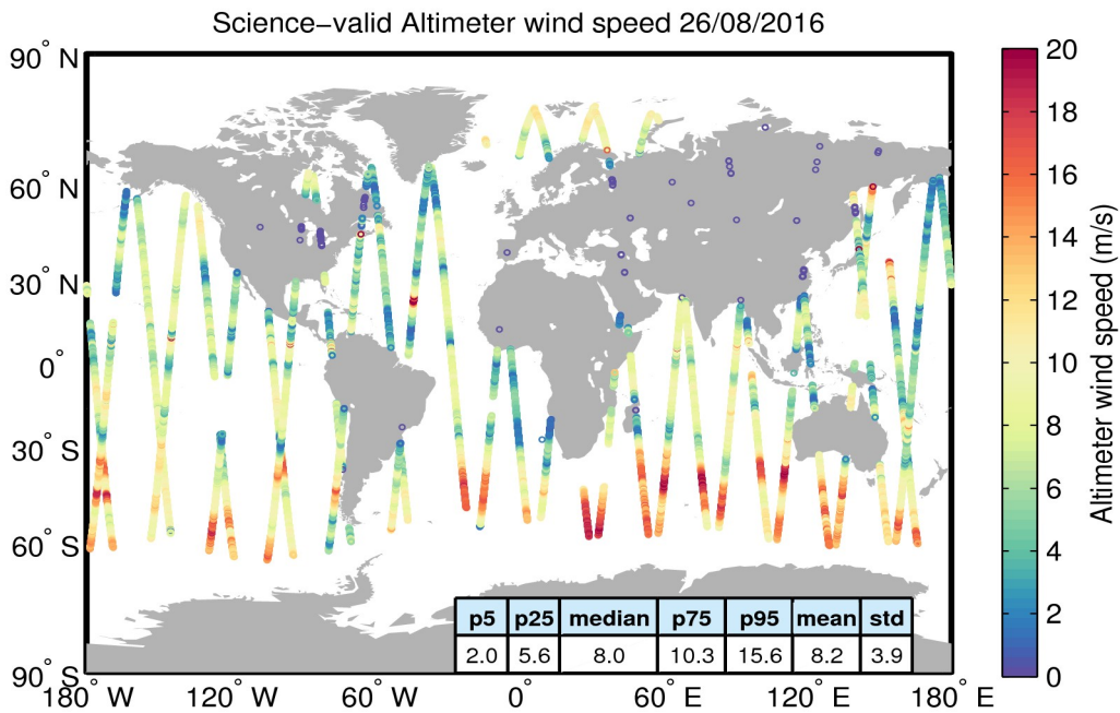
Figure 34. Geographical distribution of science-valid wind data over oceans and lakes for 26/08/2016. The statistical values shown in the table refer to the wind in m/s and are calculated over all measurements shown in the figure. Gray circles denote records that have been rejected based on the editing criteria described in Table 5.
