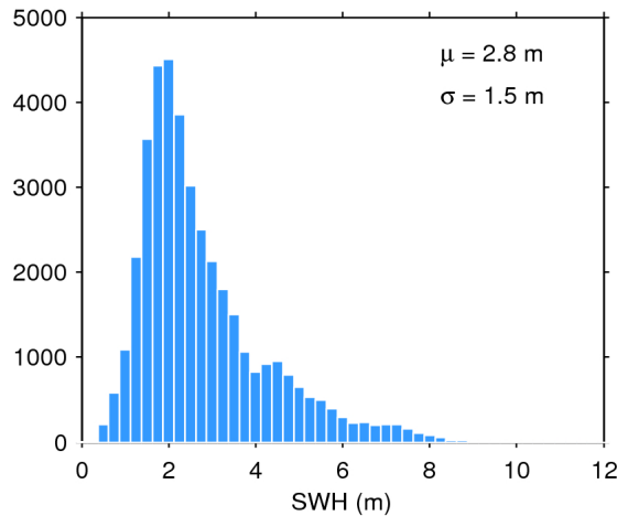
Figure 20. Histogram of science-valid SWH over oceans and lakes for 26/08/2016. The mean ( \mu ) and standard deviation ( \sigma ) are also shown. Note that values larger than 12 m are excluded from the histogram for the sake of readability but not from the computation of \mu and \sigma .
