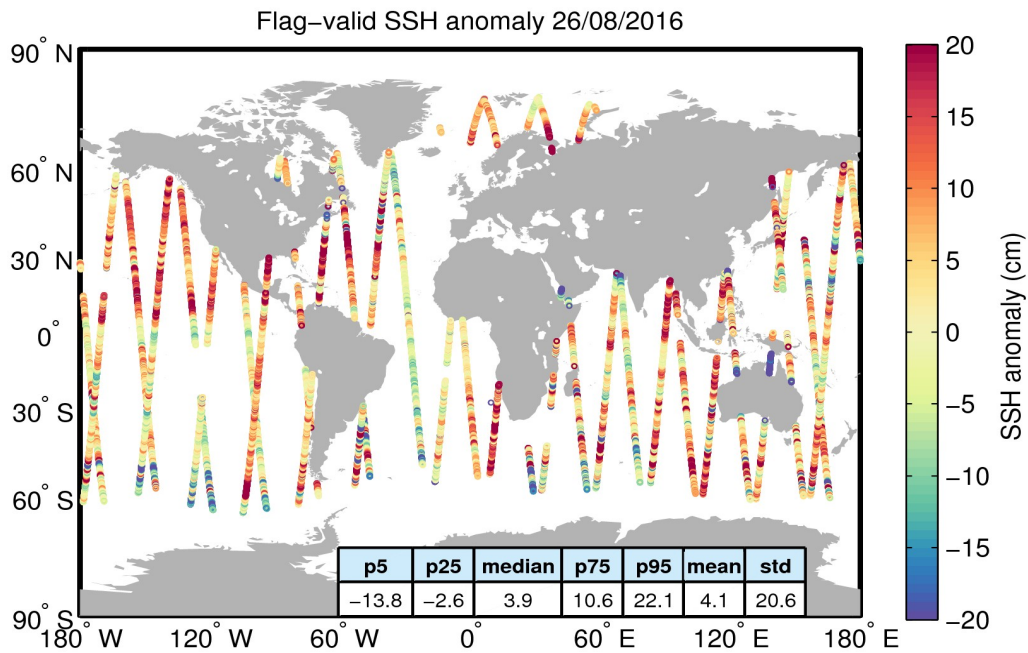
Figure 5. Geographical distribution of flag-valid 1-Hz SSH anomaly data over oceans and lakes for 26/08/2016. The statistical values shown in the table refer to the SSH anomaly in cm and are calculated over all measurements shown in the figure.
