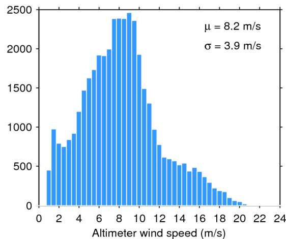
Figure 35. Histogram of science-valid wind over oceans and lakes for 26/08/2016. The mean ( \mu ) and standard deviation ( \sigma ) are also shown. Note that values larger than 24 m/s are excluded from the histogram for the sake of readability but not from the computation of \mu and \sigma .
