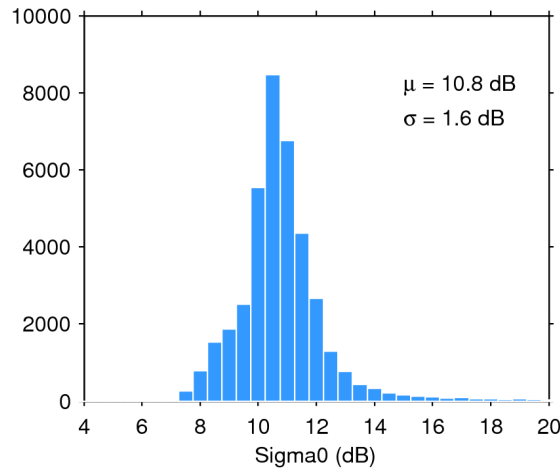
Figure 28. Histogram of science-valid sigma0 over oceans and lakes for 26/08/2016. The mean ( \mu ) and standard deviation ( \sigma ) are also shown. Note that values outside [4 20] dB are excluded from the histogram for the sake of readability but not from the computation of \mu and \sigma .
