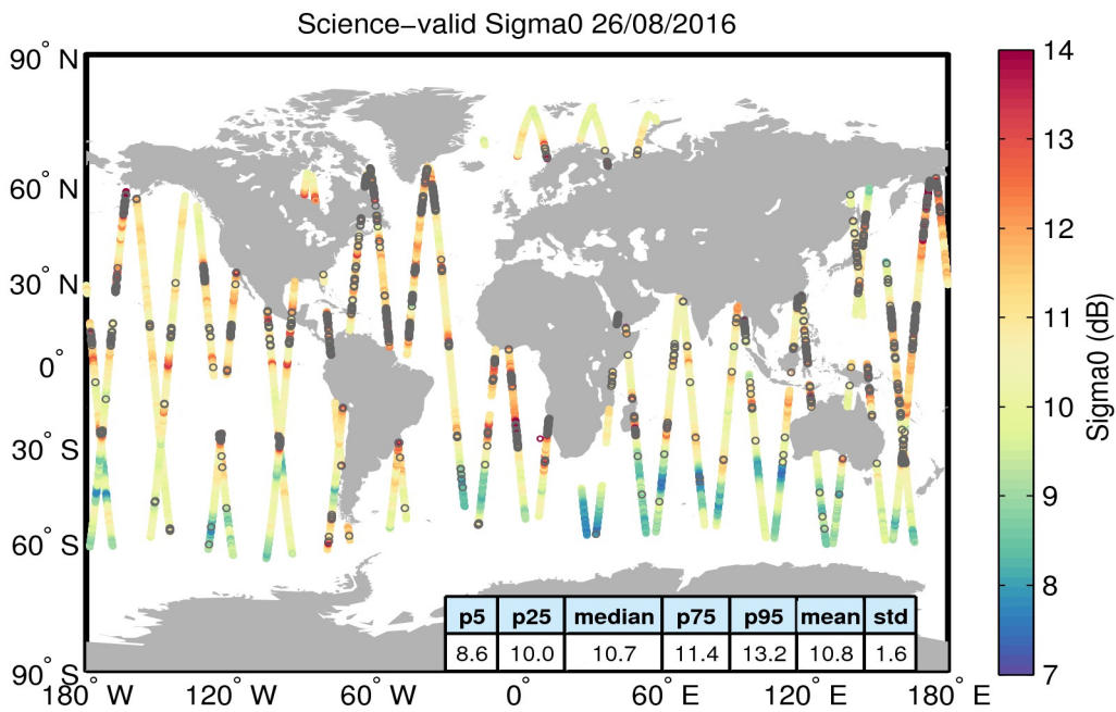
Figure 27. Geographical distribution of science-valid sigma0 data over oceans and lakes for 26/08/2016. The statistical values shown in the table refer to the sigma0 in dB and are calculated over all measurements shown in the figure. Gray circles denote records that have been rejected based on the editing criteria described in Table 4.
