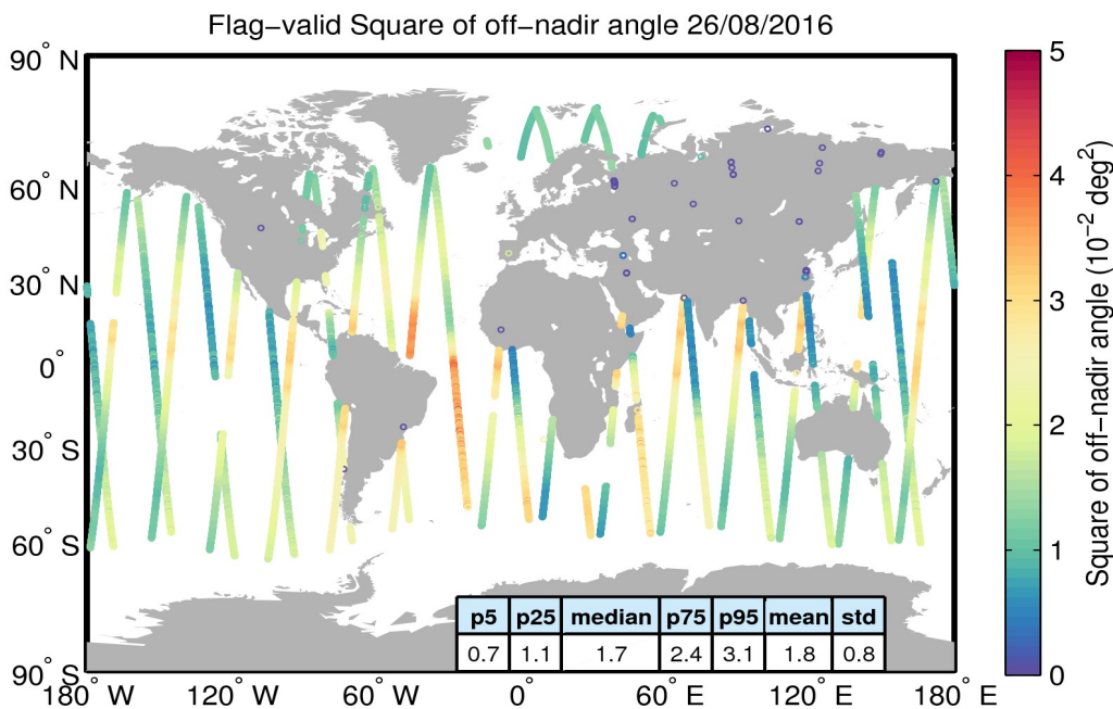
Figure 37. Geographical distribution of flag-valid mispointing data over oceans and lakes for 26/08/2016. The statistical values shown in the table refer to the mispointing in 10^{-2} deg 2 and are calculated over all measurements shown in the figure.
