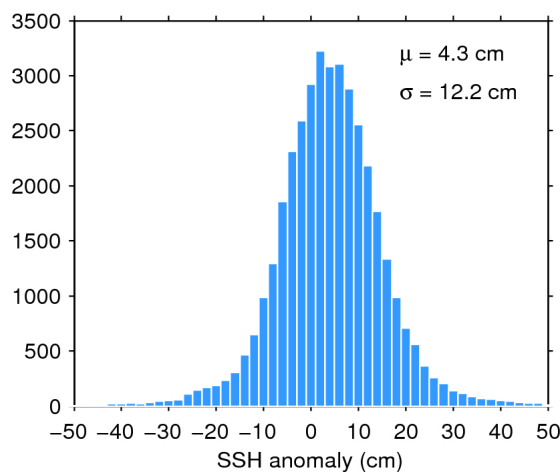
Figure 11. Histogram of science-valid SSH anomaly over oceans and lakes for 26/08/2016. The mean ( \mu ) and standard deviation ( \sigma ) are also shown. Note that values outside [-50 50] cm are excluded from the histogram for the sake of readability but not from the computation of \mu and \sigma .
