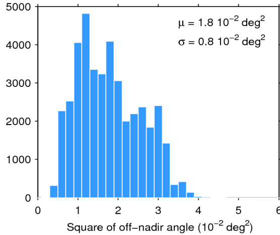
Figure 39. Histogram of flag-valid mispointing over oceans and lakes for 26/08/2016. The mean ( \mu ) and standard deviation ( \sigma ) are also shown. Note that values larger than 6 \cdot 10^{-2} \text{ deg}^2 are excluded from the histogram for the sake of readability but not from the computation of \mu and \sigma .
