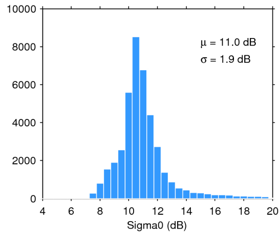
Figure 25. Histogram of flag-valid sigma0 over oceans and lakes for 26/08/2016. The mean ( \mu ) and standard deviation ( \sigma ) are also shown. Note that values outside [4 20] dB are excluded from the histogram for the sake of readability but not from the computation of \mu and \sigma .
