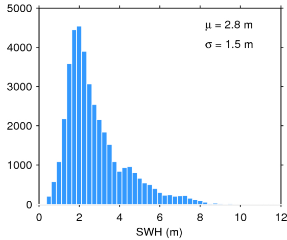
Figure 17. Histogram of flag-valid SWH over oceans and lakes for 26/08/2016. The mean ( \mu ) and standard deviation ( \sigma ) are also shown. Note that values larger than 12 m are excluded from the histogram for the sake of readability but not from the computation of \mu and \sigma .
