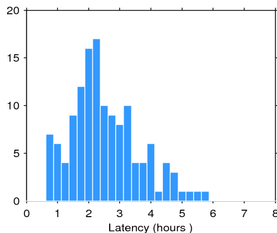
Figure 2. Histogram of the data latency for 26/08/2016. The y-axis denotes the number of files that are made available with a delay of x-hours with respect to the mean time of the records stored in the file.
