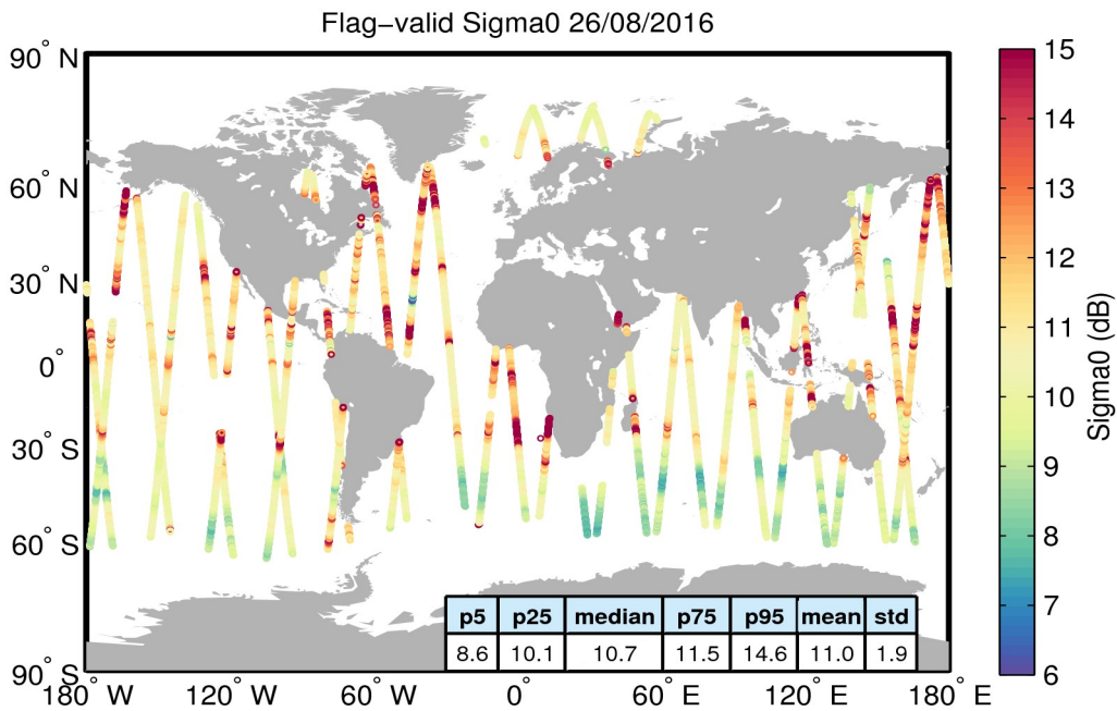
Figure 23. Geographical distribution of flag-valid sigma0 data over oceans and lakes for 26/08/2016. The statistical values shown in the table refer to the sigma0 in dB and are calculated over all measurements shown in the figure.
