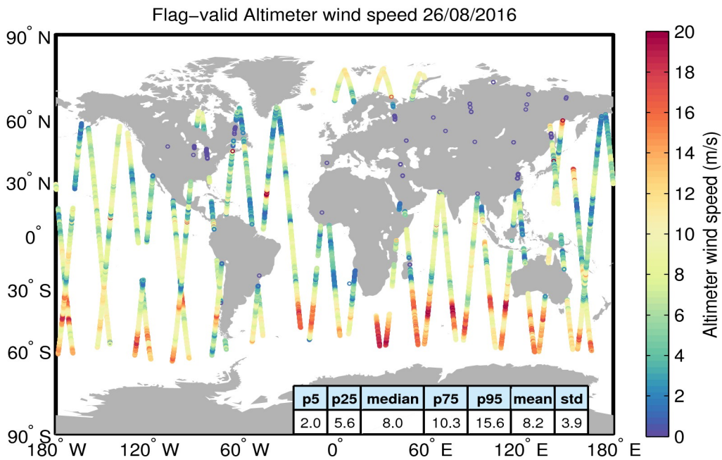
Figure 31. Geographical distribution of flag-valid wind data over oceans and lakes for 26/08/2016. The statistical values shown in the table refer to the wind in m/s and are calculated over all measurements shown in the figure.
