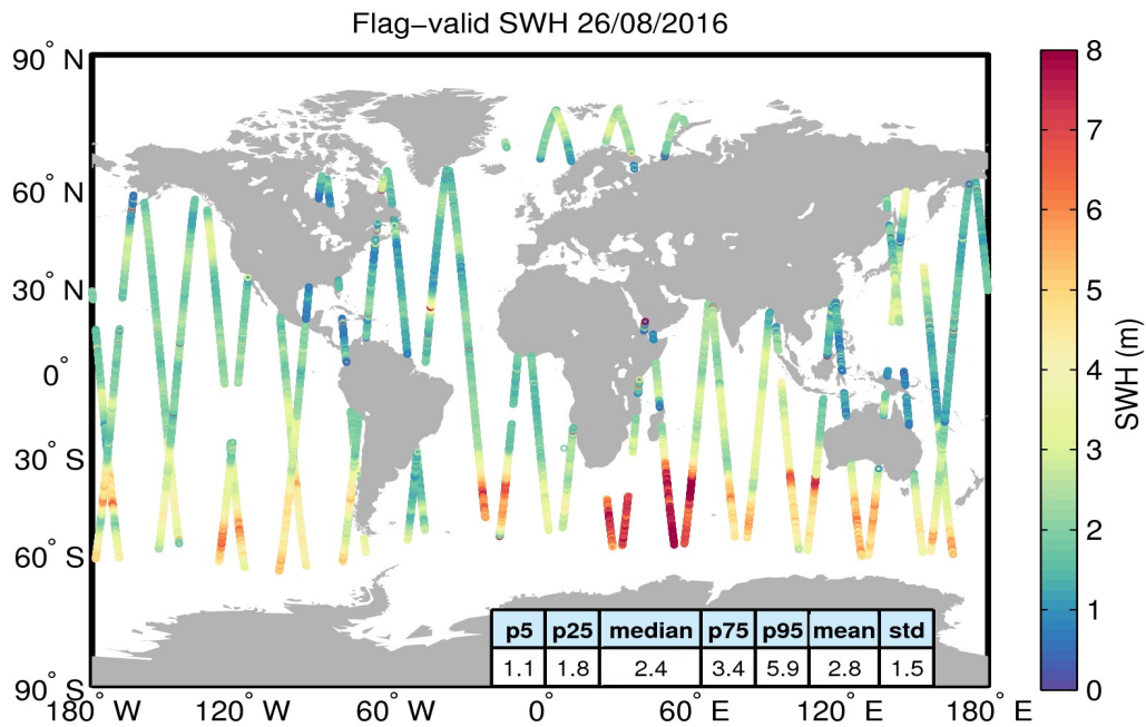
Figure 15. Geographical distribution of flag-valid SWH data over oceans and lakes for 26/08/2016. The statistical values shown in the table refer to the SWH in m and are calculated over all measurements shown in the figure.
