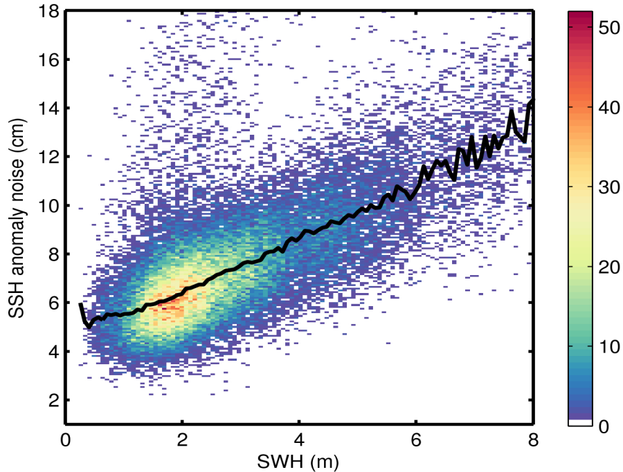
Figure 9. 2D histogram showing flag-valid SSH anomaly noise as a function of SWH for 26/08/2016. The black line denotes the median SSH anomaly noise as a function of SWH.
