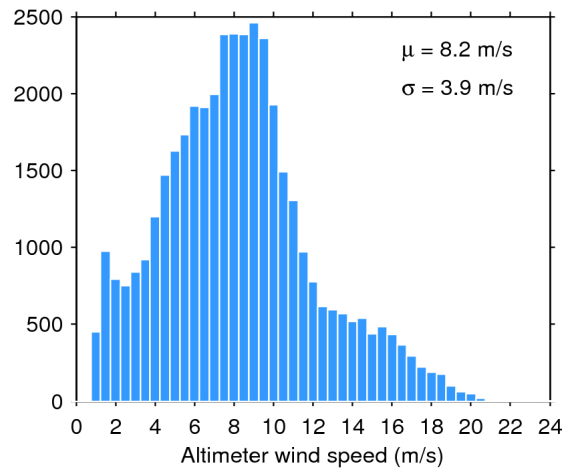
Figure 33. Histogram of flag-valid wind over oceans and lakes for 26/08/2016. The mean ( \mu ) and standard deviation ( \sigma ) are also shown. Note that values larger than 24 m/s are excluded from the histogram for the sake of readability but not from the computation of \mu and \sigma .
