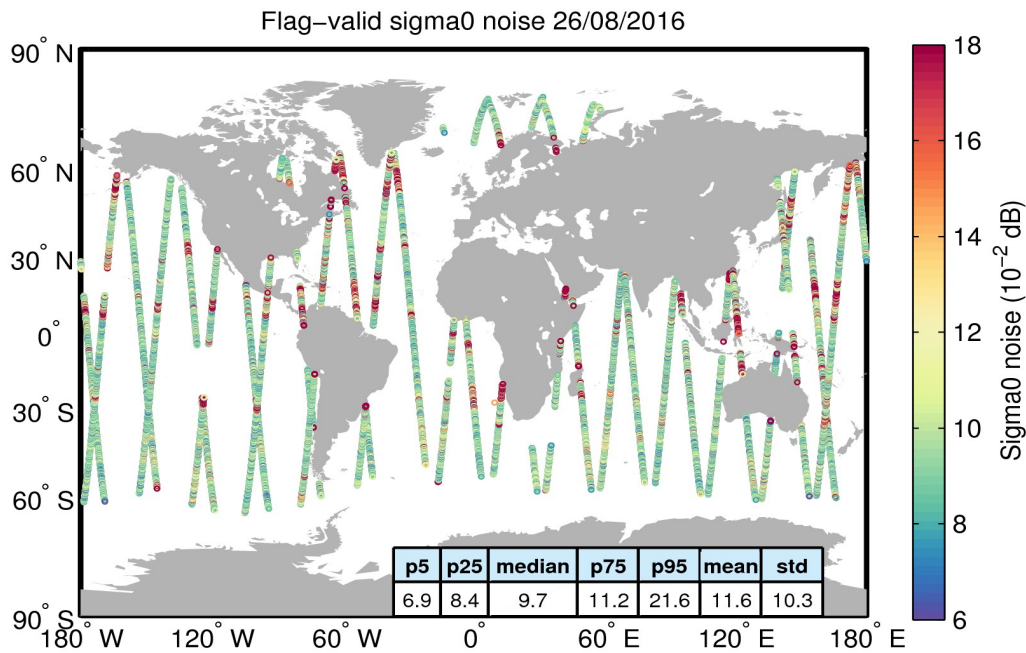
Figure 26. Geographical distribution of flag-valid 20-Hz sigma0 measurement noise over oceans and lakes for 26/08/2016. The statistical values shown in the table refer to the sigma0 noise and are calculated over all measurements shown in the figure.
