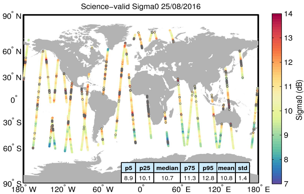
Figure 27. Geographical distribution of science-valid sigma0 data over oceans and lakes for 25/08/2016. The statistical values shown in the table refer to the sigma0 in dB and are calculated over all measurements shown in the figure. Gray circles denote records that have been rejected based on the editing criteria described in Table 4.
