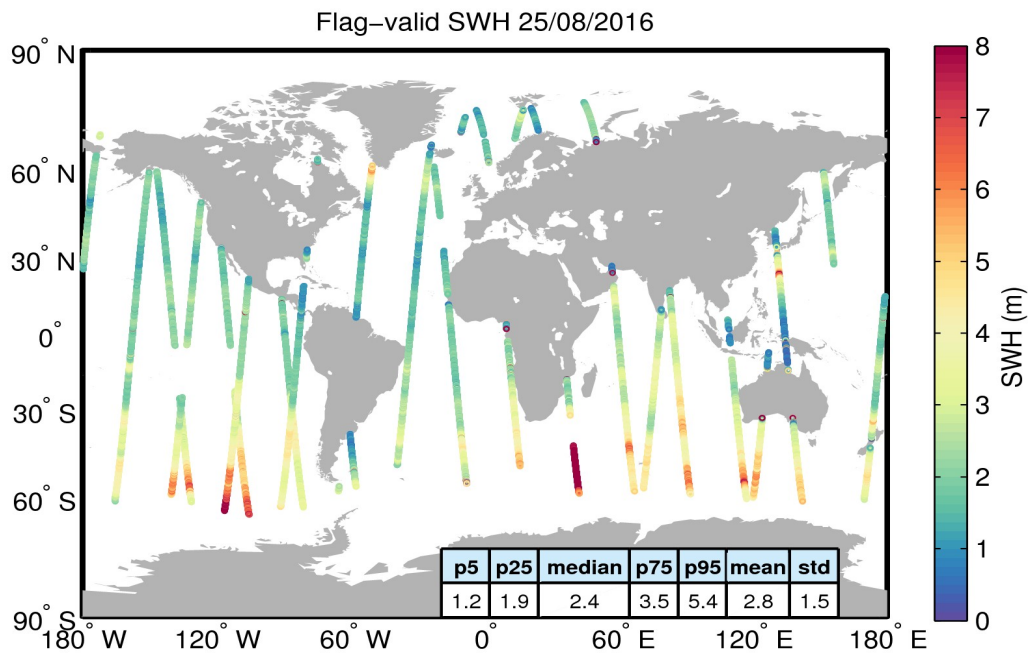
Figure 15. Geographical distribution of flag-valid SWH data over oceans and lakes for 25/08/2016. The statistical values shown in the table refer to the SWH in m and are calculated over all measurements shown in the figure.
