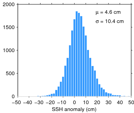
Figure 11. Histogram of science-valid SSH anomaly over oceans and lakes for 25/08/2016. The mean ( \mu ) and standard deviation ( \sigma ) are also shown. Note that values outside [-50 50] cm are excluded from the histogram for the sake of readability but not from the computation of \mu and \sigma .
