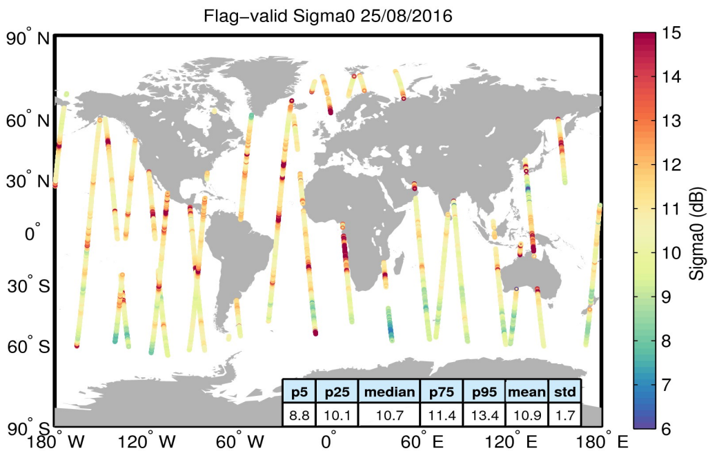
Figure 23. Geographical distribution of flag-valid sigma0 data over oceans and lakes for 25/08/2016. The statistical values shown in the table refer to the sigma0 in dB and are calculated over all measurements shown in the figure.
