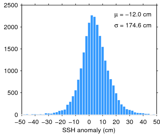
Figure 7. Histogram of flag-valid SSH anomaly over oceans and lakes for 25/08/2016. The mean ( \mu ) and standard deviation ( \sigma ) are also shown. Note that values outside [-50 50] cm are excluded from the histogram for the sake of readability but not from the computation of \mu and \sigma .
