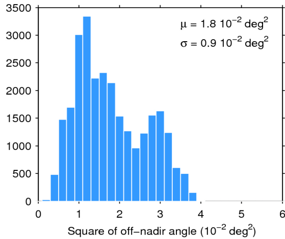
Figure 39. Histogram of flag-valid mispointing over oceans and lakes for 25/08/2016. The mean ( \mu ) and standard deviation ( \sigma ) are also shown. Note that values larger than 6 \cdot 10^{-2} \text{ deg}^2 are excluded from the histogram for the sake of readability but not from the computation of \mu and \sigma .
