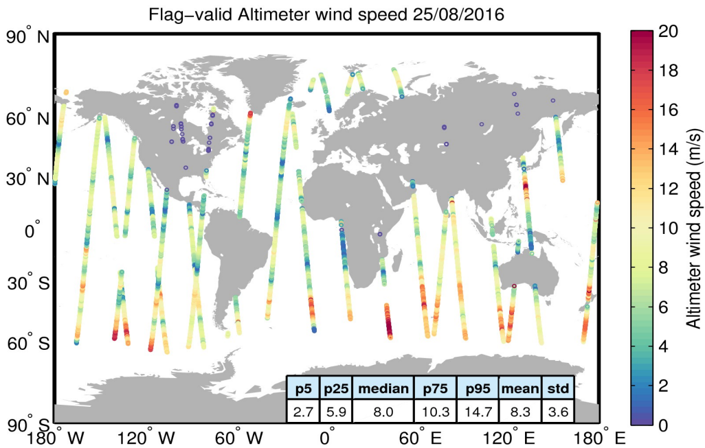
Figure 31. Geographical distribution of flag-valid wind data over oceans and lakes for 25/08/2016. The statistical values shown in the table refer to the wind in m/s and are calculated over all measurements shown in the figure.
