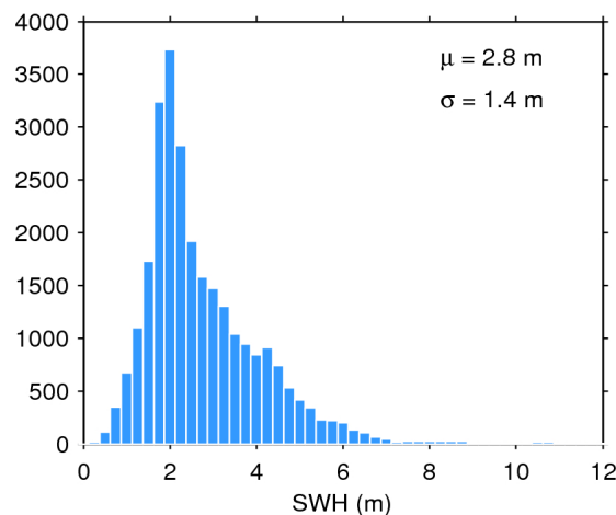
Figure 20. Histogram of science-valid SWH over oceans and lakes for 25/08/2016. The mean ( \mu ) and standard deviation ( \sigma ) are also shown. Note that values larger than 12 m are excluded from the histogram for the sake of readability but not from the computation of \mu and \sigma .
