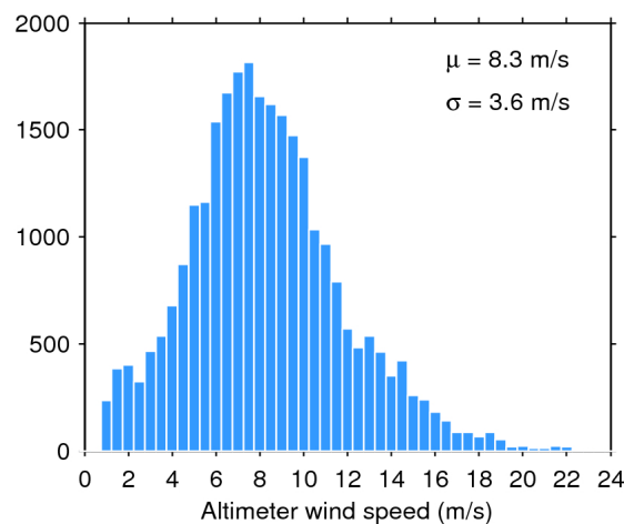
Figure 35. Histogram of science-valid wind over oceans and lakes for 25/08/2016. The mean ( \mu ) and standard deviation ( \sigma ) are also shown. Note that values larger than 24 m/s are excluded from the histogram for the sake of readability but not from the computation of \mu and \sigma .
