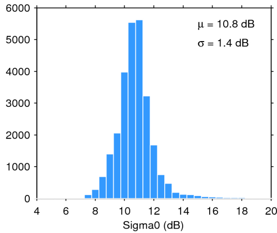
Figure 28. Histogram of science-valid sigma0 over oceans and lakes for 25/08/2016. The mean ( \mu ) and standard deviation ( \sigma ) are also shown. Note that values outside [4 20] dB are excluded from the histogram for the sake of readability but not from the computation of \mu and \sigma .
