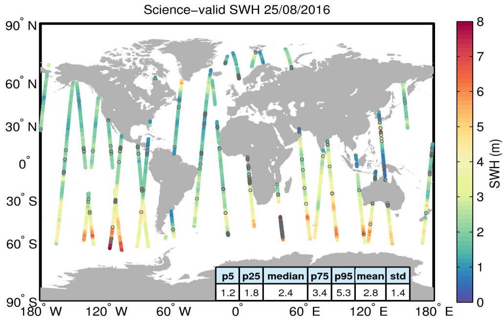
Figure 19. Geographical distribution of science-valid SWH data over oceans and lakes for 25/08/2016. The statistical values shown in the table refer to the SWH in m and are calculated over all measurements shown in the figure. Gray circles denote records that have been rejected based on the editing criteria described in Table 3.
