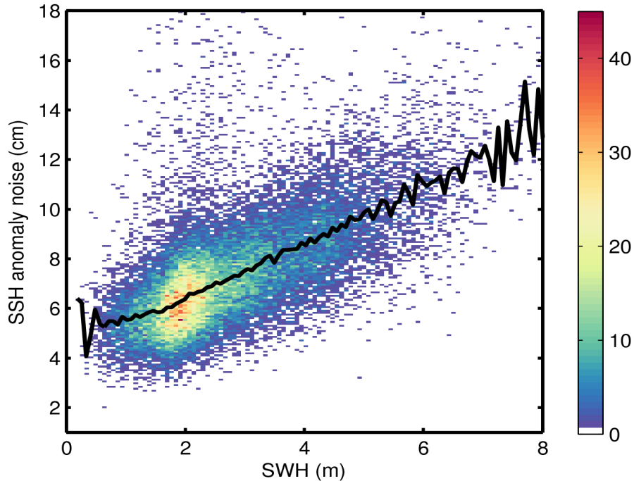
Figure 9. 2D histogram showing flag-valid SSH anomaly noise as a function of SWH for 25/08/2016. The black line denotes the median SSH anomaly noise as a function of SWH.
