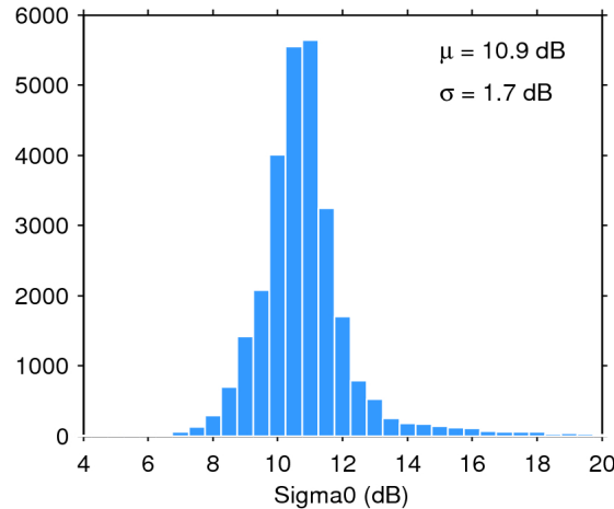
Figure 25. Histogram of flag-valid sigma0 over oceans and lakes for 25/08/2016. The mean ( \mu ) and standard deviation ( \sigma ) are also shown. Note that values outside [4 20] dB are excluded from the histogram for the sake of readability but not from the computation of \mu and \sigma .
