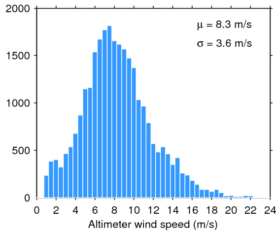
Figure 33. Histogram of flag-valid wind over oceans and lakes for 25/08/2016. The mean ( \mu ) and standard deviation ( \sigma ) are also shown. Note that values larger than 24 m/s are excluded from the histogram for the sake of readability but not from the computation of \mu and \sigma .
