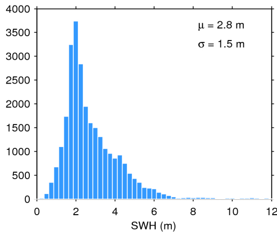
Figure 17. Histogram of flag-valid SWH over oceans and lakes for 25/08/2016. The mean ( \mu ) and standard deviation ( \sigma ) are also shown. Note that values larger than 12 m are excluded from the histogram for the sake of readability but not from the computation of \mu and \sigma .
