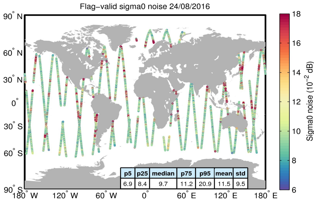
Figure 26. Geographical distribution of flag-valid 20-Hz sigma0 measurement noise over oceans and lakes for 24/08/2016. The statistical values shown in the table refer to the sigma0 noise and are calculated over all measurements shown in the figure.
