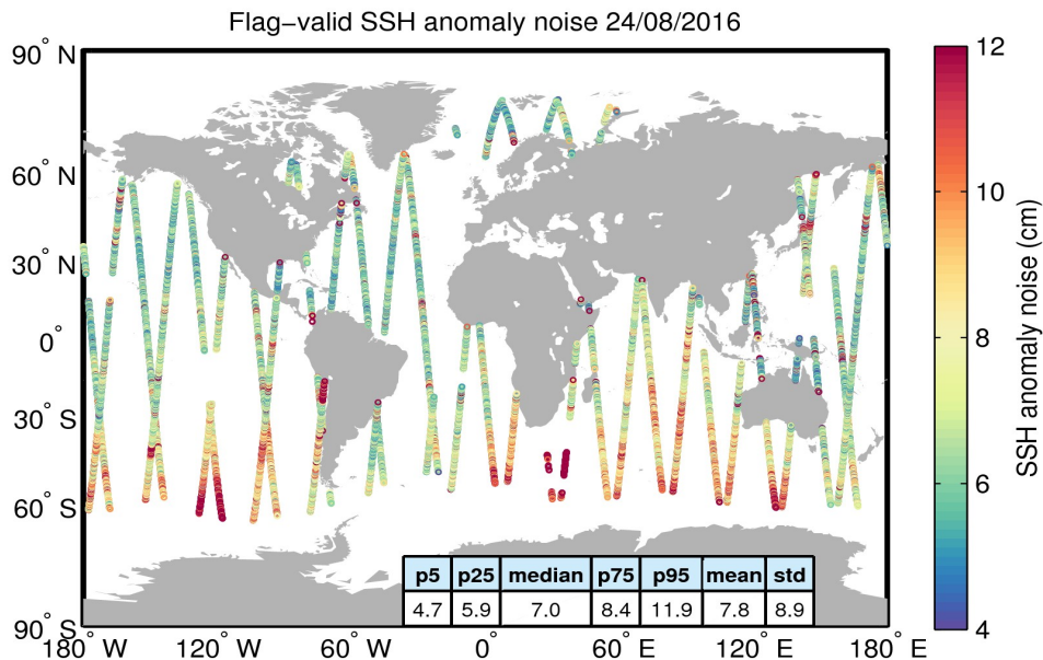
Figure 8. Geographical distribution of flag-valid 20-Hz SSH anomaly measurement noise over oceans and lakes for 24/08/2016. The statistical values shown in the table refer to the SSH anomaly noise and are calculated over all measurements shown in the figure.
