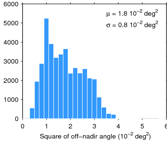
Figure 39. Histogram of flag-valid mispointing over oceans and lakes for 24/08/2016. The mean ( \mu ) and standard deviation ( \sigma ) are also shown. Note that values larger than 6 \cdot 10^{-2} \text{ deg}^2 are excluded from the histogram for the sake of readability but not from the computation of \mu and \sigma .
