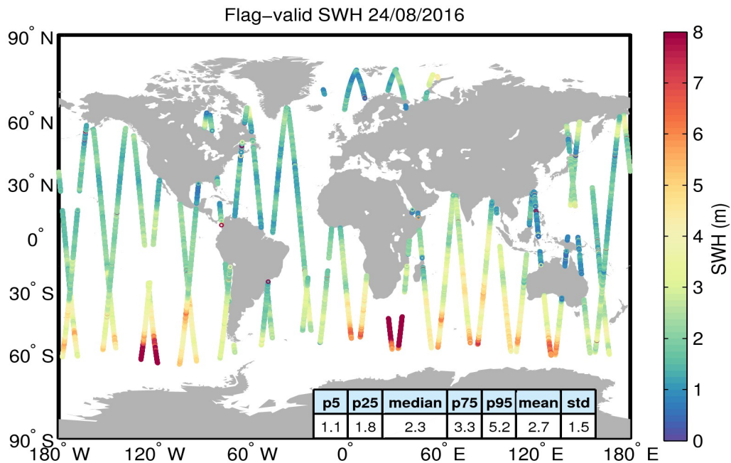
Figure 15. Geographical distribution of flag-valid SWH data over oceans and lakes for 24/08/2016. The statistical values shown in the table refer to the SWH in m and are calculated over all measurements shown in the figure.
