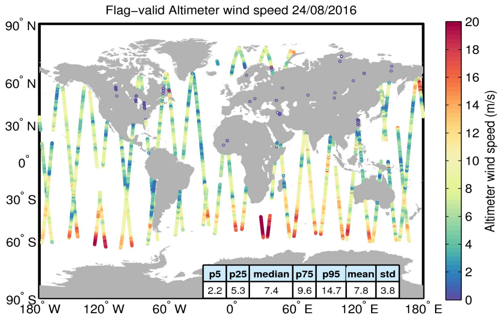
Figure 31. Geographical distribution of flag-valid wind data over oceans and lakes for 24/08/2016. The statistical values shown in the table refer to the wind in m/s and are calculated over all measurements shown in the figure.
