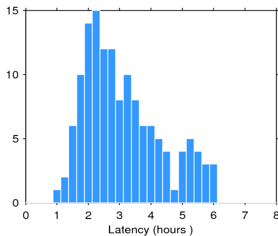
Figure 2. Histogram of the data latency for 24/08/2016. The y-axis denotes the number of files that are made available with a delay of x-hours with respect to the mean time of the records stored in the file.
