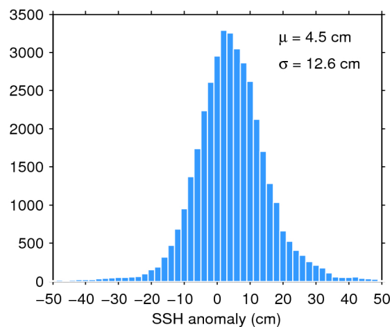
Figure 11. Histogram of science-valid SSH anomaly over oceans and lakes for 24/08/2016. The mean ( \mu ) and standard deviation ( \sigma ) are also shown. Note that values outside [-50 50] cm are excluded from the histogram for the sake of readability but not from the computation of \mu and \sigma .
