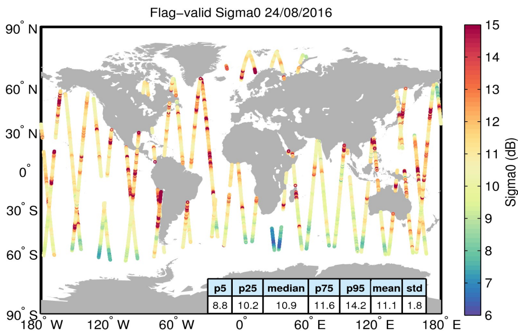
Figure 23. Geographical distribution of flag-valid sigma0 data over oceans and lakes for 24/08/2016. The statistical values shown in the table refer to the sigma0 in dB and are calculated over all measurements shown in the figure.
