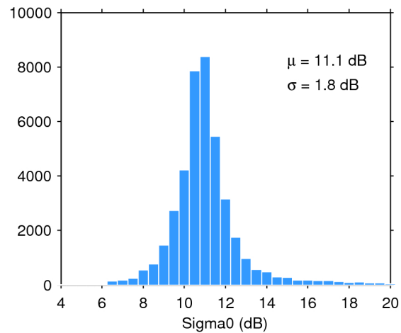
Figure 25. Histogram of flag-valid sigma0 over oceans and lakes for 24/08/2016. The mean ( \mu ) and standard deviation ( \sigma ) are also shown. Note that values outside [4 20] dB are excluded from the histogram for the sake of readability but not from the computation of \mu and \sigma .
