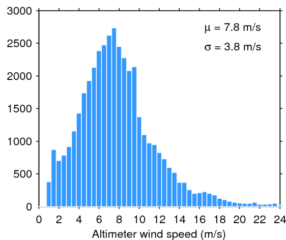
Figure 35. Histogram of science-valid wind over oceans and lakes for 24/08/2016. The mean ( \mu ) and standard deviation ( \sigma ) are also shown. Note that values larger than 24 m/s are excluded from the histogram for the sake of readability but not from the computation of \mu and \sigma .
