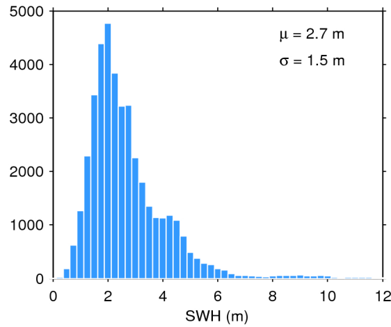
Figure 17. Histogram of flag-valid SWH over oceans and lakes for 24/08/2016. The mean ( \mu ) and standard deviation ( \sigma ) are also shown. Note that values larger than 12 m are excluded from the histogram for the sake of readability but not from the computation of \mu and \sigma .
