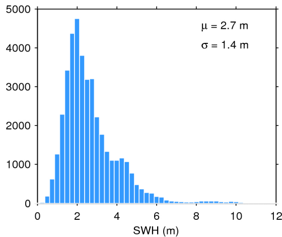
Figure 20. Histogram of science-valid SWH over oceans and lakes for 24/08/2016. The mean ( \mu ) and standard deviation ( \sigma ) are also shown. Note that values larger than 12 m are excluded from the histogram for the sake of readability but not from the computation of \mu and \sigma .
