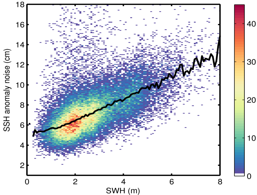
Figure 9. 2D histogram showing flag-valid SSH anomaly noise as a function of SWH for 24/08/2016. The black line denotes the median SSH anomaly noise as a function of SWH.
