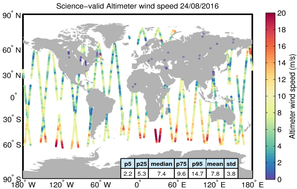
Figure 34. Geographical distribution of science-valid wind data over oceans and lakes for 24/08/2016. The statistical values shown in the table refer to the wind in m/s and are calculated over all measurements shown in the figure. Gray circles denote records that have been rejected based on the editing criteria described in Table 5.
