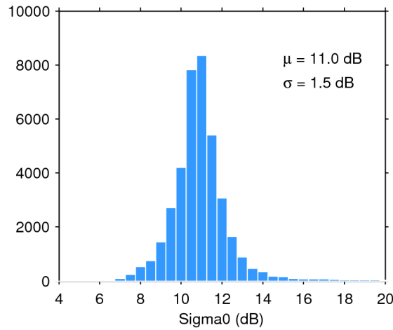
Figure 28. Histogram of science-valid sigma0 over oceans and lakes for 24/08/2016. The mean ( \mu ) and standard deviation ( \sigma ) are also shown. Note that values outside [4 20] dB are excluded from the histogram for the sake of readability but not from the computation of \mu and \sigma .
