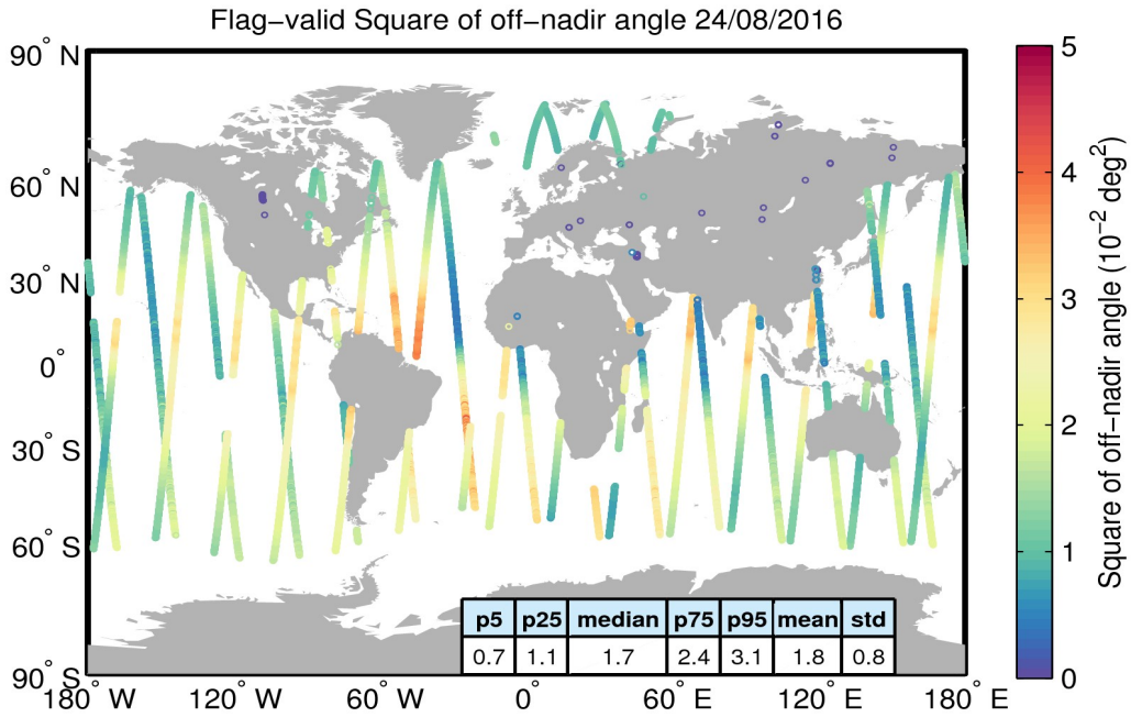
Figure 37. Geographical distribution of flag-valid mispointing data over oceans and lakes for 24/08/2016. The statistical values shown in the table refer to the mispointing in 10^{-2} deg 2 and are calculated over all measurements shown in the figure.
