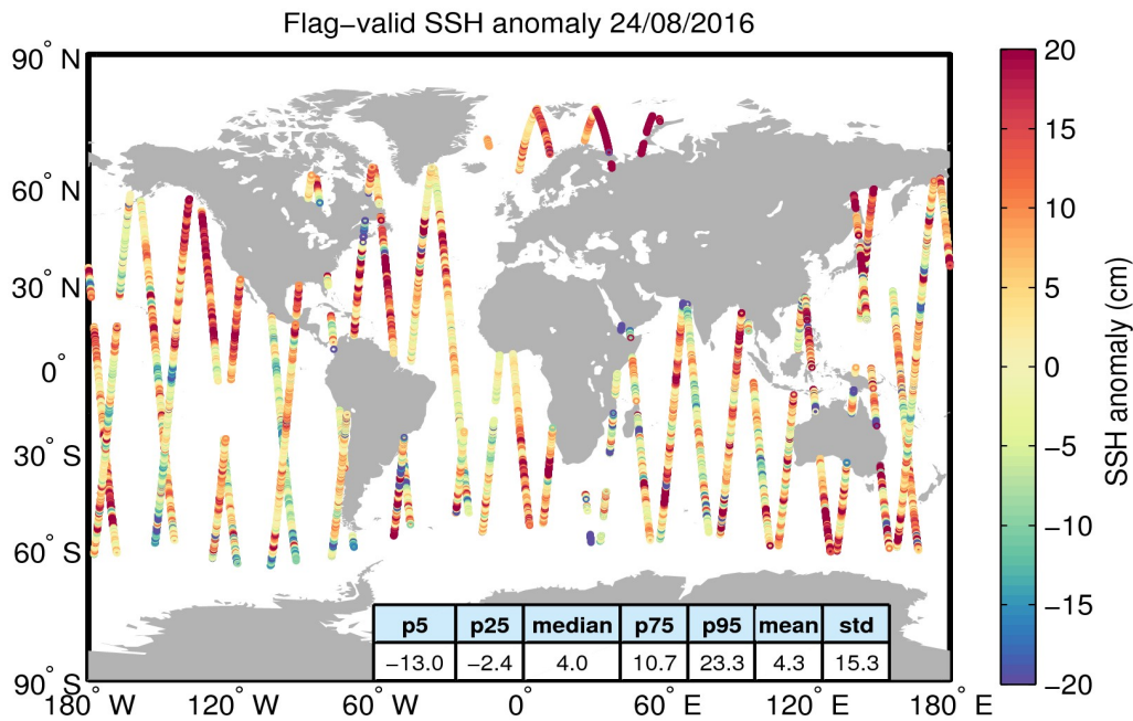
Figure 5. Geographical distribution of flag-valid 1-Hz SSH anomaly data over oceans and lakes for 24/08/2016. The statistical values shown in the table refer to the SSH anomaly in cm and are calculated over all measurements shown in the figure.
