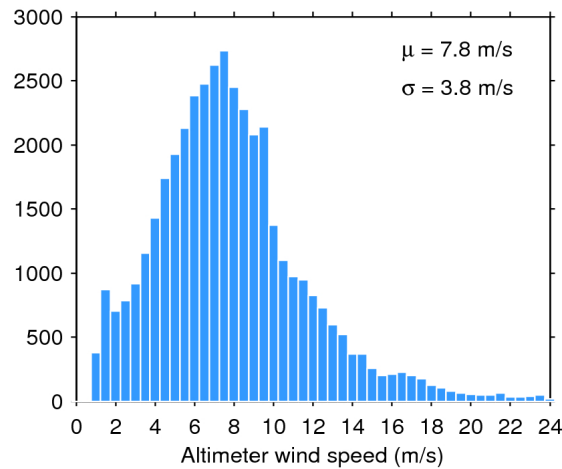
Figure 33. Histogram of flag-valid wind over oceans and lakes for 24/08/2016. The mean ( \mu ) and standard deviation ( \sigma ) are also shown. Note that values larger than 24 m/s are excluded from the histogram for the sake of readability but not from the computation of \mu and \sigma .
