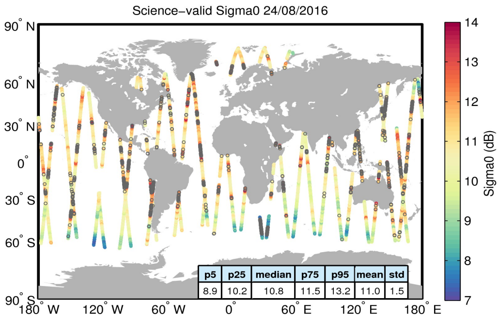
Figure 27. Geographical distribution of science-valid sigma0 data over oceans and lakes for 24/08/2016. The statistical values shown in the table refer to the sigma0 in dB and are calculated over all measurements shown in the figure. Gray circles denote records that have been rejected based on the editing criteria described in Table 4.
