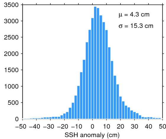
Figure 7. Histogram of flag-valid SSH anomaly over oceans and lakes for 24/08/2016. The mean ( \mu ) and standard deviation ( \sigma ) are also shown. Note that values outside [-50 50] cm are excluded from the histogram for the sake of readability but not from the computation of \mu and \sigma .
