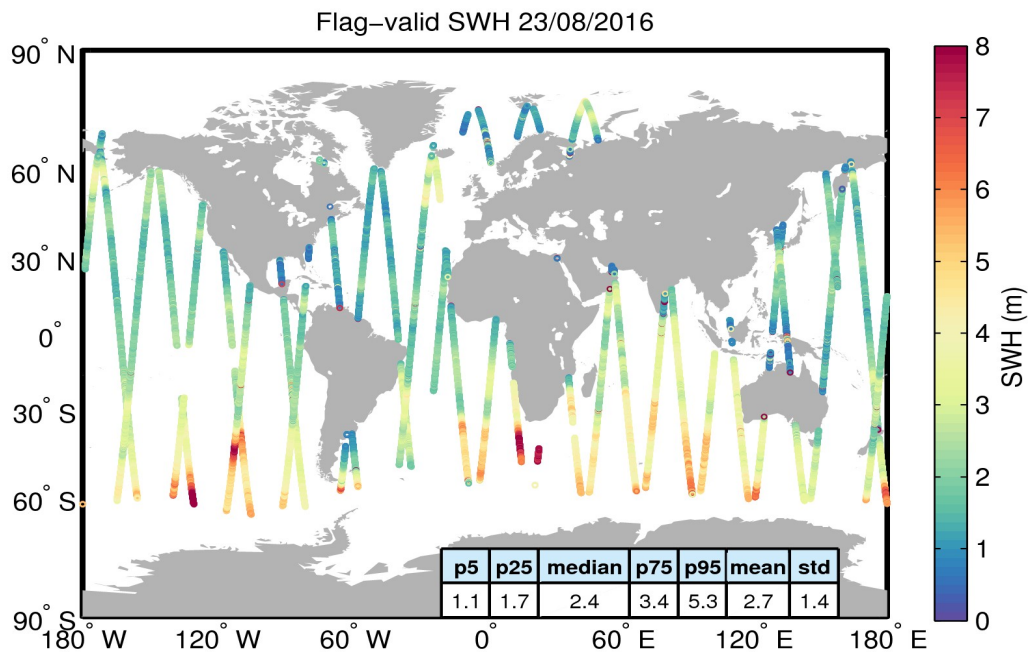
Figure 15. Geographical distribution of flag-valid SWH data over oceans and lakes for 23/08/2016. The statistical values shown in the table refer to the SWH in m and are calculated over all measurements shown in the figure.
