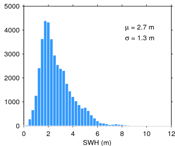
Figure 20. Histogram of science-valid SWH over oceans and lakes for 23/08/2016. The mean ( \mu ) and standard deviation ( \sigma ) are also shown. Note that values larger than 12 m are excluded from the histogram for the sake of readability but not from the computation of \mu and \sigma .
