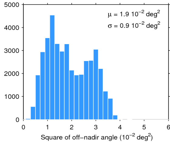
Figure 39. Histogram of flag-valid mispointing over oceans and lakes for 23/08/2016. The mean ( \mu ) and standard deviation ( \sigma ) are also shown. Note that values larger than 6 \cdot 10^{-2} \text{ deg}^2 are excluded from the histogram for the sake of readability but not from the computation of \mu and \sigma .
