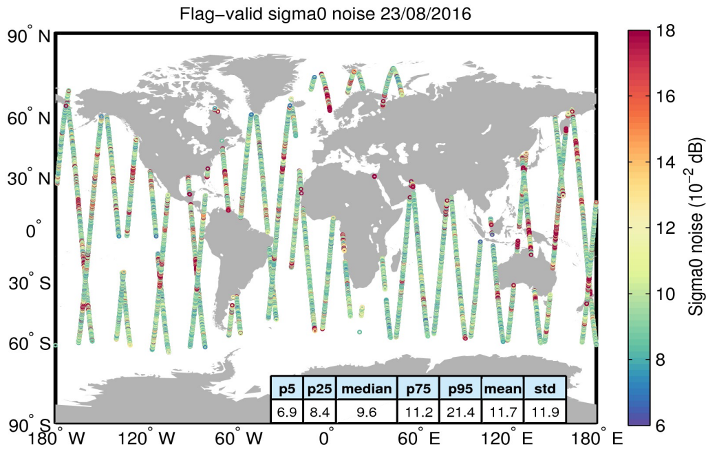
Figure 26. Geographical distribution of flag-valid 20-Hz sigma0 measurement noise over oceans and lakes for 23/08/2016. The statistical values shown in the table refer to the sigma0 noise and are calculated over all measurements shown in the figure.
