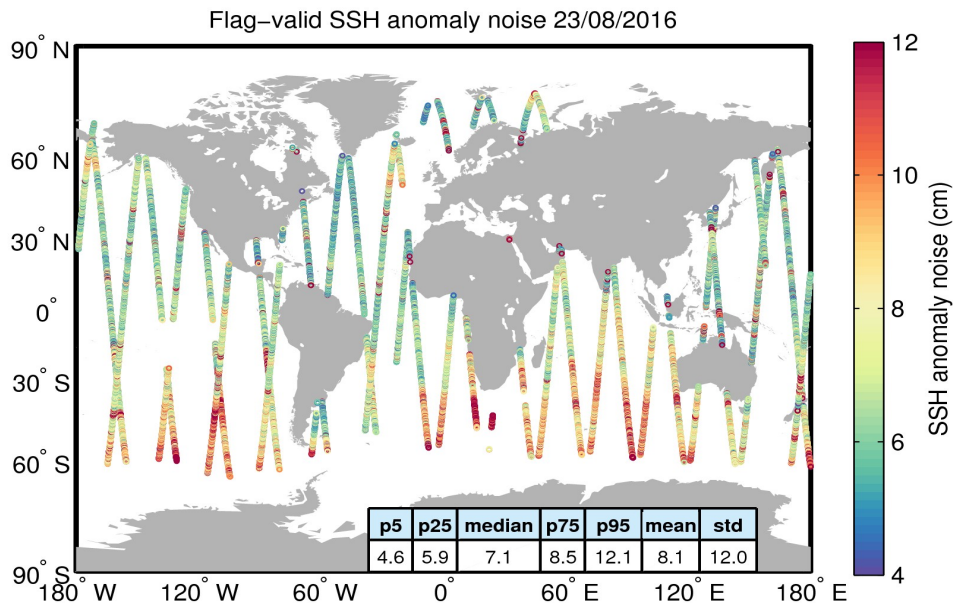
Figure 8. Geographical distribution of flag-valid 20-Hz SSH anomaly measurement noise over oceans and lakes for 23/08/2016. The statistical values shown in the table refer to the SSH anomaly noise and are calculated over all measurements shown in the figure.
