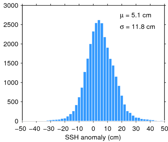
Figure 11. Histogram of science-valid SSH anomaly over oceans and lakes for 23/08/2016. The mean ( \mu ) and standard deviation ( \sigma ) are also shown. Note that values outside [-50 50] cm are excluded from the histogram for the sake of readability but not from the computation of \mu and \sigma .
