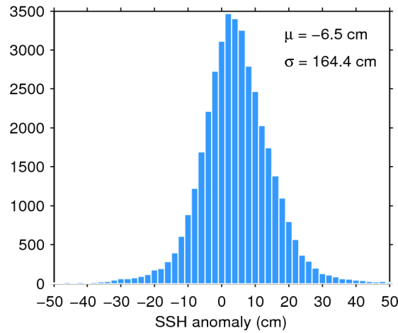
Figure 7. Histogram of flag-valid SSH anomaly over oceans and lakes for 23/08/2016. The mean ( \mu ) and standard deviation ( \sigma ) are also shown. Note that values outside [-50 50] cm are excluded from the histogram for the sake of readability but not from the computation of \mu and \sigma .
