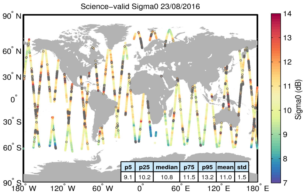
Figure 27. Geographical distribution of science-valid sigma0 data over oceans and lakes for 23/08/2016. The statistical values shown in the table refer to the sigma0 in dB and are calculated over all measurements shown in the figure. Gray circles denote records that have been rejected based on the editing criteria described in Table 4.
