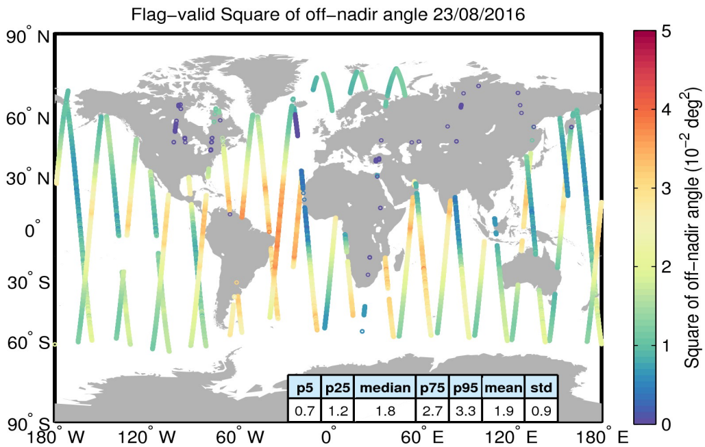
Figure 37. Geographical distribution of flag-valid mispointing data over oceans and lakes for 23/08/2016. The statistical values shown in the table refer to the mispointing in 10^{-2} deg 2 and are calculated over all measurements shown in the figure.
