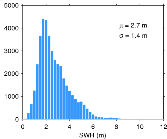
Figure 17. Histogram of flag-valid SWH over oceans and lakes for 23/08/2016. The mean ( \mu ) and standard deviation ( \sigma ) are also shown. Note that values larger than 12 m are excluded from the histogram for the sake of readability but not from the computation of \mu and \sigma .
