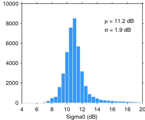
Figure 25. Histogram of flag-valid sigma0 over oceans and lakes for 23/08/2016. The mean ( \mu ) and standard deviation ( \sigma ) are also shown. Note that values outside [4 20] dB are excluded from the histogram for the sake of readability but not from the computation of \mu and \sigma .
