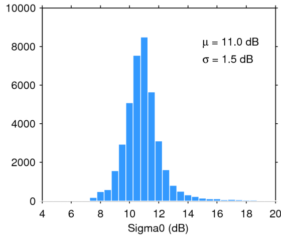
Figure 28. Histogram of science-valid sigma0 over oceans and lakes for 23/08/2016. The mean ( \mu ) and standard deviation ( \sigma ) are also shown. Note that values outside [4 20] dB are excluded from the histogram for the sake of readability but not from the computation of \mu and \sigma .
