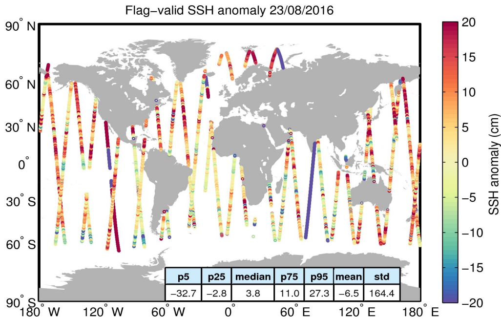
Figure 5. Geographical distribution of flag-valid 1-Hz SSH anomaly data over oceans and lakes for 23/08/2016. The statistical values shown in the table refer to the SSH anomaly in cm and are calculated over all measurements shown in the figure.
