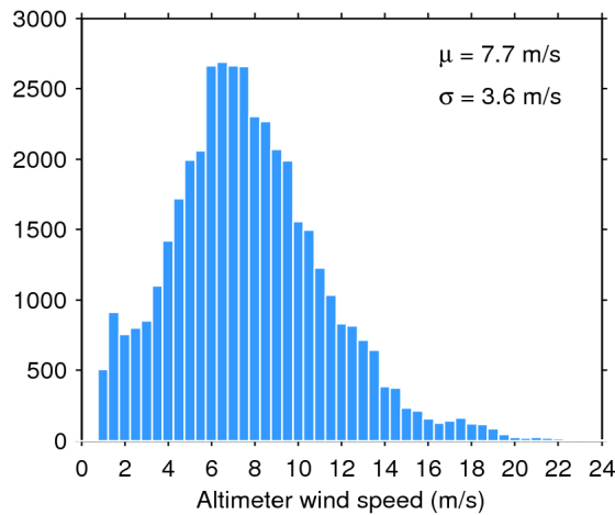
Figure 33. Histogram of flag-valid wind over oceans and lakes for 23/08/2016. The mean ( \mu ) and standard deviation ( \sigma ) are also shown. Note that values larger than 24 m/s are excluded from the histogram for the sake of readability but not from the computation of \mu and \sigma .
