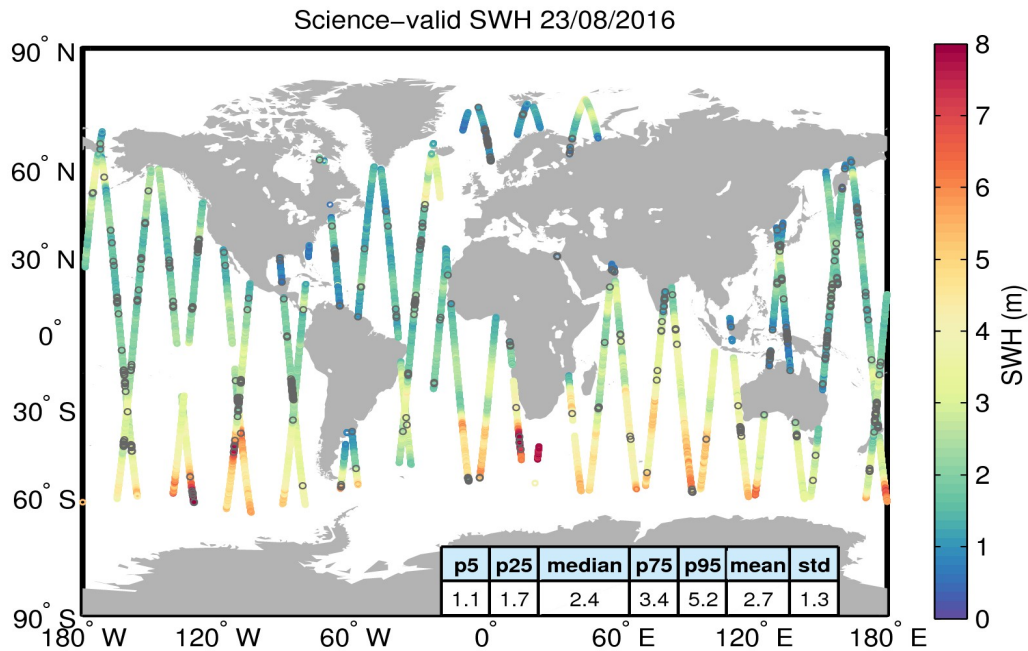
Figure 19. Geographical distribution of science-valid SWH data over oceans and lakes for 23/08/2016. The statistical values shown in the table refer to the SWH in m and are calculated over all measurements shown in the figure. Gray circles denote records that have been rejected based on the editing criteria described in Table 3.
