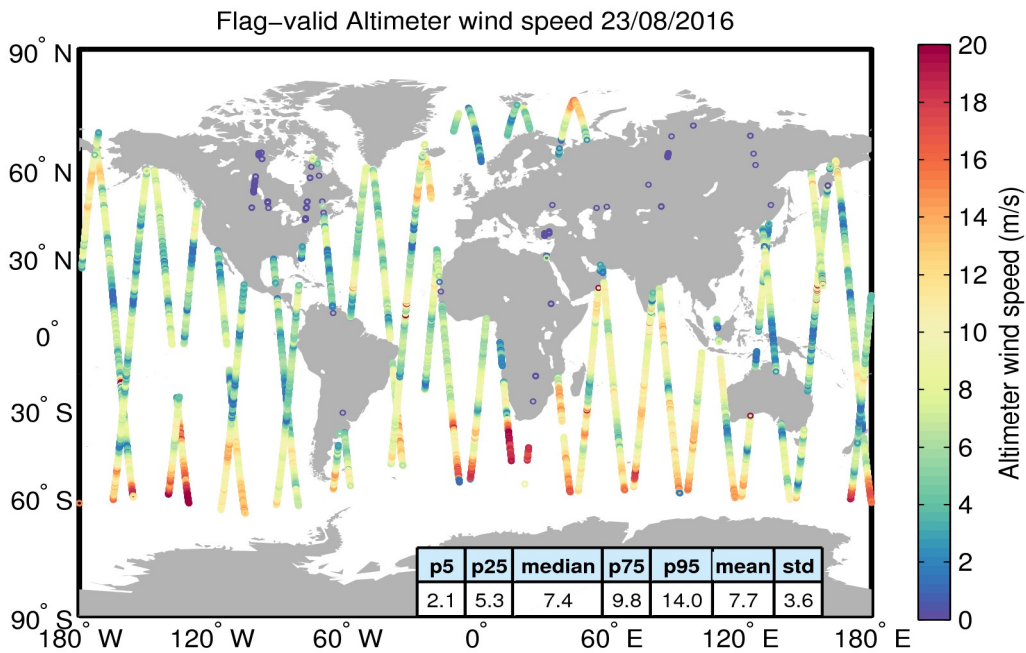
Figure 31. Geographical distribution of flag-valid wind data over oceans and lakes for 23/08/2016. The statistical values shown in the table refer to the wind in m/s and are calculated over all measurements shown in the figure.
