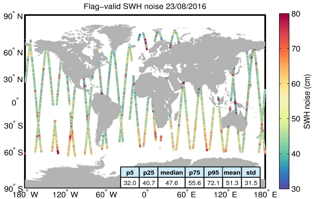
Figure 18. Geographical distribution of flag-valid 20-Hz SWH measurement noise over oceans and lakes for 23/08/2016. The statistical values shown in the table refer to the SWH noise and are calculated over all measurements shown in the figure.
