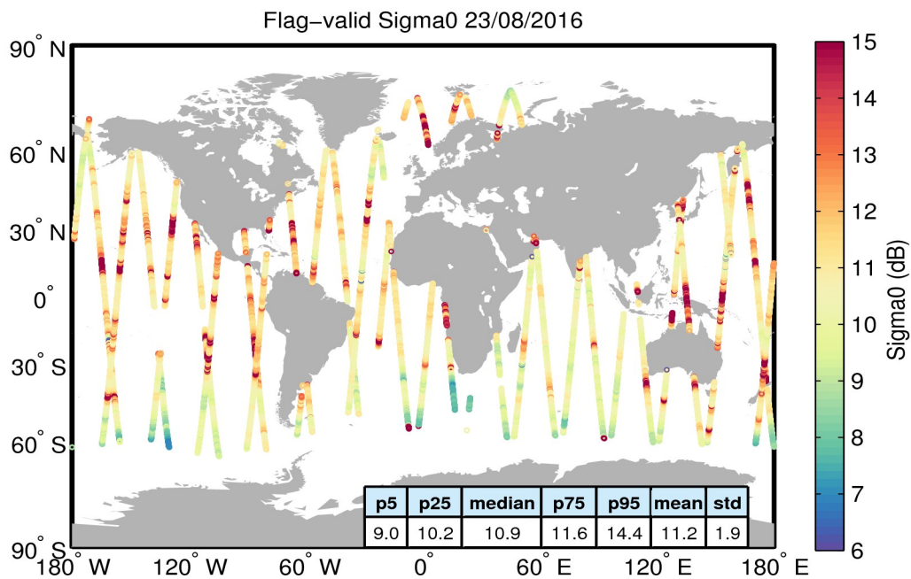
Figure 23. Geographical distribution of flag-valid sigma0 data over oceans and lakes for 23/08/2016. The statistical values shown in the table refer to the sigma0 in dB and are calculated over all measurements shown in the figure.
