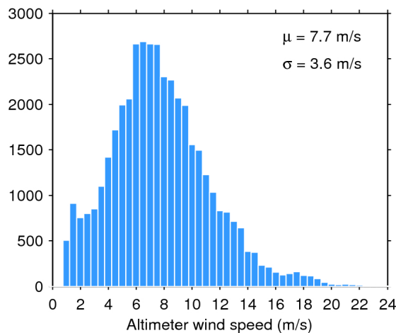
Figure 35. Histogram of science-valid wind over oceans and lakes for 23/08/2016. The mean ( \mu ) and standard deviation ( \sigma ) are also shown. Note that values larger than 24 m/s are excluded from the histogram for the sake of readability but not from the computation of \mu and \sigma .
