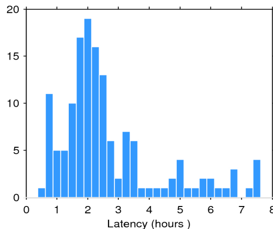
Figure 2. Histogram of the data latency for 23/08/2016. The y-axis denotes the number of files that are made available with a delay of x-hours with respect to the mean time of the records stored in the file.
