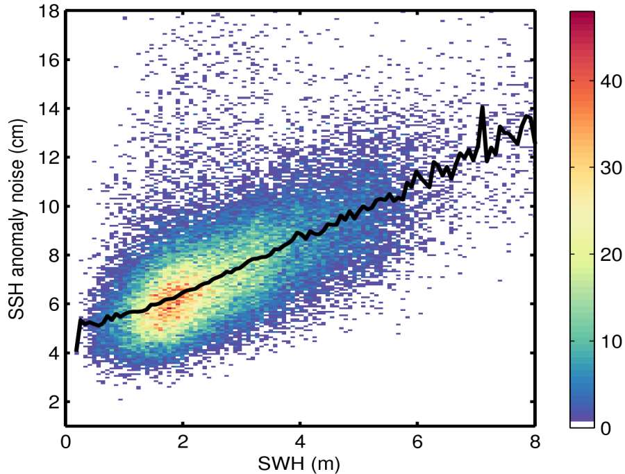
Figure 9. 2D histogram showing flag-valid SSH anomaly noise as a function of SWH for 23/08/2016. The black line denotes the median SSH anomaly noise as a function of SWH.
