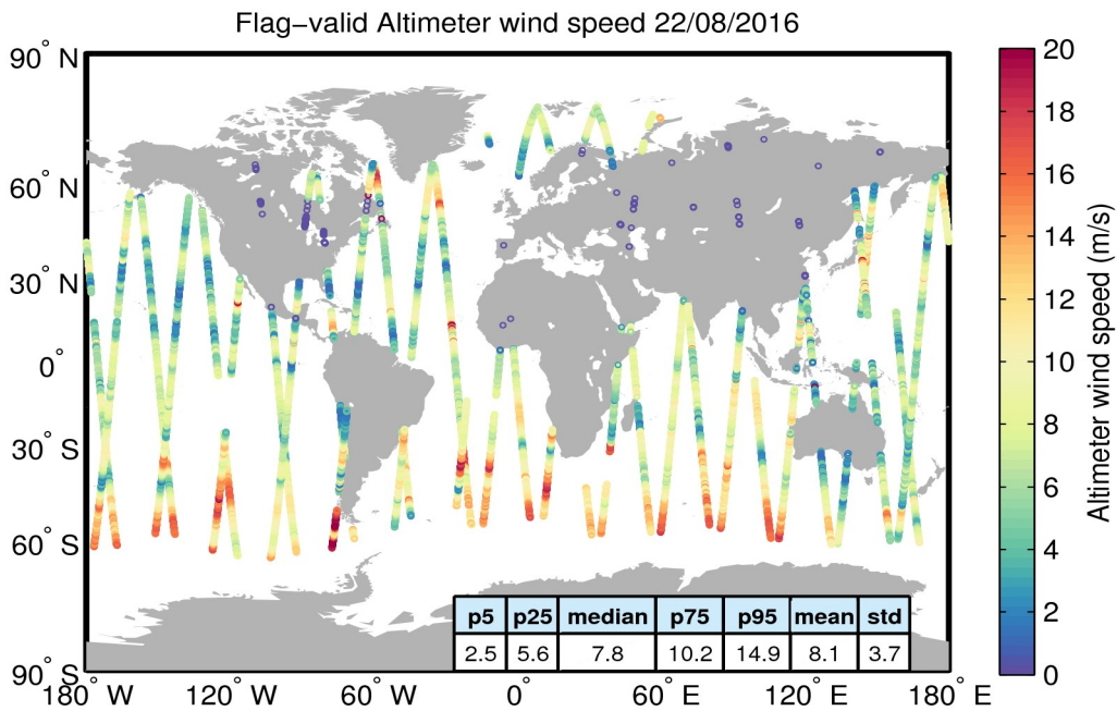
Figure 31. Geographical distribution of flag-valid wind data over oceans and lakes for 22/08/2016. The statistical values shown in the table refer to the wind in m/s and are calculated over all measurements shown in the figure.
