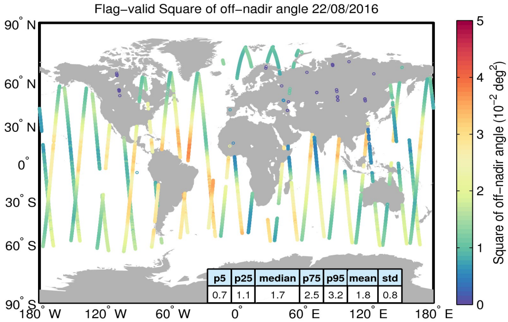
Figure 37. Geographical distribution of flag-valid mispointing data over oceans and lakes for 22/08/2016. The statistical values shown in the table refer to the mispointing in 10^{-2} deg 2 and are calculated over all measurements shown in the figure.
