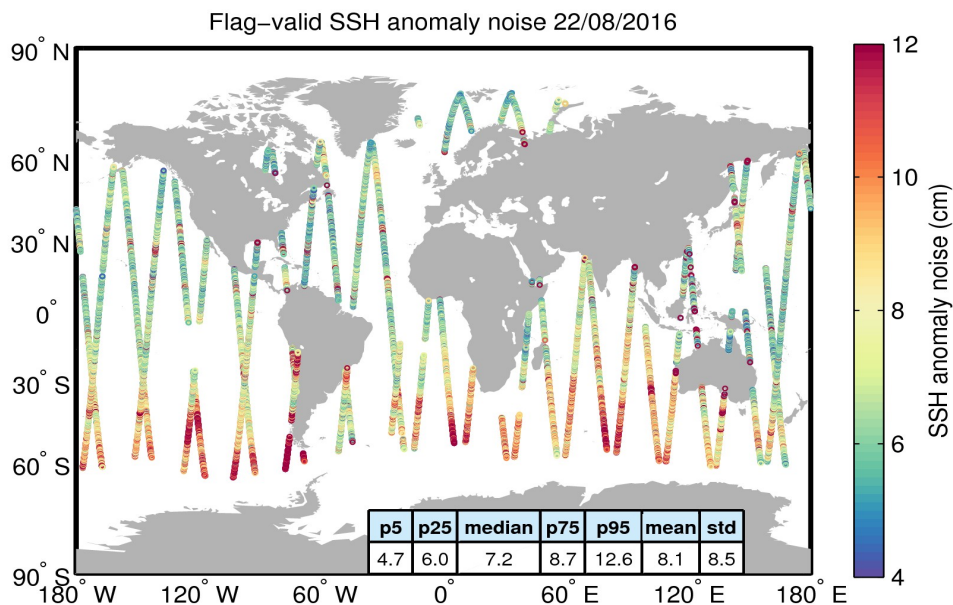
Figure 8. Geographical distribution of flag-valid 20-Hz SSH anomaly measurement noise over oceans and lakes for 22/08/2016. The statistical values shown in the table refer to the SSH anomaly noise and are calculated over all measurements shown in the figure.
