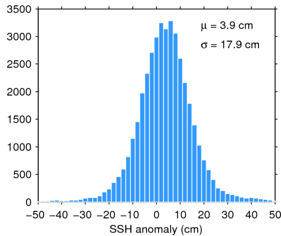
Figure 7. Histogram of flag-valid SSH anomaly over oceans and lakes for 22/08/2016. The mean ( \mu ) and standard deviation ( \sigma ) are also shown. Note that values outside [-50 50] cm are excluded from the histogram for the sake of readability but not from the computation of \mu and \sigma .
