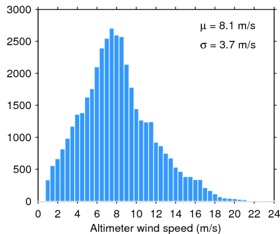
Figure 35. Histogram of science-valid wind over oceans and lakes for 22/08/2016. The mean ( \mu ) and standard deviation ( \sigma ) are also shown. Note that values larger than 24 m/s are excluded from the histogram for the sake of readability but not from the computation of \mu and \sigma .
