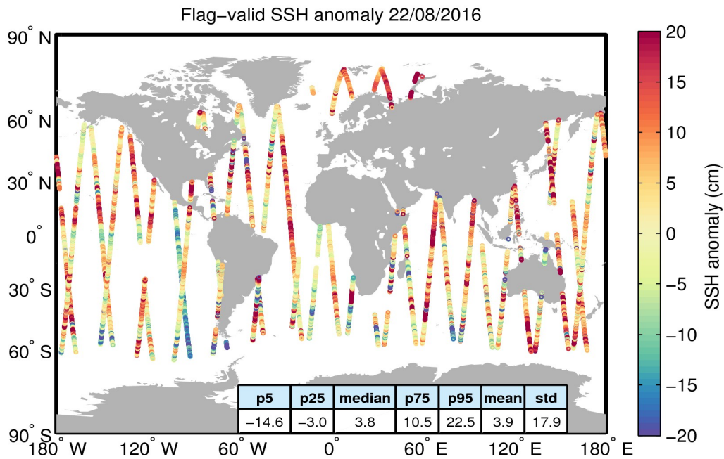
Figure 5. Geographical distribution of flag-valid 1-Hz SSH anomaly data over oceans and lakes for 22/08/2016. The statistical values shown in the table refer to the SSH anomaly in cm and are calculated over all measurements shown in the figure.
