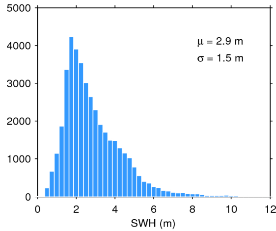
Figure 17. Histogram of flag-valid SWH over oceans and lakes for 22/08/2016. The mean ( \mu ) and standard deviation ( \sigma ) are also shown. Note that values larger than 12 m are excluded from the histogram for the sake of readability but not from the computation of \mu and \sigma .
