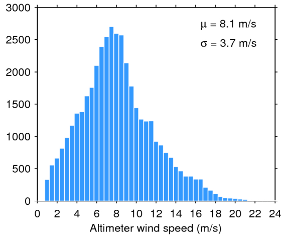
Figure 33. Histogram of flag-valid wind over oceans and lakes for 22/08/2016. The mean ( \mu ) and standard deviation ( \sigma ) are also shown. Note that values larger than 24 m/s are excluded from the histogram for the sake of readability but not from the computation of \mu and \sigma .
