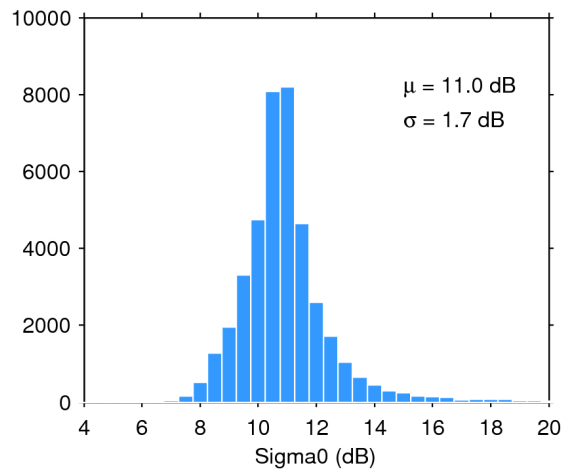
Figure 25. Histogram of flag-valid sigma0 over oceans and lakes for 22/08/2016. The mean ( \mu ) and standard deviation ( \sigma ) are also shown. Note that values outside [4 20] dB are excluded from the histogram for the sake of readability but not from the computation of \mu and \sigma .
