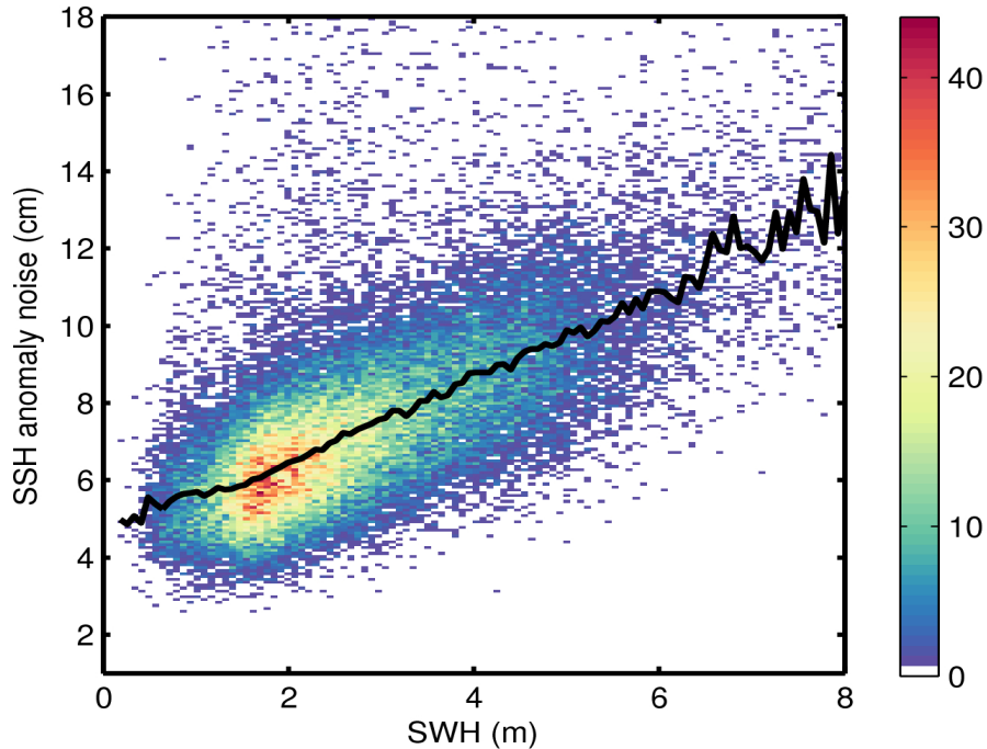
Figure 9. 2D histogram showing flag-valid SSH anomaly noise as a function of SWH for 22/08/2016. The black line denotes the median SSH anomaly noise as a function of SWH.
