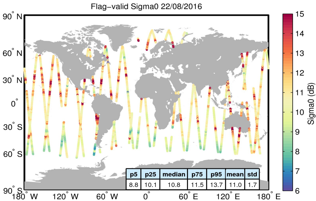
Figure 23. Geographical distribution of flag-valid sigma0 data over oceans and lakes for 22/08/2016. The statistical values shown in the table refer to the sigma0 in dB and are calculated over all measurements shown in the figure.
