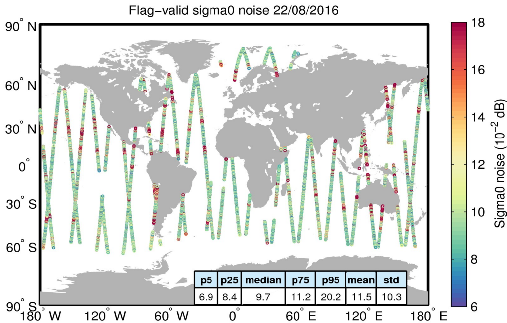
Figure 26. Geographical distribution of flag-valid 20-Hz sigma0 measurement noise over oceans and lakes for 22/08/2016. The statistical values shown in the table refer to the sigma0 noise and are calculated over all measurements shown in the figure.
