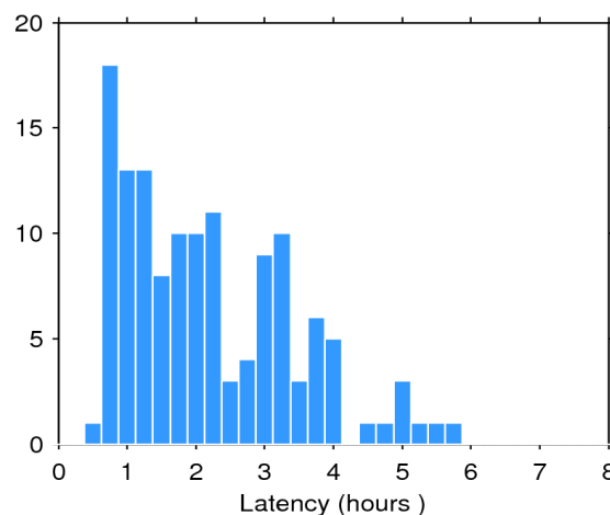
Figure 2. Histogram of the data latency for 22/08/2016. The y-axis denotes the number of files that are made available with a delay of x-hours with respect to the mean time of the records stored in the file.
