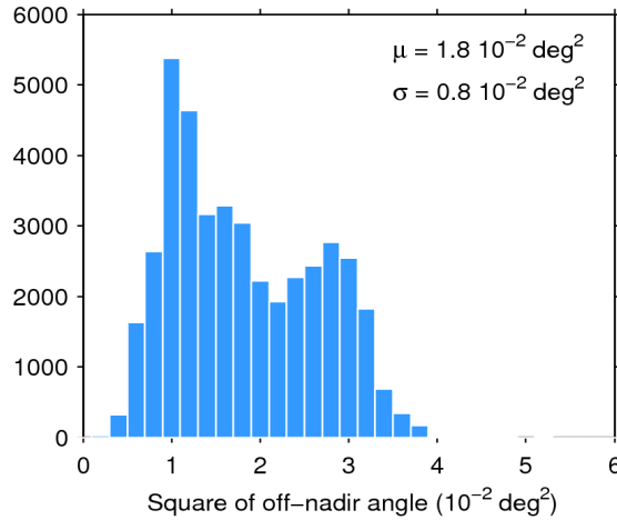
Figure 39. Histogram of flag-valid mispointing over oceans and lakes for 22/08/2016. The mean ( \mu ) and standard deviation ( \sigma ) are also shown. Note that values larger than 6 \cdot 10^{-2} \text{ deg}^2 are excluded from the histogram for the sake of readability but not from the computation of \mu and \sigma .
