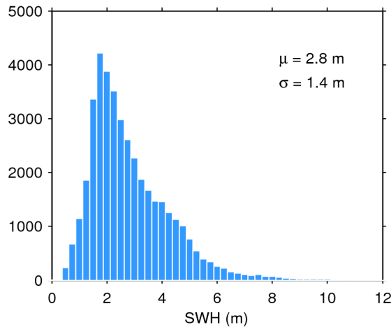
Figure 20. Histogram of science-valid SWH over oceans and lakes for 22/08/2016. The mean ( \mu ) and standard deviation ( \sigma ) are also shown. Note that values larger than 12 m are excluded from the histogram for the sake of readability but not from the computation of \mu and \sigma .
