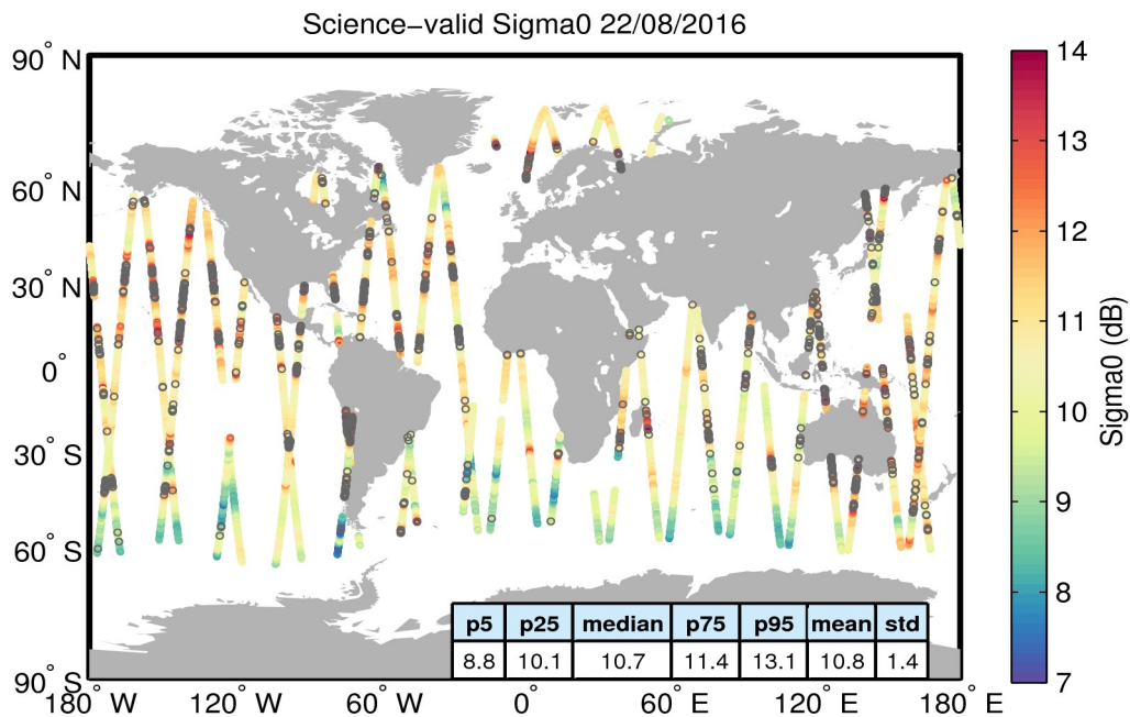
Figure 27. Geographical distribution of science-valid sigma0 data over oceans and lakes for 22/08/2016. The statistical values shown in the table refer to the sigma0 in dB and are calculated over all measurements shown in the figure. Gray circles denote records that have been rejected based on the editing criteria described in Table 4.
