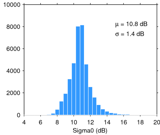
Figure 28. Histogram of science-valid sigma0 over oceans and lakes for 22/08/2016. The mean ( \mu ) and standard deviation ( \sigma ) are also shown. Note that values outside [4 20] dB are excluded from the histogram for the sake of readability but not from the computation of \mu and \sigma .
