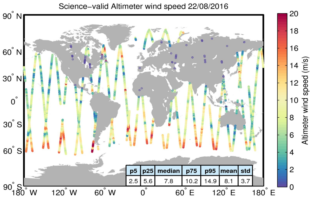
Figure 34. Geographical distribution of science-valid wind data over oceans and lakes for 22/08/2016. The statistical values shown in the table refer to the wind in m/s and are calculated over all measurements shown in the figure. Gray circles denote records that have been rejected based on the editing criteria described in Table 5.
