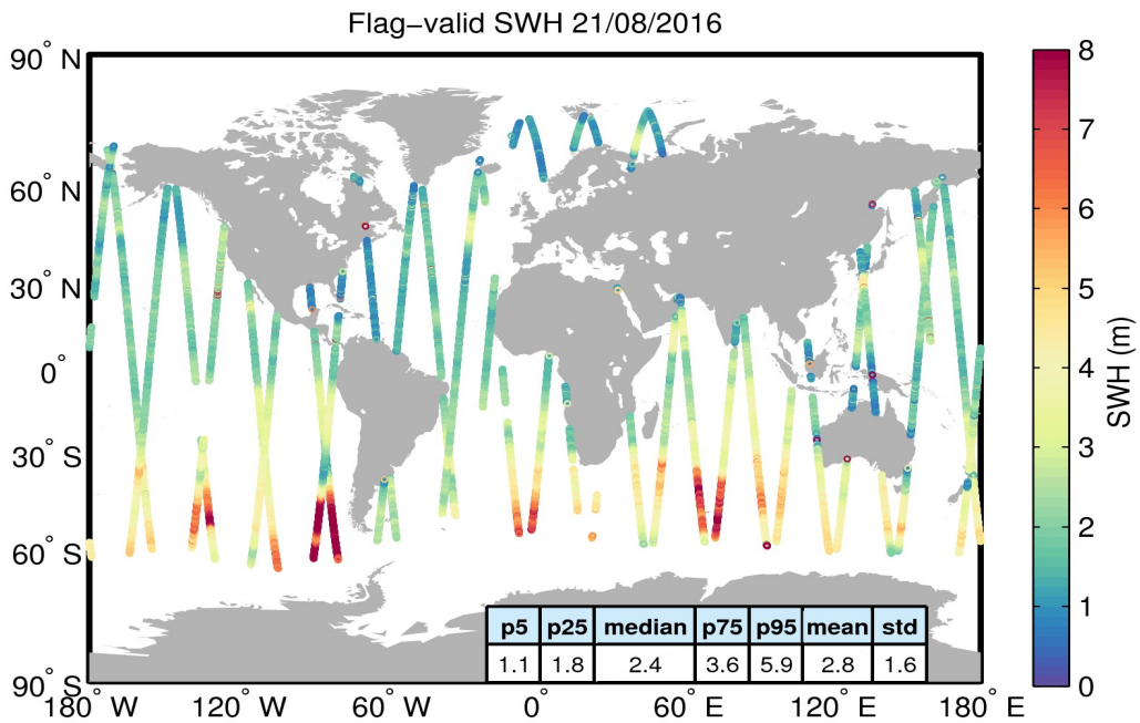
Figure 15. Geographical distribution of flag-valid SWH data over oceans and lakes for 21/08/2016. The statistical values shown in the table refer to the SWH in m and are calculated over all measurements shown in the figure.
