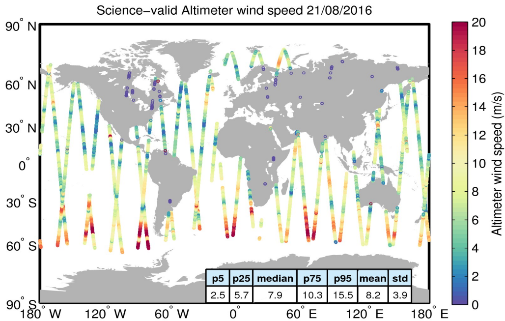
Figure 34. Geographical distribution of science-valid wind data over oceans and lakes for 21/08/2016. The statistical values shown in the table refer to the wind in m/s and are calculated over all measurements shown in the figure. Gray circles denote records that have been rejected based on the editing criteria described in Table 5.
