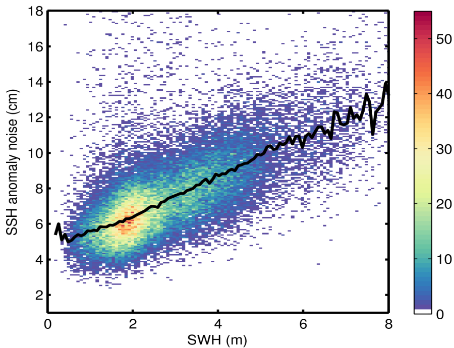
Figure 9. 2D histogram showing flag-valid SSH anomaly noise as a function of SWH for 21/08/2016. The black line denotes the median SSH anomaly noise as a function of SWH.
