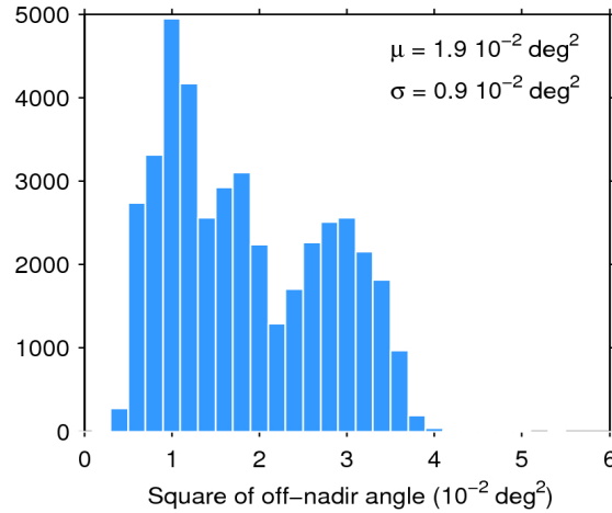
Figure 39. Histogram of flag-valid mispointing over oceans and lakes for 21/08/2016. The mean ( \mu ) and standard deviation ( \sigma ) are also shown. Note that values larger than 6 \cdot 10^{-2} \text{ deg}^2 are excluded from the histogram for the sake of readability but not from the computation of \mu and \sigma .
