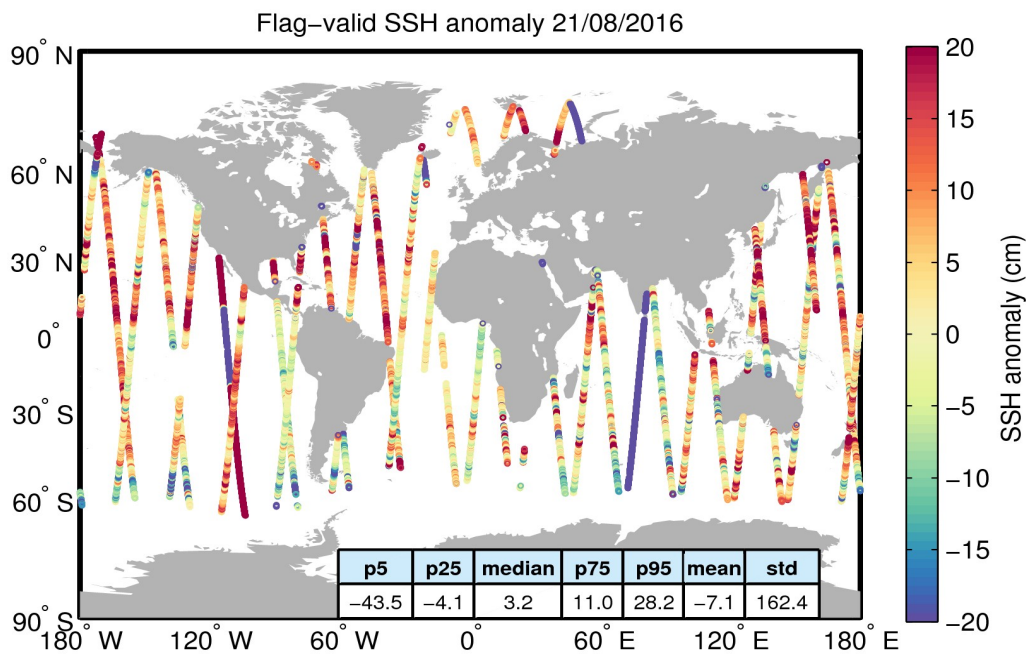
Figure 5. Geographical distribution of flag-valid 1-Hz SSH anomaly data over oceans and lakes for 21/08/2016. The statistical values shown in the table refer to the SSH anomaly in cm and are calculated over all measurements shown in the figure.
