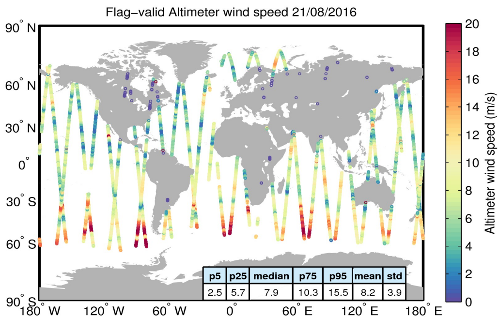
Figure 31. Geographical distribution of flag-valid wind data over oceans and lakes for 21/08/2016. The statistical values shown in the table refer to the wind in m/s and are calculated over all measurements shown in the figure.
