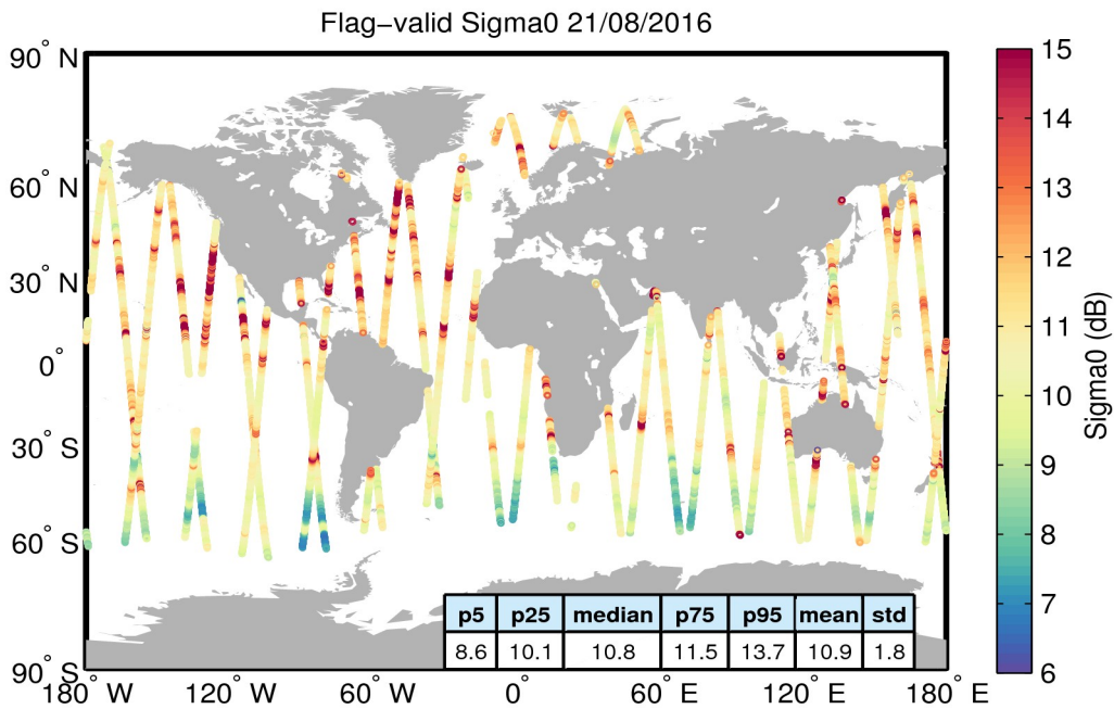
Figure 23. Geographical distribution of flag-valid sigma0 data over oceans and lakes for 21/08/2016. The statistical values shown in the table refer to the sigma0 in dB and are calculated over all measurements shown in the figure.
