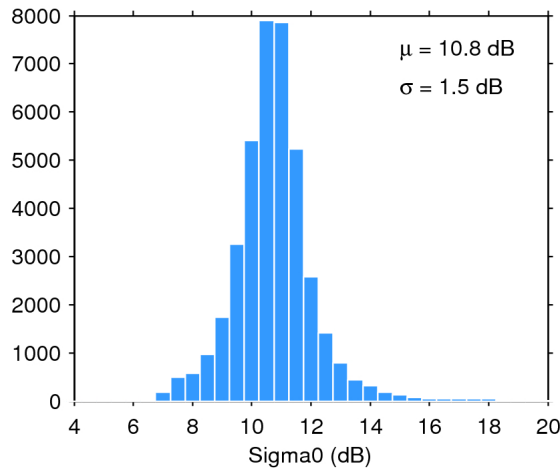
Figure 28. Histogram of science-valid sigma0 over oceans and lakes for 21/08/2016. The mean ( \mu ) and standard deviation ( \sigma ) are also shown. Note that values outside [4 20] dB are excluded from the histogram for the sake of readability but not from the computation of \mu and \sigma .
