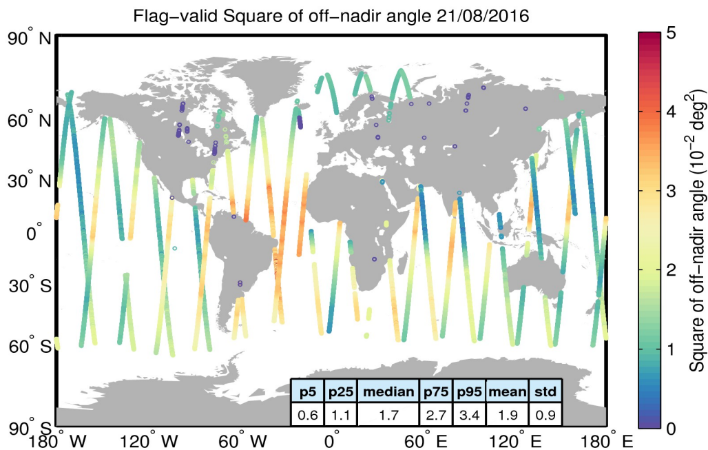
Figure 37. Geographical distribution of flag-valid mispointing data over oceans and lakes for 21/08/2016. The statistical values shown in the table refer to the mispointing in 10^{-2} deg 2 and are calculated over all measurements shown in the figure.
