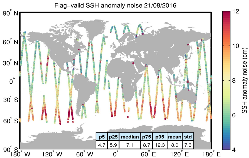
Figure 8. Geographical distribution of flag-valid 20-Hz SSH anomaly measurement noise over oceans and lakes for 21/08/2016. The statistical values shown in the table refer to the SSH anomaly noise and are calculated over all measurements shown in the figure.
