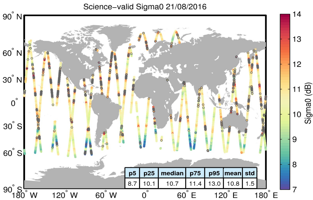
Figure 27. Geographical distribution of science-valid sigma0 data over oceans and lakes for 21/08/2016. The statistical values shown in the table refer to the sigma0 in dB and are calculated over all measurements shown in the figure. Gray circles denote records that have been rejected based on the editing criteria described in Table 4.
