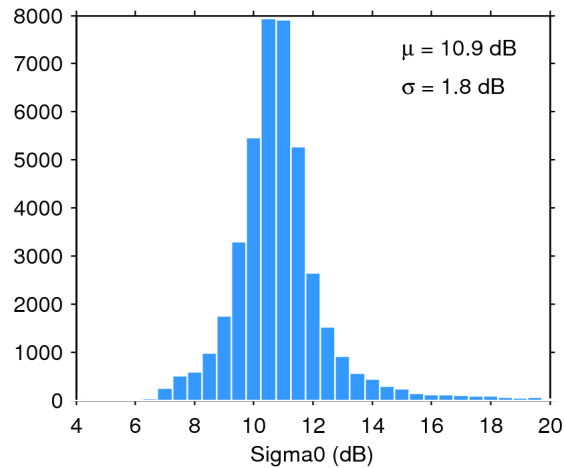
Figure 25. Histogram of flag-valid sigma0 over oceans and lakes for 21/08/2016. The mean ( \mu ) and standard deviation ( \sigma ) are also shown. Note that values outside [4 20] dB are excluded from the histogram for the sake of readability but not from the computation of \mu and \sigma .
