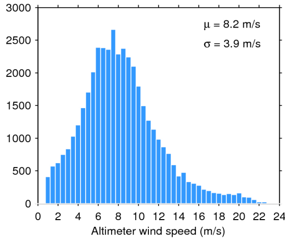
Figure 33. Histogram of flag-valid wind over oceans and lakes for 21/08/2016. The mean ( \mu ) and standard deviation ( \sigma ) are also shown. Note that values larger than 24 m/s are excluded from the histogram for the sake of readability but not from the computation of \mu and \sigma .
