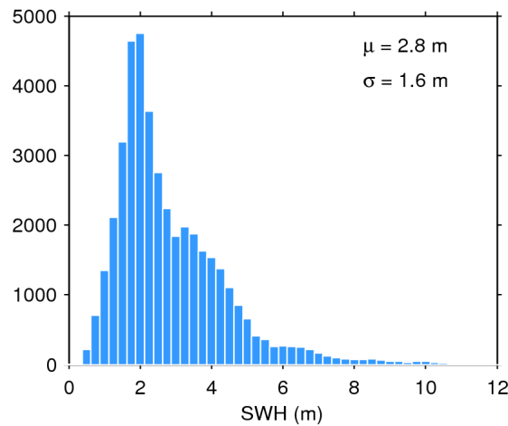
Figure 17. Histogram of flag-valid SWH over oceans and lakes for 21/08/2016. The mean ( \mu ) and standard deviation ( \sigma ) are also shown. Note that values larger than 12 m are excluded from the histogram for the sake of readability but not from the computation of \mu and \sigma .
