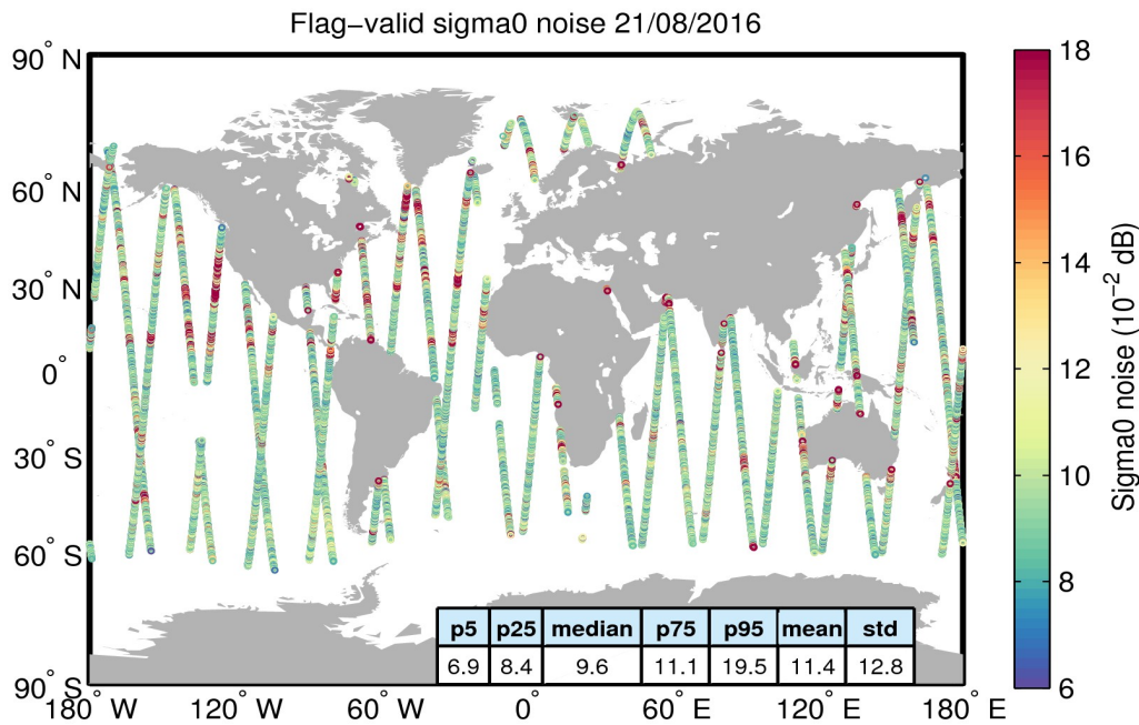
Figure 26. Geographical distribution of flag-valid 20-Hz sigma0 measurement noise over oceans and lakes for 21/08/2016. The statistical values shown in the table refer to the sigma0 noise and are calculated over all measurements shown in the figure.
