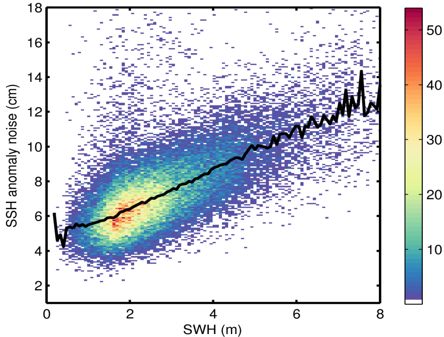
Figure 9. 2D histogram showing flag-valid SSH anomaly noise as a function of SWH for 19/08/2016. The black line denotes the median SSH anomaly noise as a function of SWH.
