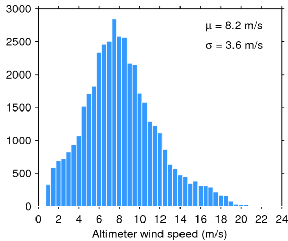
Figure 33. Histogram of flag-valid wind over oceans and lakes for 19/08/2016. The mean ( \mu ) and standard deviation ( \sigma ) are also shown. Note that values larger than 24 m/s are excluded from the histogram for the sake of readability but not from the computation of \mu and \sigma .
