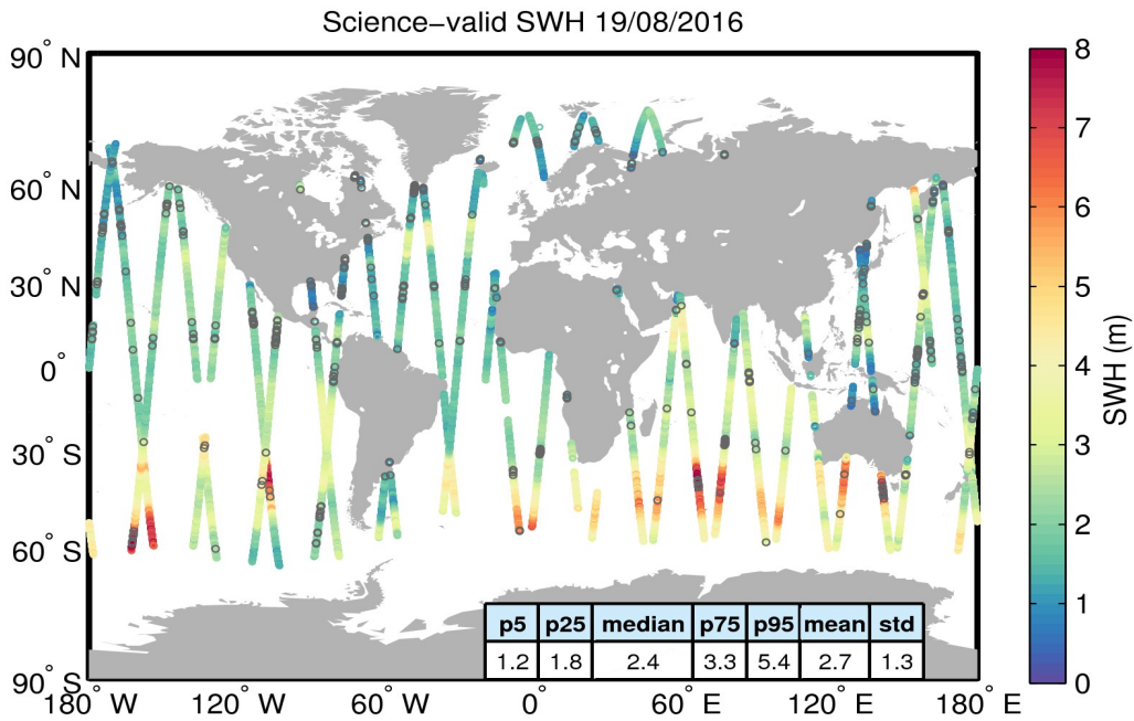
Figure 19. Geographical distribution of science-valid SWH data over oceans and lakes for 19/08/2016. The statistical values shown in the table refer to the SWH in m and are calculated over all measurements shown in the figure. Gray circles denote records that have been rejected based on the editing criteria described in Table 3.
