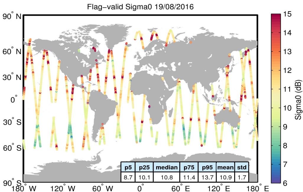
Figure 23. Geographical distribution of flag-valid sigma0 data over oceans and lakes for 19/08/2016. The statistical values shown in the table refer to the sigma0 in dB and are calculated over all measurements shown in the figure.
