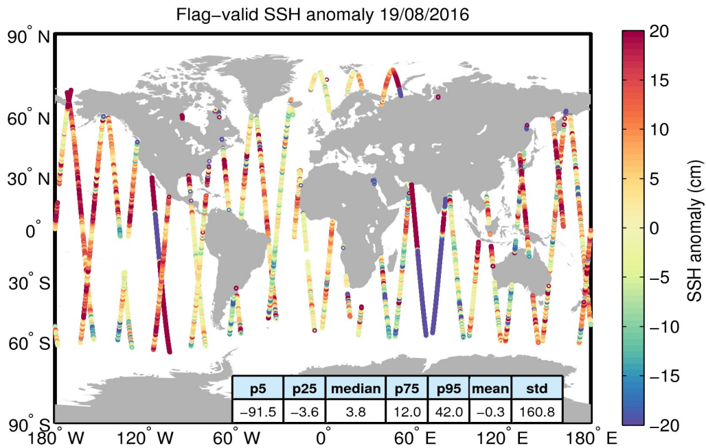
Figure 5. Geographical distribution of flag-valid 1-Hz SSH anomaly data over oceans and lakes for 19/08/2016. The statistical values shown in the table refer to the SSH anomaly in cm and are calculated over all measurements shown in the figure.
