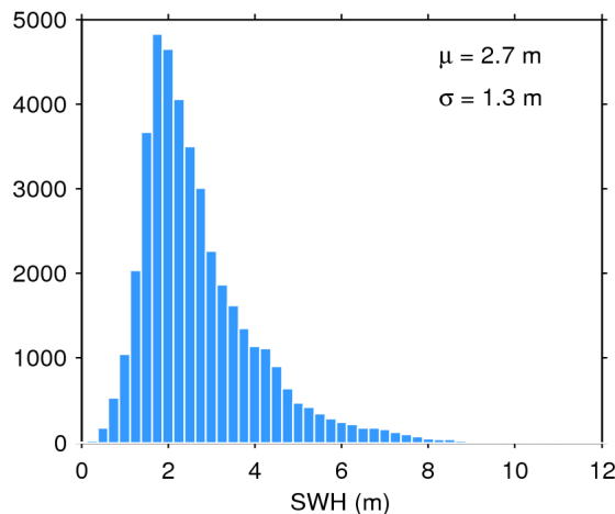
Figure 20. Histogram of science-valid SWH over oceans and lakes for 19/08/2016. The mean ( \mu ) and standard deviation ( \sigma ) are also shown. Note that values larger than 12 m are excluded from the histogram for the sake of readability but not from the computation of \mu and \sigma .
