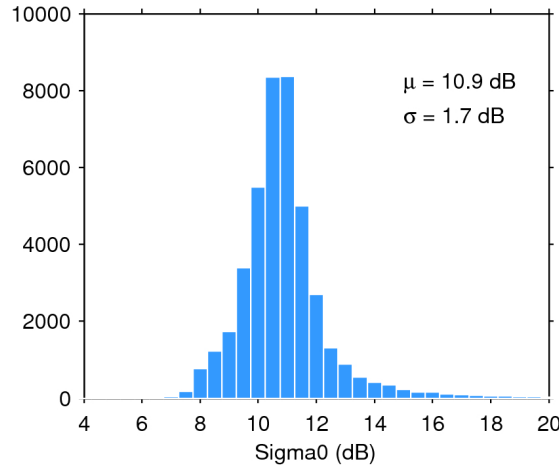
Figure 25. Histogram of flag-valid sigma0 over oceans and lakes for 19/08/2016. The mean ( \mu ) and standard deviation ( \sigma ) are also shown. Note that values outside [4 20] dB are excluded from the histogram for the sake of readability but not from the computation of \mu and \sigma .
