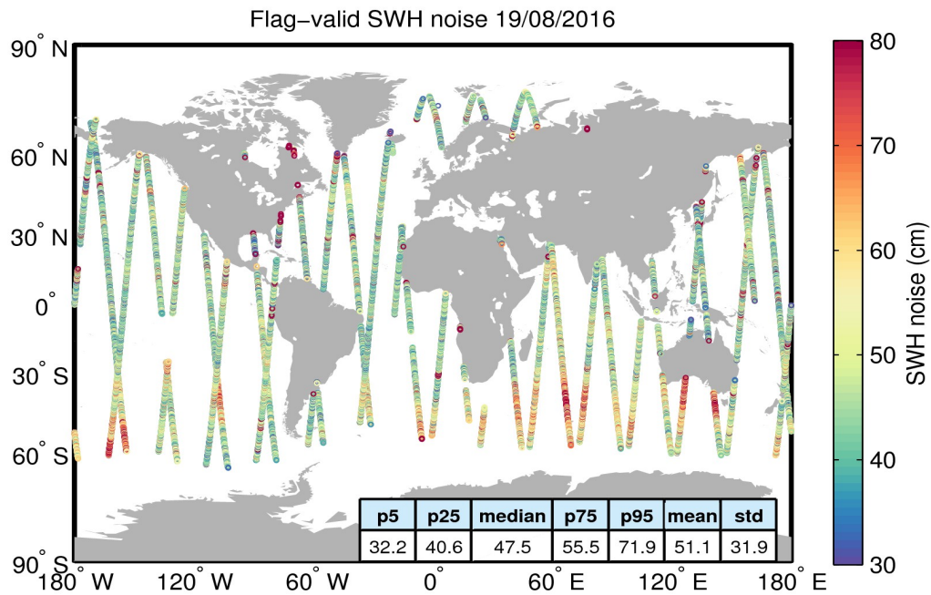
Figure 18. Geographical distribution of flag-valid 20-Hz SWH measurement noise over oceans and lakes for 19/08/2016. The statistical values shown in the table refer to the SWH noise and are calculated over all measurements shown in the figure.
