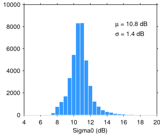
Figure 28. Histogram of science-valid sigma0 over oceans and lakes for 19/08/2016. The mean ( \mu ) and standard deviation ( \sigma ) are also shown. Note that values outside [4 20] dB are excluded from the histogram for the sake of readability but not from the computation of \mu and \sigma .
