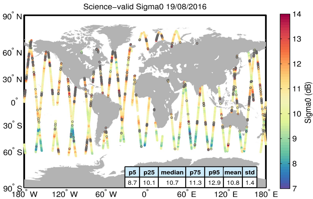
Figure 27. Geographical distribution of science-valid sigma0 data over oceans and lakes for 19/08/2016. The statistical values shown in the table refer to the sigma0 in dB and are calculated over all measurements shown in the figure. Gray circles denote records that have been rejected based on the editing criteria described in Table 4.
