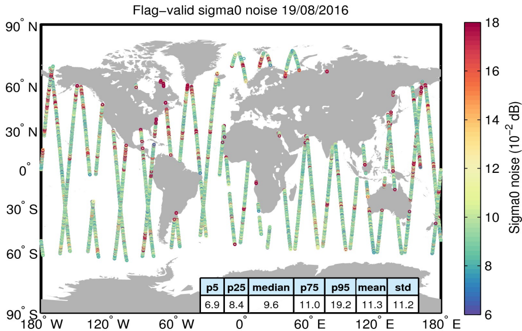
Figure 26. Geographical distribution of flag-valid 20-Hz sigma0 measurement noise over oceans and lakes for 19/08/2016. The statistical values shown in the table refer to the sigma0 noise and are calculated over all measurements shown in the figure.
