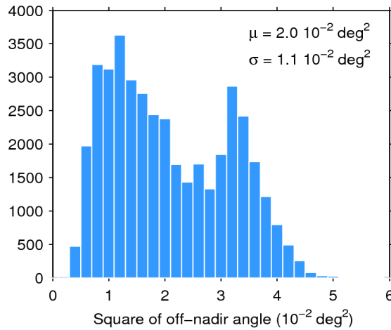
Figure 39. Histogram of flag-valid mispointing over oceans and lakes for 19/08/2016. The mean ( \mu ) and standard deviation ( \sigma ) are also shown. Note that values larger than 6 \cdot 10^{-2} \text{ deg}^2 are excluded from the histogram for the sake of readability but not from the computation of \mu and \sigma .
