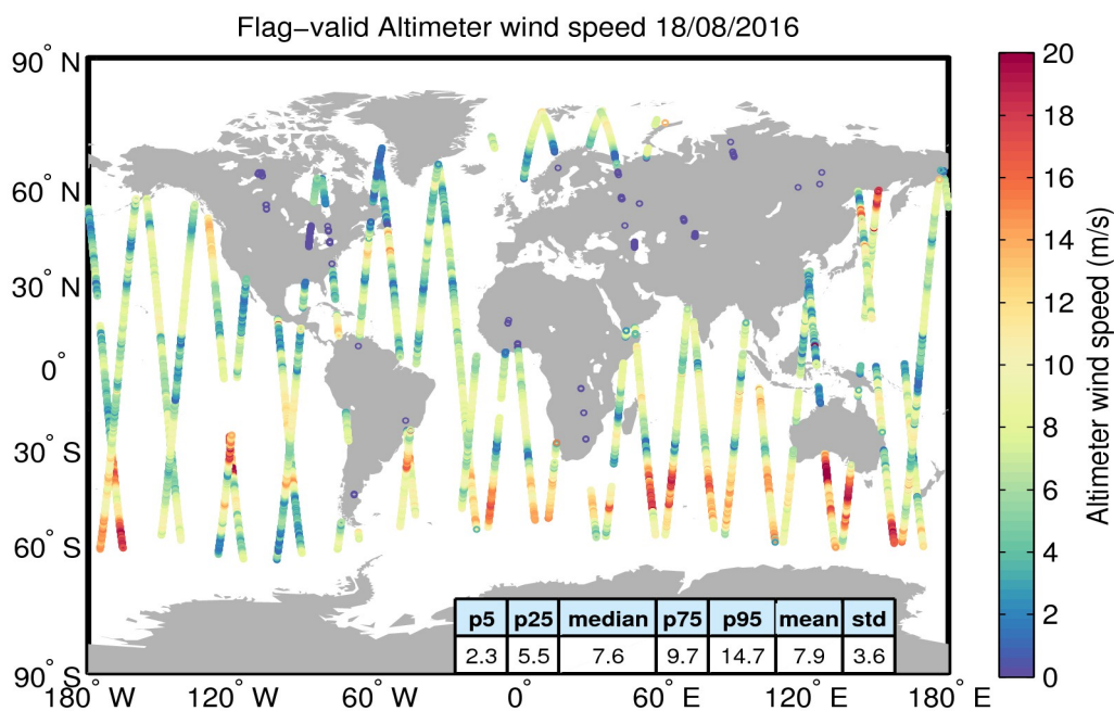
Figure 31. Geographical distribution of flag-valid wind data over oceans and lakes for 18/08/2016. The statistical values shown in the table refer to the wind in m/s and are calculated over all measurements shown in the figure.
