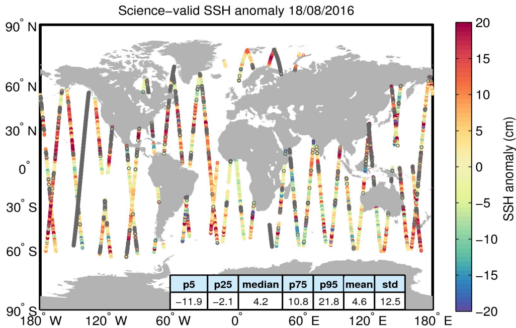
Figure 10. Geographical distribution of science-valid SSH anomaly data over oceans and lakes for 18/08/2016. The statistical values shown in the table refer to the SSH anomaly in cm and are calculated over all measurements shown in the figure. Gray circles denote records that have been rejected based on the editing criteria described in Table 2.
