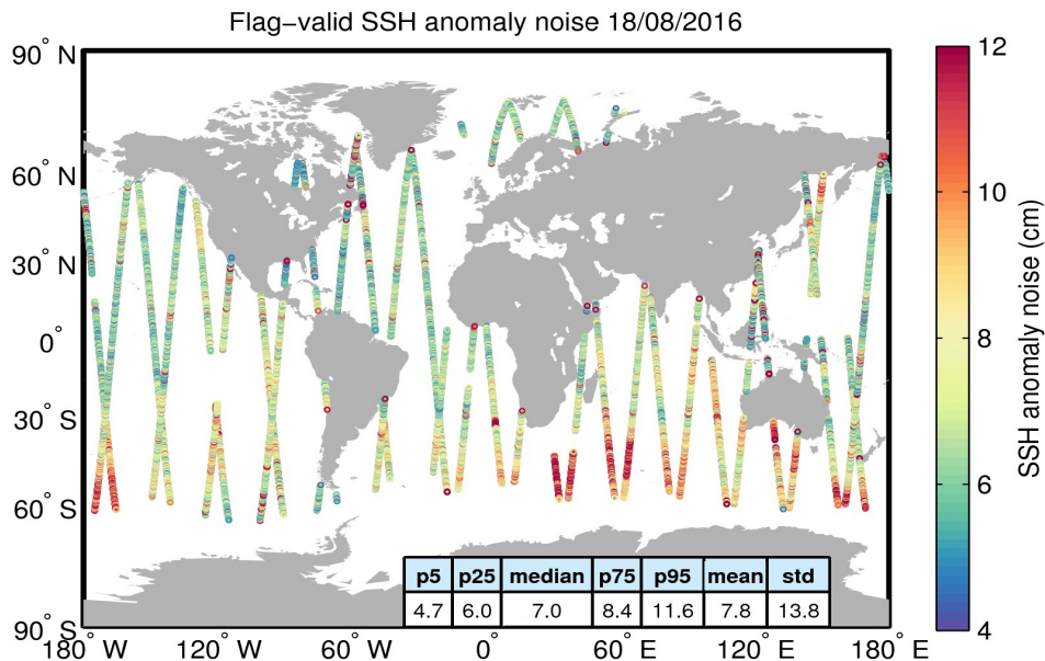
Figure 8. Geographical distribution of flag-valid 20-Hz SSH anomaly measurement noise over oceans and lakes for 18/08/2016. The statistical values shown in the table refer to the SSH anomaly noise and are calculated over all measurements shown in the figure.
