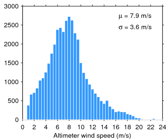
Figure 35. Histogram of science-valid wind over oceans and lakes for 18/08/2016. The mean ( \mu ) and standard deviation ( \sigma ) are also shown. Note that values larger than 24 m/s are excluded from the histogram for the sake of readability but not from the computation of \mu and \sigma .
