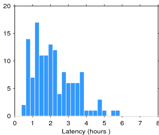
Figure 2. Histogram of the data latency for 18/08/2016. The y-axis denotes the number of files that are made available with a delay of x-hours with respect to the mean time of the records stored in the file.
