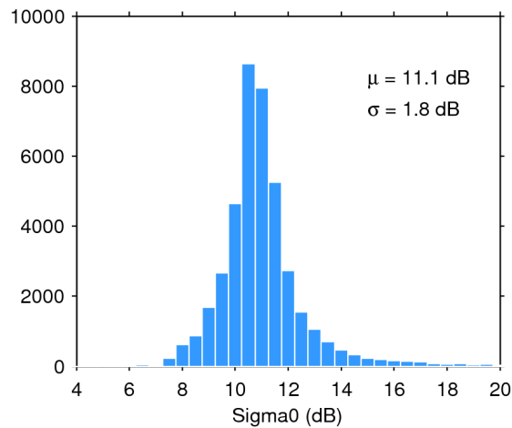
Figure 25. Histogram of flag-valid sigma0 over oceans and lakes for 18/08/2016. The mean ( \mu ) and standard deviation ( \sigma ) are also shown. Note that values outside [4 20] dB are excluded from the histogram for the sake of readability but not from the computation of \mu and \sigma .
