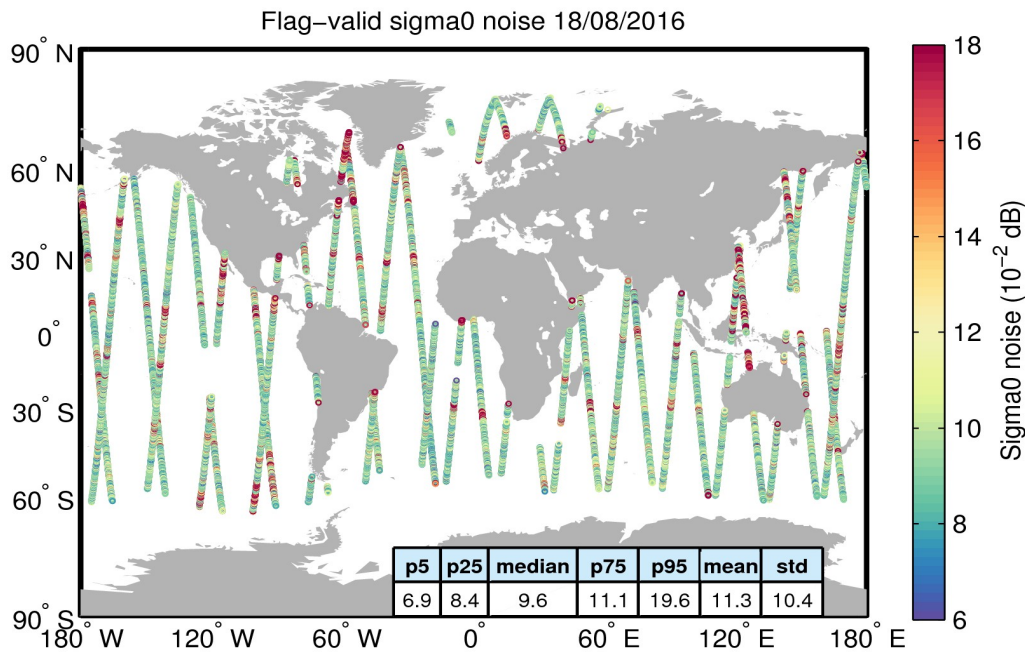
Figure 26. Geographical distribution of flag-valid 20-Hz sigma0 measurement noise over oceans and lakes for 18/08/2016. The statistical values shown in the table refer to the sigma0 noise and are calculated over all measurements shown in the figure.
