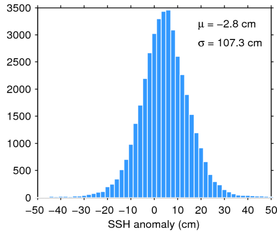
Figure 7. Histogram of flag-valid SSH anomaly over oceans and lakes for 18/08/2016. The mean ( \mu ) and standard deviation ( \sigma ) are also shown. Note that values outside [-50 50] cm are excluded from the histogram for the sake of readability but not from the computation of \mu and \sigma .
