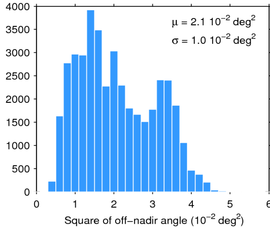
Figure 39. Histogram of flag-valid mispointing over oceans and lakes for 18/08/2016. The mean ( \mu ) and standard deviation ( \sigma ) are also shown. Note that values larger than 6 \cdot 10^{-2} \text{ deg}^2 are excluded from the histogram for the sake of readability but not from the computation of \mu and \sigma .
