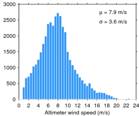
Figure 33. Histogram of flag-valid wind over oceans and lakes for 18/08/2016. The mean ( \mu ) and standard deviation ( \sigma ) are also shown. Note that values larger than 24 m/s are excluded from the histogram for the sake of readability but not from the computation of \mu and \sigma .
