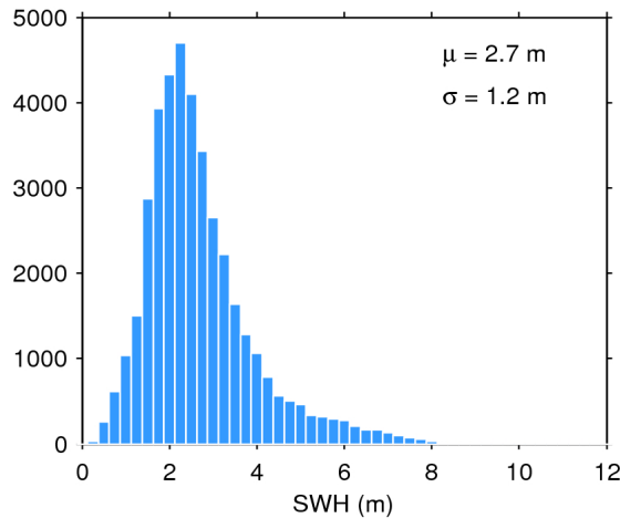
Figure 20. Histogram of science-valid SWH over oceans and lakes for 18/08/2016. The mean ( \mu ) and standard deviation ( \sigma ) are also shown. Note that values larger than 12 m are excluded from the histogram for the sake of readability but not from the computation of \mu and \sigma .
