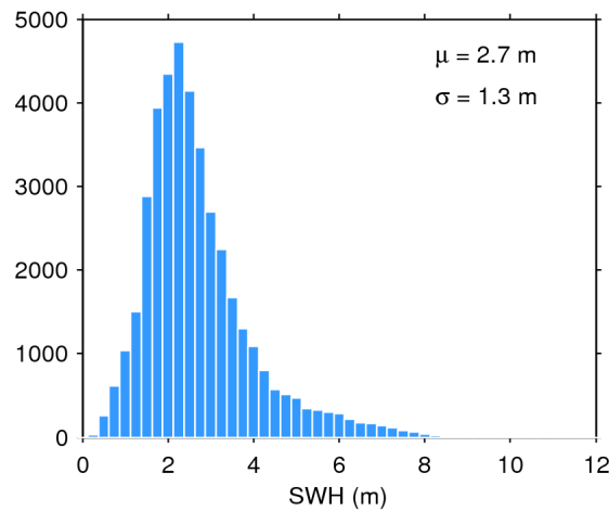
Figure 17. Histogram of flag-valid SWH over oceans and lakes for 18/08/2016. The mean ( \mu ) and standard deviation ( \sigma ) are also shown. Note that values larger than 12 m are excluded from the histogram for the sake of readability but not from the computation of \mu and \sigma .
