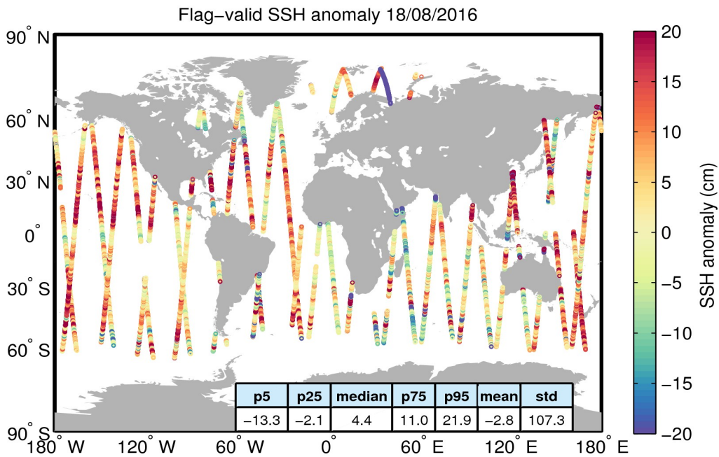
Figure 5. Geographical distribution of flag-valid 1-Hz SSH anomaly data over oceans and lakes for 18/08/2016. The statistical values shown in the table refer to the SSH anomaly in cm and are calculated over all measurements shown in the figure.
