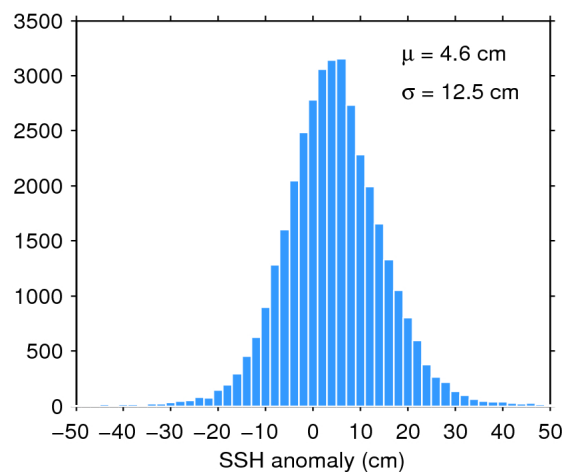
Figure 11. Histogram of science-valid SSH anomaly over oceans and lakes for 18/08/2016. The mean ( \mu ) and standard deviation ( \sigma ) are also shown. Note that values outside [-50 50] cm are excluded from the histogram for the sake of readability but not from the computation of \mu and \sigma .
