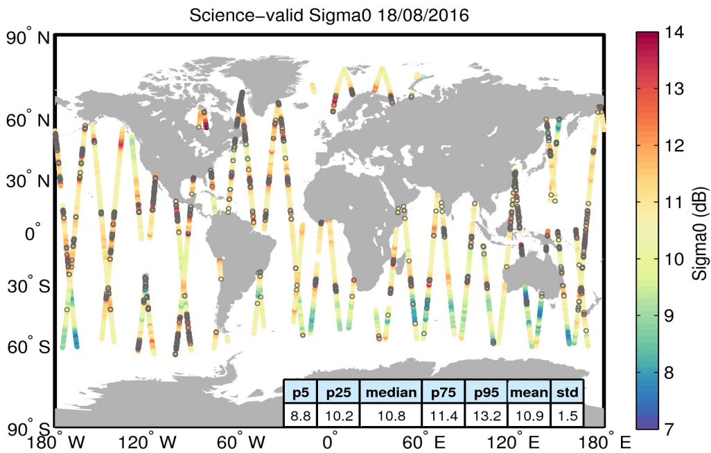
Figure 27. Geographical distribution of science-valid sigma0 data over oceans and lakes for 18/08/2016. The statistical values shown in the table refer to the sigma0 in dB and are calculated over all measurements shown in the figure. Gray circles denote records that have been rejected based on the editing criteria described in Table 4.
