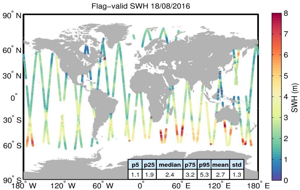
Figure 15. Geographical distribution of flag-valid SWH data over oceans and lakes for 18/08/2016. The statistical values shown in the table refer to the SWH in m and are calculated over all measurements shown in the figure.
