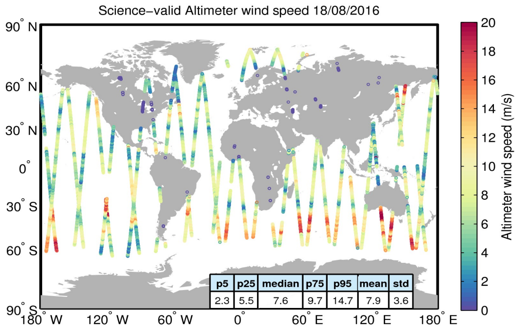
Figure 34. Geographical distribution of science-valid wind data over oceans and lakes for 18/08/2016. The statistical values shown in the table refer to the wind in m/s and are calculated over all measurements shown in the figure. Gray circles denote records that have been rejected based on the editing criteria described in Table 5.
