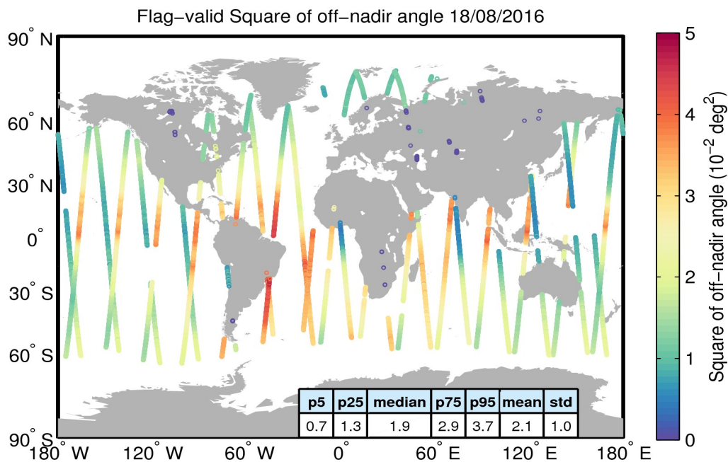
Figure 37. Geographical distribution of flag-valid mispointing data over oceans and lakes for 18/08/2016. The statistical values shown in the table refer to the mispointing in 10^{-2} deg 2 and are calculated over all measurements shown in the figure.
