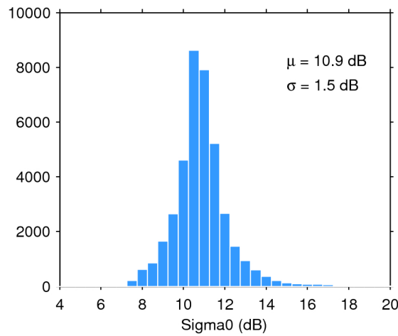
Figure 28. Histogram of science-valid sigma0 over oceans and lakes for 18/08/2016. The mean ( \mu ) and standard deviation ( \sigma ) are also shown. Note that values outside [4 20] dB are excluded from the histogram for the sake of readability but not from the computation of \mu and \sigma .
