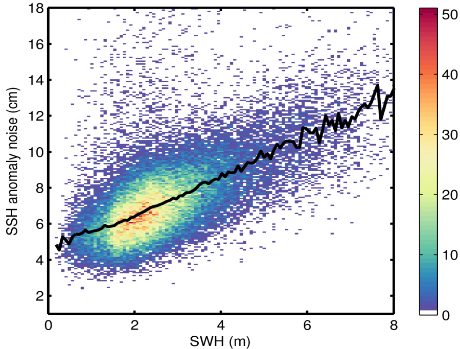
Figure 9. 2D histogram showing flag-valid SSH anomaly noise as a function of SWH for 18/08/2016. The black line denotes the median SSH anomaly noise as a function of SWH.
