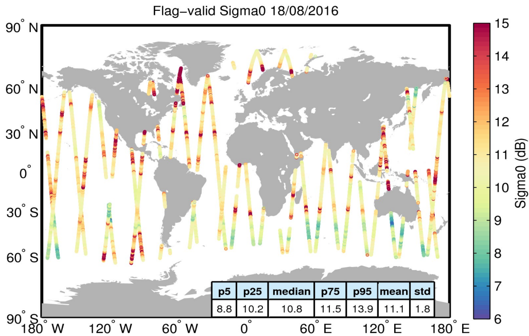
Figure 23. Geographical distribution of flag-valid sigma0 data over oceans and lakes for 18/08/2016. The statistical values shown in the table refer to the sigma0 in dB and are calculated over all measurements shown in the figure.
