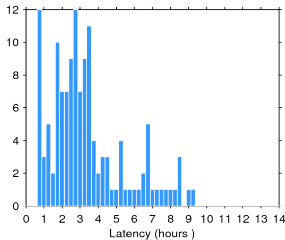
Figure 2. Histogram of the data latency for 17/08/2016. The y-axis denotes the number of files that are made available with a delay of x-hours with respect to the mean time of the records stored in the file.
