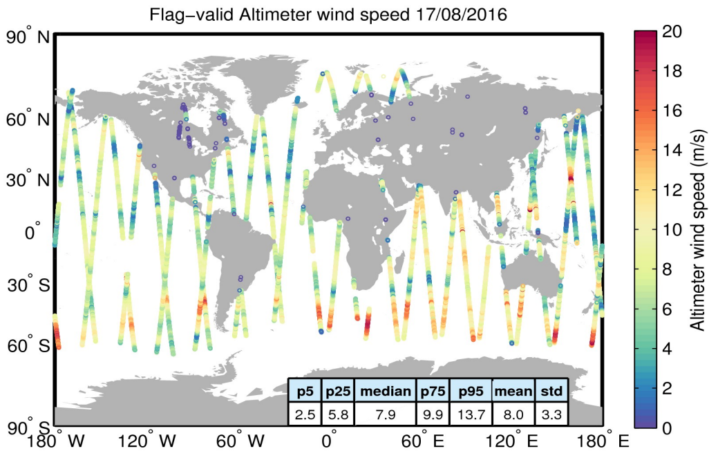
Figure 31. Geographical distribution of flag-valid wind data over oceans and lakes for 17/08/2016. The statistical values shown in the table refer to the wind in m/s and are calculated over all measurements shown in the figure.
