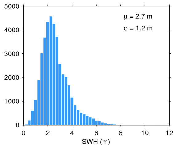
Figure 20. Histogram of science-valid SWH over oceans and lakes for 17/08/2016. The mean ( \mu ) and standard deviation ( \sigma ) are also shown. Note that values larger than 12 m are excluded from the histogram for the sake of readability but not from the computation of \mu and \sigma .
