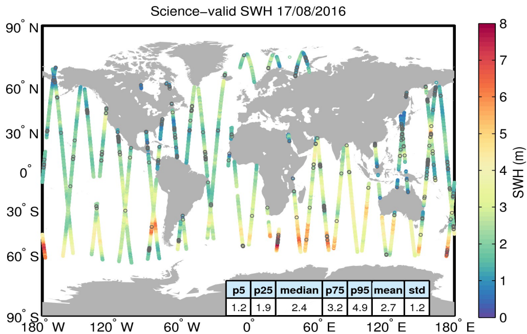
Figure 19. Geographical distribution of science-valid SWH data over oceans and lakes for 17/08/2016. The statistical values shown in the table refer to the SWH in m and are calculated over all measurements shown in the figure. Gray circles denote records that have been rejected based on the editing criteria described in Table 3.
