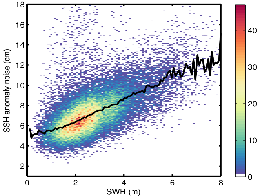
Figure 9. 2D histogram showing flag-valid SSH anomaly noise as a function of SWH for 17/08/2016. The black line denotes the median SSH anomaly noise as a function of SWH.
