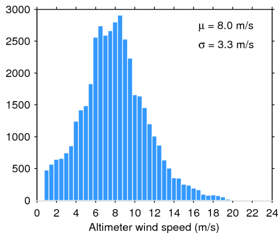
Figure 35. Histogram of science-valid wind over oceans and lakes for 17/08/2016. The mean ( \mu ) and standard deviation ( \sigma ) are also shown. Note that values larger than 24 m/s are excluded from the histogram for the sake of readability but not from the computation of \mu and \sigma .
