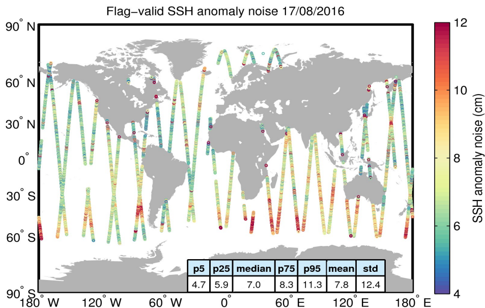
Figure 8. Geographical distribution of flag-valid 20-Hz SSH anomaly measurement noise over oceans and lakes for 17/08/2016. The statistical values shown in the table refer to the SSH anomaly noise and are calculated over all measurements shown in the figure.
