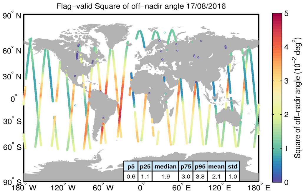
Figure 37. Geographical distribution of flag-valid mispointing data over oceans and lakes for 17/08/2016. The statistical values shown in the table refer to the mispointing in 10^{-2} deg 2 and are calculated over all measurements shown in the figure.
