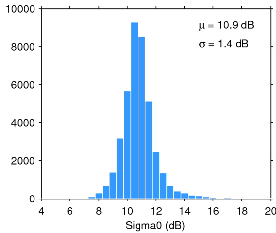
Figure 28. Histogram of science-valid sigma0 over oceans and lakes for 17/08/2016. The mean ( \mu ) and standard deviation ( \sigma ) are also shown. Note that values outside [4 20] dB are excluded from the histogram for the sake of readability but not from the computation of \mu and \sigma .
