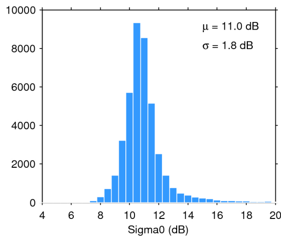
Figure 25. Histogram of flag-valid sigma0 over oceans and lakes for 17/08/2016. The mean ( \mu ) and standard deviation ( \sigma ) are also shown. Note that values outside [4 20] dB are excluded from the histogram for the sake of readability but not from the computation of \mu and \sigma .
