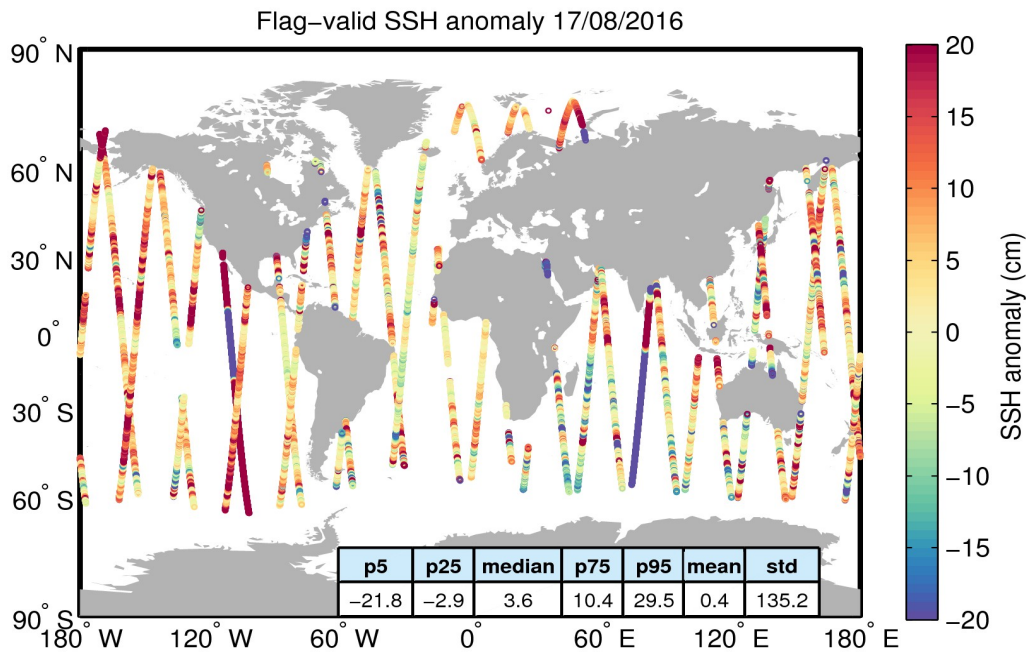
Figure 5. Geographical distribution of flag-valid 1-Hz SSH anomaly data over oceans and lakes for 17/08/2016. The statistical values shown in the table refer to the SSH anomaly in cm and are calculated over all measurements shown in the figure.
