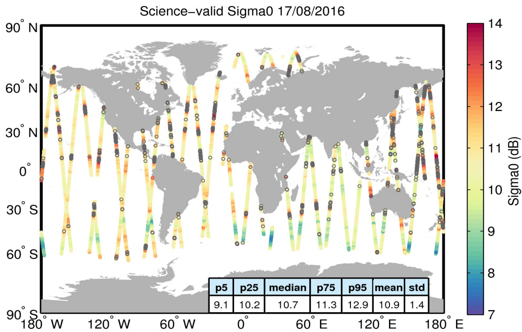
Figure 27. Geographical distribution of science-valid sigma0 data over oceans and lakes for 17/08/2016. The statistical values shown in the table refer to the sigma0 in dB and are calculated over all measurements shown in the figure. Gray circles denote records that have been rejected based on the editing criteria described in Table 4.
