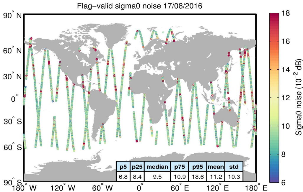
Figure 26. Geographical distribution of flag-valid 20-Hz sigma0 measurement noise over oceans and lakes for 17/08/2016. The statistical values shown in the table refer to the sigma0 noise and are calculated over all measurements shown in the figure.
