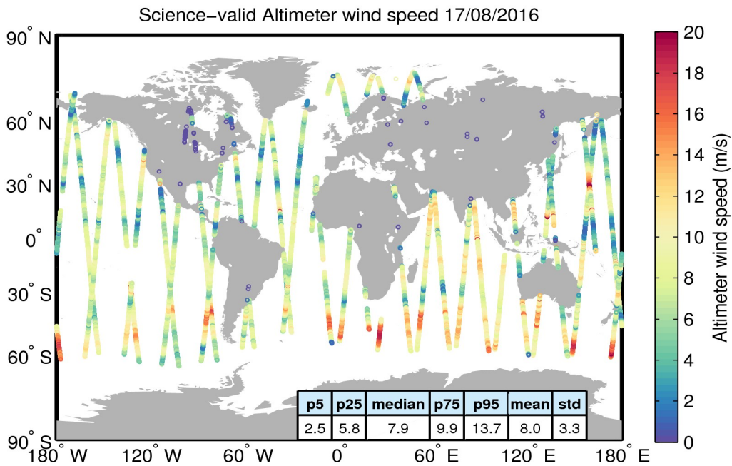
Figure 34. Geographical distribution of science-valid wind data over oceans and lakes for 17/08/2016. The statistical values shown in the table refer to the wind in m/s and are calculated over all measurements shown in the figure. Gray circles denote records that have been rejected based on the editing criteria described in Table 5.
