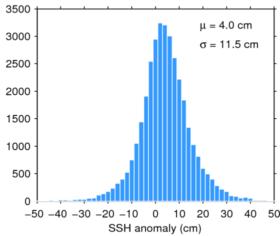
Figure 11. Histogram of science-valid SSH anomaly over oceans and lakes for 17/08/2016. The mean ( \mu ) and standard deviation ( \sigma ) are also shown. Note that values outside [-50 50] cm are excluded from the histogram for the sake of readability but not from the computation of \mu and \sigma .
