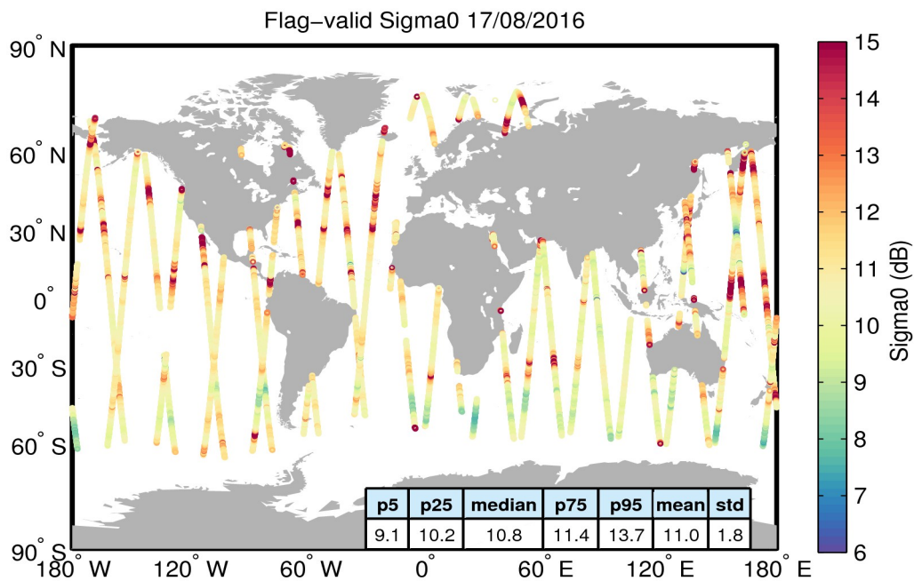
Figure 23. Geographical distribution of flag-valid sigma0 data over oceans and lakes for 17/08/2016. The statistical values shown in the table refer to the sigma0 in dB and are calculated over all measurements shown in the figure.
