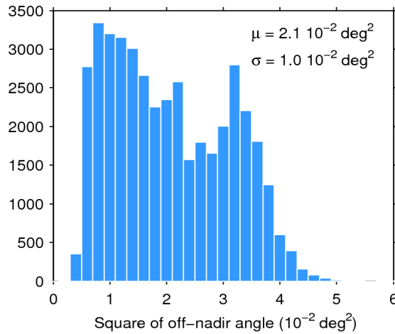
Figure 39. Histogram of flag-valid mispointing over oceans and lakes for 17/08/2016. The mean ( \mu ) and standard deviation ( \sigma ) are also shown. Note that values larger than 6 \cdot 10^{-2} \text{ deg}^2 are excluded from the histogram for the sake of readability but not from the computation of \mu and \sigma .
