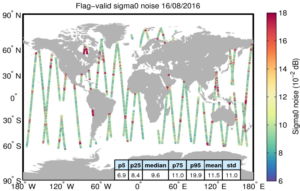
Figure 26. Geographical distribution of flag-valid 20-Hz sigma0 measurement noise over oceans and lakes for 16/08/2016. The statistical values shown in the table refer to the sigma0 noise and are calculated over all measurements shown in the figure.
