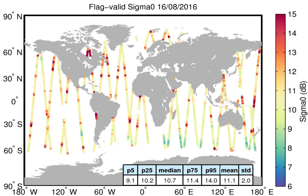
Figure 23. Geographical distribution of flag-valid sigma0 data over oceans and lakes for 16/08/2016. The statistical values shown in the table refer to the sigma0 in dB and are calculated over all measurements shown in the figure.
