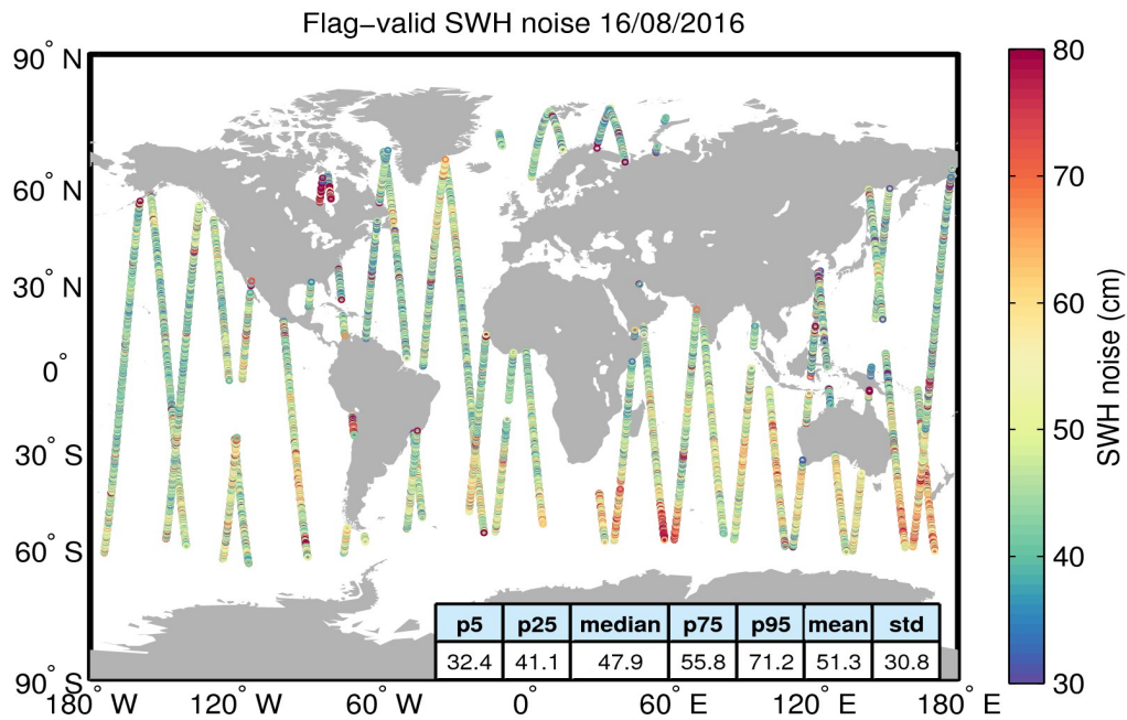
Figure 18. Geographical distribution of flag-valid 20-Hz SWH measurement noise over oceans and lakes for 16/08/2016. The statistical values shown in the table refer to the SWH noise and are calculated over all measurements shown in the figure.
