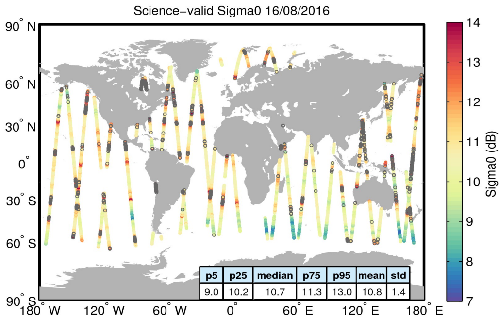
Figure 27. Geographical distribution of science-valid sigma0 data over oceans and lakes for 16/08/2016. The statistical values shown in the table refer to the sigma0 in dB and are calculated over all measurements shown in the figure. Gray circles denote records that have been rejected based on the editing criteria described in Table 4.
