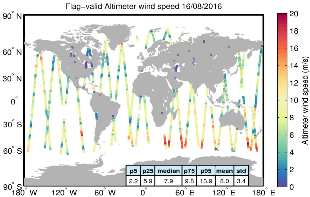
Figure 31. Geographical distribution of flag-valid wind data over oceans and lakes for 16/08/2016. The statistical values shown in the table refer to the wind in m/s and are calculated over all measurements shown in the figure.
