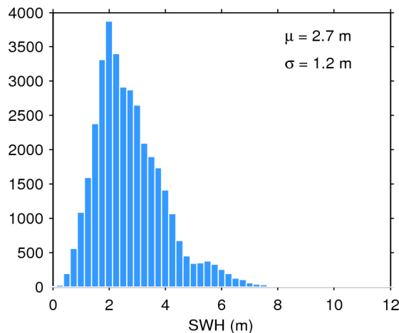
Figure 20. Histogram of science-valid SWH over oceans and lakes for 16/08/2016. The mean ( \mu ) and standard deviation ( \sigma ) are also shown. Note that values larger than 12 m are excluded from the histogram for the sake of readability but not from the computation of \mu and \sigma .
