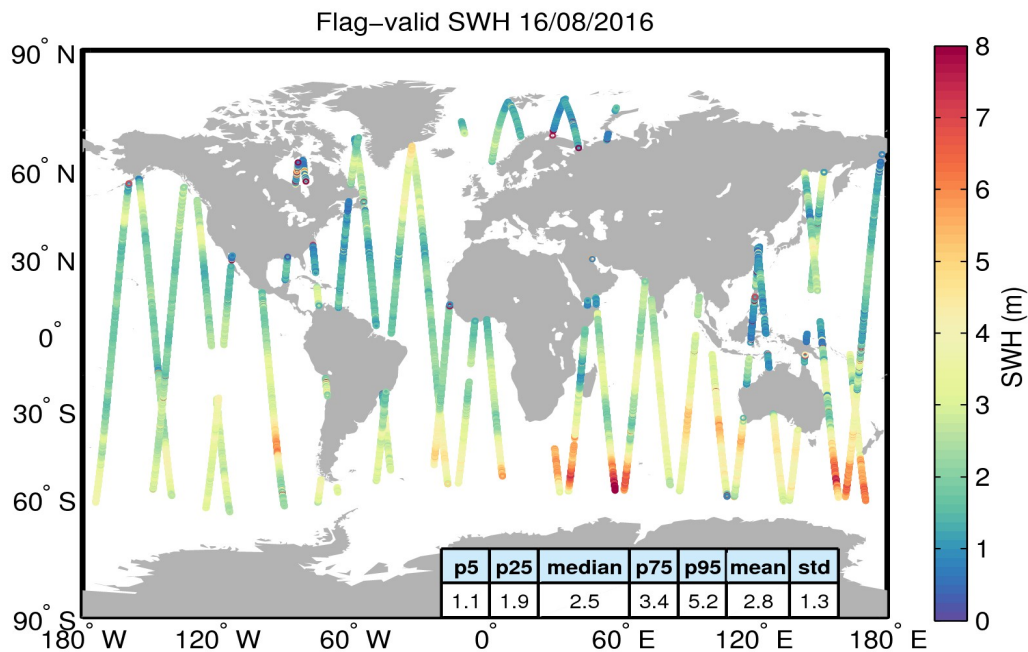
Figure 15. Geographical distribution of flag-valid SWH data over oceans and lakes for 16/08/2016. The statistical values shown in the table refer to the SWH in m and are calculated over all measurements shown in the figure.
