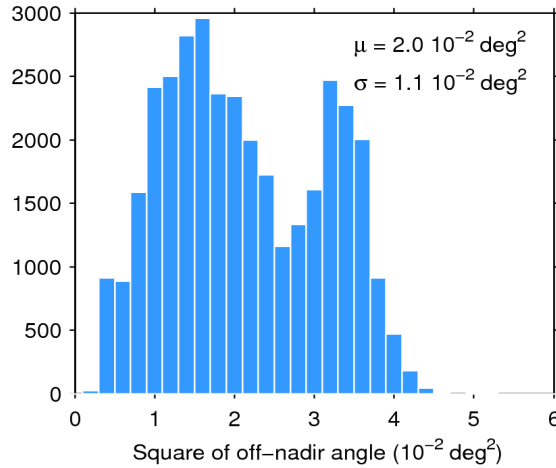
Figure 39. Histogram of flag-valid mispointing over oceans and lakes for 16/08/2016. The mean ( \mu ) and standard deviation ( \sigma ) are also shown. Note that values larger than 6 \cdot 10^{-2} \text{ deg}^2 are excluded from the histogram for the sake of readability but not from the computation of \mu and \sigma .
