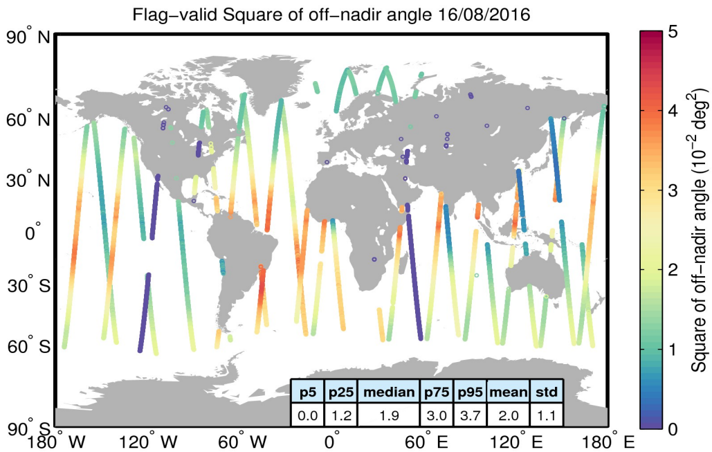
Figure 37. Geographical distribution of flag-valid mispointing data over oceans and lakes for 16/08/2016. The statistical values shown in the table refer to the mispointing in 10^{-2} deg 2 and are calculated over all measurements shown in the figure.
