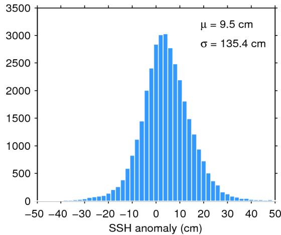
Figure 7. Histogram of flag-valid SSH anomaly over oceans and lakes for 16/08/2016. The mean ( \mu ) and standard deviation ( \sigma ) are also shown. Note that values outside [-50 50] cm are excluded from the histogram for the sake of readability but not from the computation of \mu and \sigma .
