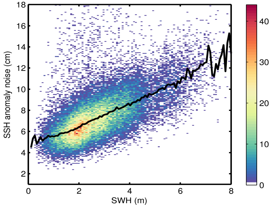
Figure 9. 2D histogram showing flag-valid SSH anomaly noise as a function of SWH for 16/08/2016. The black line denotes the median SSH anomaly noise as a function of SWH.
