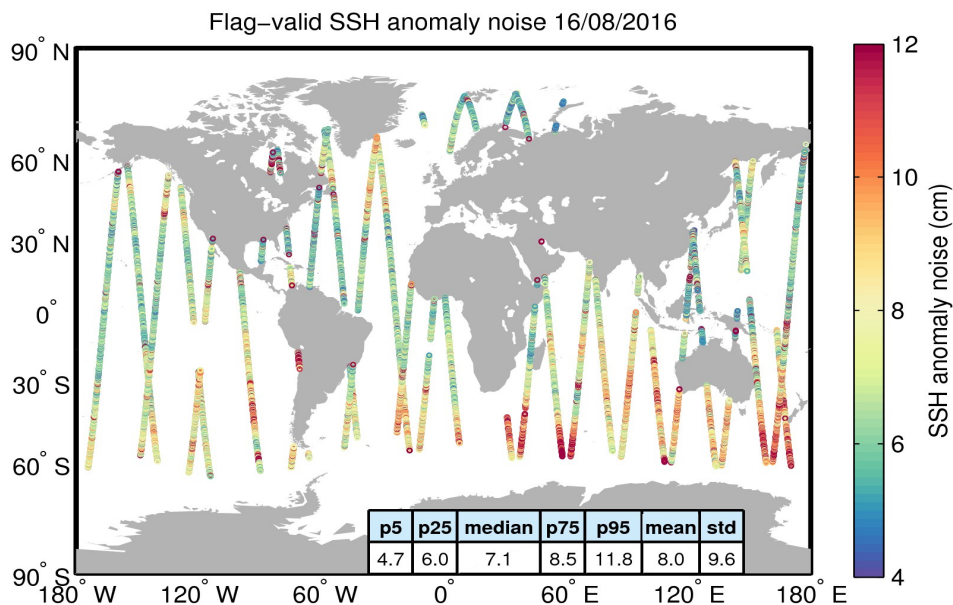
Figure 8. Geographical distribution of flag-valid 20-Hz SSH anomaly measurement noise over oceans and lakes for 16/08/2016. The statistical values shown in the table refer to the SSH anomaly noise and are calculated over all measurements shown in the figure.
