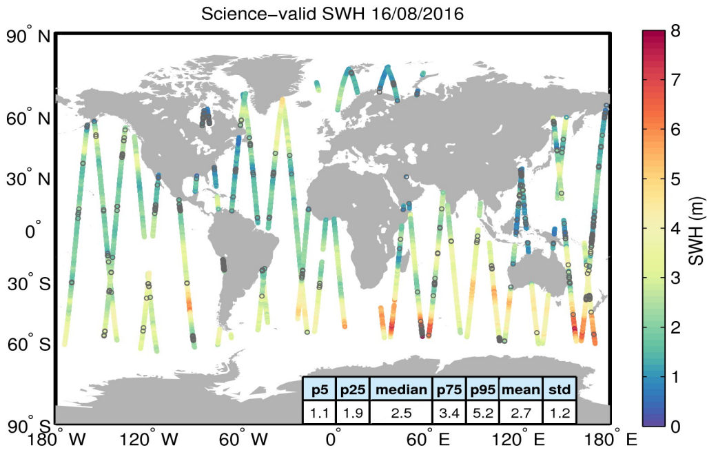
Figure 19. Geographical distribution of science-valid SWH data over oceans and lakes for 16/08/2016. The statistical values shown in the table refer to the SWH in m and are calculated over all measurements shown in the figure. Gray circles denote records that have been rejected based on the editing criteria described in Table 3.
