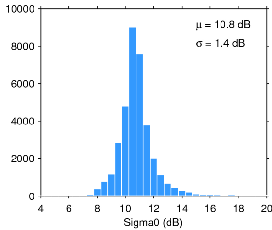
Figure 28. Histogram of science-valid sigma0 over oceans and lakes for 16/08/2016. The mean ( \mu ) and standard deviation ( \sigma ) are also shown. Note that values outside [4 20] dB are excluded from the histogram for the sake of readability but not from the computation of \mu and \sigma .
