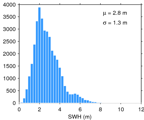
Figure 17. Histogram of flag-valid SWH over oceans and lakes for 16/08/2016. The mean ( \mu ) and standard deviation ( \sigma ) are also shown. Note that values larger than 12 m are excluded from the histogram for the sake of readability but not from the computation of \mu and \sigma .
