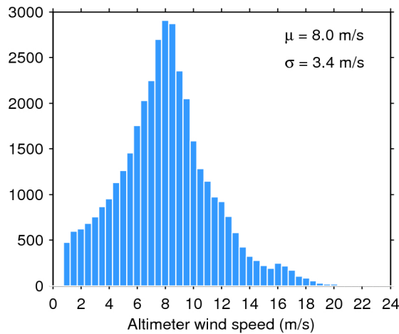
Figure 33. Histogram of flag-valid wind over oceans and lakes for 16/08/2016. The mean ( \mu ) and standard deviation ( \sigma ) are also shown. Note that values larger than 24 m/s are excluded from the histogram for the sake of readability but not from the computation of \mu and \sigma .
