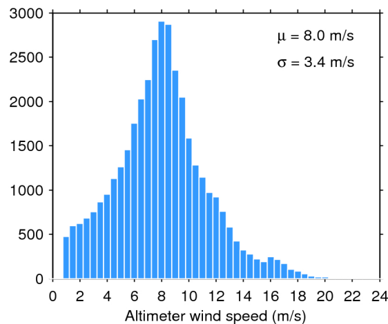
Figure 35. Histogram of science-valid wind over oceans and lakes for 16/08/2016. The mean ( \mu ) and standard deviation ( \sigma ) are also shown. Note that values larger than 24 m/s are excluded from the histogram for the sake of readability but not from the computation of \mu and \sigma .
