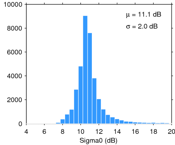
Figure 25. Histogram of flag-valid sigma0 over oceans and lakes for 16/08/2016. The mean ( \mu ) and standard deviation ( \sigma ) are also shown. Note that values outside [4 20] dB are excluded from the histogram for the sake of readability but not from the computation of \mu and \sigma .
