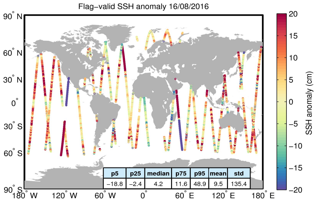
Figure 5. Geographical distribution of flag-valid 1-Hz SSH anomaly data over oceans and lakes for 16/08/2016. The statistical values shown in the table refer to the SSH anomaly in cm and are calculated over all measurements shown in the figure.
