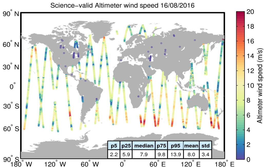
Figure 34. Geographical distribution of science-valid wind data over oceans and lakes for 16/08/2016. The statistical values shown in the table refer to the wind in m/s and are calculated over all measurements shown in the figure. Gray circles denote records that have been rejected based on the editing criteria described in Table 5.
