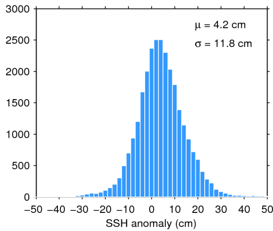
Figure 11. Histogram of science-valid SSH anomaly over oceans and lakes for 16/08/2016. The mean ( \mu ) and standard deviation ( \sigma ) are also shown. Note that values outside [-50 50] cm are excluded from the histogram for the sake of readability but not from the computation of \mu and \sigma .
