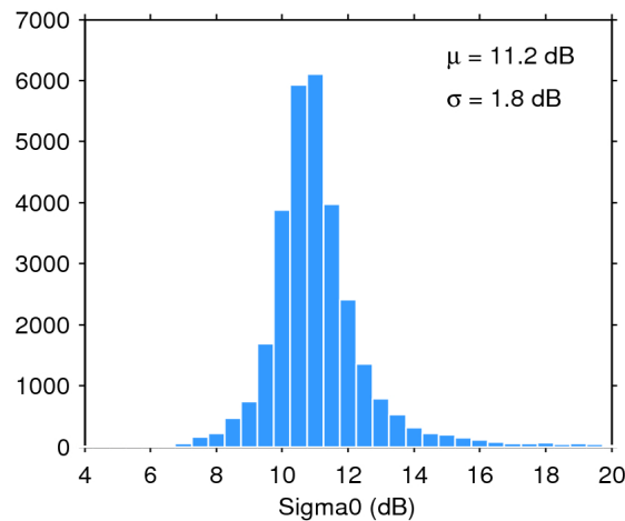
Figure 25. Histogram of flag-valid sigma0 over oceans and lakes for 15/08/2016. The mean ( \mu ) and standard deviation ( \sigma ) are also shown. Note that values outside [4 20] dB are excluded from the histogram for the sake of readability but not from the computation of \mu and \sigma .
