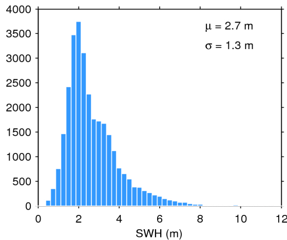
Figure 17. Histogram of flag-valid SWH over oceans and lakes for 15/08/2016. The mean ( \mu ) and standard deviation ( \sigma ) are also shown. Note that values larger than 12 m are excluded from the histogram for the sake of readability but not from the computation of \mu and \sigma .
