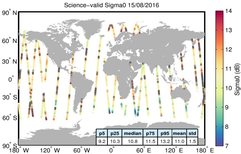
Figure 27. Geographical distribution of science-valid sigma0 data over oceans and lakes for 15/08/2016. The statistical values shown in the table refer to the sigma0 in dB and are calculated over all measurements shown in the figure. Gray circles denote records that have been rejected based on the editing criteria described in Table 4.
