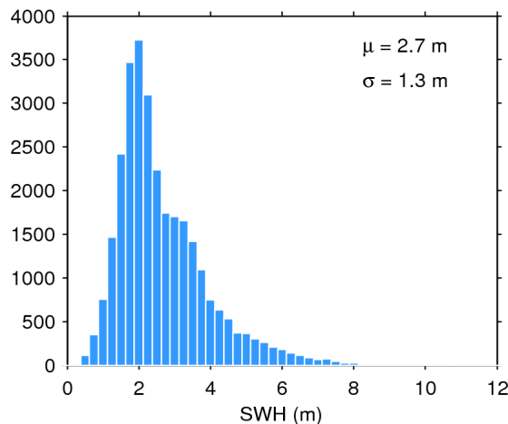
Figure 20. Histogram of science-valid SWH over oceans and lakes for 15/08/2016. The mean ( \mu ) and standard deviation ( \sigma ) are also shown. Note that values larger than 12 m are excluded from the histogram for the sake of readability but not from the computation of \mu and \sigma .
