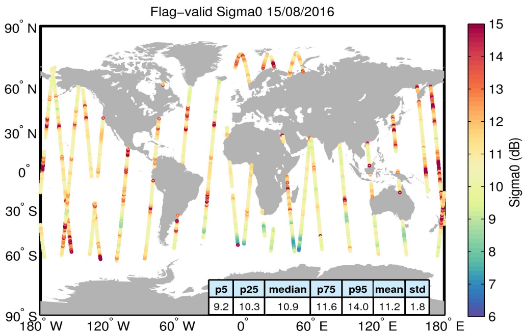
Figure 23. Geographical distribution of flag-valid sigma0 data over oceans and lakes for 15/08/2016. The statistical values shown in the table refer to the sigma0 in dB and are calculated over all measurements shown in the figure.
