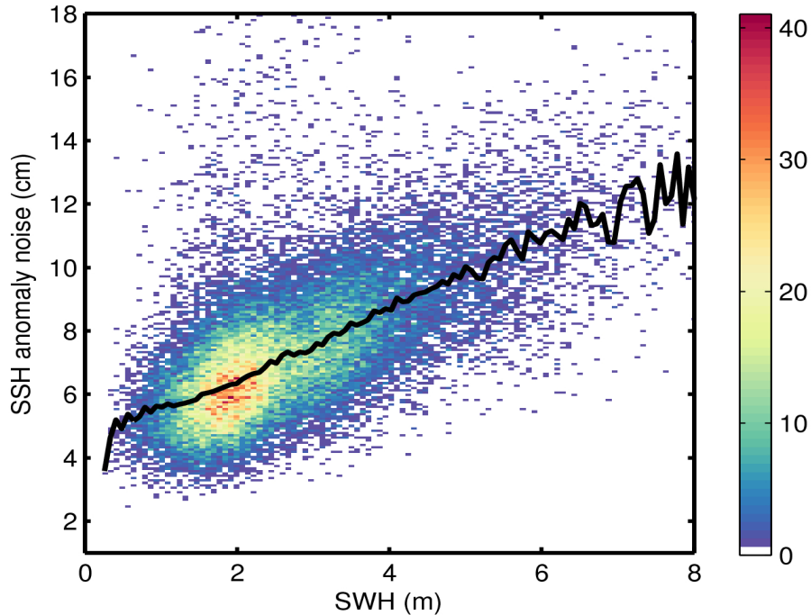
Figure 9. 2D histogram showing flag-valid SSH anomaly noise as a function of SWH for 15/08/2016. The black line denotes the median SSH anomaly noise as a function of SWH.
