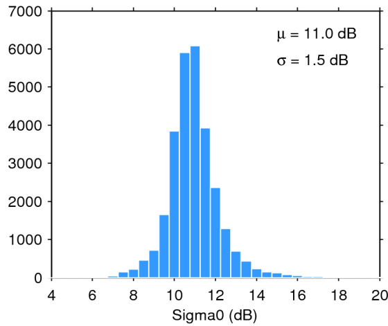
Figure 28. Histogram of science-valid sigma0 over oceans and lakes for 15/08/2016. The mean ( \mu ) and standard deviation ( \sigma ) are also shown. Note that values outside [4 20] dB are excluded from the histogram for the sake of readability but not from the computation of \mu and \sigma .
