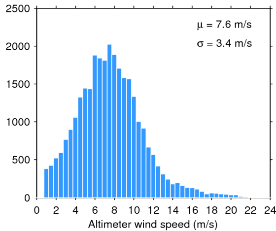
Figure 33. Histogram of flag-valid wind over oceans and lakes for 15/08/2016. The mean ( \mu ) and standard deviation ( \sigma ) are also shown. Note that values larger than 24 m/s are excluded from the histogram for the sake of readability but not from the computation of \mu and \sigma .
