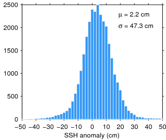
Figure 7. Histogram of flag-valid SSH anomaly over oceans and lakes for 15/08/2016. The mean ( \mu ) and standard deviation ( \sigma ) are also shown. Note that values outside [-50 50] cm are excluded from the histogram for the sake of readability but not from the computation of \mu and \sigma .
