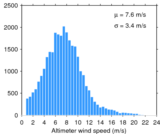
Figure 35. Histogram of science-valid wind over oceans and lakes for 15/08/2016. The mean ( \mu ) and standard deviation ( \sigma ) are also shown. Note that values larger than 24 m/s are excluded from the histogram for the sake of readability but not from the computation of \mu and \sigma .
