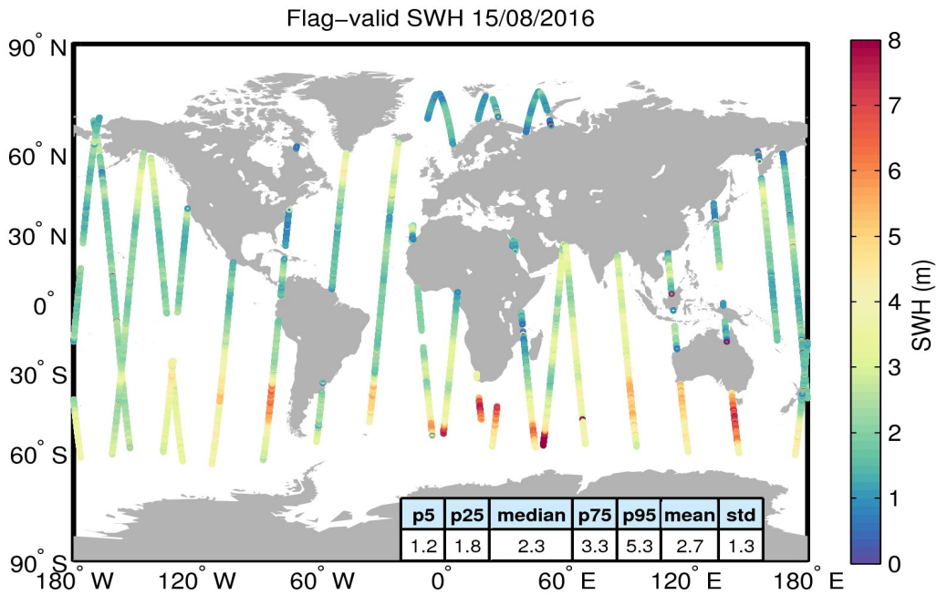
Figure 15. Geographical distribution of flag-valid SWH data over oceans and lakes for 15/08/2016. The statistical values shown in the table refer to the SWH in m and are calculated over all measurements shown in the figure.
