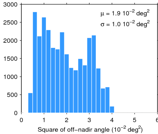
Figure 39. Histogram of flag-valid mispointing over oceans and lakes for 15/08/2016. The mean ( \mu ) and standard deviation ( \sigma ) are also shown. Note that values larger than 6 \cdot 10^{-2} \text{ deg}^2 are excluded from the histogram for the sake of readability but not from the computation of \mu and \sigma .
