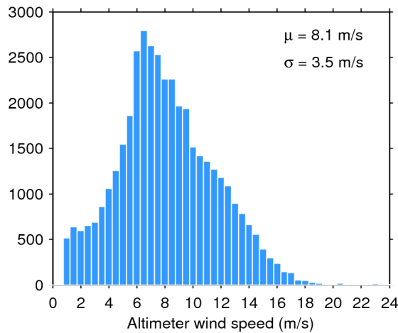
Figure 33. Histogram of flag-valid wind over oceans and lakes for 14/08/2016. The mean ( \mu ) and standard deviation ( \sigma ) are also shown. Note that values larger than 24 m/s are excluded from the histogram for the sake of readability but not from the computation of \mu and \sigma .
