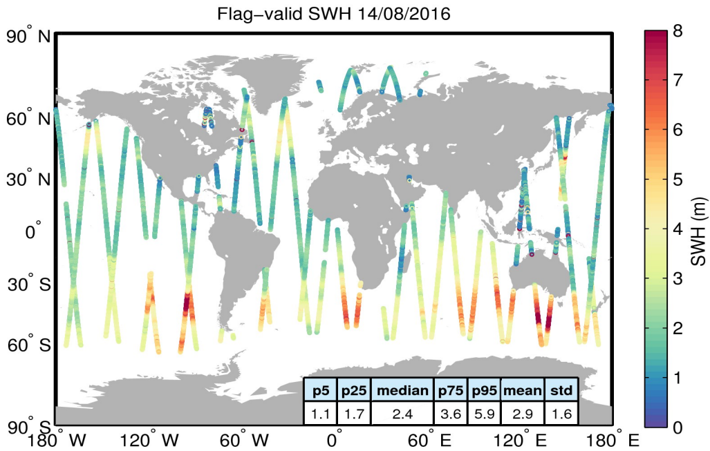
Figure 15. Geographical distribution of flag-valid SWH data over oceans and lakes for 14/08/2016. The statistical values shown in the table refer to the SWH in m and are calculated over all measurements shown in the figure.
