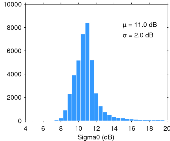
Figure 25. Histogram of flag-valid sigma0 over oceans and lakes for 14/08/2016. The mean ( \mu ) and standard deviation ( \sigma ) are also shown. Note that values outside [4 20] dB are excluded from the histogram for the sake of readability but not from the computation of \mu and \sigma .
