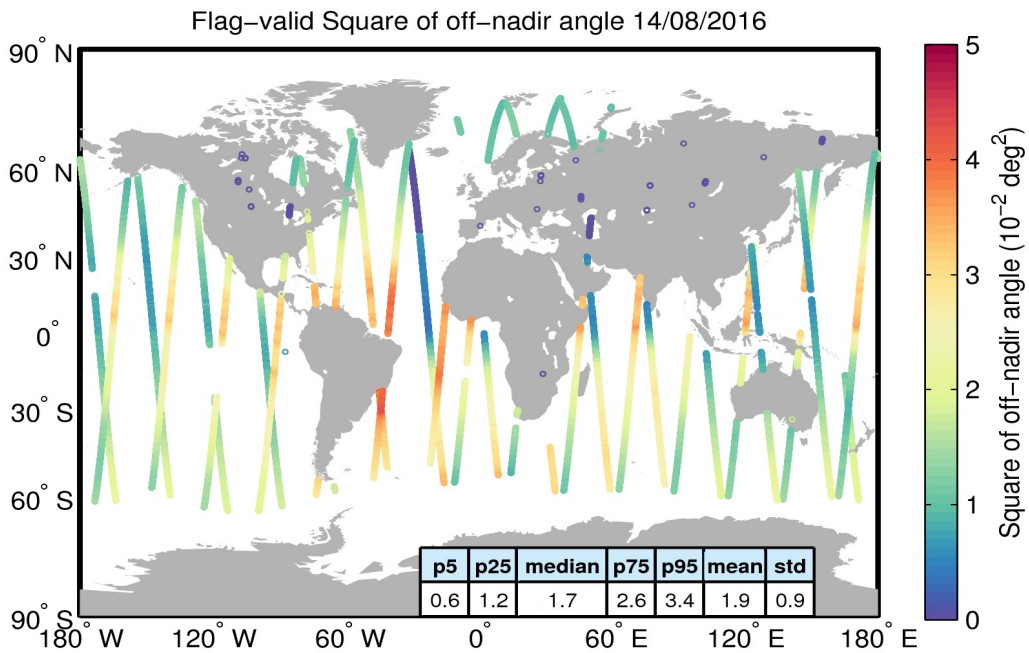
Figure 37. Geographical distribution of flag-valid mispointing data over oceans and lakes for 14/08/2016. The statistical values shown in the table refer to the mispointing in 10^{-2} deg 2 and are calculated over all measurements shown in the figure.
