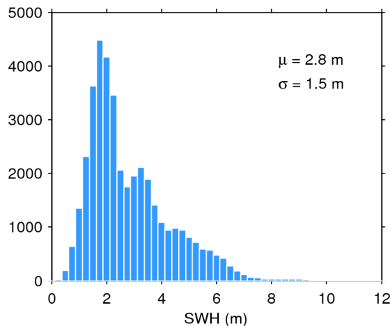
Figure 20. Histogram of science-valid SWH over oceans and lakes for 14/08/2016. The mean ( \mu ) and standard deviation ( \sigma ) are also shown. Note that values larger than 12 m are excluded from the histogram for the sake of readability but not from the computation of \mu and \sigma .
