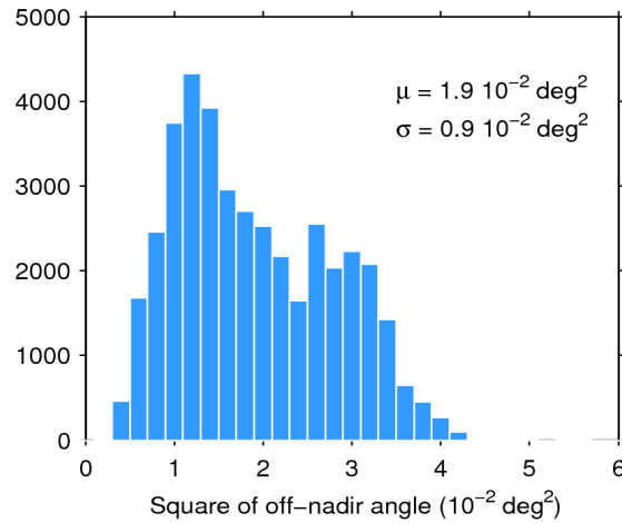
Figure 39. Histogram of flag-valid mispointing over oceans and lakes for 14/08/2016. The mean ( \mu ) and standard deviation ( \sigma ) are also shown. Note that values larger than 6 \cdot 10^{-2} \text{ deg}^2 are excluded from the histogram for the sake of readability but not from the computation of \mu and \sigma .
