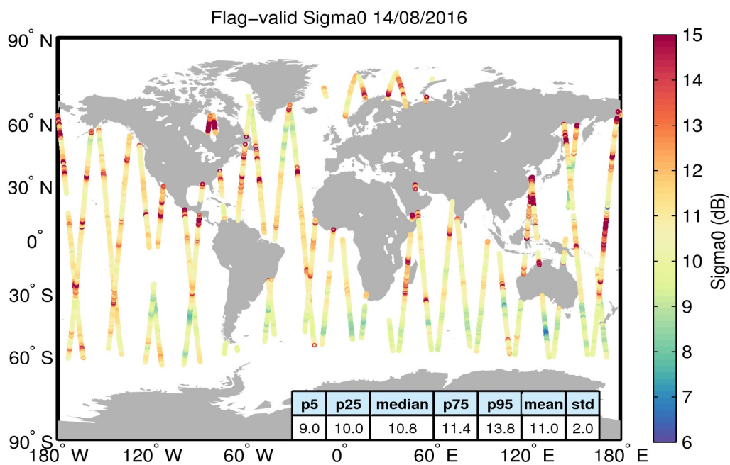
Figure 23. Geographical distribution of flag-valid sigma0 data over oceans and lakes for 14/08/2016. The statistical values shown in the table refer to the sigma0 in dB and are calculated over all measurements shown in the figure.
