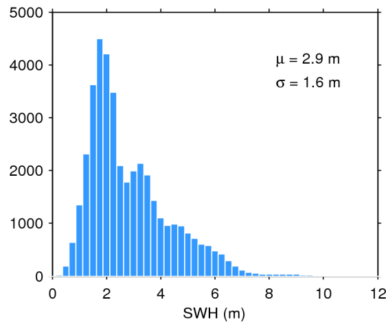
Figure 17. Histogram of flag-valid SWH over oceans and lakes for 14/08/2016. The mean ( \mu ) and standard deviation ( \sigma ) are also shown. Note that values larger than 12 m are excluded from the histogram for the sake of readability but not from the computation of \mu and \sigma .
