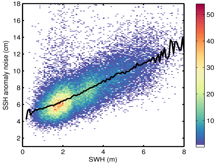
Figure 9. 2D histogram showing flag-valid SSH anomaly noise as a function of SWH for 14/08/2016. The black line denotes the median SSH anomaly noise as a function of SWH.
