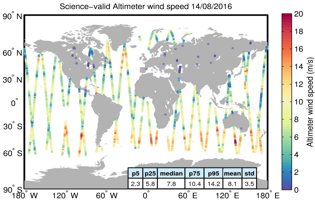
Figure 34. Geographical distribution of science-valid wind data over oceans and lakes for 14/08/2016. The statistical values shown in the table refer to the wind in m/s and are calculated over all measurements shown in the figure. Gray circles denote records that have been rejected based on the editing criteria described in Table 5.
