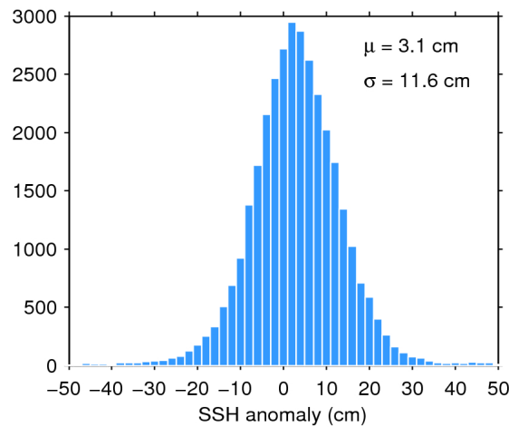
Figure 11. Histogram of science-valid SSH anomaly over oceans and lakes for 14/08/2016. The mean ( \mu ) and standard deviation ( \sigma ) are also shown. Note that values outside [-50 50] cm are excluded from the histogram for the sake of readability but not from the computation of \mu and \sigma .
