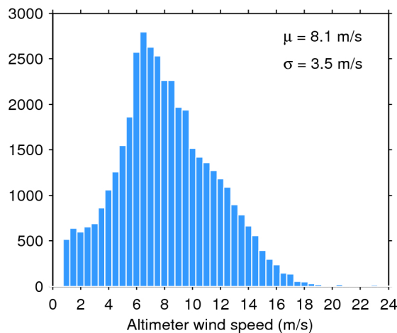
Figure 35. Histogram of science-valid wind over oceans and lakes for 14/08/2016. The mean ( \mu ) and standard deviation ( \sigma ) are also shown. Note that values larger than 24 m/s are excluded from the histogram for the sake of readability but not from the computation of \mu and \sigma .
