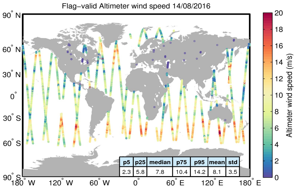
Figure 31. Geographical distribution of flag-valid wind data over oceans and lakes for 14/08/2016. The statistical values shown in the table refer to the wind in m/s and are calculated over all measurements shown in the figure.
