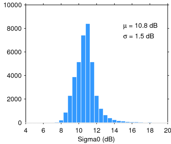
Figure 28. Histogram of science-valid sigma0 over oceans and lakes for 14/08/2016. The mean ( \mu ) and standard deviation ( \sigma ) are also shown. Note that values outside [4 20] dB are excluded from the histogram for the sake of readability but not from the computation of \mu and \sigma .
