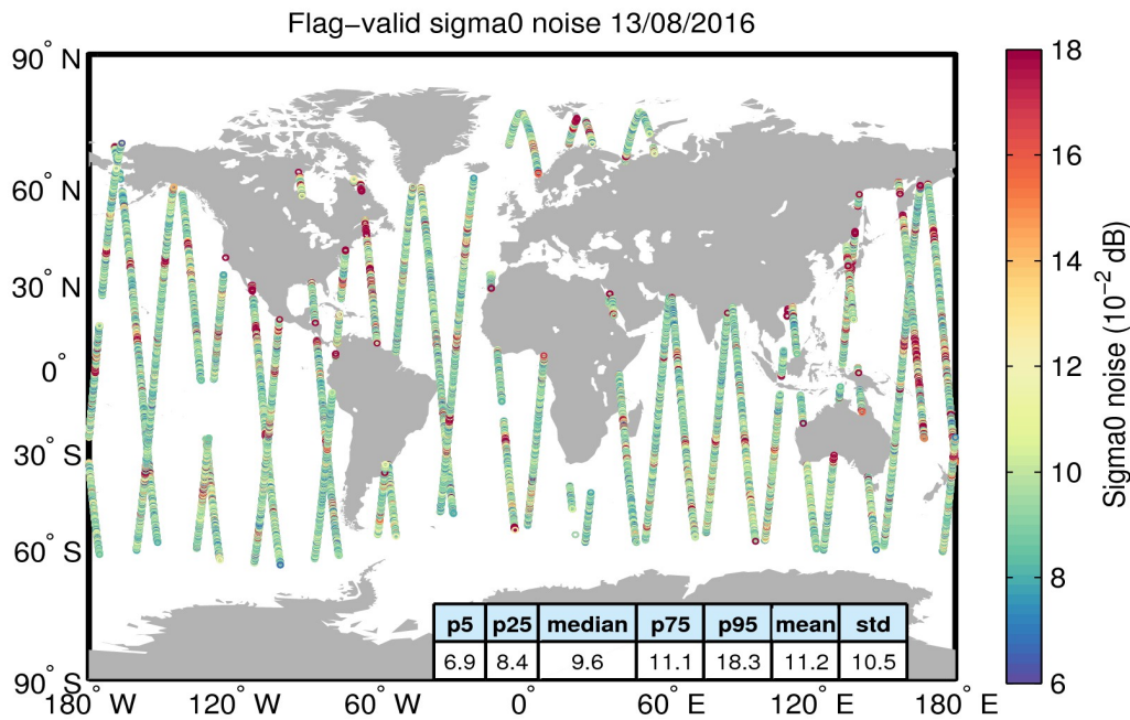
Figure 26. Geographical distribution of flag-valid 20-Hz sigma0 measurement noise over oceans and lakes for 13/08/2016. The statistical values shown in the table refer to the sigma0 noise and are calculated over all measurements shown in the figure.
