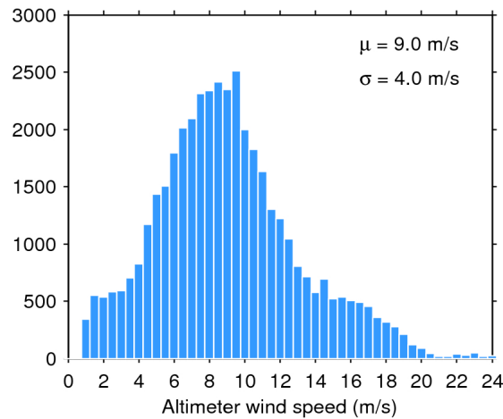
Figure 33. Histogram of flag-valid wind over oceans and lakes for 13/08/2016. The mean ( \mu ) and standard deviation ( \sigma ) are also shown. Note that values larger than 24 m/s are excluded from the histogram for the sake of readability but not from the computation of \mu and \sigma .
