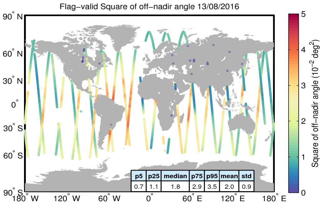
Figure 37. Geographical distribution of flag-valid mispointing data over oceans and lakes for 13/08/2016. The statistical values shown in the table refer to the mispointing in 10^{-2} deg 2 and are calculated over all measurements shown in the figure.
