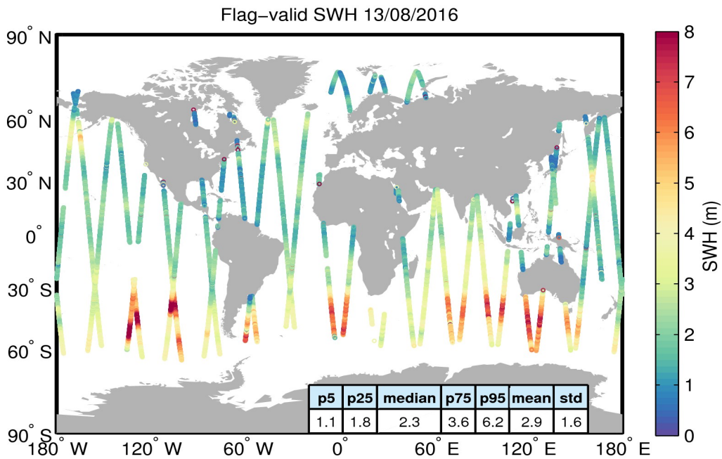
Figure 15. Geographical distribution of flag-valid SWH data over oceans and lakes for 13/08/2016. The statistical values shown in the table refer to the SWH in m and are calculated over all measurements shown in the figure.
