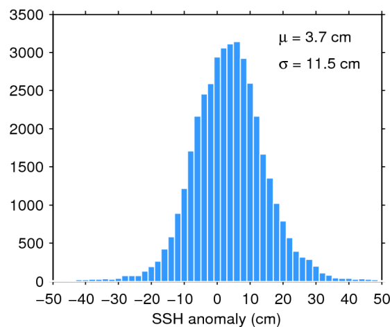
Figure 11. Histogram of science-valid SSH anomaly over oceans and lakes for 13/08/2016. The mean ( \mu ) and standard deviation ( \sigma ) are also shown. Note that values outside [-50 50] cm are excluded from the histogram for the sake of readability but not from the computation of \mu and \sigma .
