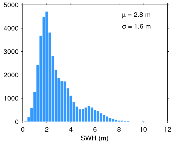
Figure 20. Histogram of science-valid SWH over oceans and lakes for 13/08/2016. The mean ( \mu ) and standard deviation ( \sigma ) are also shown. Note that values larger than 12 m are excluded from the histogram for the sake of readability but not from the computation of \mu and \sigma .
