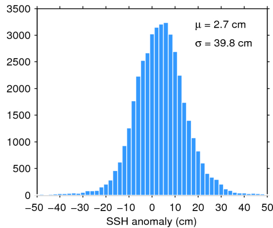
Figure 7. Histogram of flag-valid SSH anomaly over oceans and lakes for 13/08/2016. The mean ( \mu ) and standard deviation ( \sigma ) are also shown. Note that values outside [-50 50] cm are excluded from the histogram for the sake of readability but not from the computation of \mu and \sigma .
