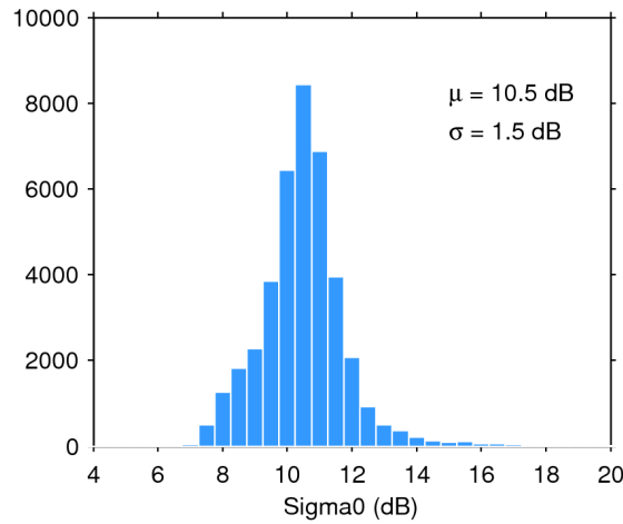
Figure 28. Histogram of science-valid sigma0 over oceans and lakes for 13/08/2016. The mean ( \mu ) and standard deviation ( \sigma ) are also shown. Note that values outside [4 20] dB are excluded from the histogram for the sake of readability but not from the computation of \mu and \sigma .
