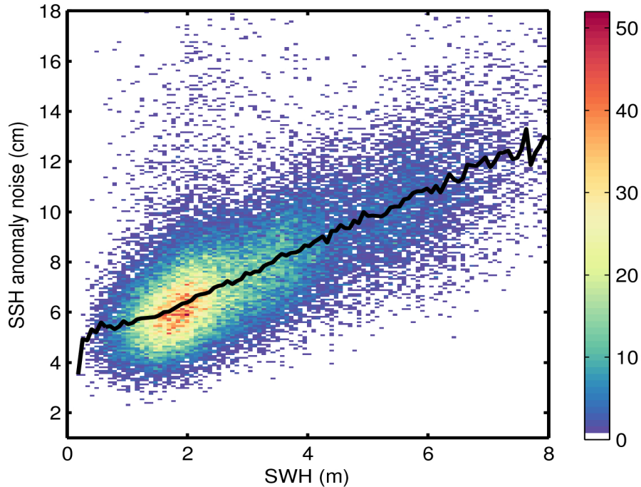
Figure 9. 2D histogram showing flag-valid SSH anomaly noise as a function of SWH for 13/08/2016. The black line denotes the median SSH anomaly noise as a function of SWH.
