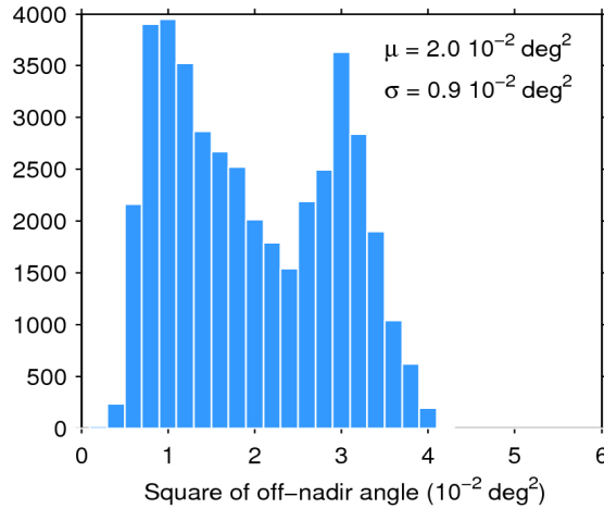
Figure 39. Histogram of flag-valid mispointing over oceans and lakes for 13/08/2016. The mean ( \mu ) and standard deviation ( \sigma ) are also shown. Note that values larger than 6 \cdot 10^{-2} \text{ deg}^2 are excluded from the histogram for the sake of readability but not from the computation of \mu and \sigma .
