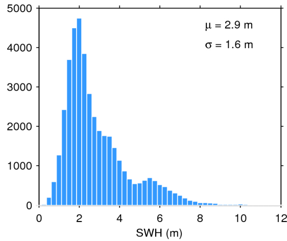
Figure 17. Histogram of flag-valid SWH over oceans and lakes for 13/08/2016. The mean ( \mu ) and standard deviation ( \sigma ) are also shown. Note that values larger than 12 m are excluded from the histogram for the sake of readability but not from the computation of \mu and \sigma .
