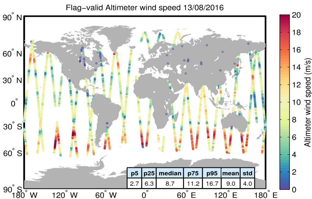
Figure 31. Geographical distribution of flag-valid wind data over oceans and lakes for 13/08/2016. The statistical values shown in the table refer to the wind in m/s and are calculated over all measurements shown in the figure.
