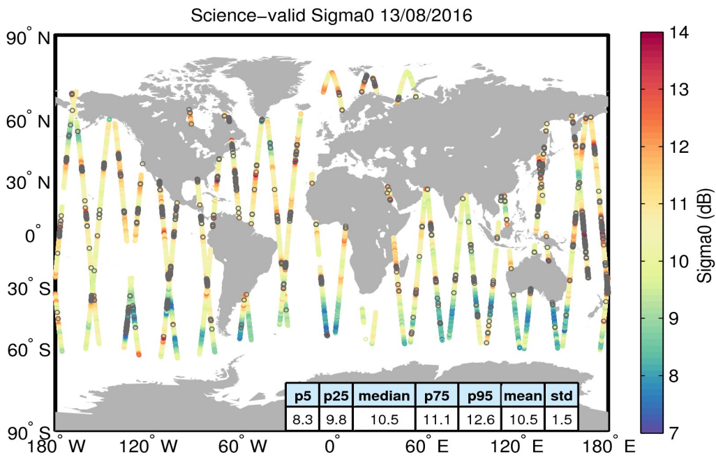
Figure 27. Geographical distribution of science-valid sigma0 data over oceans and lakes for 13/08/2016. The statistical values shown in the table refer to the sigma0 in dB and are calculated over all measurements shown in the figure. Gray circles denote records that have been rejected based on the editing criteria described in Table 4.
