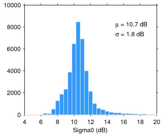
Figure 25. Histogram of flag-valid sigma0 over oceans and lakes for 13/08/2016. The mean ( \mu ) and standard deviation ( \sigma ) are also shown. Note that values outside [4 20] dB are excluded from the histogram for the sake of readability but not from the computation of \mu and \sigma .
