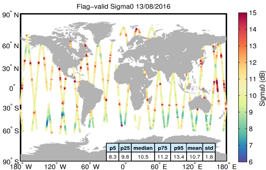
Figure 23. Geographical distribution of flag-valid sigma0 data over oceans and lakes for 13/08/2016. The statistical values shown in the table refer to the sigma0 in dB and are calculated over all measurements shown in the figure.
